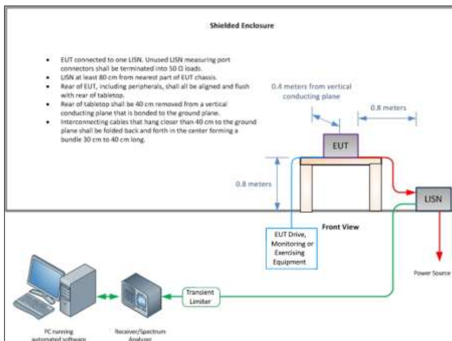
Figure 1 - Conducted Disturbance
