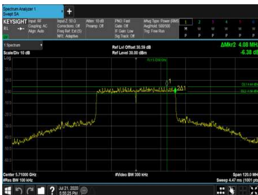
Figure 890 - 5710 MHz - 6 dB DTS Bandwidth
