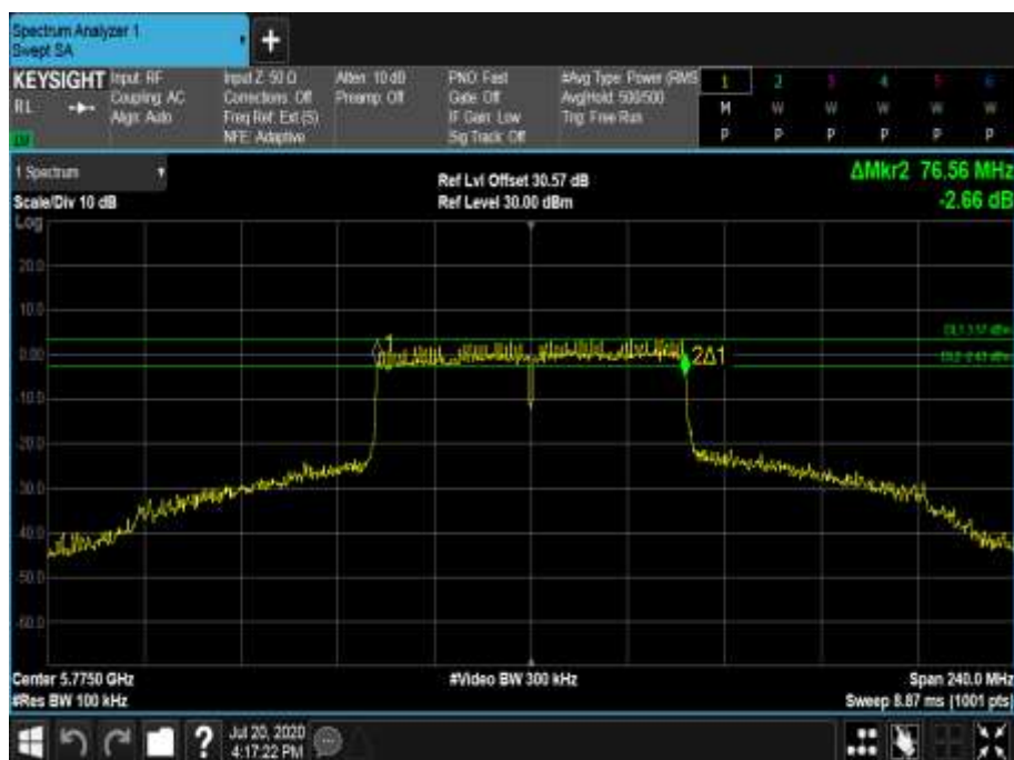
Figure 935 - 5775 MHz - 6 dB DTS Bandwidth
