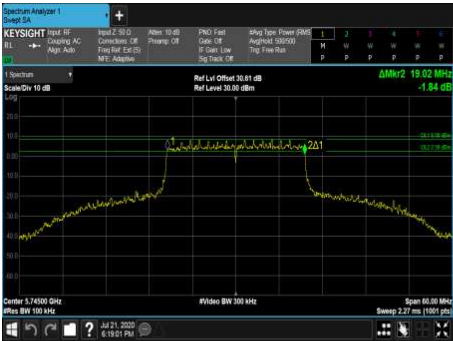
Figure 815 - 5745 MHz - 6 dB DTS Bandwidth
