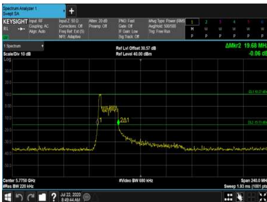
Figure 981 - 5775 MHz - 26 dB Emission Bandwidth
