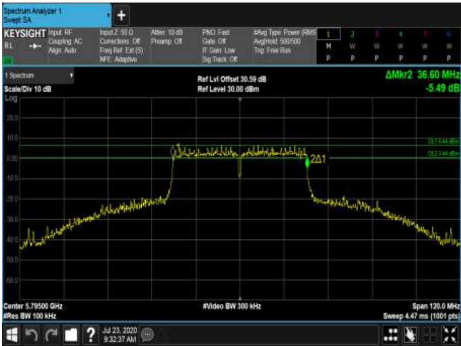
Figure 866 - 5795 MHz - 6 dB DTS Bandwidth
