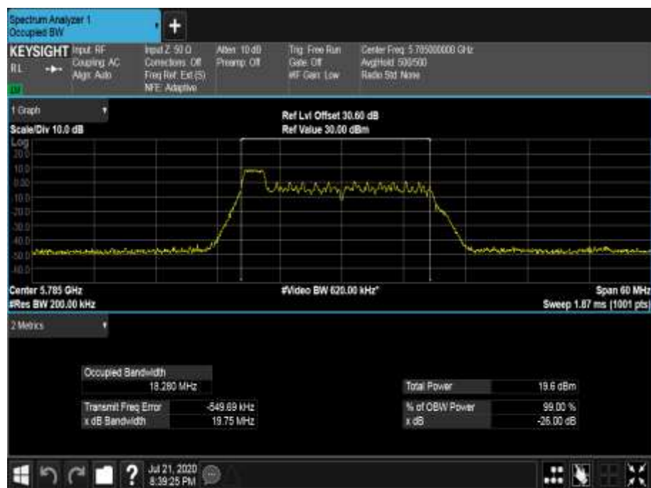
Figure 799 - 5785 MHz - 99% Occupied Bandwidth
