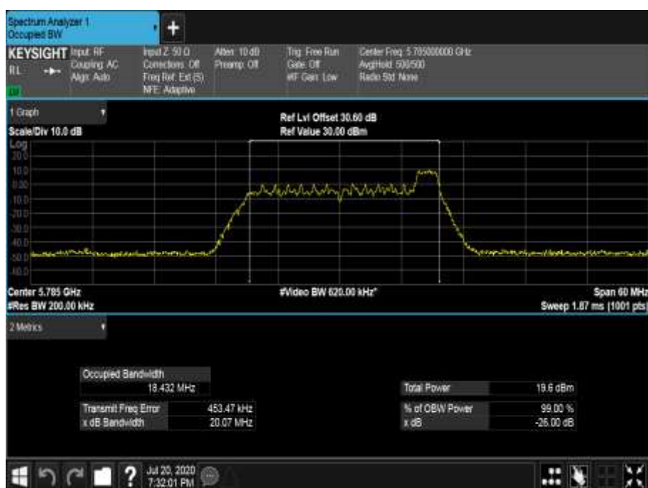
Figure 778 - 5785 MHz - 99% Occupied Bandwidth
