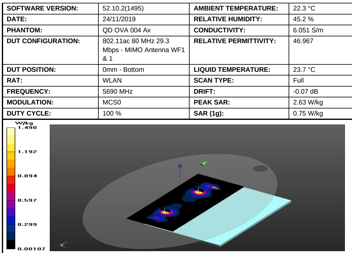
Figure 26: SAR Body Testing Results for the A2179 at 5690 MHz.
