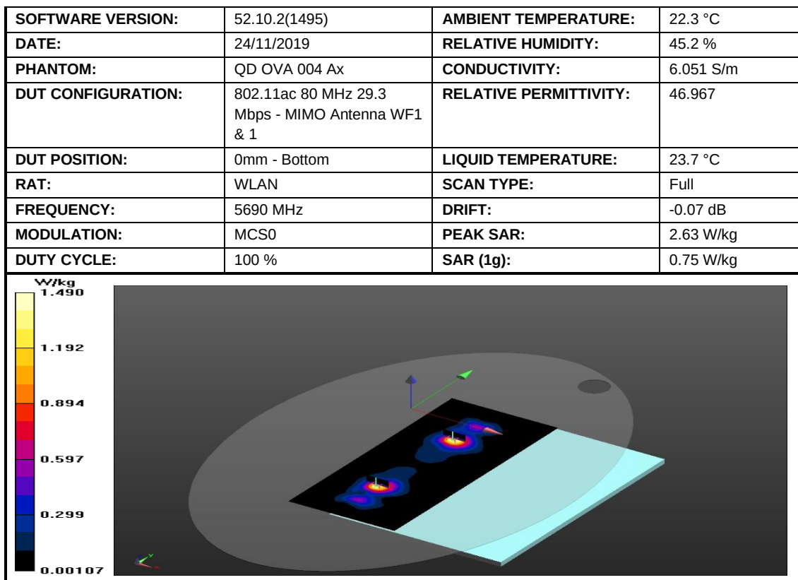
Figure 26: SAR Body Testing Results for the A2179 at 5690 MHz.
