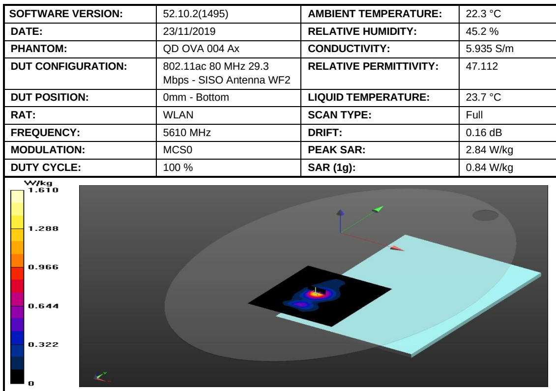
Figure 21: SAR Body Testing Results for the A2179 at 5610 MHz.
