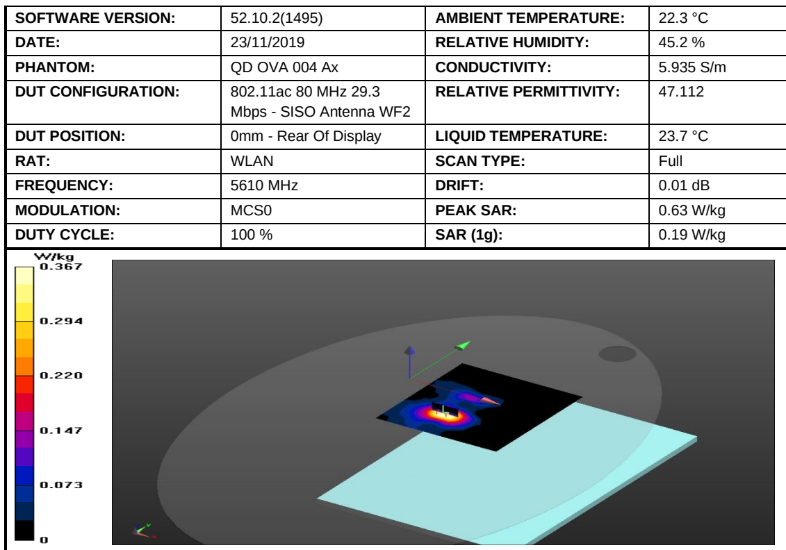
Figure 22: SAR Body Testing Results for the A2179 at 5610 MHz.
