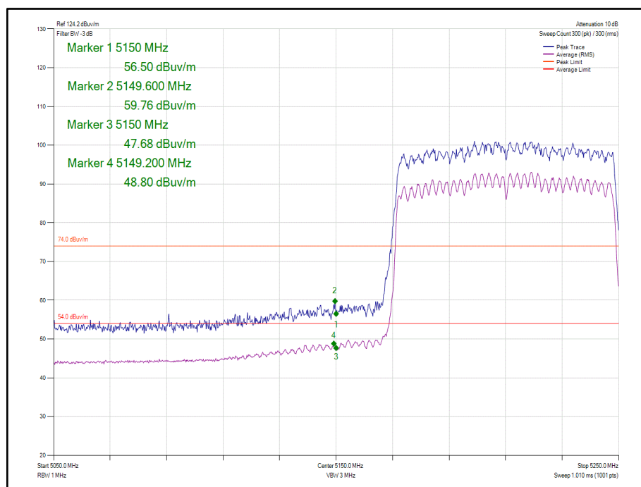
Figure 443 - 802.11ac VHT80 CDD Cores 0-1- 5210 MHz Band Edge Frequency 5150 MHz
