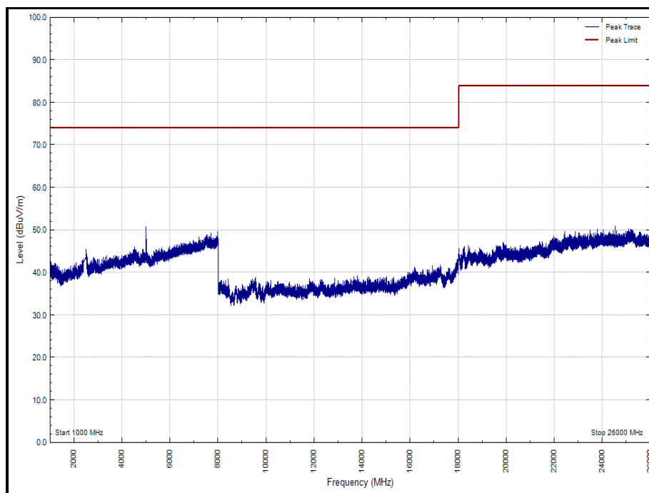
Figure 47 - 2480 MHz - 1 GHz to 26 GHz, Polarity: Horizontal (Peak)
