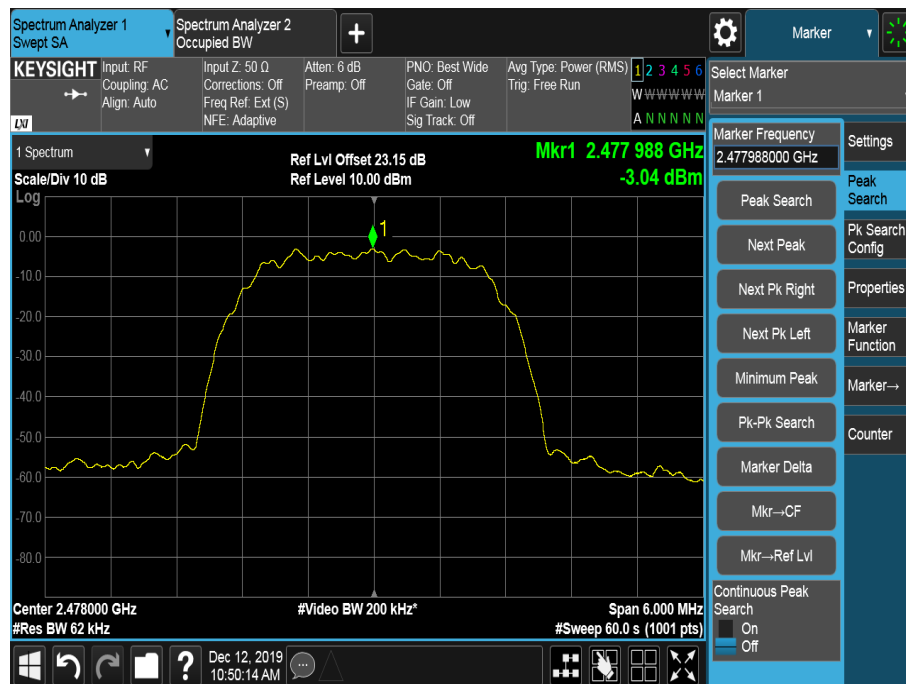
Figure 33 – 2478 MHz
