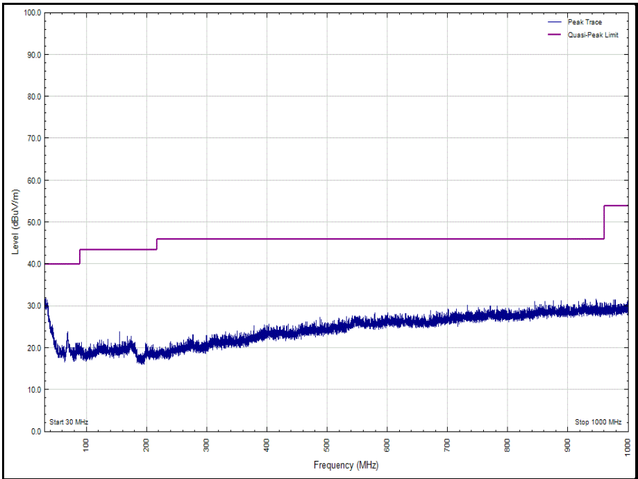
Figure 38 - 2440 MHz, 30 MHz to 1 GHz, Polarity: Vertical
