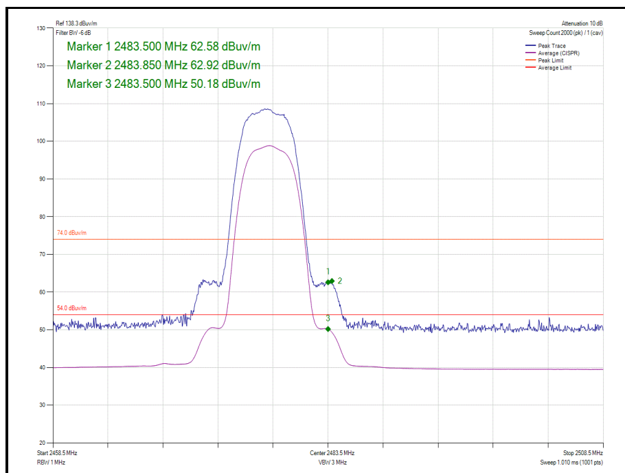
Figure 68 - Static - 8-GFSK/8DH5 - 2478 MHz - Band Edge Frequency 2483.5 MHz
