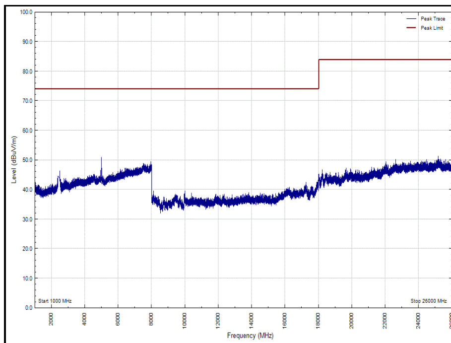
Figure 39 - 2402 MHz - 1 GHz to 26 GHz, Polarity: Horizontal (Peak)
