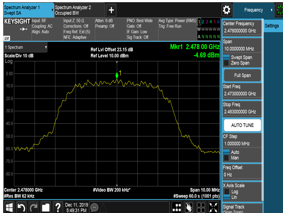
Figure 36 – 2478 MHz
