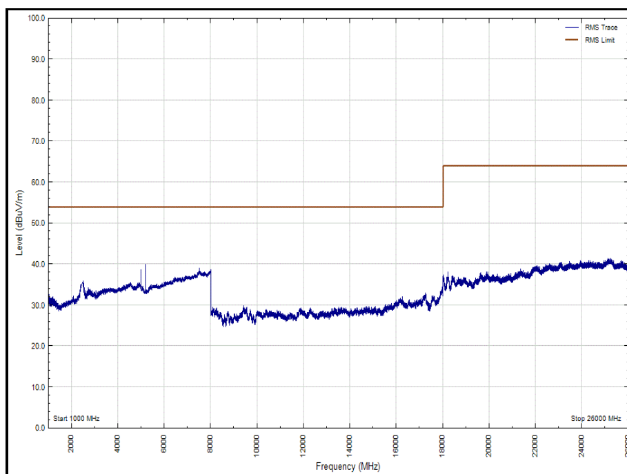
Figure 44 - 2440 MHz - 1 GHz to 26 GHz, Polarity: Horizontal (Average)
