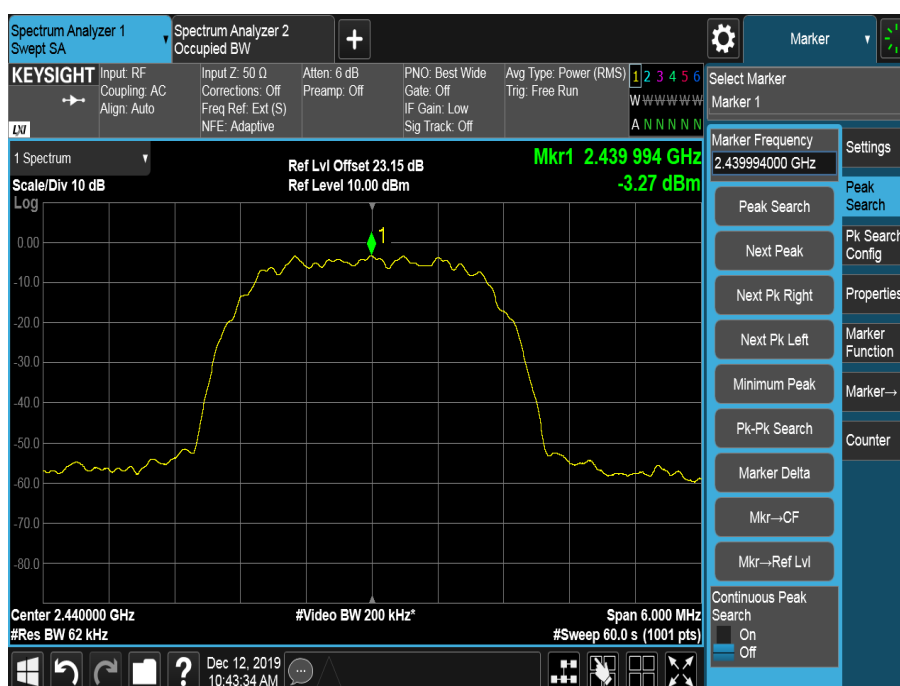
Figure 32 – 2440 MHz
