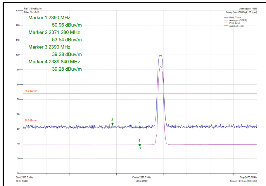
Figure 63 - Static - GFSK/8DH5 - 2404 MHz - Band Edge Frequency 2390.0 MHz
