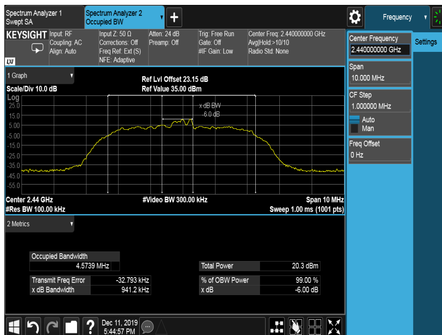
Figure 17 - 2440 MHz – Emission Bandwidth
