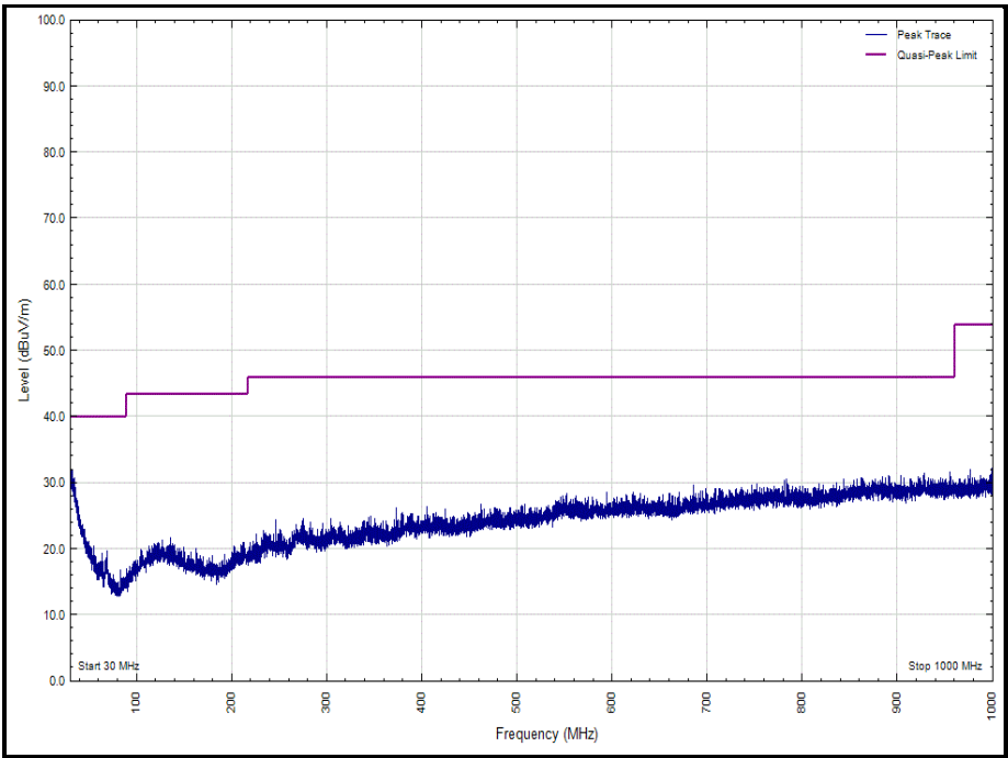
Figure 37 - 2440 MHz, 30 MHz to 1 GHz, Polarity: Horizontal
