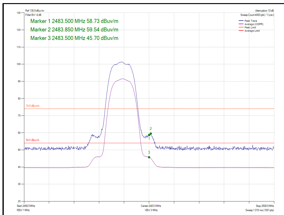
Figure 64 - Static - 8-GFSK/8DH5 - 2478 MHz - Band Edge Frequency 2483.5 MHz
