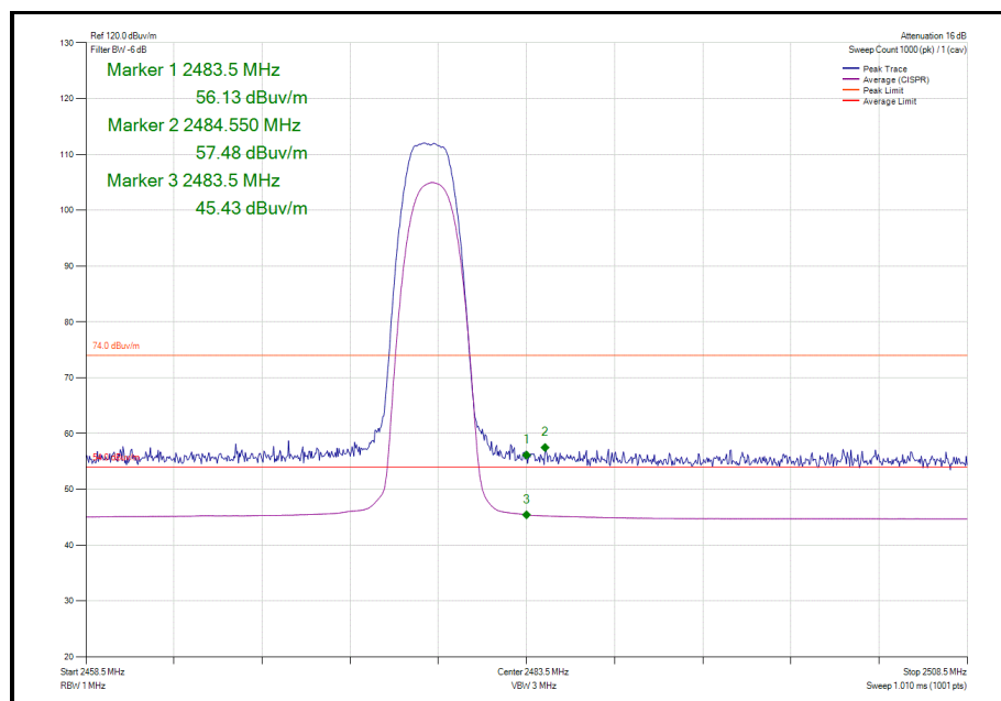
Figure 66 - Static - GFSK/8DH5 - 2478 MHz - Band Edge Frequency 2483.5 MHz
