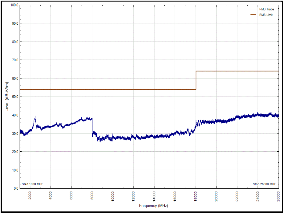
Figure 42 - 2402 MHz - 1 GHz to 26 GHz, Polarity: Vertical (Average)
