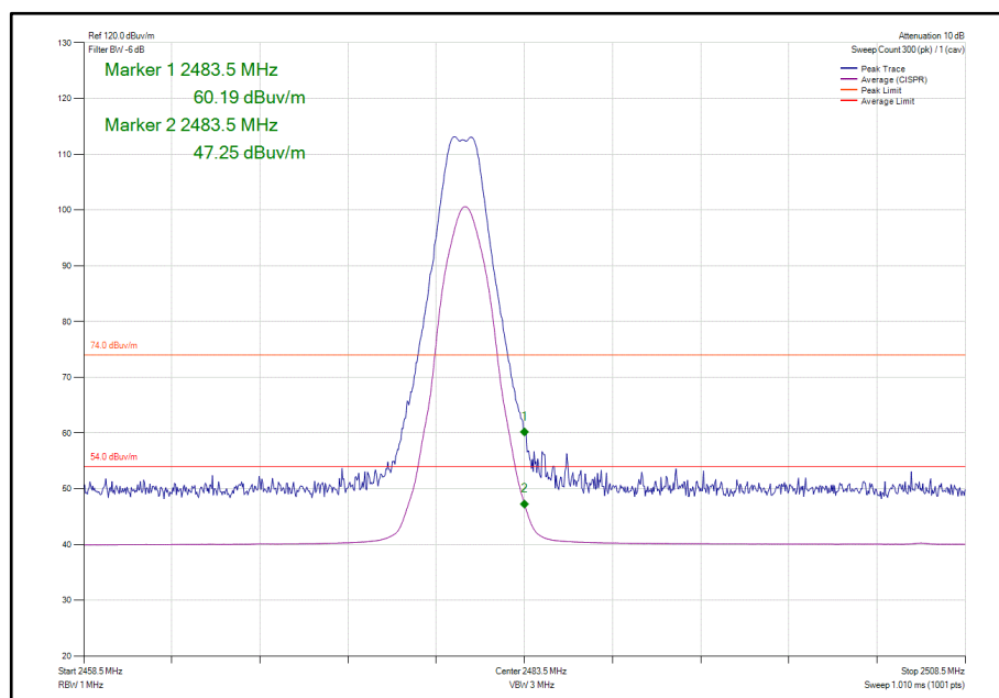
Figure 60 – GFSK/DH1 - 2480 MHz - Band Edge Frequency 2483.5 MHz
