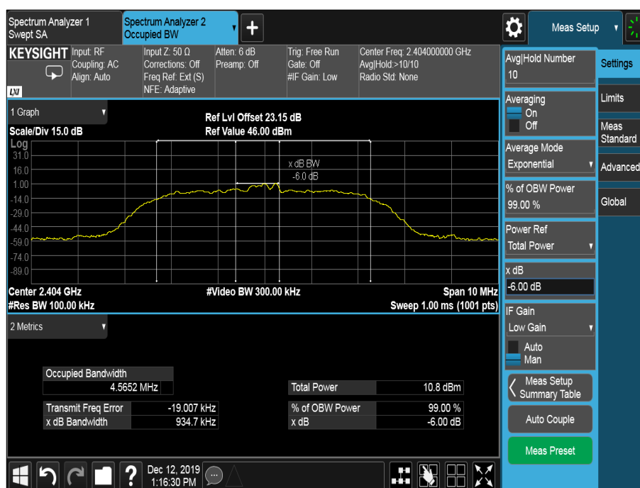
Figure 10 - 2404 MHz – Emission Bandwidth
