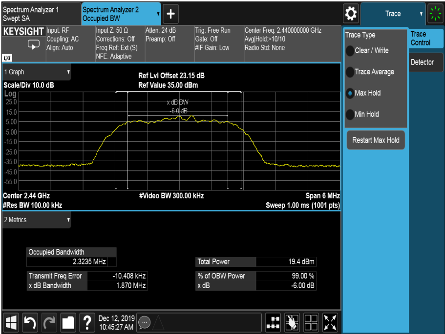
Figure 14 - 2440 MHz – Emission Bandwidth
