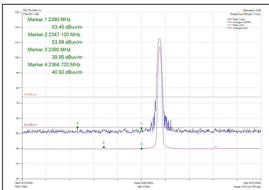
Figure 57 – GFSK/DH1 - 2402 MHz - Band Edge Frequency 2390.0 MHz
