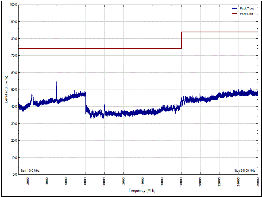
Figure 41 - 2402 MHz - 1 GHz to 26 GHz, Polarity: Vertical (Peak)
