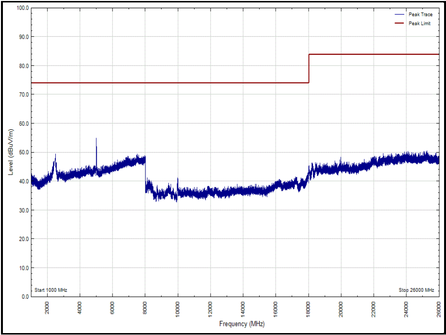
Figure 45 - 2440 MHz - 1 GHz to 26 GHz, Polarity: Vertical (Peak)
