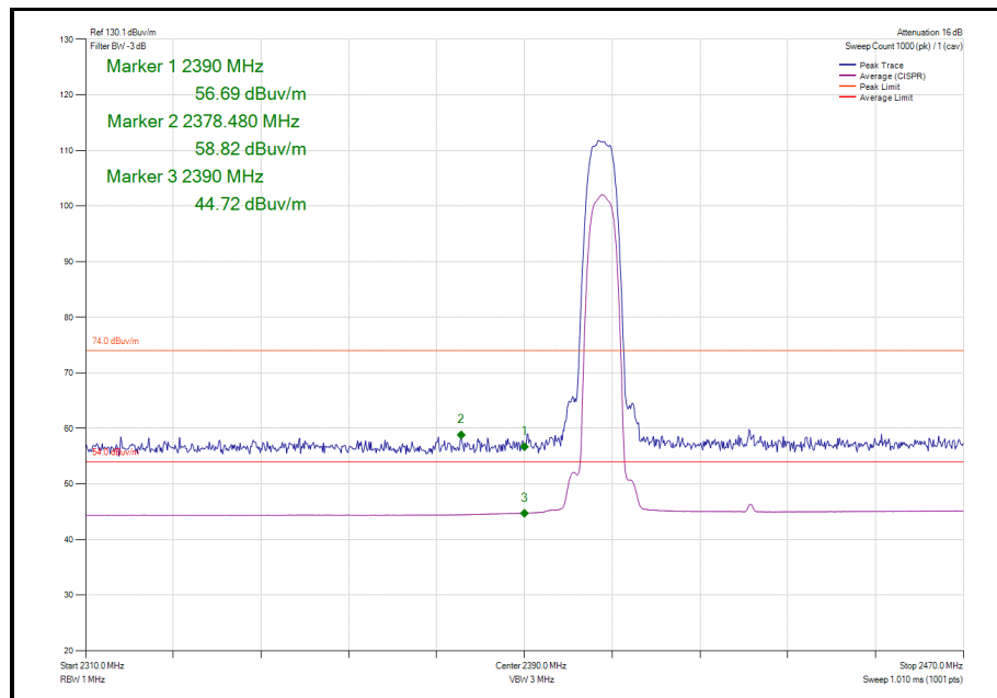
Figure 67 - Static - GFSK/8DH5 - 2404 MHz - Band Edge Frequency 2390.0 MHz
