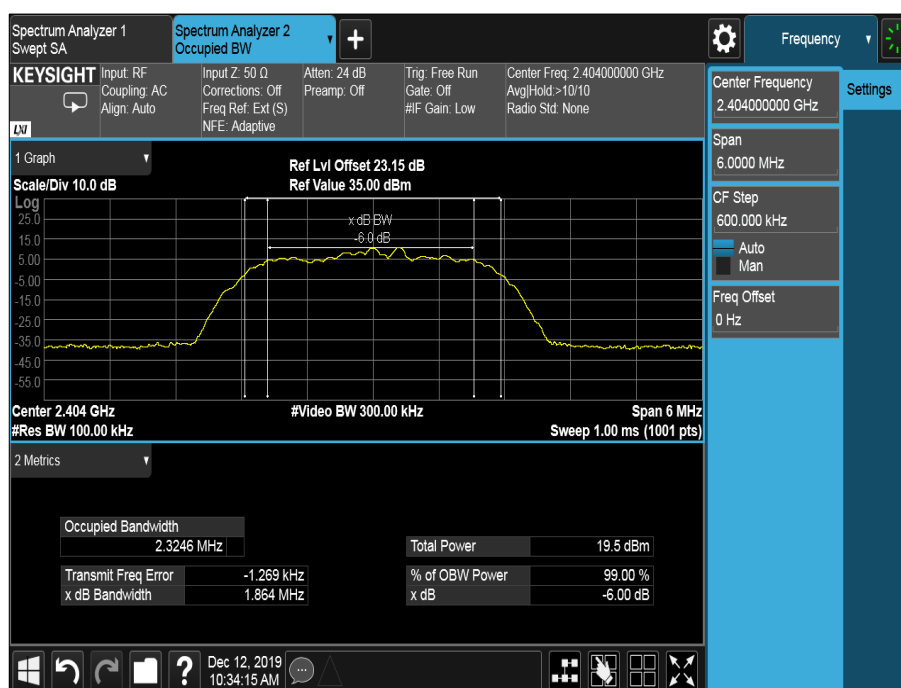
Figure 13 - 2404 MHz – Emission Bandwidth
