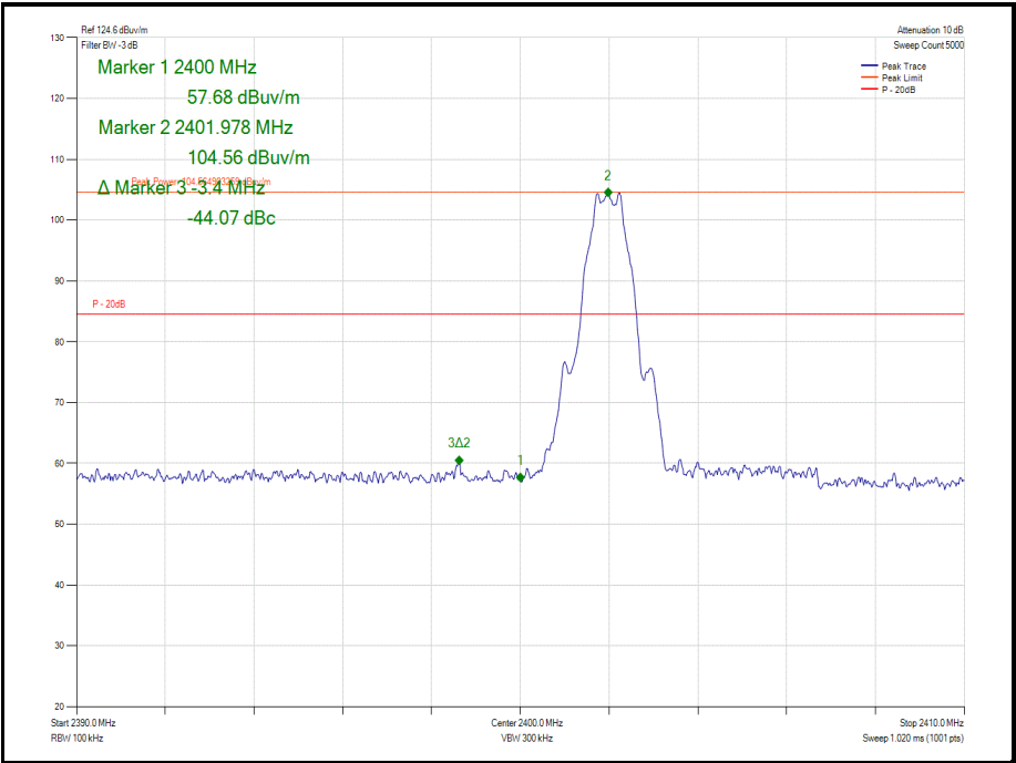
Figure 51 - GFSK/DH1- 2402 MHz – Band Edge Frequency 2400.0 MHz
