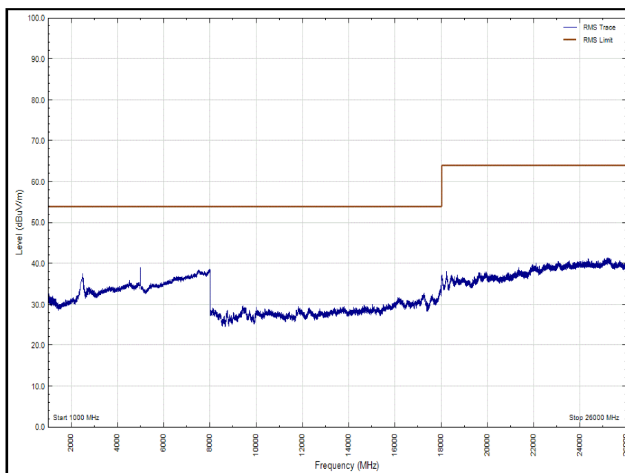
Figure 48 - 2480 MHz - 1 GHz to 26 GHz, Polarity: Horizontal (Average)
