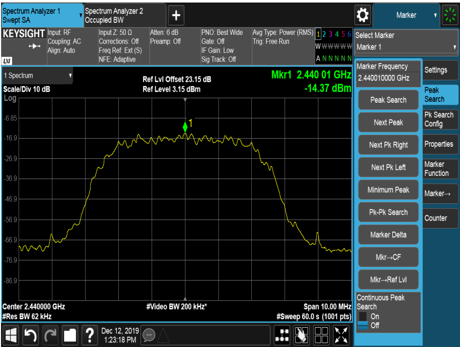
Figure 29 – 2440 MHz
