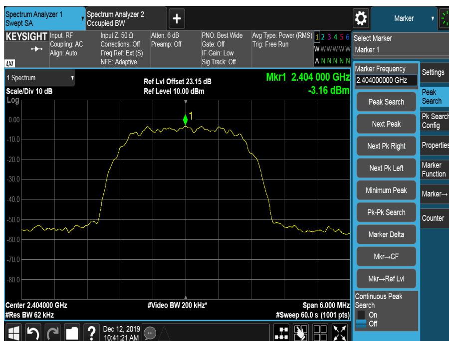
Figure 31 – 2404 MHz
