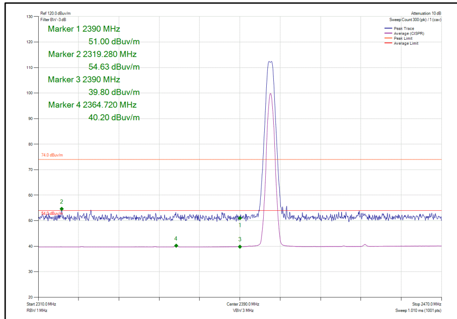
Figure 59 – GFSK/DH1 - 2402 MHz - Band Edge Frequency 2390.0 MHz
