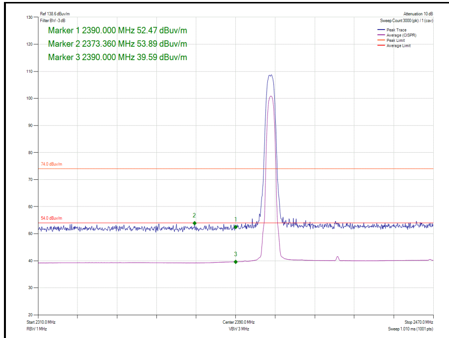
Figure 65 - Static - GFSK/4DH5 - 2404 MHz - Band Edge Frequency 2390.0 MHz
