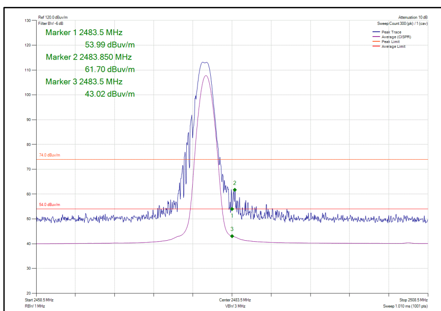
Figure 58 – GFSK/DH1 - 2480 MHz - Band Edge Frequency 2483.5 MHz
