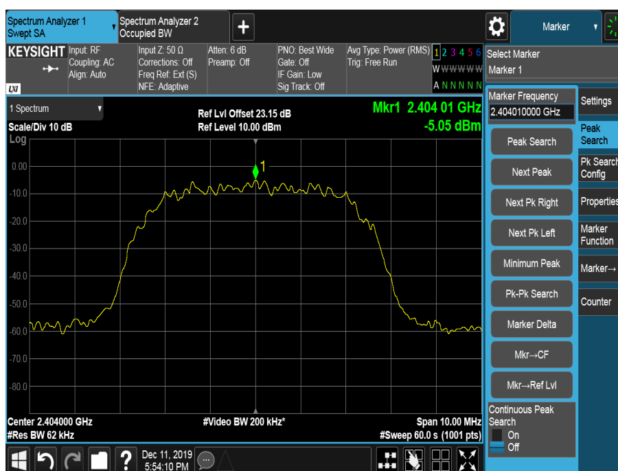
Figure 34 – 2404 MHz
