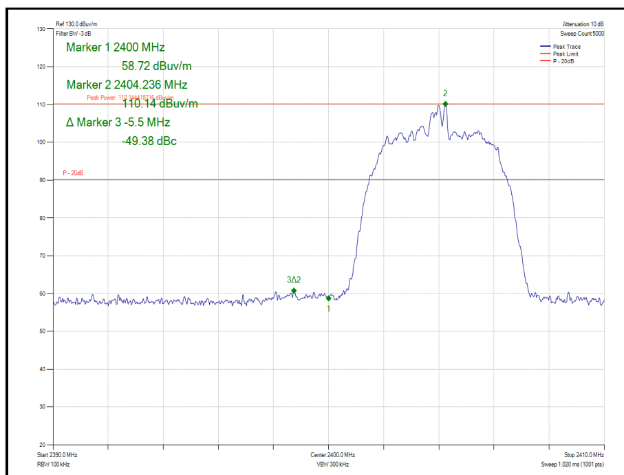
Figure 56 - GFSK/8DH5 - 2404 MHz - Band Edge Frequency 2400.0 MHz (Plot should show P- 30dB limit in place of P- 20dB)
