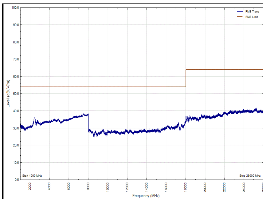
Figure 40 - 2402 MHz - 1 GHz to 26 GHz, Polarity: Horizontal (Average)
