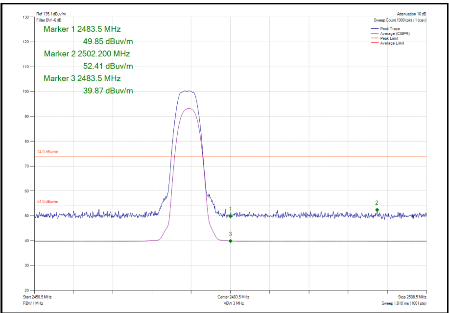
Figure 62 - Static - GFSK/4DH5 - 2478 MHz - Band Edge Frequency 2483.5 MHz
