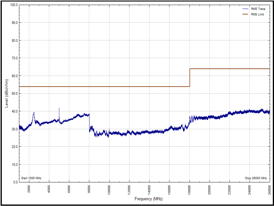
Figure 46 - 2440 MHz - 1 GHz to 26 GHz, Polarity: Vertical (Average)
