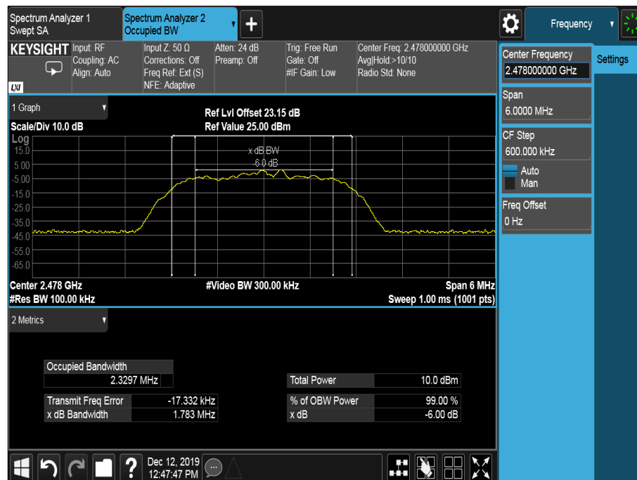
Figure 9 - 2478 MHz – Emission Bandwidth
