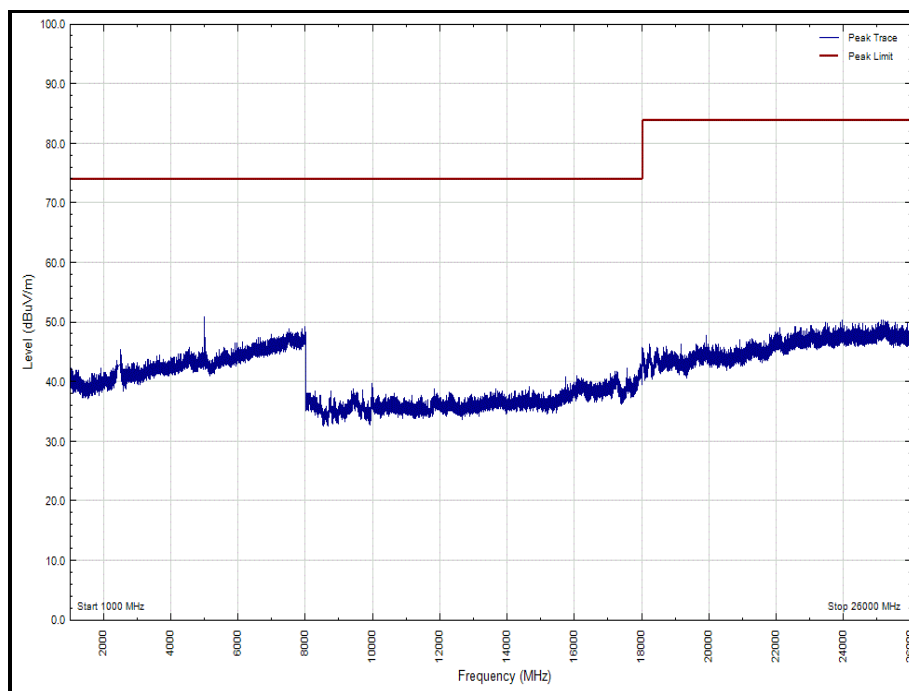
Figure 43 - 2440 MHz - 1 GHz to 26 GHz, Polarity: Horizontal (Peak)
