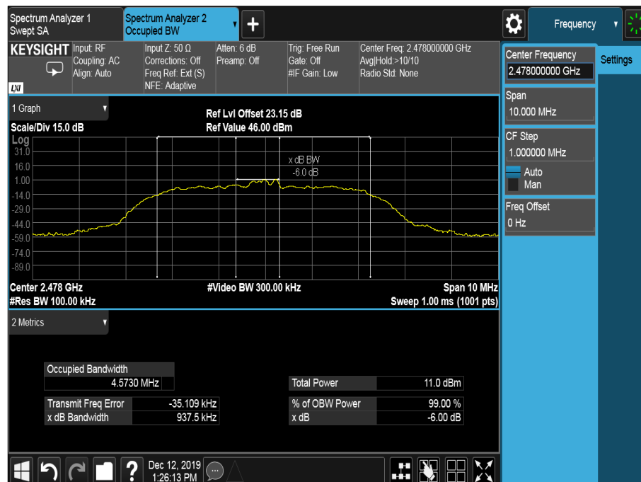
Figure 12 - 2478 MHz – Emission Bandwidth
