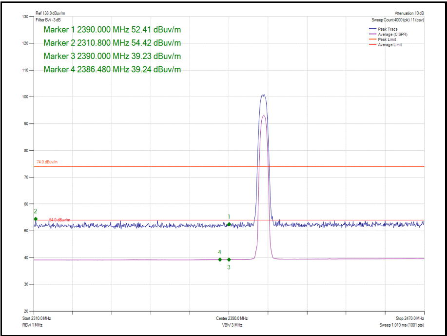
Figure 61 - Static - GFSK/4DH5 - 2404 MHz - Band Edge Frequency 2390.0 MHz
