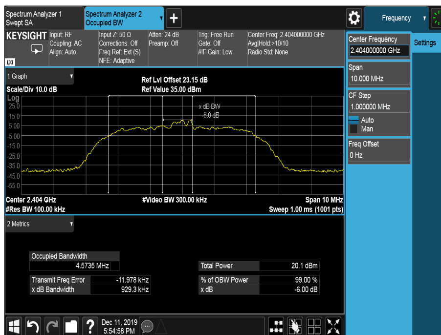
Figure 16 - 2404 MHz – Emission Bandwidth
