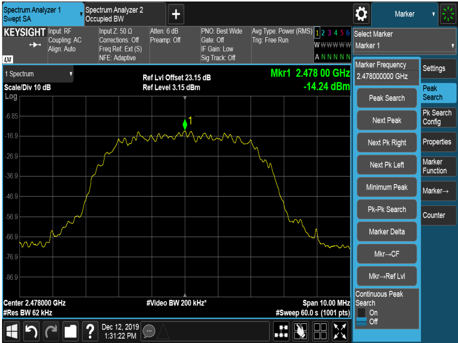
Figure 30 – 2478 MHz
