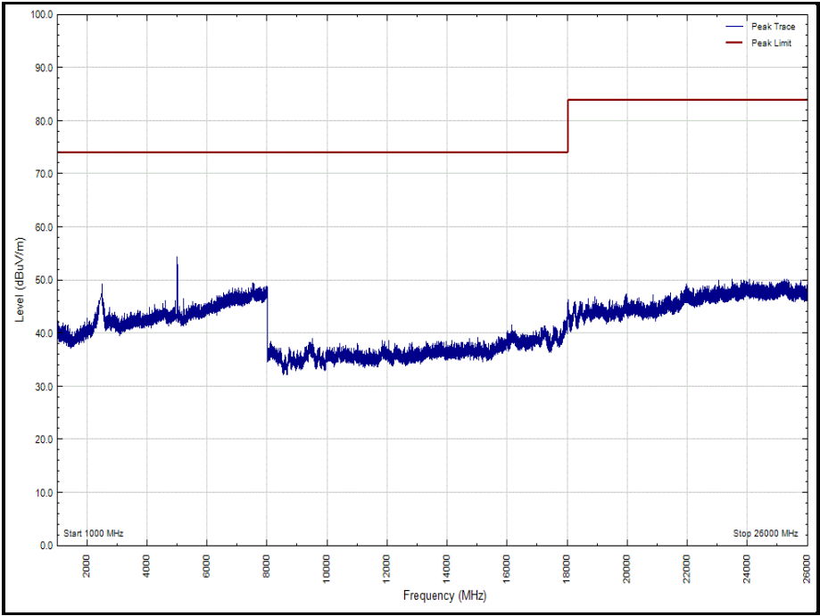
Figure 49 - 2480 MHz - 1 GHz to 26 GHz, Polarity: Vertical (Peak)
