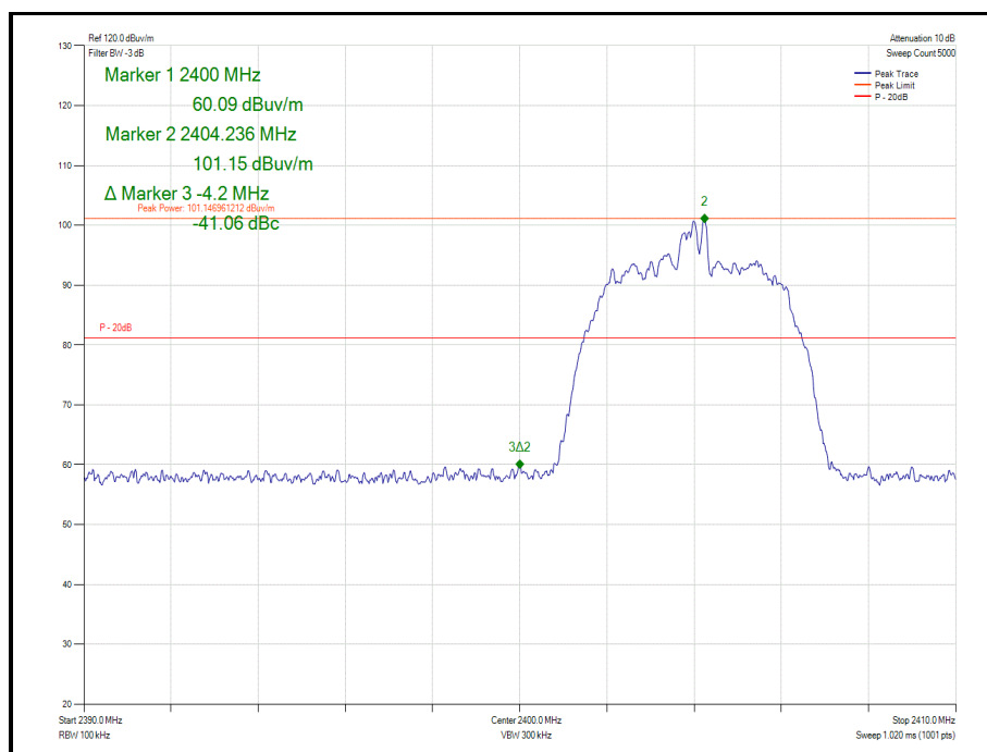
Figure 54 - GFSK/8DH5 - 2404 MHz - Band Edge Frequency 2400.0 MHz (Plot should show P- 30dB limit in place of P- 20dB)
