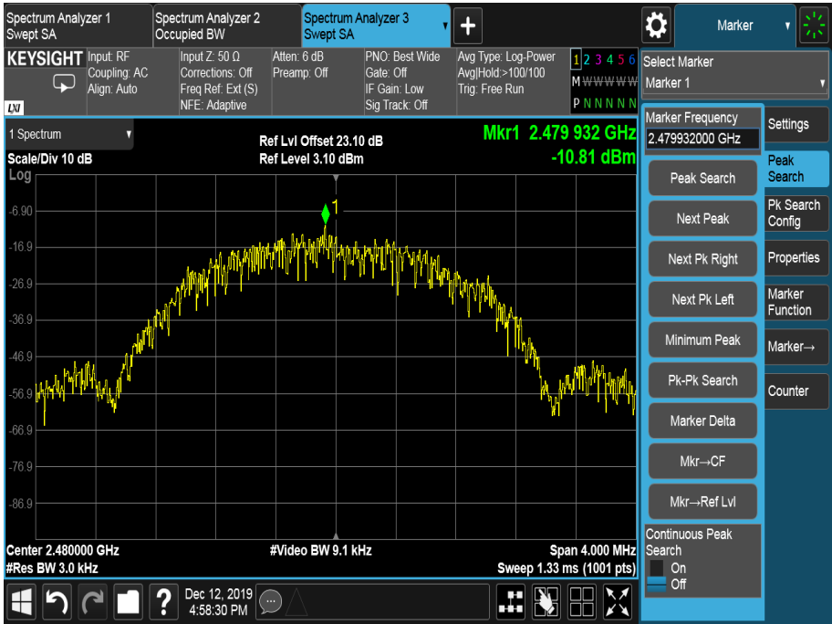
Figure 24 – 2480 MHz
