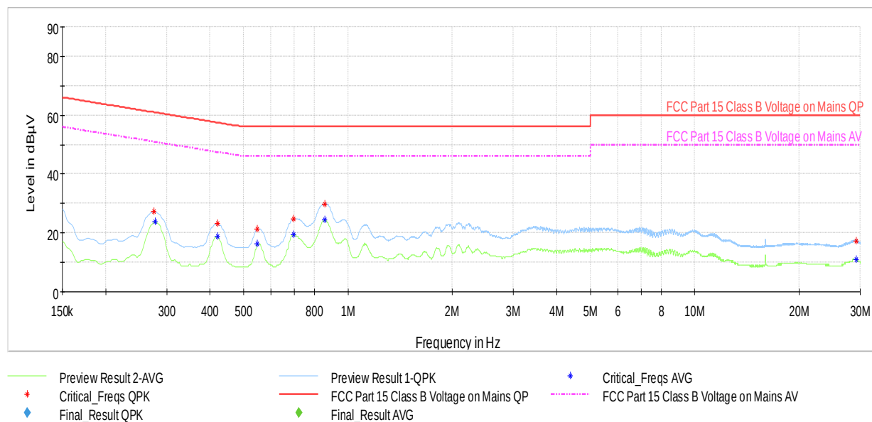
Plot 7-29. AC Line Conducted Plot with Bluetooth LE (L1, with AC/DC Adapter)
