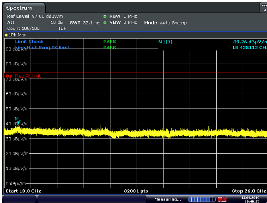
Plot 7-38. Radiated Spurious Plot above 18GHz (GFSK ePA – Ch. 39, Pol. H)
