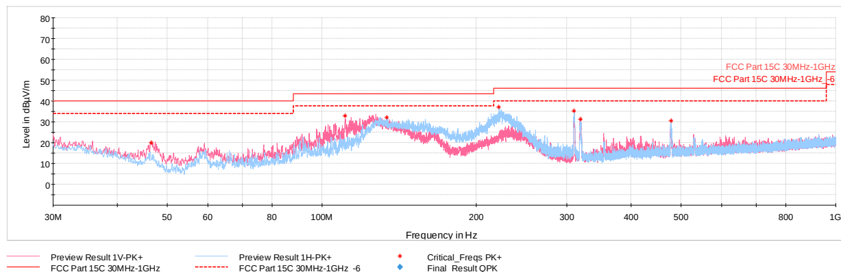
Plot 7-48. Radiated Spurious Plot below 1GHz (2.4GHz – 5GHz), with Laptop
