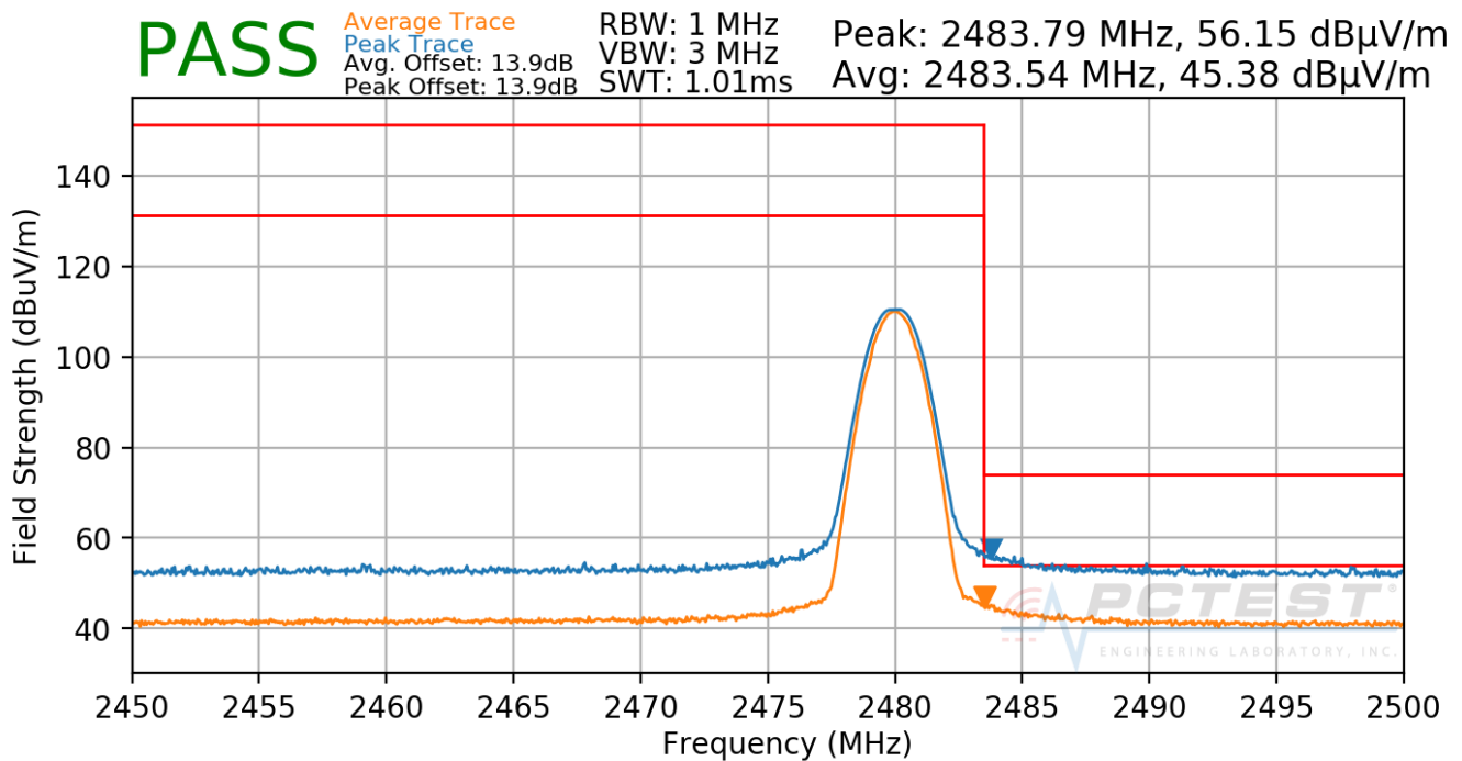
Plot 7-45. Radiated Restricted Upper Band Edge Measurement
