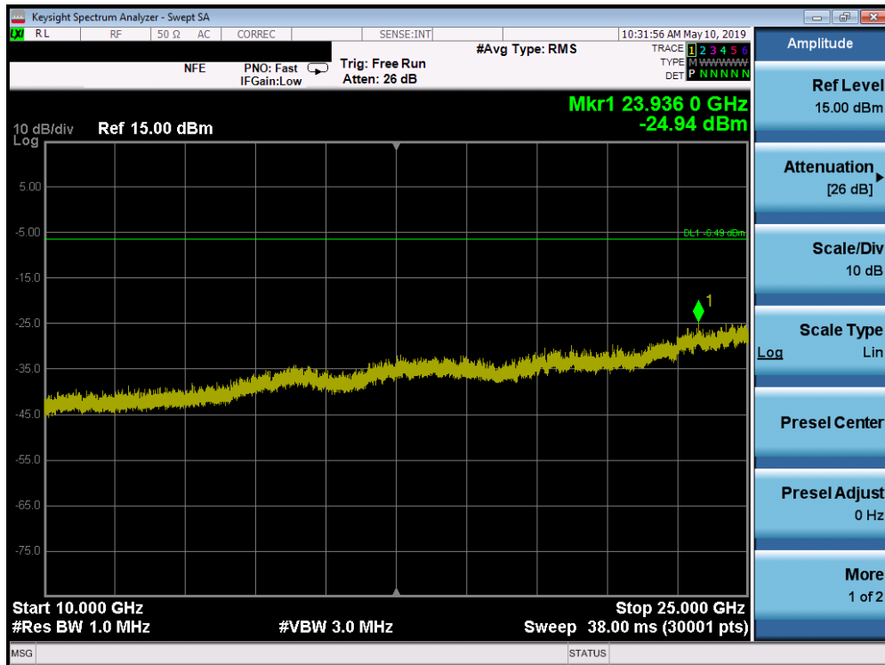
Plot 7-32. Conducted Spurious Plot (Bluetooth, 8DPSK, ePA - Ch. 39)
