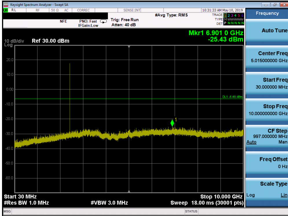
Plot 7-31. Conducted Spurious Plot (Bluetooth, 8DPSK, ePA - Ch. 39)
