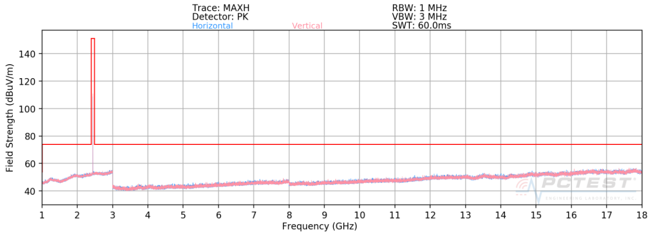
Plot 7-36. Radiated Spurious Plot above 1GHz (BT GFSK ePA – Ch. 39)
