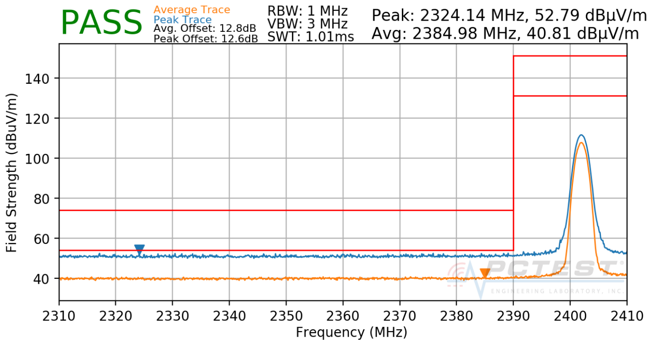
Plot 7-44. Radiated Restricted Lower Band Edge Measurement
