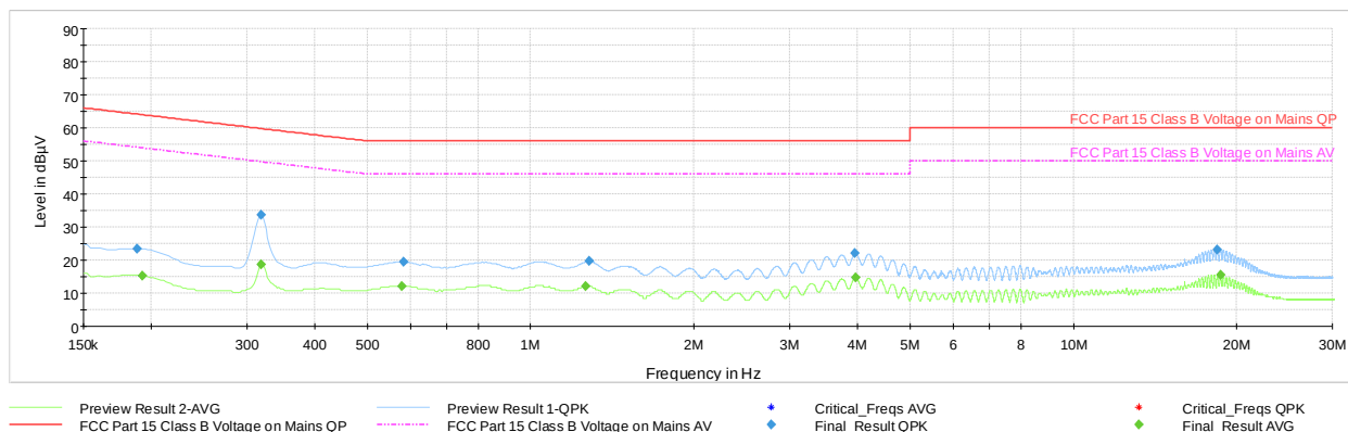
Plot 7-49. AC Line-Conducted Test Plot - Ch.39 (L1, with Laptop)
