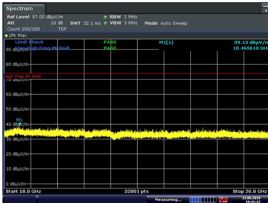
Plot 7-39. Radiated Spurious Plot above 18GHz (GFSK ePA – Ch. 39, Pol. V)
