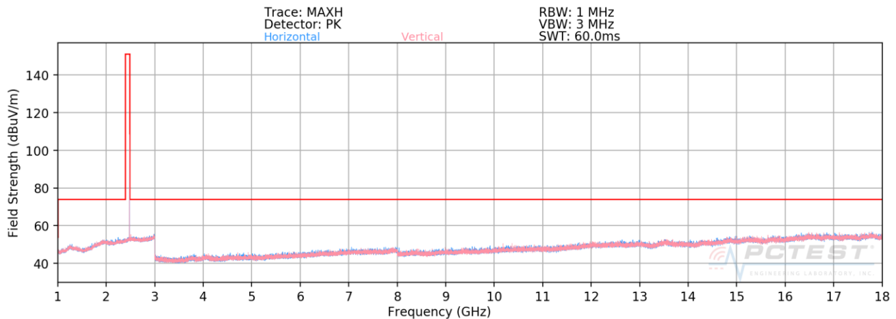
Plot 7-37. Radiated Spurious Plot above 1GHz (BT GFSK ePA – Ch. 78)
