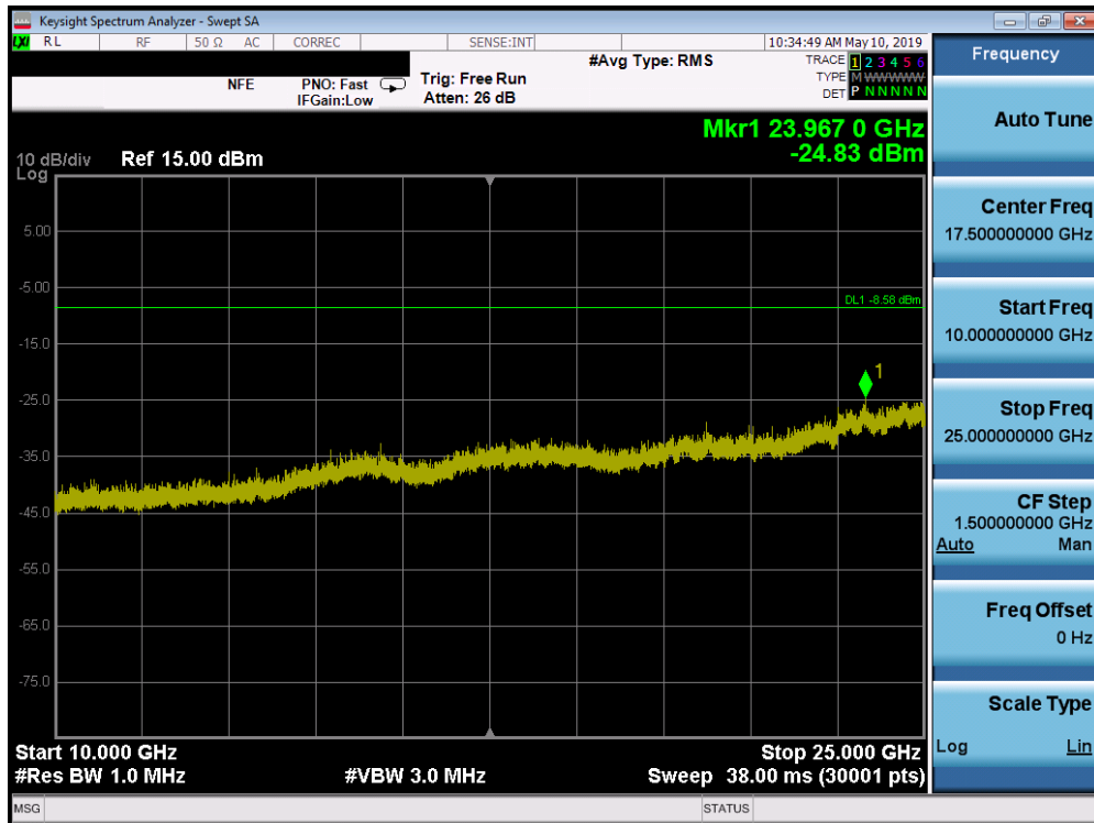
Plot 7-34. Conducted Spurious Plot (Bluetooth, 8DPSK, ePA – Ch. 78)
