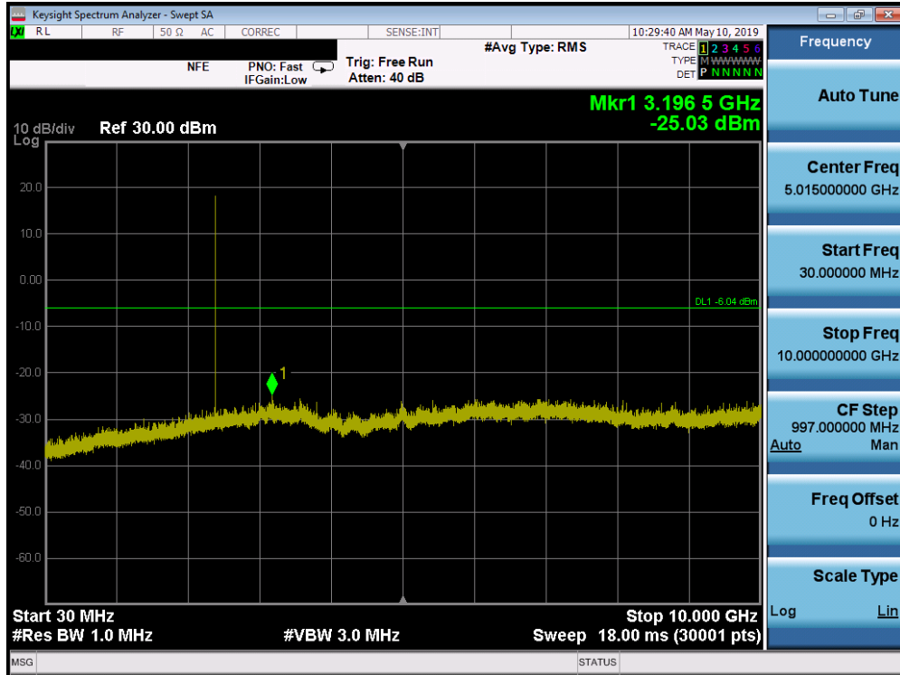
Plot 7-29. Conducted Spurious Plot (Bluetooth, 8DPSK, ePA – Ch. 0)
