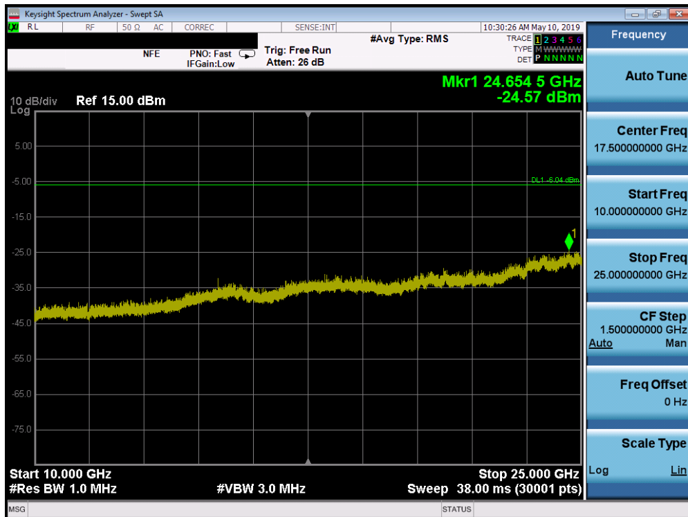
Plot 7-30. Conducted Spurious Plot (Bluetooth, 8DPSK, ePA – Ch. 0)
