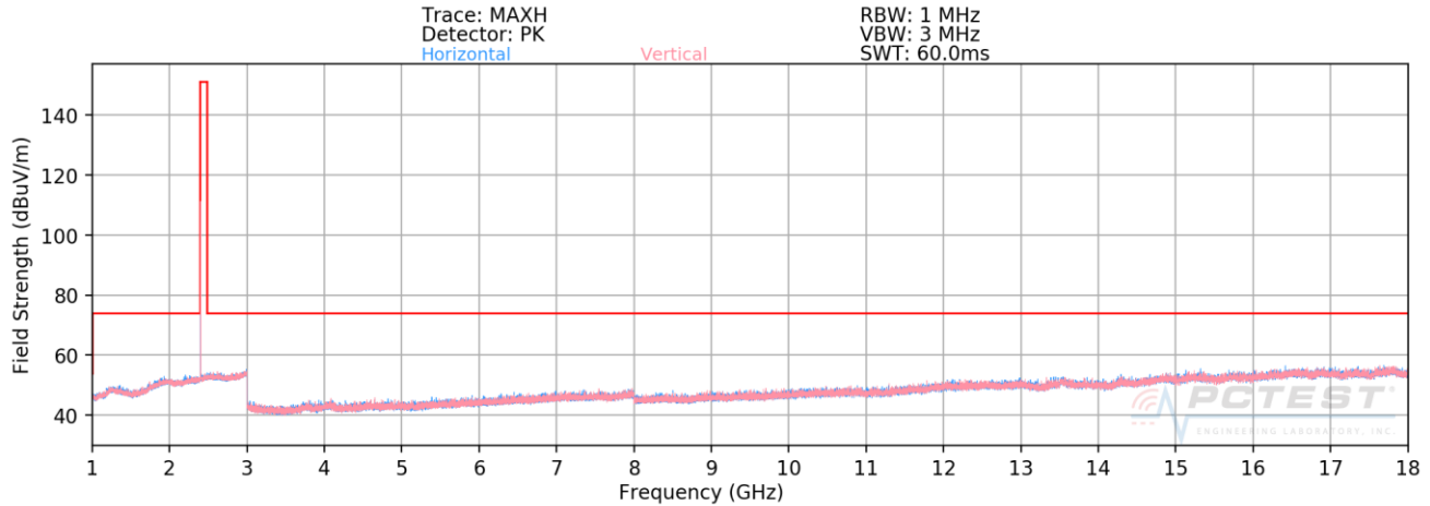
Plot 7-35. Radiated Spurious Plot above 1GHz (BT GFSK ePA – Ch. 0)
