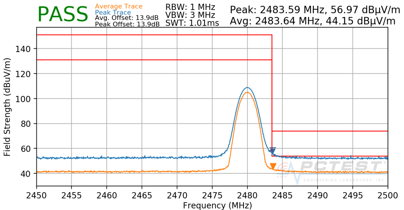
Plot 7-46. Radiated Restricted Upper Band Edge Measurement
