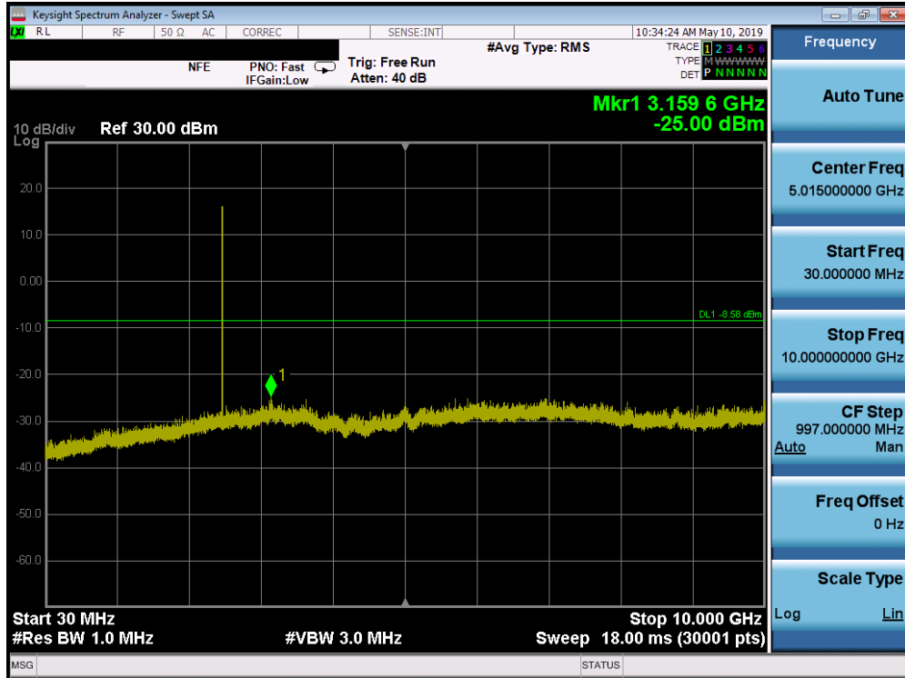
Plot 7-33. Conducted Spurious Plot (Bluetooth, 8DPSK, ePA – Ch. 78)
