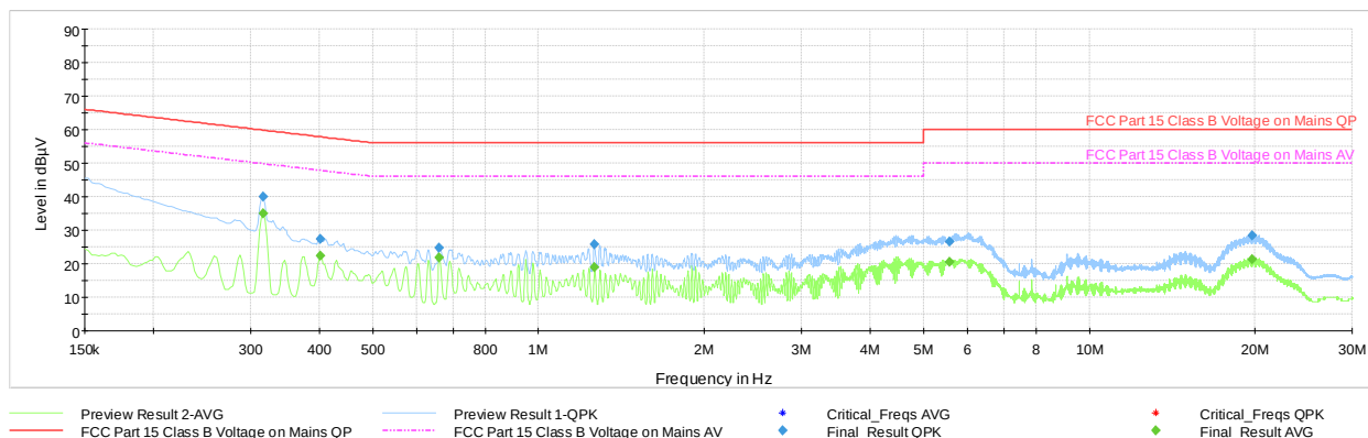
Plot 7-50. AC Line-Conducted Test Plot - Ch.39 (N, with Laptop)
