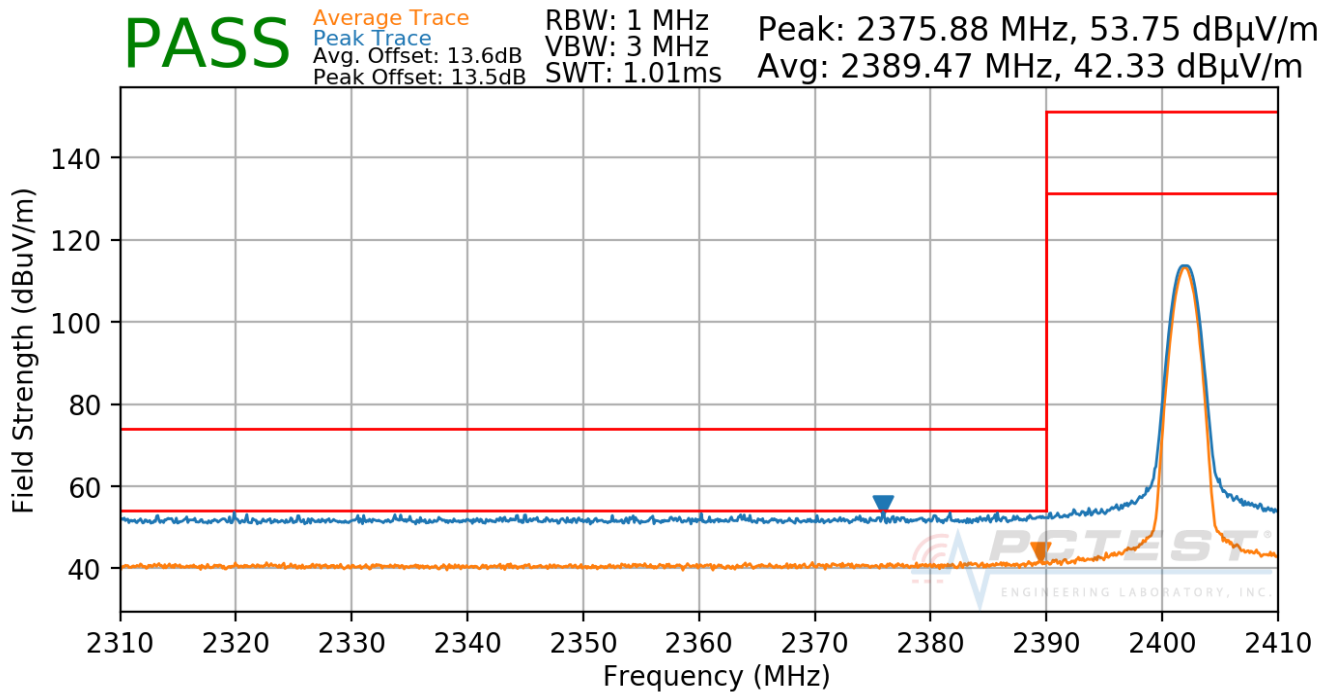
Plot 7-43. Radiated Restricted Lower Band Edge Measurement
