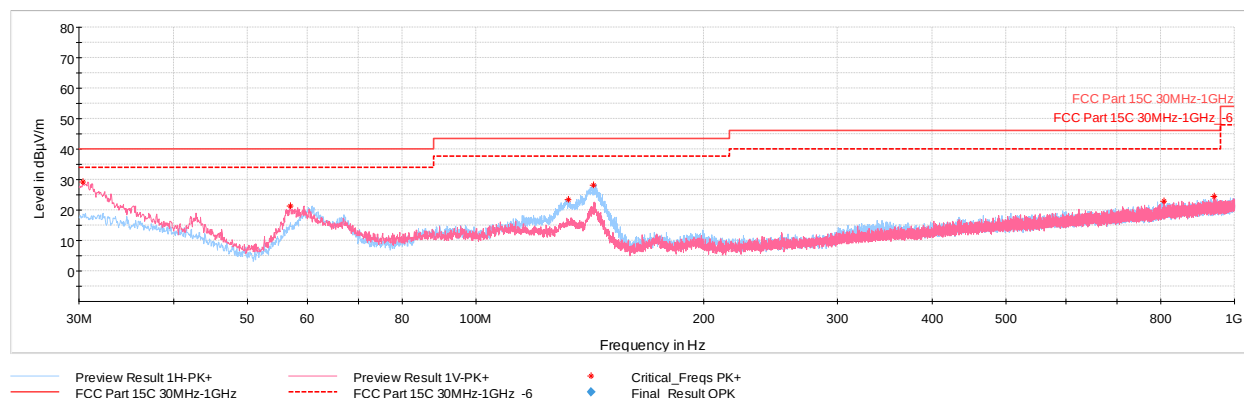
Plot 7-47. Radiated Spurious Plot below 1GHz GFSK ePA – Ch.39, with AC/DC Adapter
