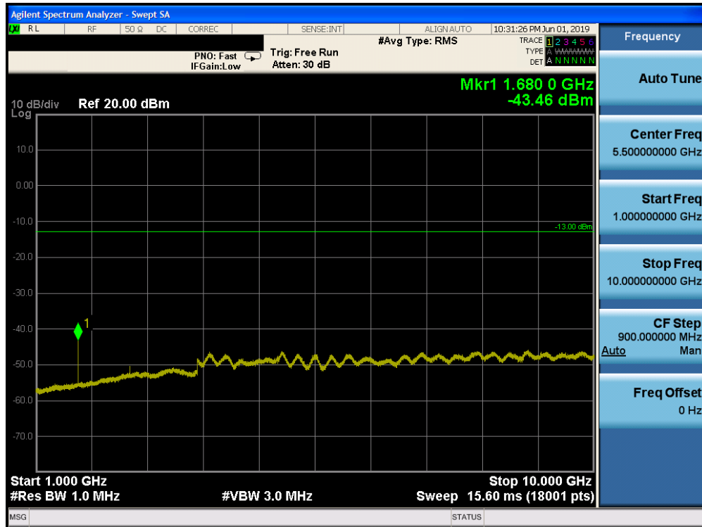
Plot 7-123. Conducted Spurious Plot (Band 5 - 10.0MHz QPSK - RB Size 1, RB Offset 0 - High Channel)
