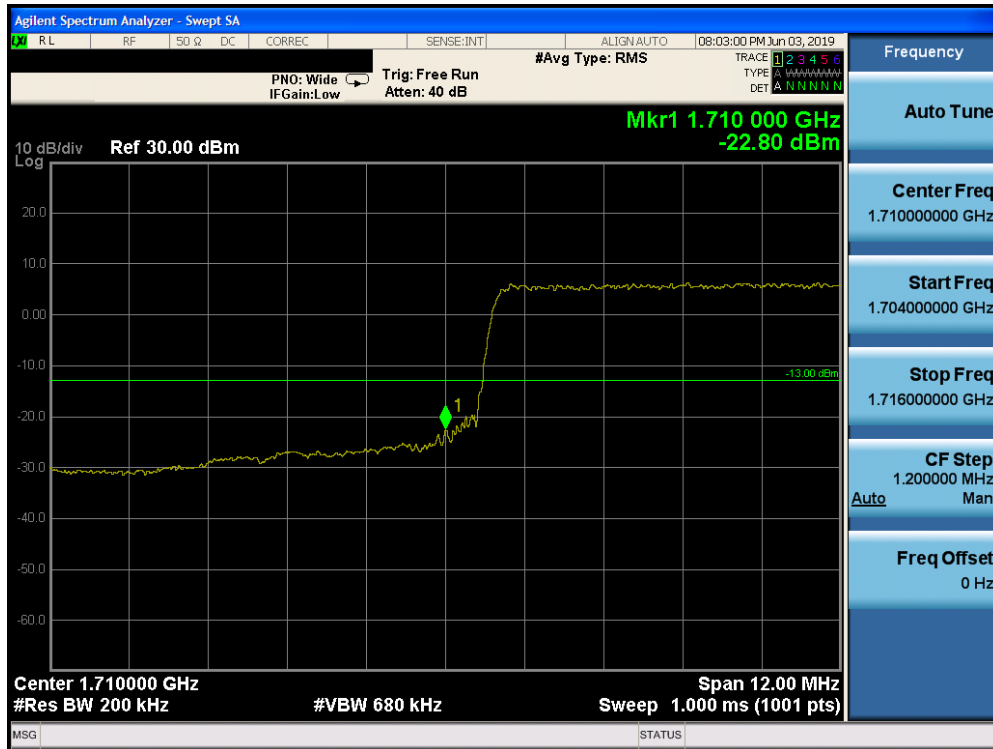
Plot 7-241. Lower Band Edge Plot (Band 4 - 15.0MHz QPSK - Full RB Configuration)
