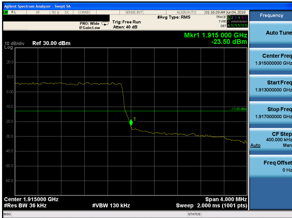
Plot 7-255. Upper Band Edge Plot (Band 25 - 3.0MHz QPSK - Full RB Configuration)
