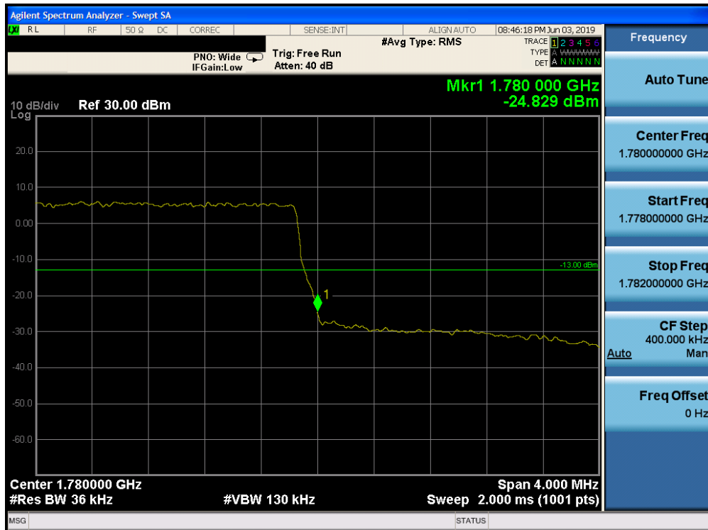
Plot 7-207. Upper Band Edge Plot (Band 66 - 3.0MHz QPSK - Full RB Configuration)
