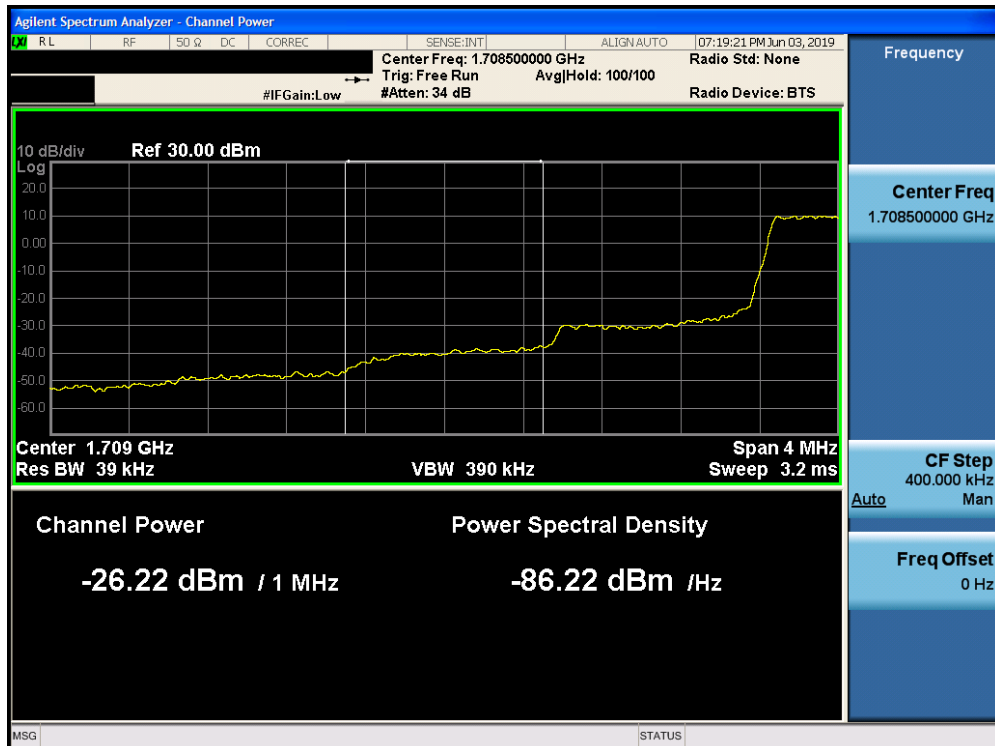
Plot 7-226. Lower Extended Band Edge Plot (Band 4 - 1.4MHz QPSK - Full RB Configuration)
