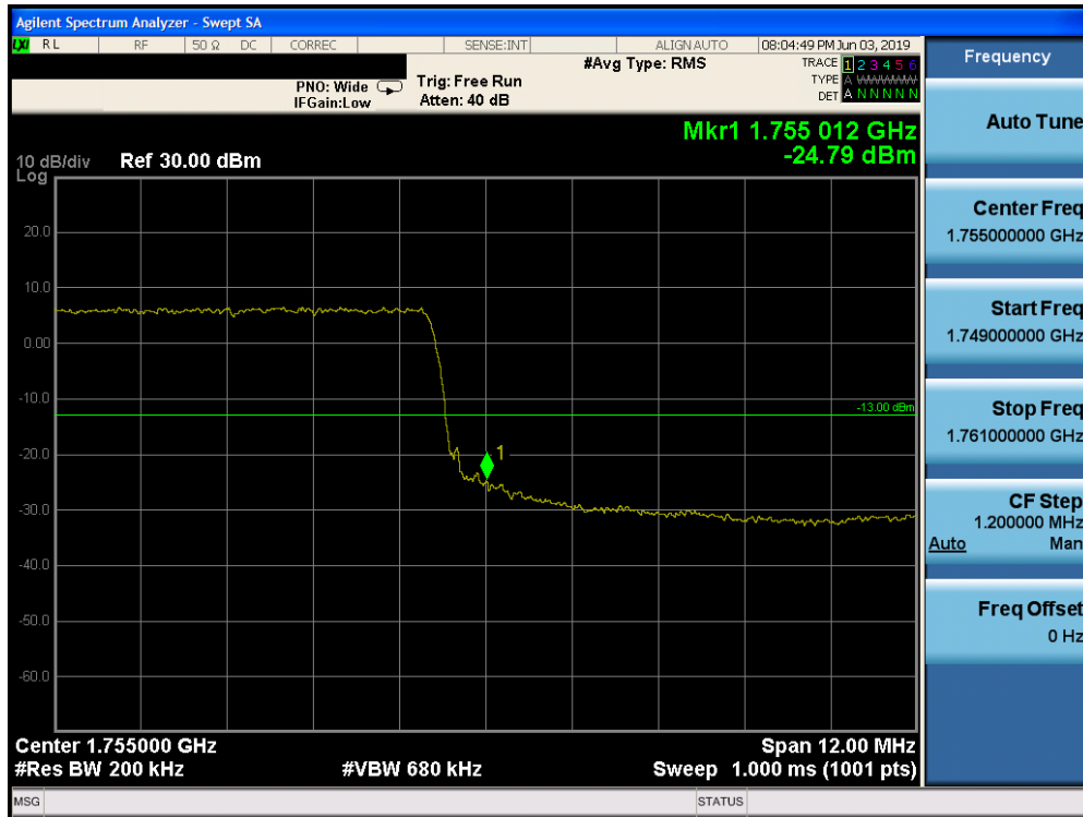
Plot 7-243. Upper Band Edge Plot (Band 4 - 15.0MHz QPSK - Full RB Configuration)
