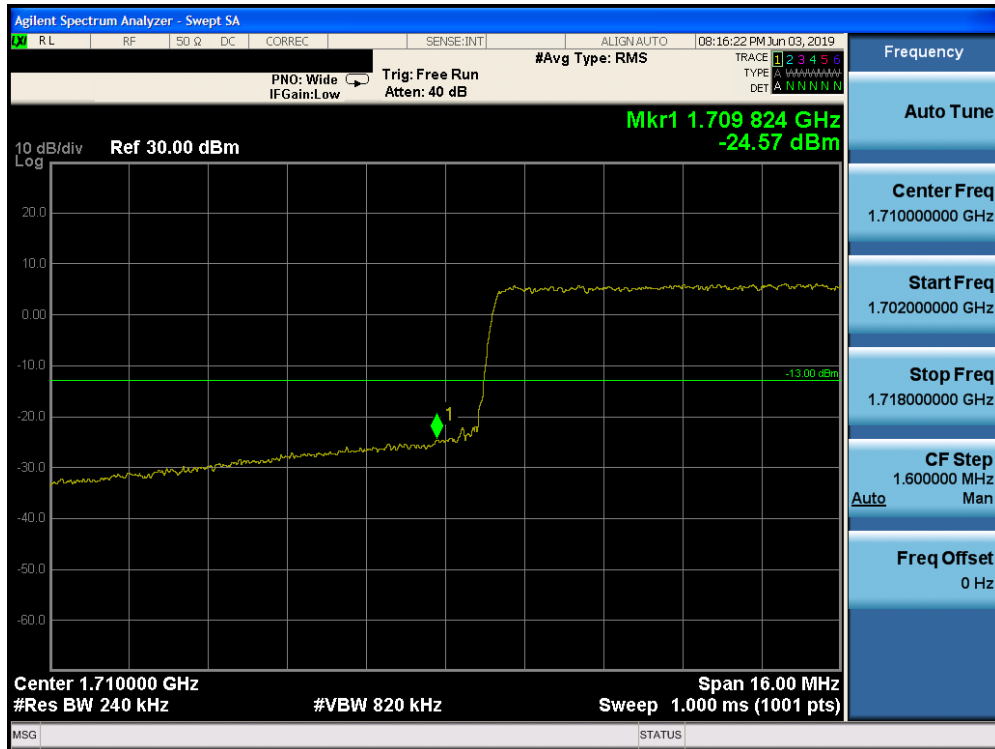
Plot 7-245. Lower Band Edge Plot (Band 4 - 20.0MHz QPSK - Full RB Configuration)
