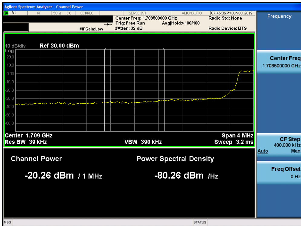
Plot 7-234. Lower Extended Band Edge Plot (Band 4 - 5.0MHz QPSK - Full RB Configuration)
