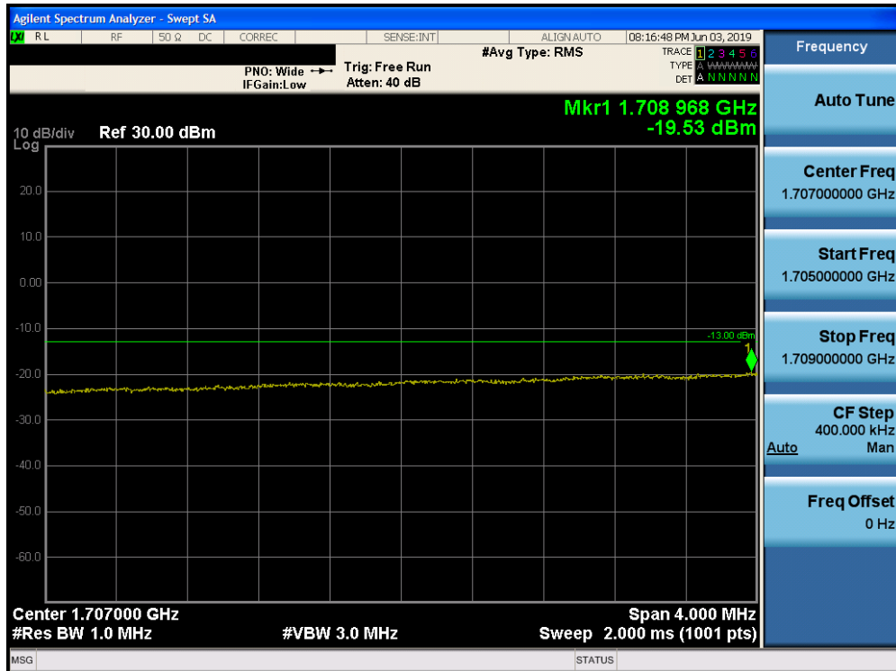
Plot 7-246. Lower Extended Band Edge Plot (Band 4 - 20.0MHz QPSK - Full RB Configuration)
