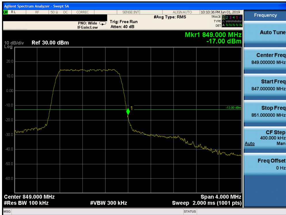
Plot 7-194. Upper Band Edge Plot (Band 5 - 1.4MHz QPSK - Full RB Configuration)
