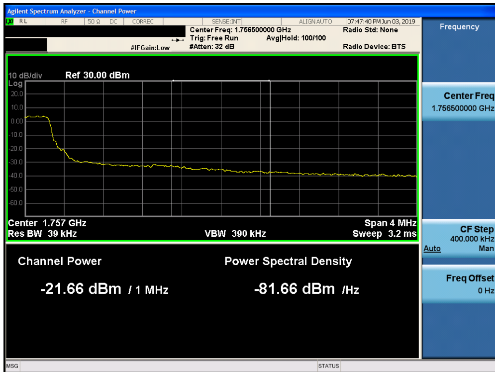
Plot 7-236. Upper Extended Band Edge Plot (Band 4 - 5.0MHz QPSK - Full RB Configuration)
