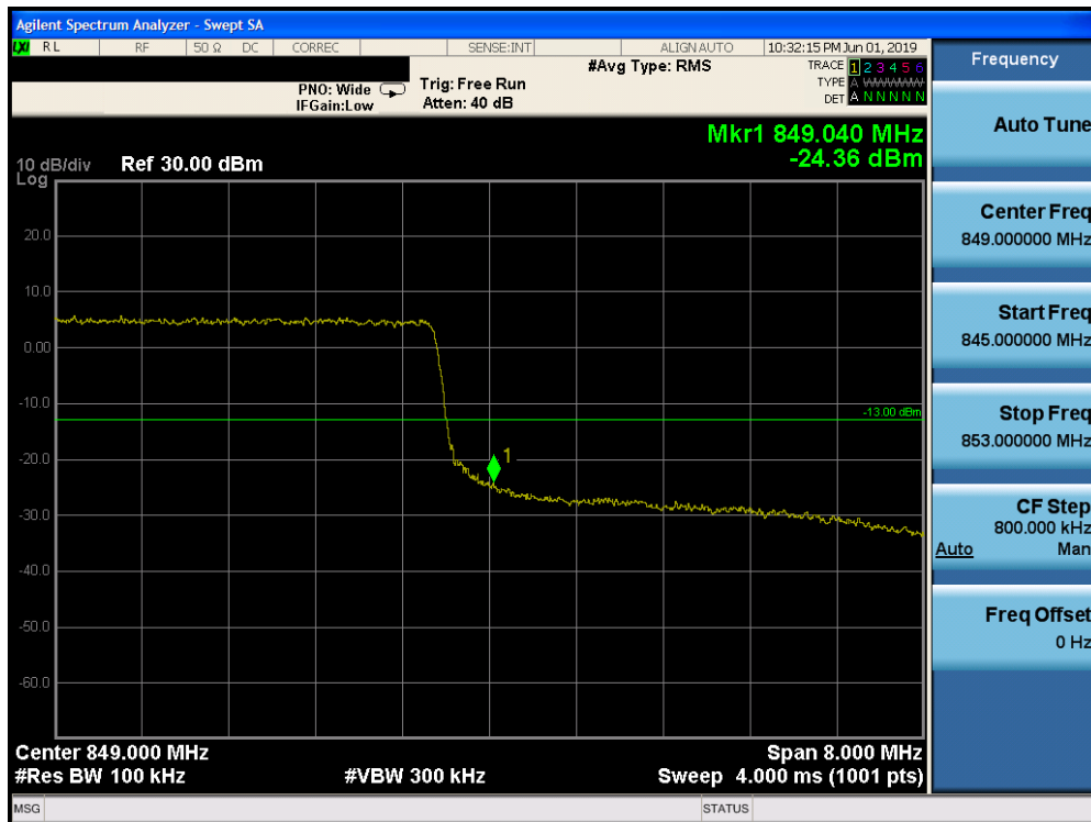
Plot 7-200. Upper Band Edge Plot (Band 5 - 10.0MHz QPSK - Full RB Configuration)
