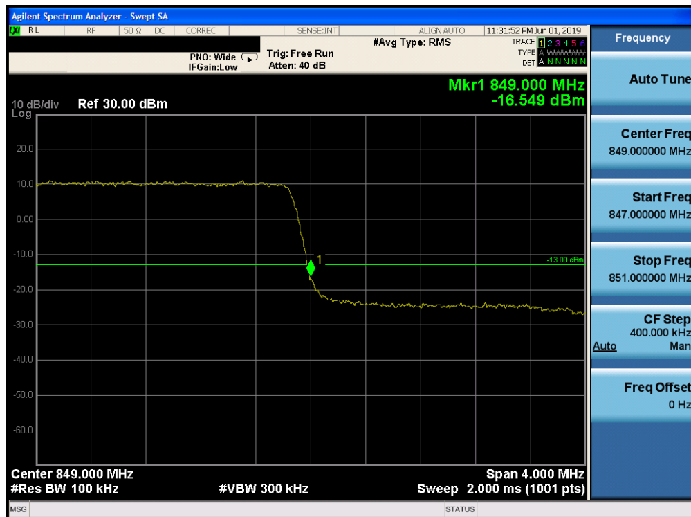
Plot 7-188. Upper Band Edge Plot (Band 26 - 3.0MHz QPSK - Full RB Configuration)
