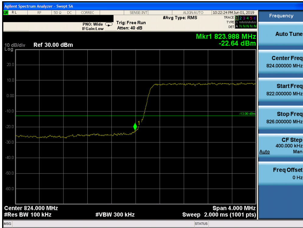
Plot 7-197. Lower Band Edge Plot (Band 5 - 5.0MHz QPSK - Full RB Configuration)
