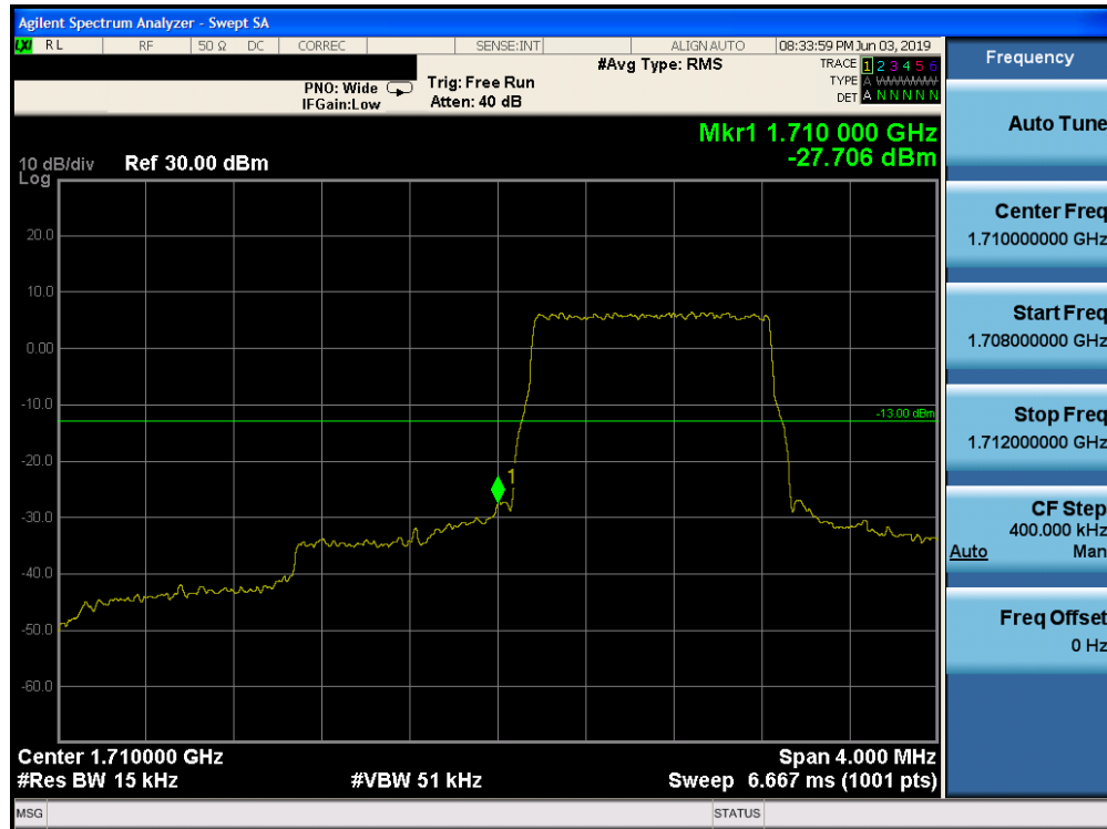
Plot 7-201. Lower Band Edge Plot (Band 66 - 1.4MHz QPSK - Full RB Configuration)
