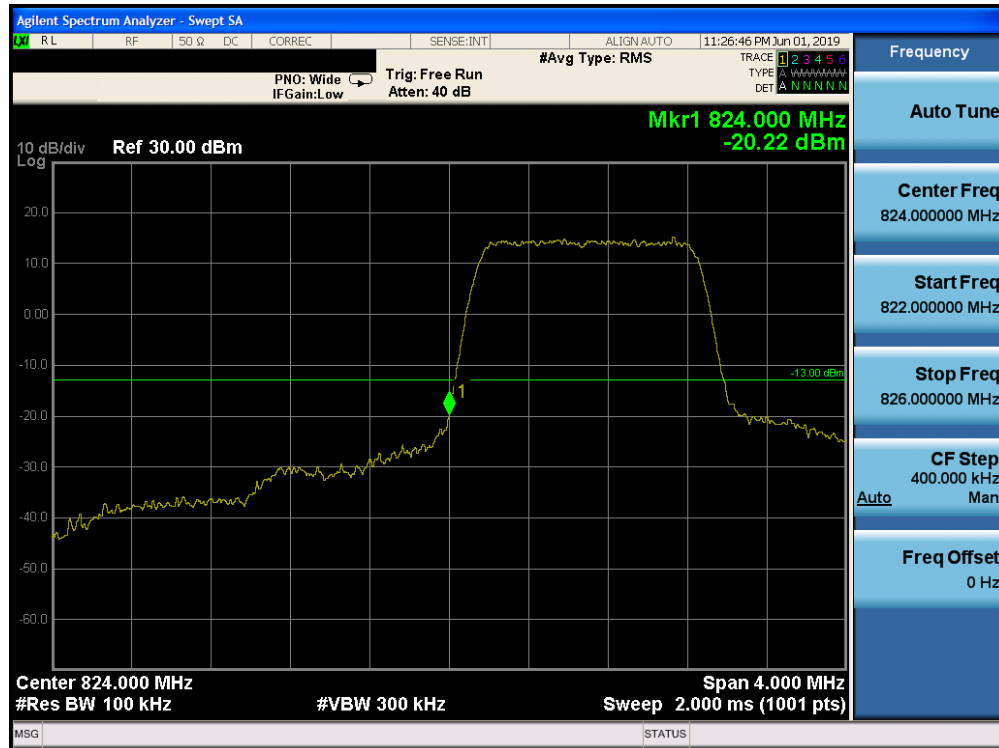
Plot 7-185. Lower Band Edge Plot (Band 26 - 1.4MHz QPSK - Full RB Configuration)
