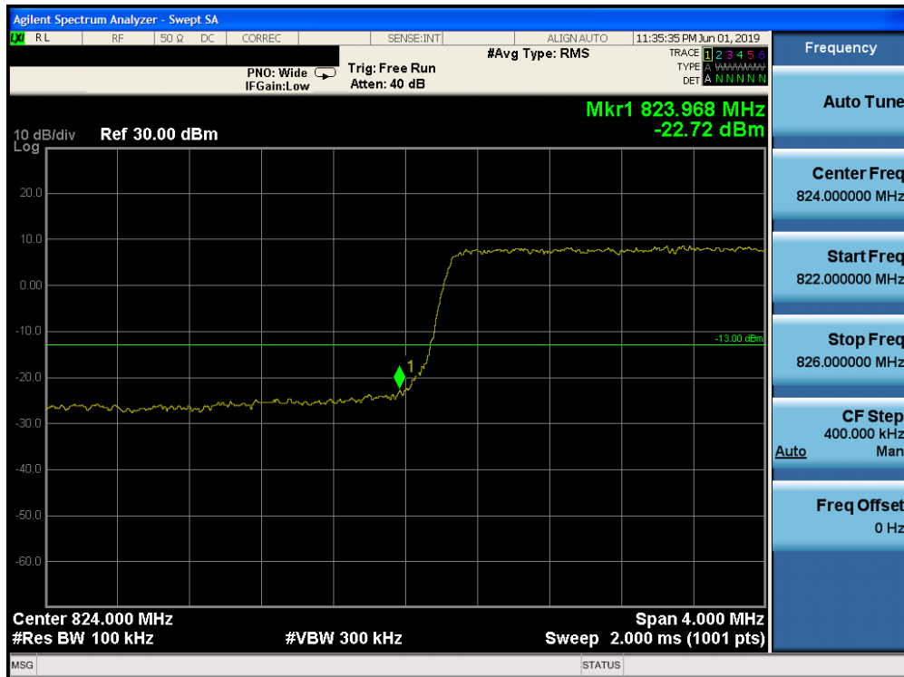
Plot 7-189. Lower Band Edge Plot (Band 26 - 5.0MHz QPSK - Full RB Configuration)
