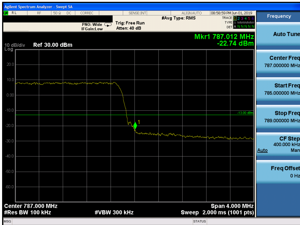
Plot 7-182. Upper Band Edge Plot (Band 13 - 5.0MHz QPSK - Full RB Configuration)
