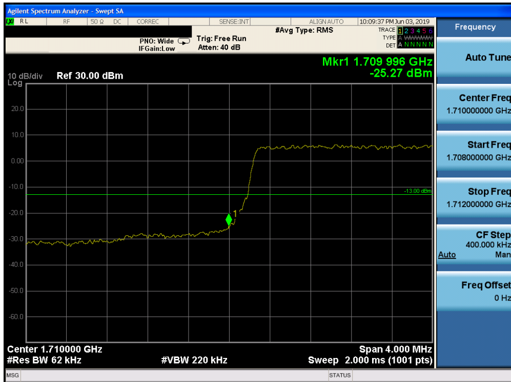
Plot 7-209. Lower Band Edge Plot (Band 66 - 5.0MHz QPSK - Full RB Configuration)
