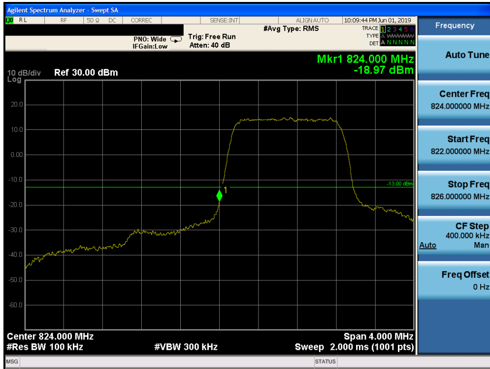
Plot 7-193. Lower Band Edge Plot (Band 5 - 1.4MHz QPSK - Full RB Configuration)
