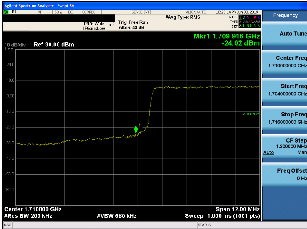
Plot 7-217. Lower Band Edge Plot (Band 66 - 15.0MHz QPSK - Full RB Configuration)
