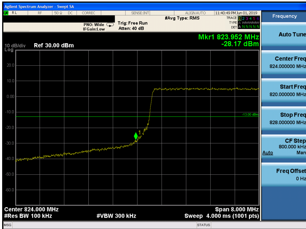
Plot 7-191. Lower Band Edge Plot (Band 26 - 10.0MHz QPSK - Full RB Configuration)
