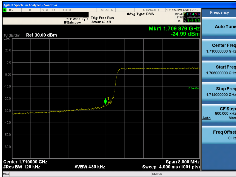
Plot 7-213. Lower Band Edge Plot (Band 66 - 10.0MHz QPSK - Full RB Configuration)
