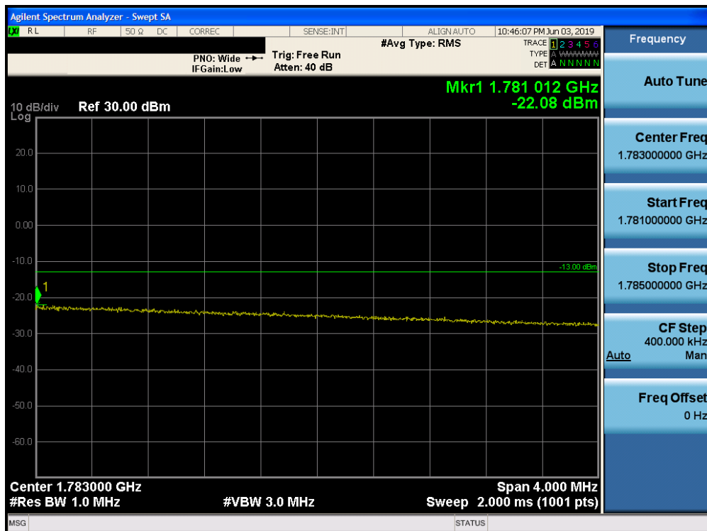
Plot 7-224. Upper Extended Band Edge Plot (Band 66 - 20.0MHz QPSK - Full RB Configuration)
