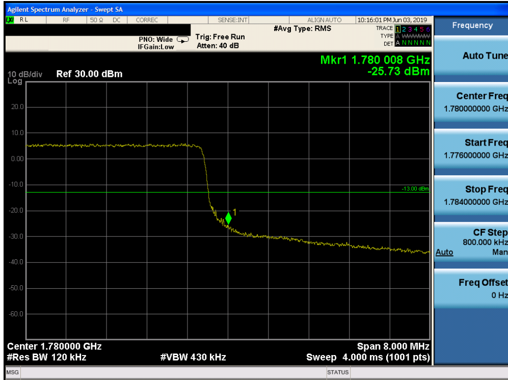
Plot 7-215. Upper Band Edge Plot (Band 66 - 10.0MHz QPSK - Full RB Configuration)
