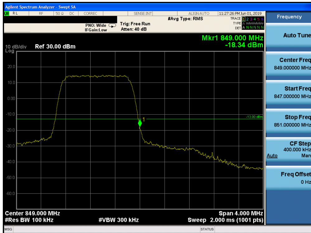
Plot 7-186. Upper Band Edge Plot (Band 26 - 1.4MHz QPSK - Full RB Configuration)
