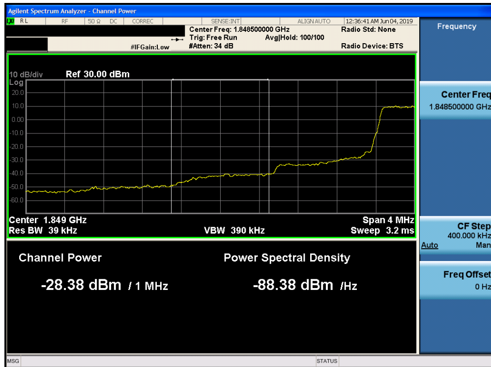
Plot 7-250. Lower Extended Band Edge Plot (Band 25 - 1.4MHz QPSK - Full RB Configuration)
