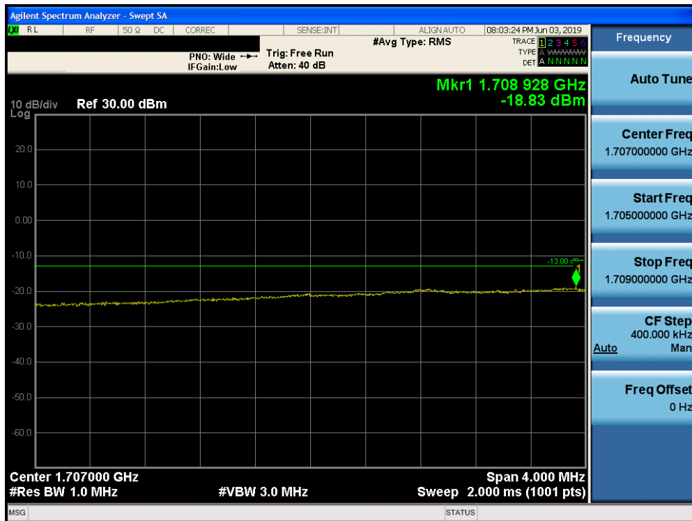
Plot 7-242. Lower Extended Band Edge Plot (Band 4 - 15.0MHz QPSK - Full RB Configuration)
