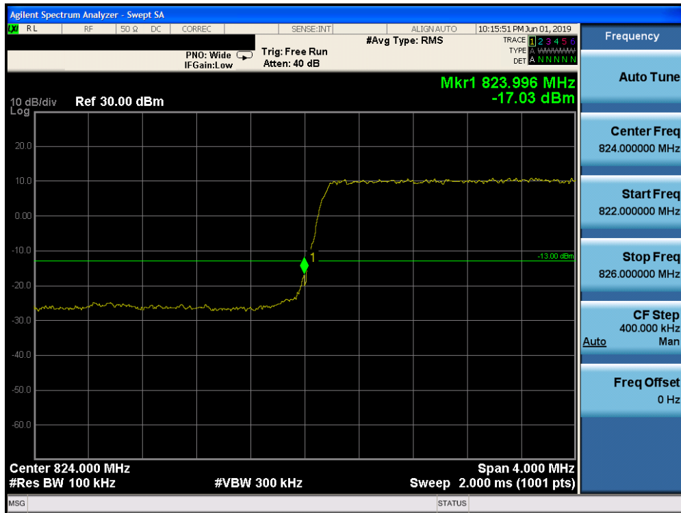
Plot 7-195. Lower Band Edge Plot (Band 5 - 3.0MHz QPSK - Full RB Configuration)
