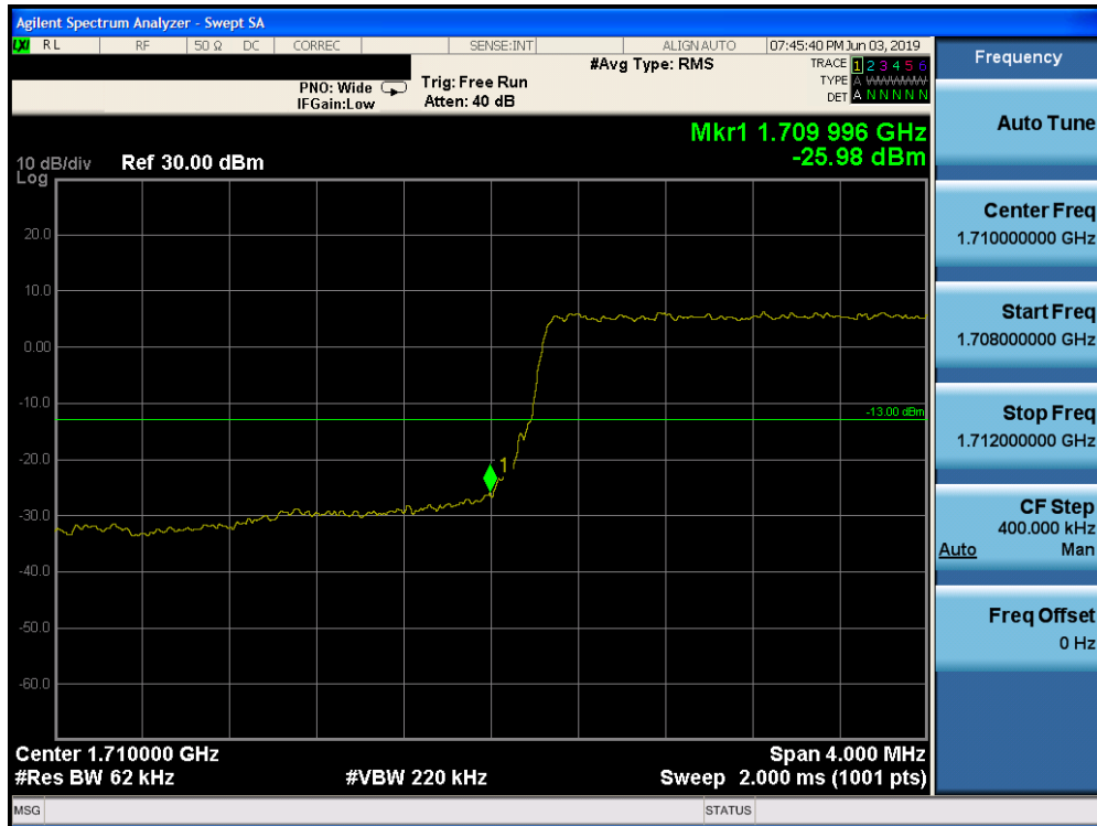
Plot 7-233. Lower Band Edge Plot (Band 4 - 5.0MHz QPSK - Full RB Configuration)
