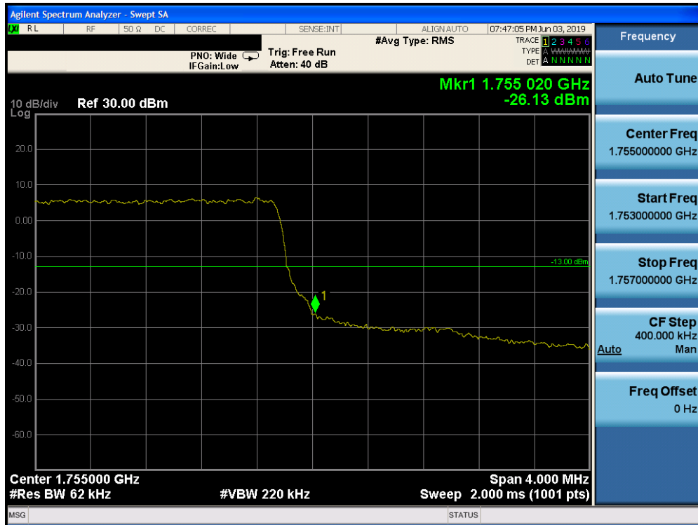
Plot 7-235. Upper Band Edge Plot (Band 4 - 5.0MHz QPSK - Full RB Configuration)
