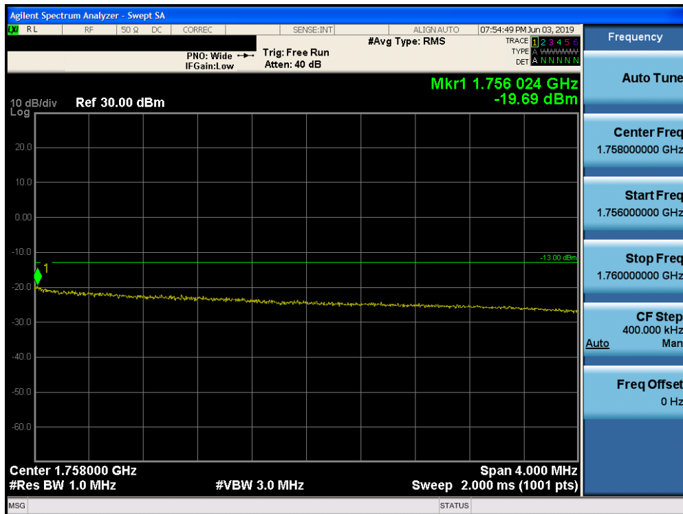
Plot 7-240. Upper Extended Band Edge Plot (Band 4 - 10.0MHz QPSK - Full RB Configuration)
