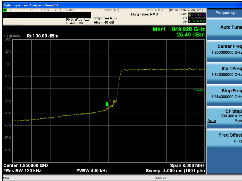
Plot 7-261. Lower Band Edge Plot (Band 25 - 10.0MHz QPSK - Full RB Configuration)
