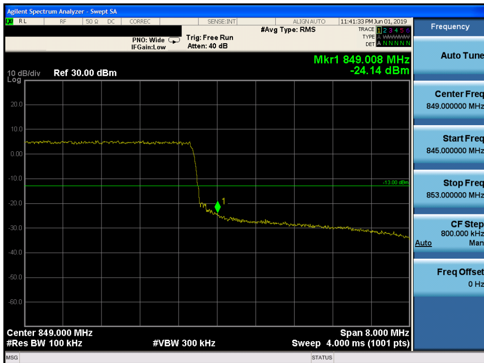
Plot 7-192. Upper Band Edge Plot (Band 26 - 10.0MHz QPSK - Full RB Configuration)
