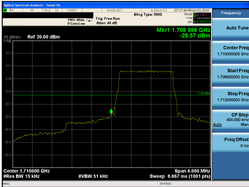
Plot 7-225. Lower Band Edge Plot (Band 4 - 1.4MHz QPSK - Full RB Configuration)
