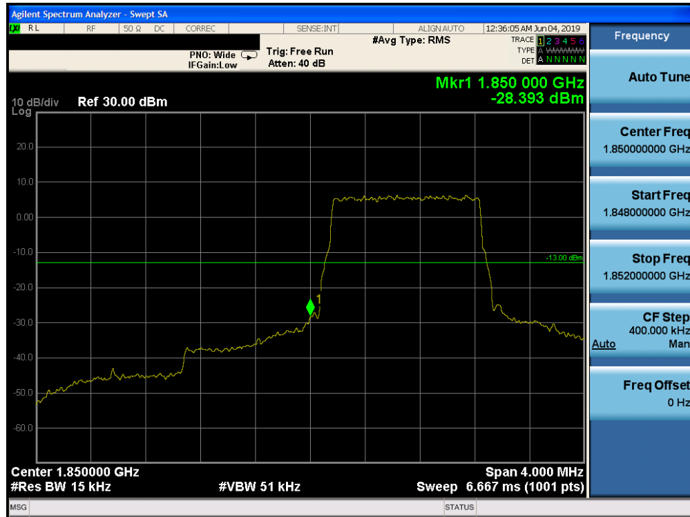
Plot 7-249. Lower Band Edge Plot (Band 25 - 1.4MHz QPSK - Full RB Configuration)
