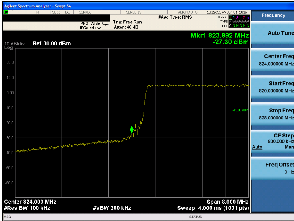
Plot 7-199. Lower Band Edge Plot (Band 5 - 10.0MHz QPSK - Full RB Configuration)
