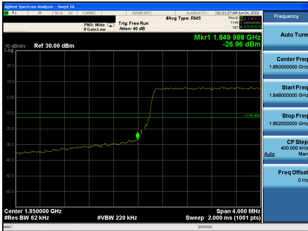
Plot 7-257. Lower Band Edge Plot (Band 25 - 5.0MHz QPSK - Full RB Configuration)
