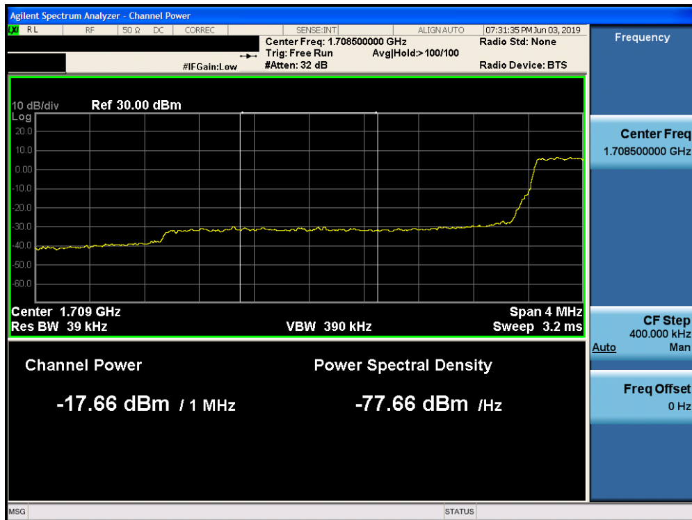
Plot 7-230. Lower Extended Band Edge Plot (Band 4 - 3.0MHz QPSK - Full RB Configuration)
