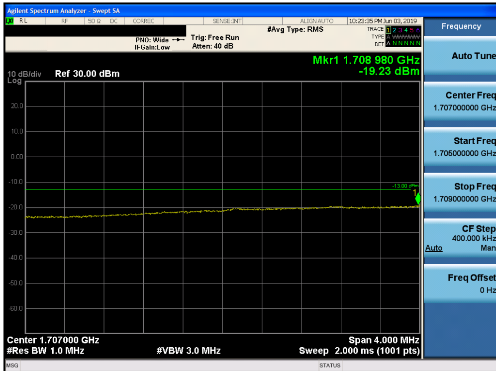
Plot 7-218. Lower Extended Band Edge Plot (Band 66 - 15.0MHz QPSK - Full RB Configuration)
