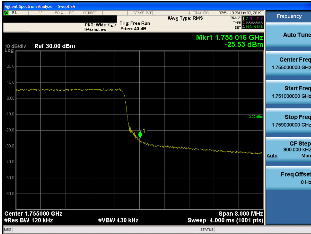
Plot 7-239. Upper Band Edge Plot (Band 4 - 10.0MHz QPSK - Full RB Configuration)
