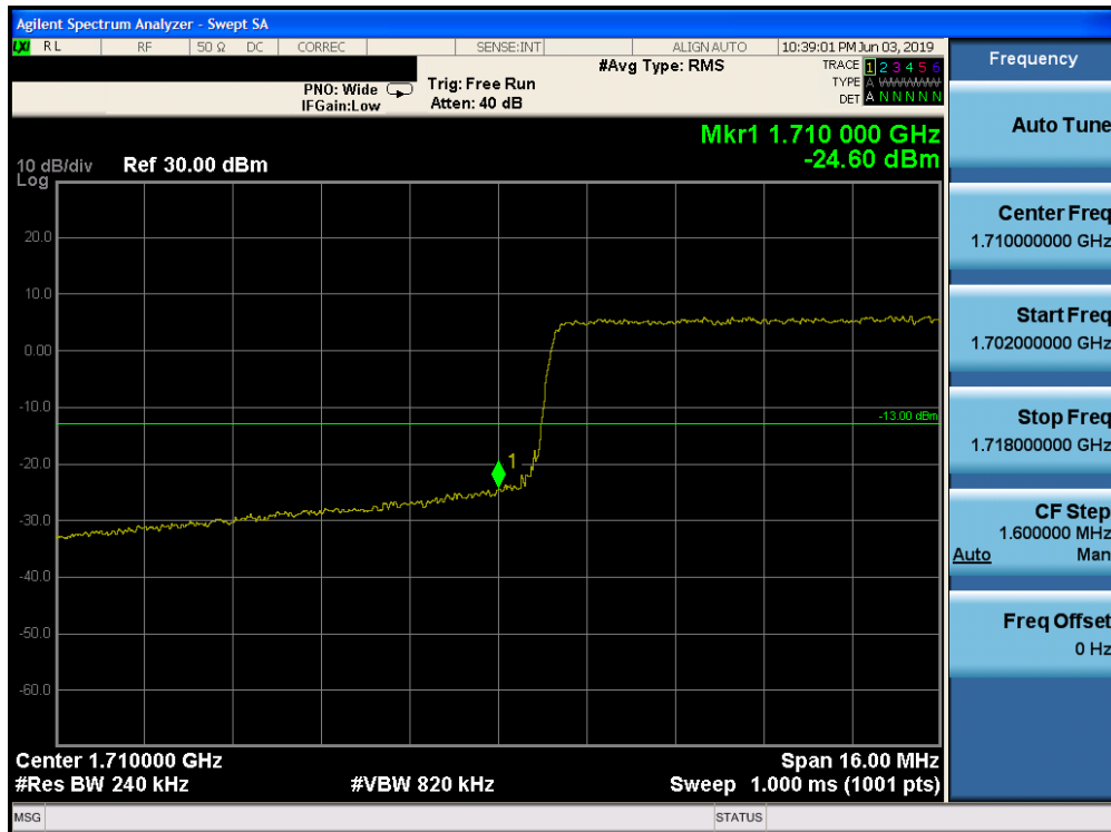
Plot 7-221. Lower Band Edge Plot (Band 66 - 20.0MHz QPSK - Full RB Configuration)
