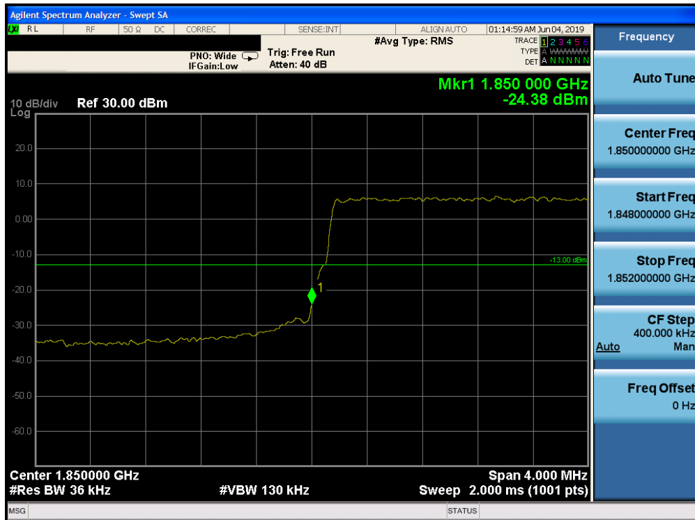
Plot 7-253. Lower Band Edge Plot (Band 25 - 3.0MHz QPSK - Full RB Configuration)
