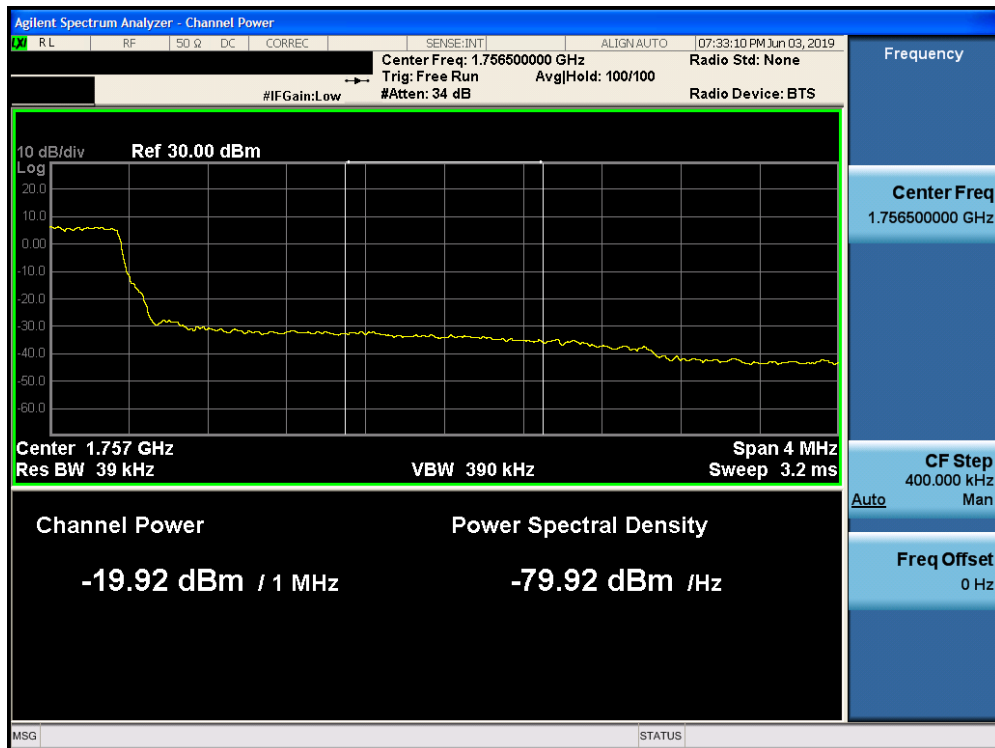
Plot 7-232. Upper Extended Band Edge Plot (Band 4 - 3.0MHz QPSK - Full RB Configuration)
