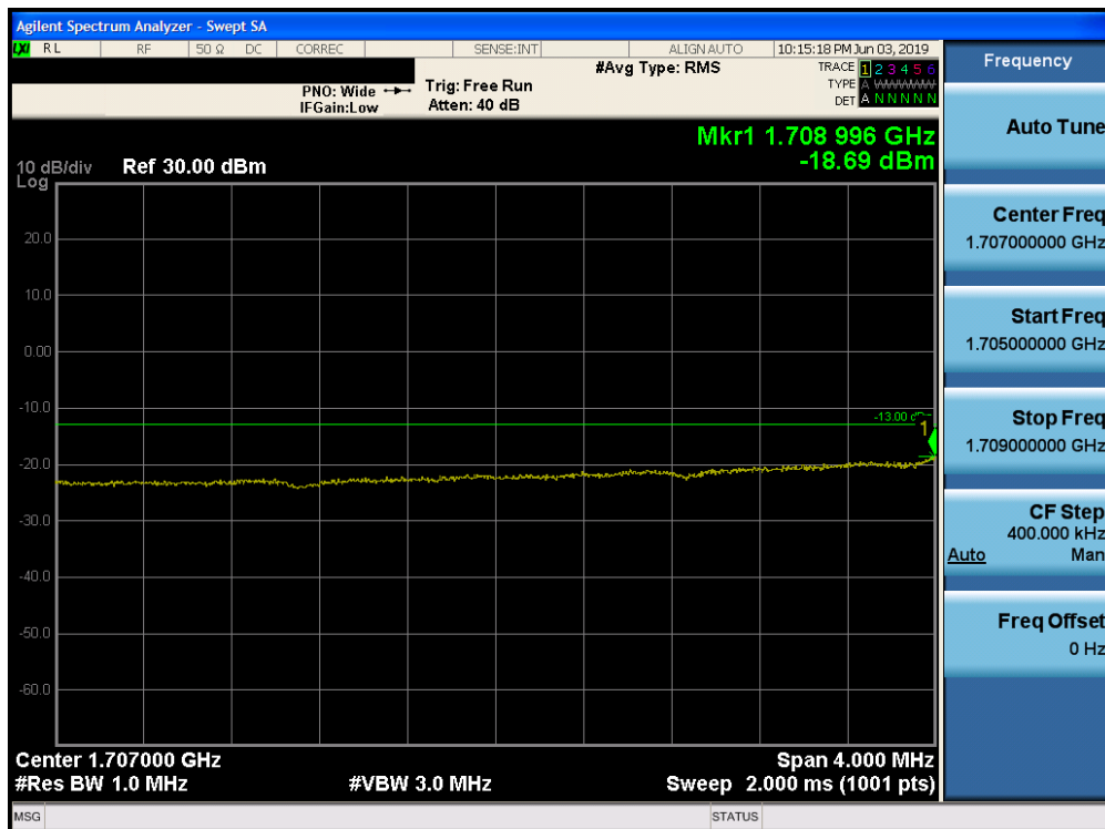
Plot 7-214. Lower Extended Band Edge Plot (Band 66 - 10.0MHz QPSK - Full RB Configuration)
