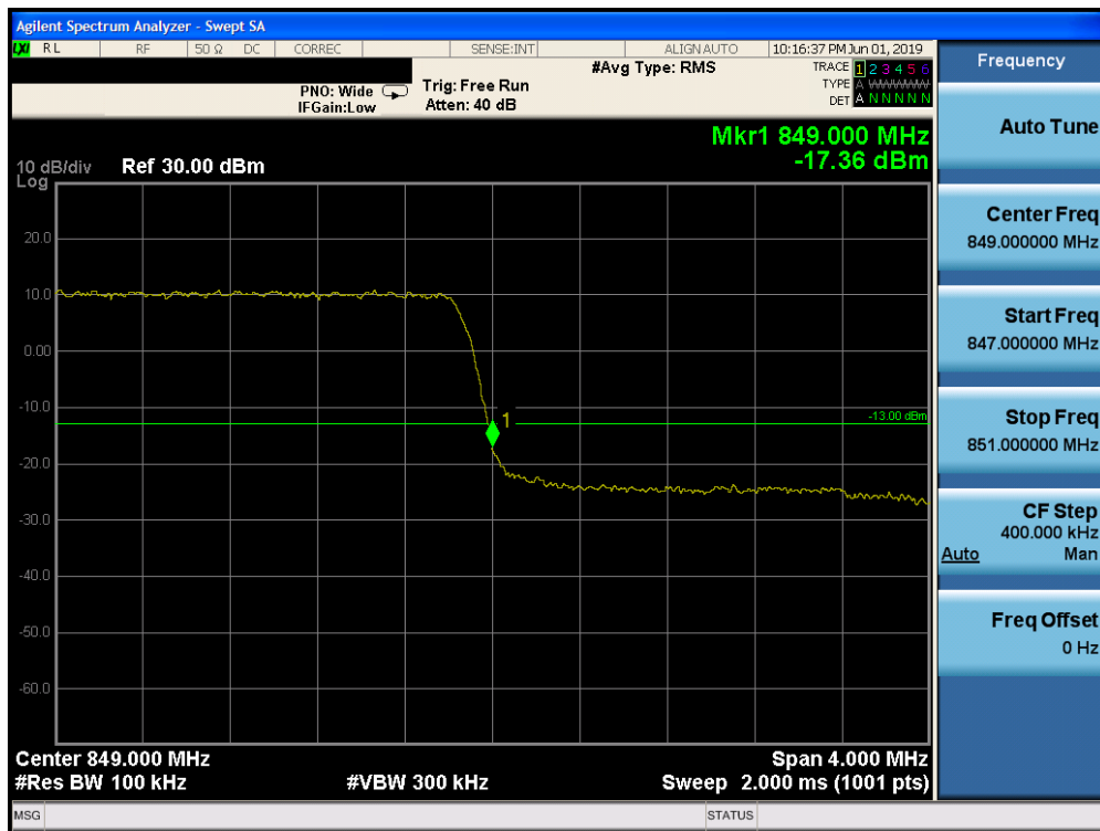
Plot 7-196. Upper Band Edge Plot (Band 5 - 3.0MHz QPSK - Full RB Configuration)
