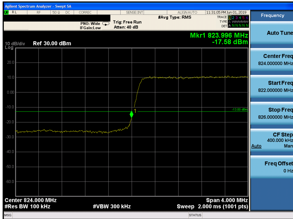
Plot 7-187. Lower Band Edge Plot (Band 26 - 3.0MHz QPSK - Full RB Configuration)
