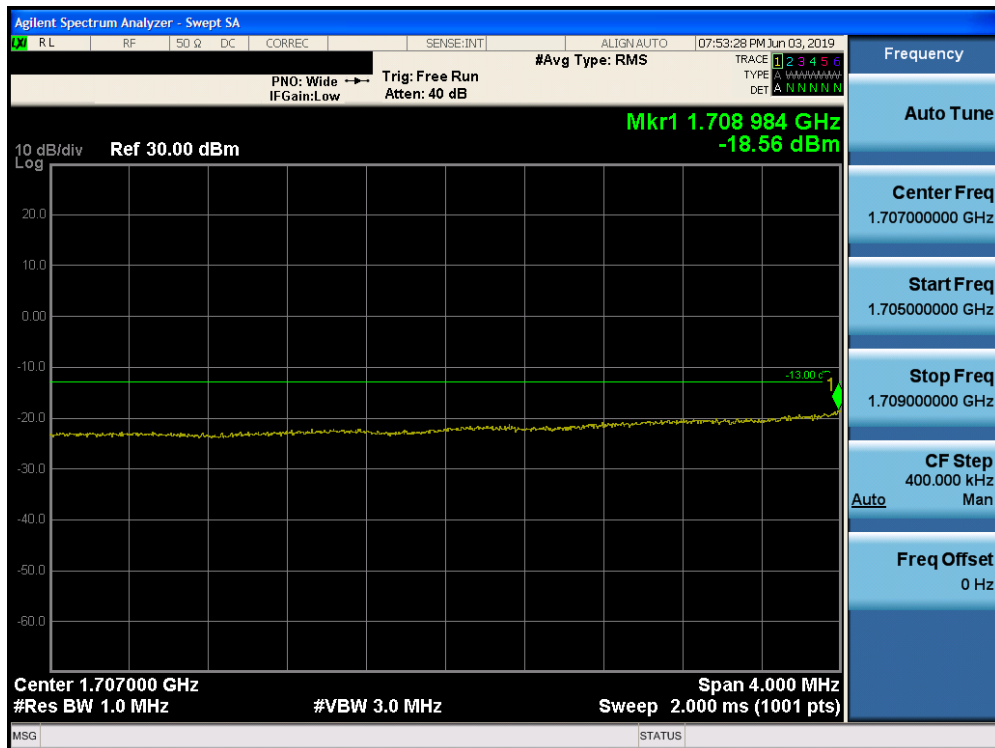
Plot 7-238. Lower Extended Band Edge Plot (Band 4 - 10.0MHz QPSK - Full RB Configuration)
