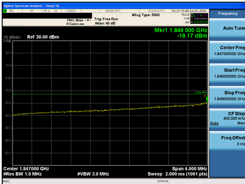
Plot 7-262. Lower Extended Band Edge Plot (Band 25 - 10.0MHz QPSK - Full RB Configuration)
