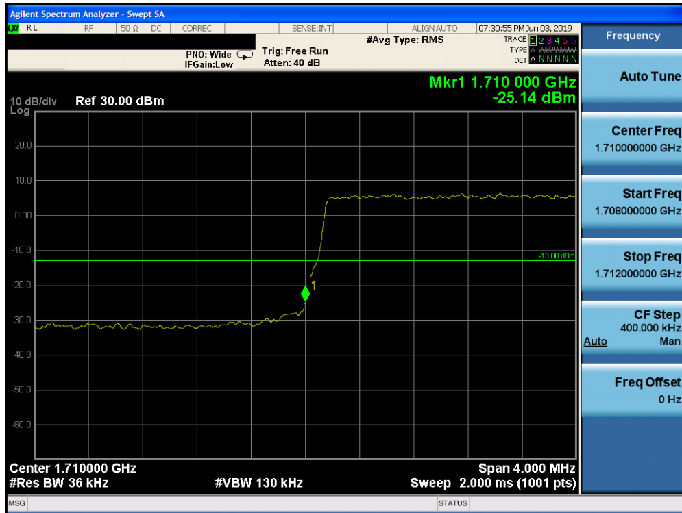
Plot 7-229. Lower Band Edge Plot (Band 4 - 3.0MHz QPSK - Full RB Configuration)
