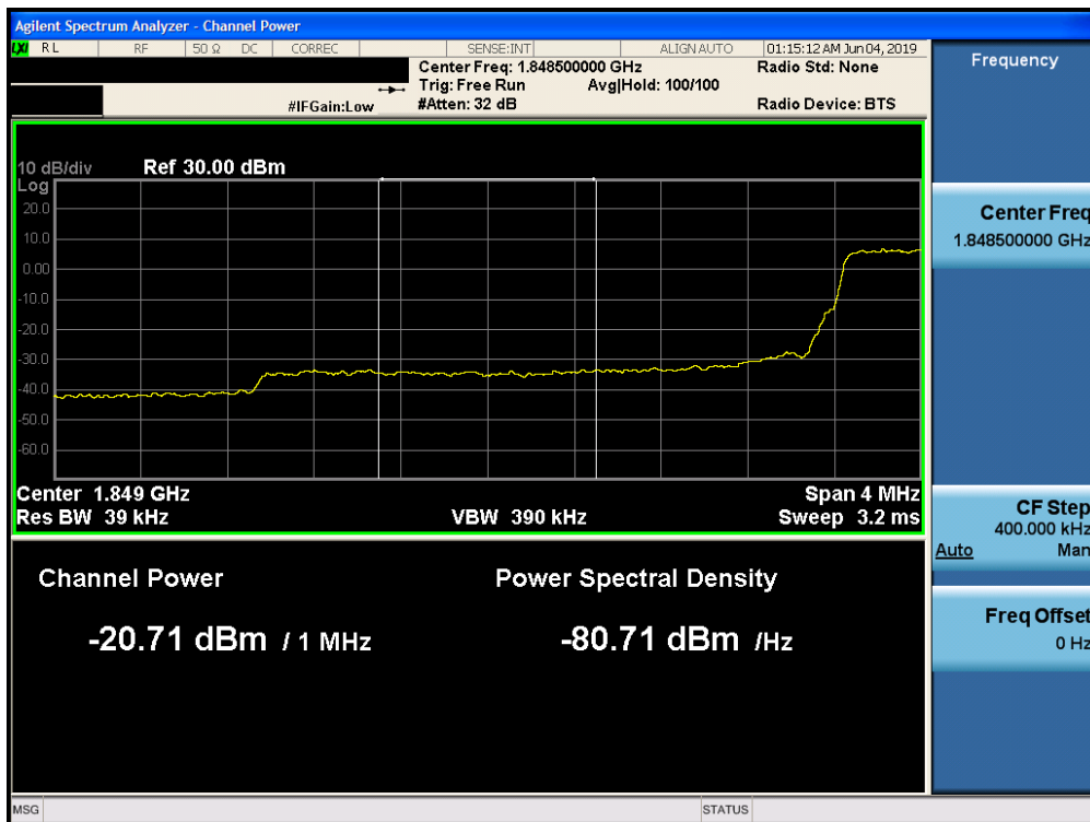
Plot 7-254. Lower Extended Band Edge Plot (Band 25 - 3.0MHz QPSK - Full RB Configuration)
