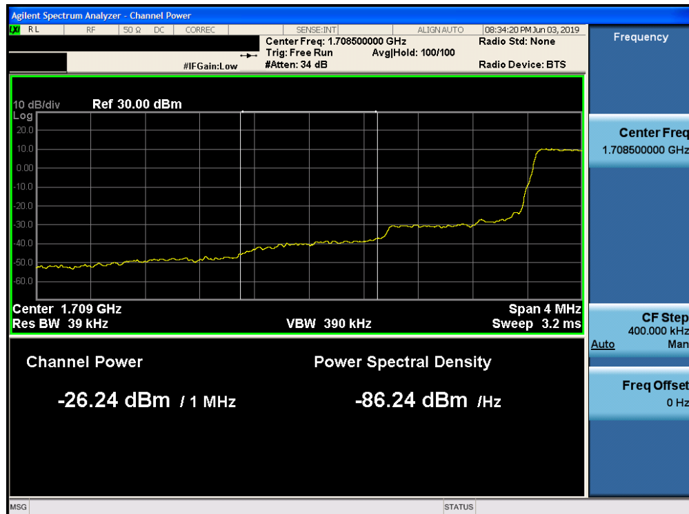
Plot 7-202. Lower Extended Band Edge Plot (Band 66 - 1.4MHz QPSK - Full RB Configuration)
