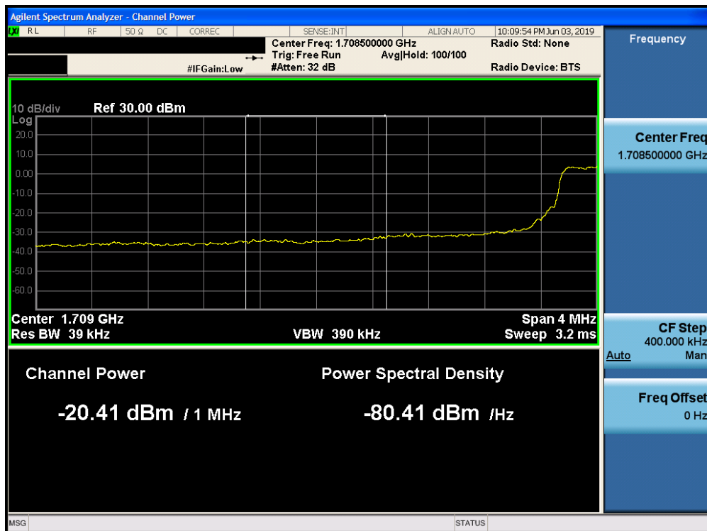
Plot 7-210. Lower Extended Band Edge Plot (Band 66 - 5.0MHz QPSK - Full RB Configuration)
