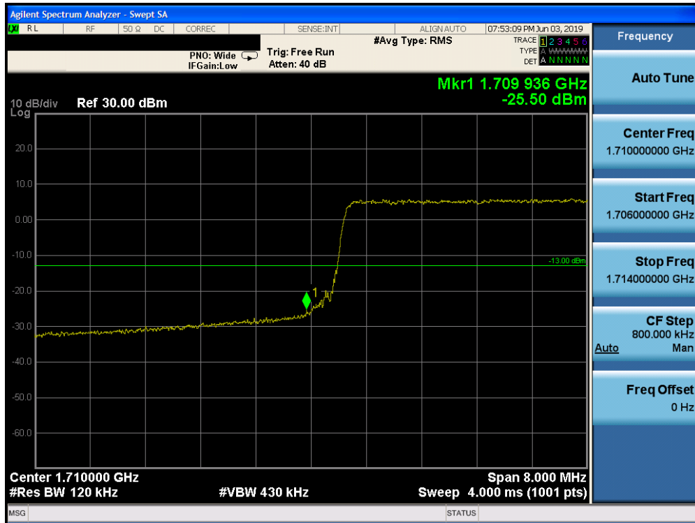
Plot 7-237. Lower Band Edge Plot (Band 4 - 10.0MHz QPSK - Full RB Configuration)
