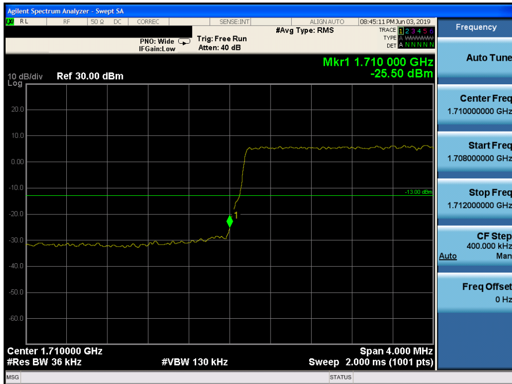
Plot 7-205. Lower Band Edge Plot (Band 66 - 3.0MHz QPSK - Full RB Configuration)
