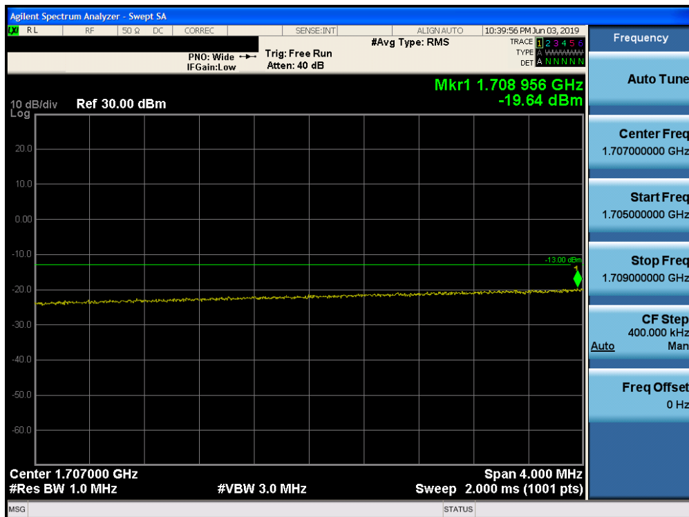
Plot 7-222. Lower Extended Band Edge Plot (Band 66 - 20.0MHz QPSK - Full RB Configuration)
