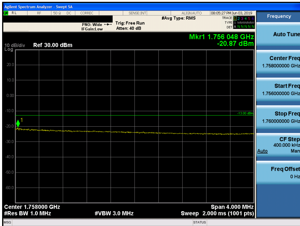
Plot 7-244. Upper Extended Band Edge Plot (Band 4 - 15.0MHz QPSK - Full RB Configuration)
