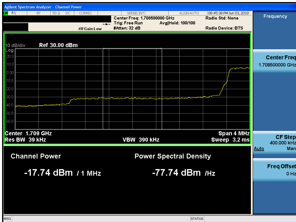
Plot 7-206. Lower Extended Band Edge Plot (Band 66 - 3.0MHz QPSK - Full RB Configuration)
