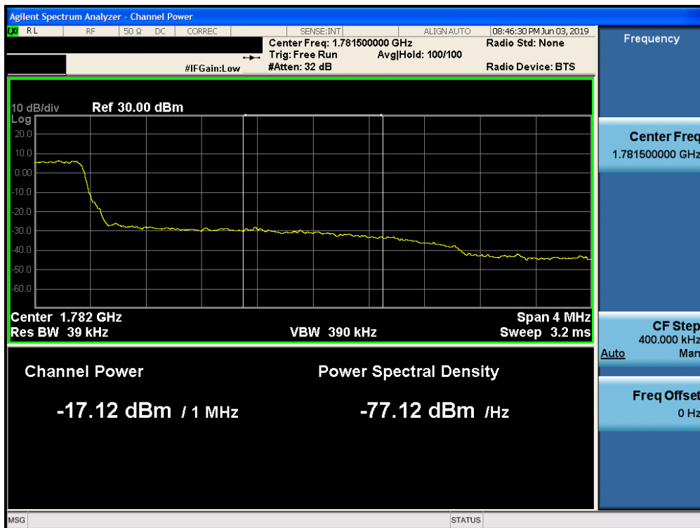
Plot 7-208. Upper Extended Band Edge Plot (Band 66 - 3.0MHz QPSK - Full RB Configuration)
