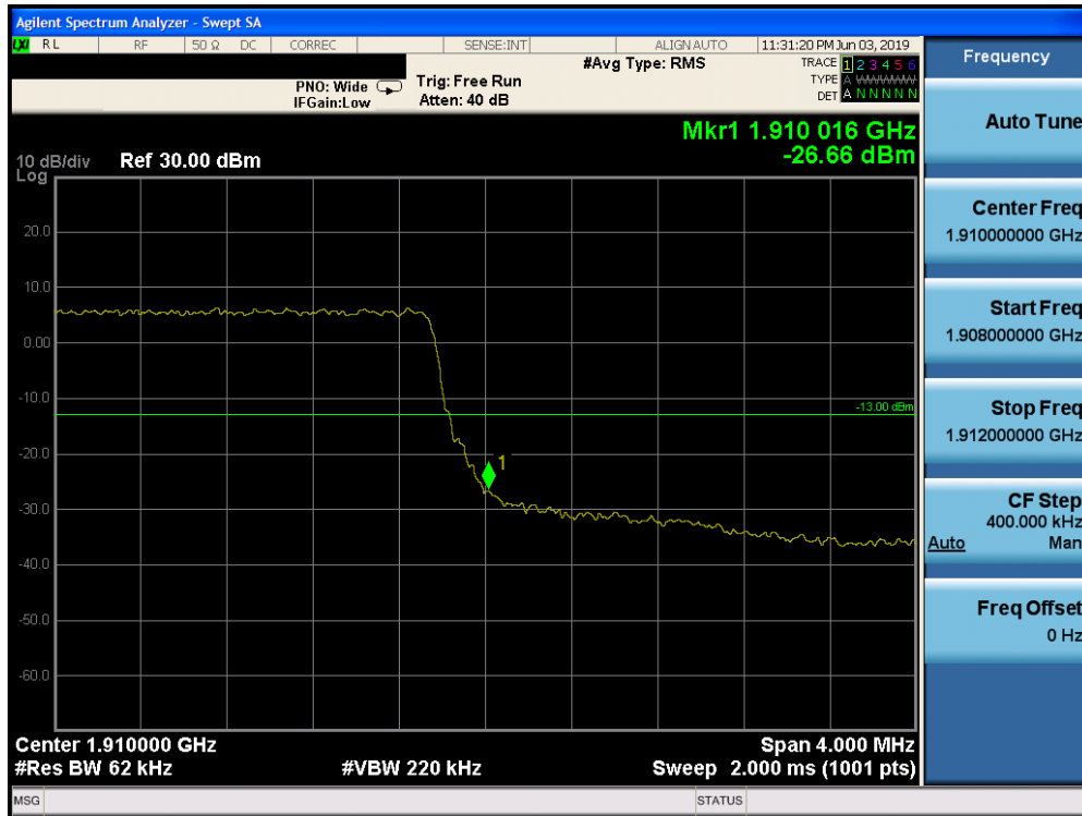
Plot 7-283. Upper Band Edge Plot (Band 2 - 5.0MHz QPSK - Full RB Configuration)
