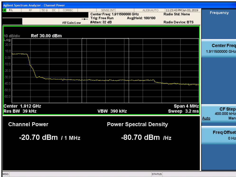
Plot 7-280. Upper Extended Band Edge Plot (Band 2 - 3.0MHz QPSK - Full RB Configuration)
