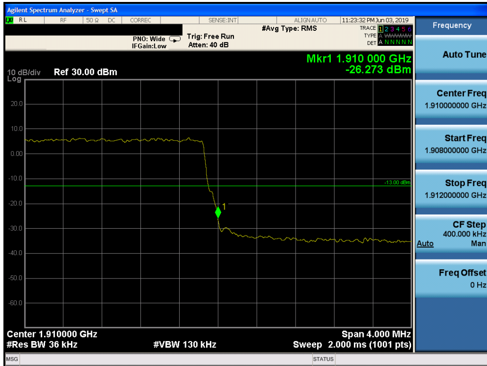
Plot 7-279. Upper Band Edge Plot (Band 2 - 3.0MHz QPSK - Full RB Configuration)
