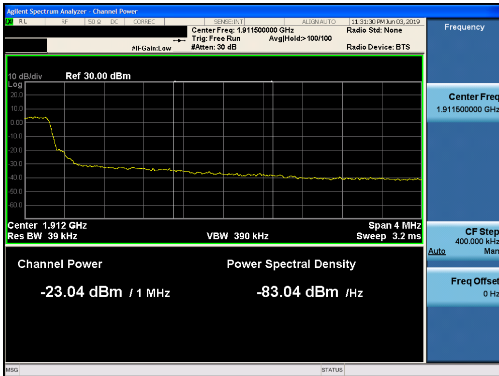
Plot 7-284. Upper Extended Band Edge Plot (Band 2 - 5.0MHz QPSK - Full RB Configuration)
