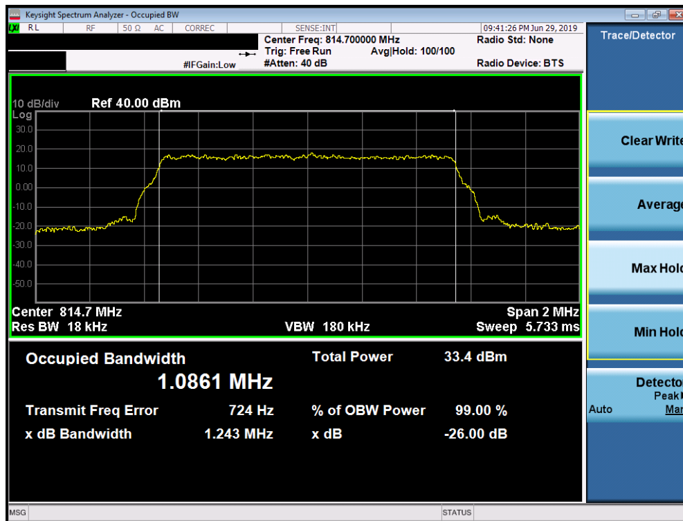
Plot 7-2. Occupied Bandwidth Plot (LTE Band 26, 1.4MHz 16-QAM – RB Size 6– Low Channel)
