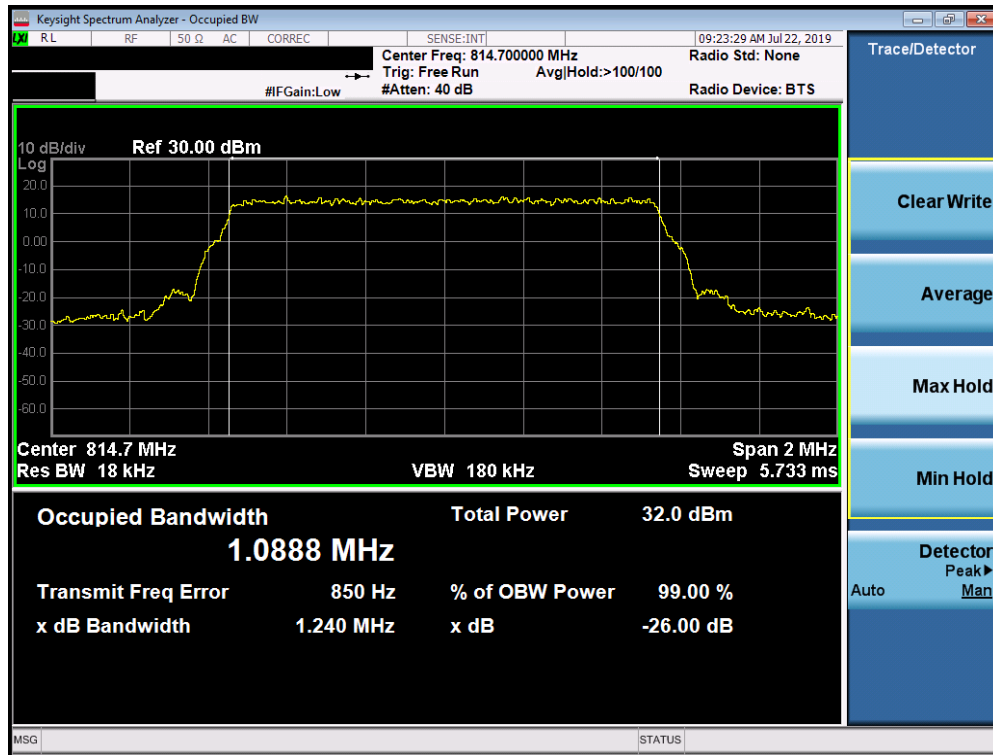
Plot 7-3. Occupied Bandwidth Plot (LTE Band 26, 1.4MHz 64-QAM – RB Size 6– Low Channel)
