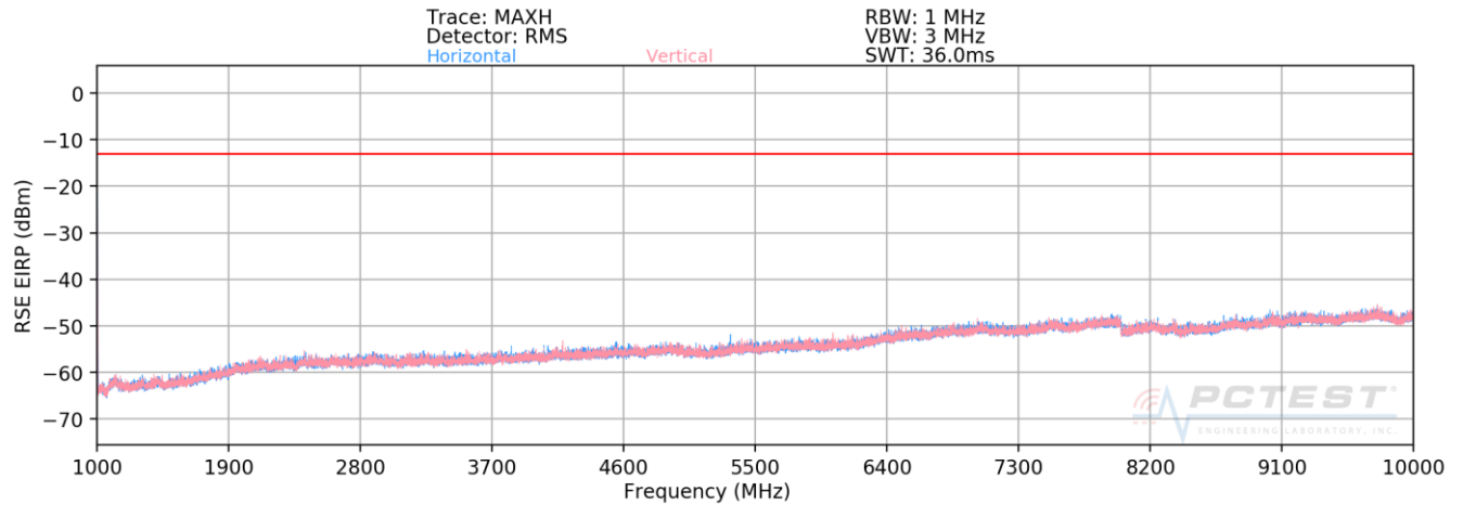
Plot 7-46. Radiated Spurious Plot above 1GHz (Band 26)
