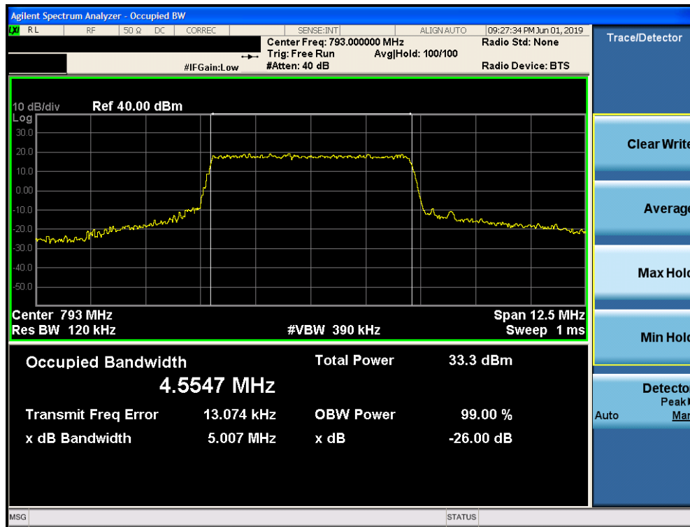
Plot 7-13. Occupied Bandwidth Plot (LTE Band 14, 5MHz QPSK – RB Size 25)
