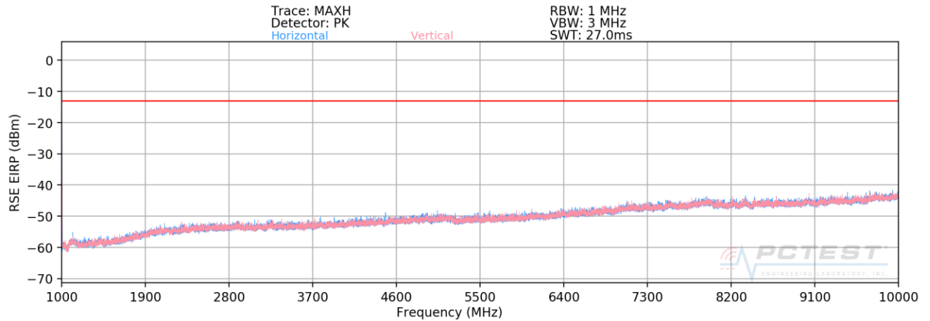
Plot 7-49. Radiated Spurious Plot above 1GHz (Band 14)
