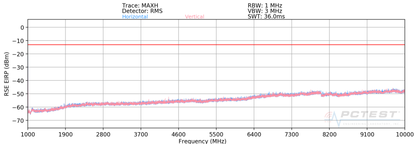
Plot 7-47. Radiated Spurious Plot above 1GHz (Band 14)
