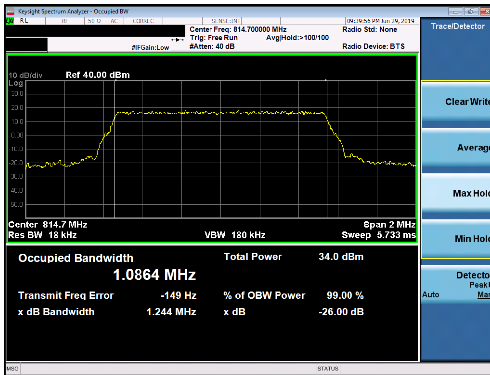
Plot 7-1. Occupied Bandwidth Plot (LTE Band 26, 1.4MHz QPSK – RB Size 6– Low Channel)
