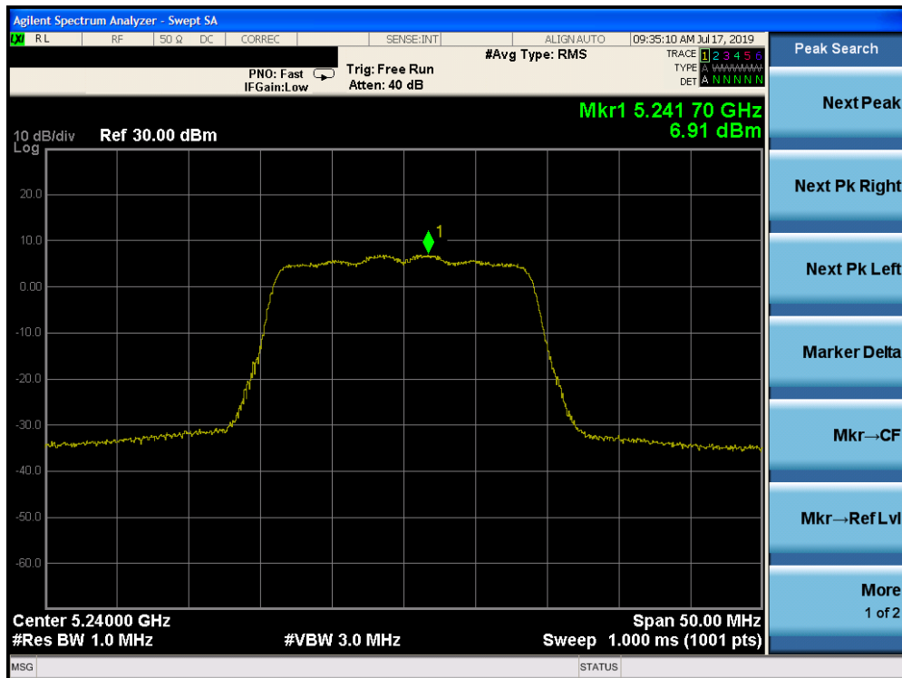
Plot 7-87. Power Spectral Density Plot SISO CORE 1 (20MHz BW 802.11n (UNII Band 1) – Ch. 48)
