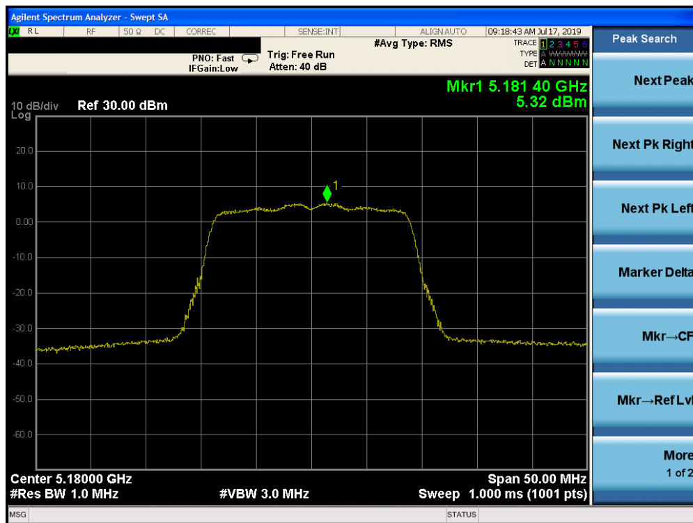
Plot 7-82. Power Spectral Density Plot SISO CORE 1 (20MHz BW 802.11n (UNII Band 1) – Ch. 36) - ISED
