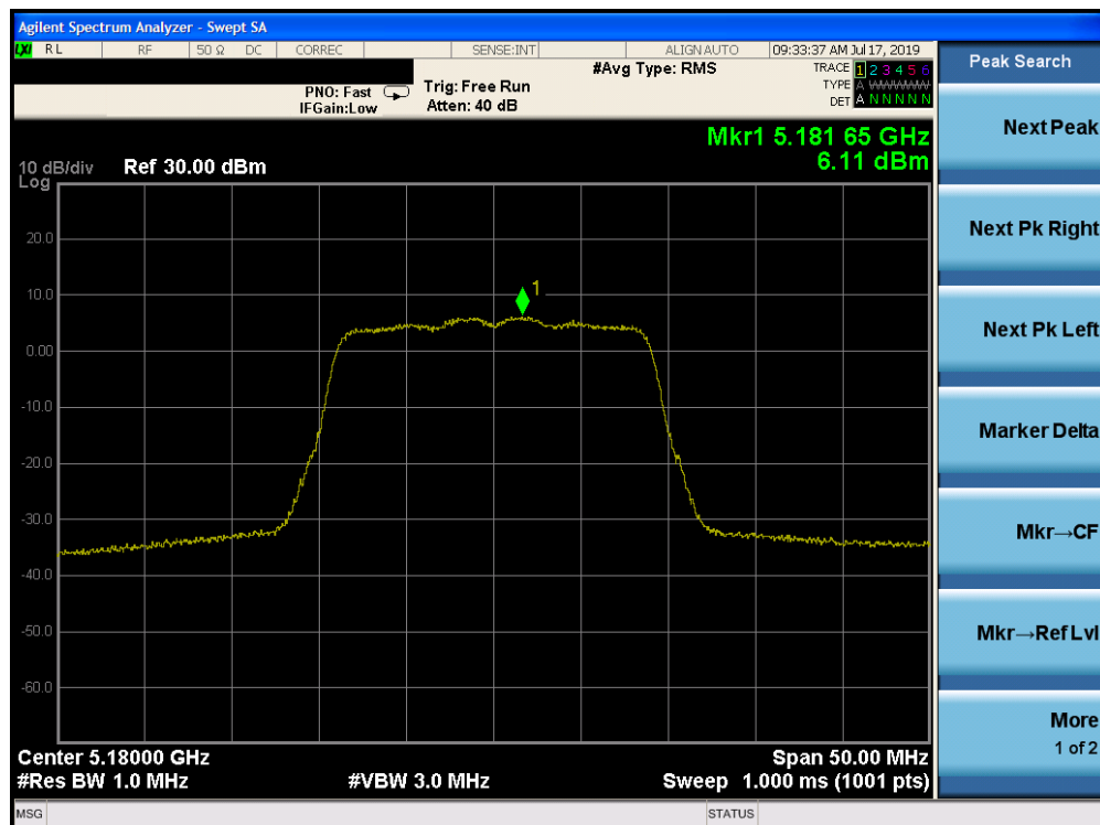
Plot 7-85. Power Spectral Density Plot SISO CORE 1 (20MHz BW 802.11n (UNII Band 1) – Ch. 36)
