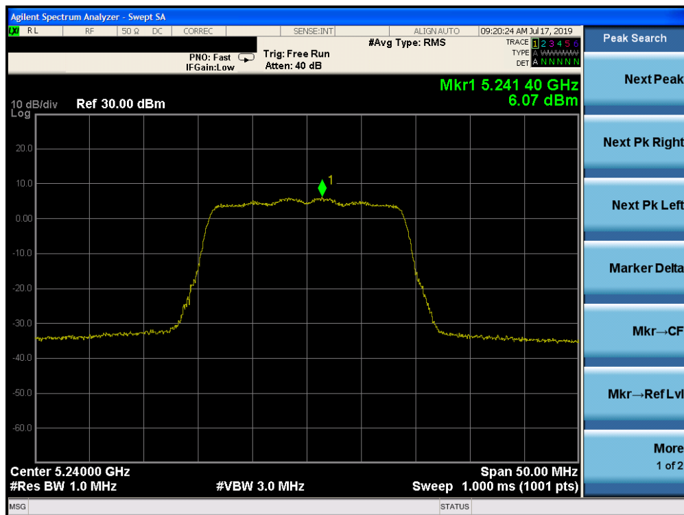
Plot 7-84. Power Spectral Density Plot SISO CORE 1 (20MHz BW 802.11n (UNII Band 1) – Ch. 48) - ISED
