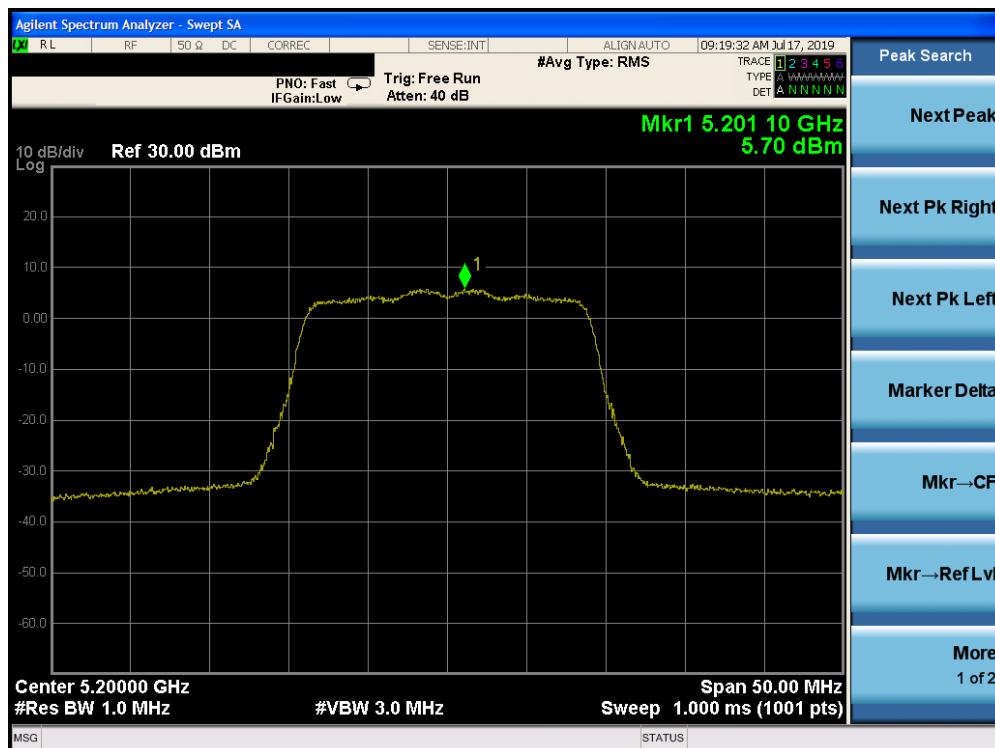
Plot 7-83. Power Spectral Density Plot SISO CORE 1 (20MHz BW 802.11n (UNII Band 1) – Ch. 40) - ISED
