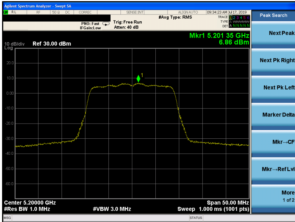
Plot 7-86. Power Spectral Density Plot SISO CORE 1 (20MHz BW 802.11n (UNII Band 1) – Ch. 40)
