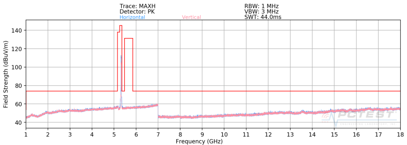
Plot 7-186. Radiated Spurious Plot above 1GHz SISO CORE 1 (802.11n – U2A Ch. 64)
