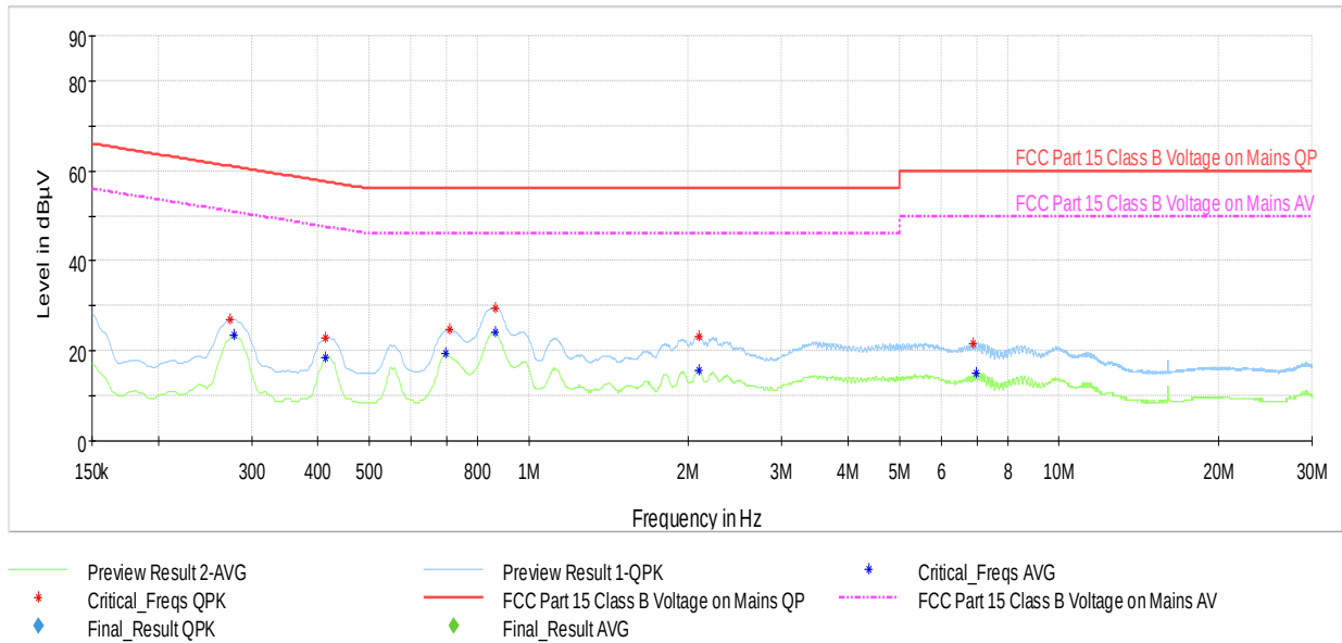
Plot 7-121. AC Line Conducted Plot with 802.11n CDD Ch.6 (L1, with AC/DC Adapter)
