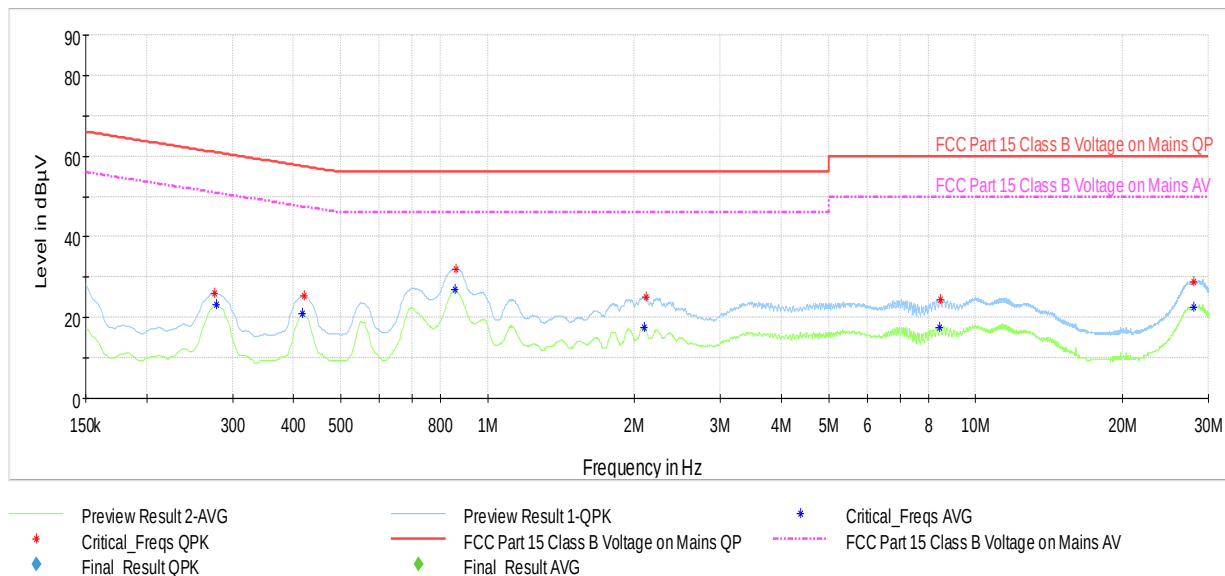
Plot 7-122. AC Line Conducted Plot with 802.11n CDD Ch.6 (N, WITH AC/DC Adapter)
