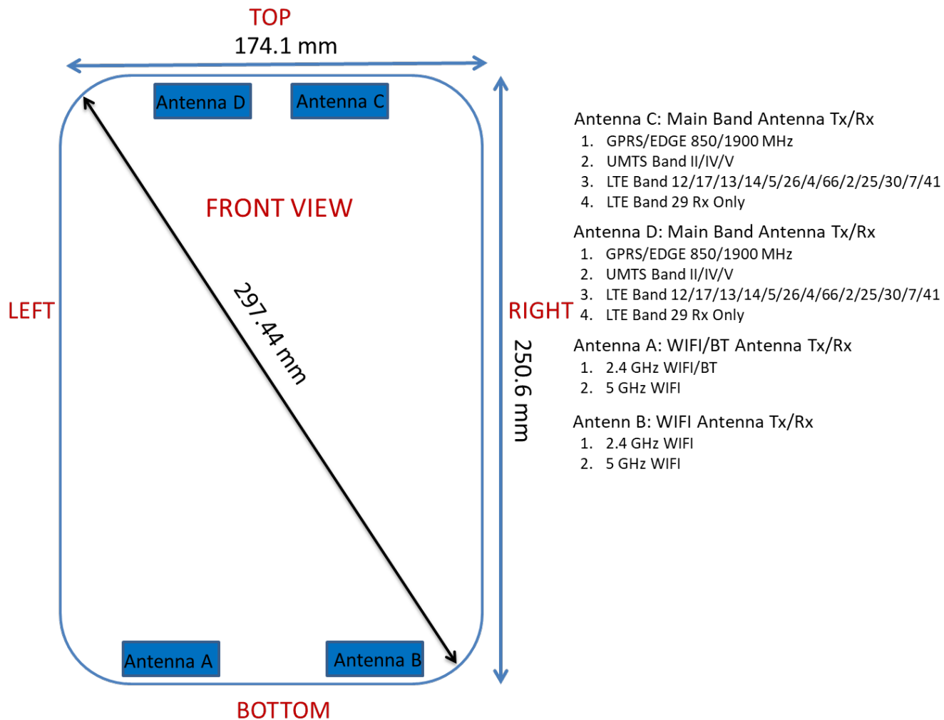
Figure F-1 DUT Antenna Locations
