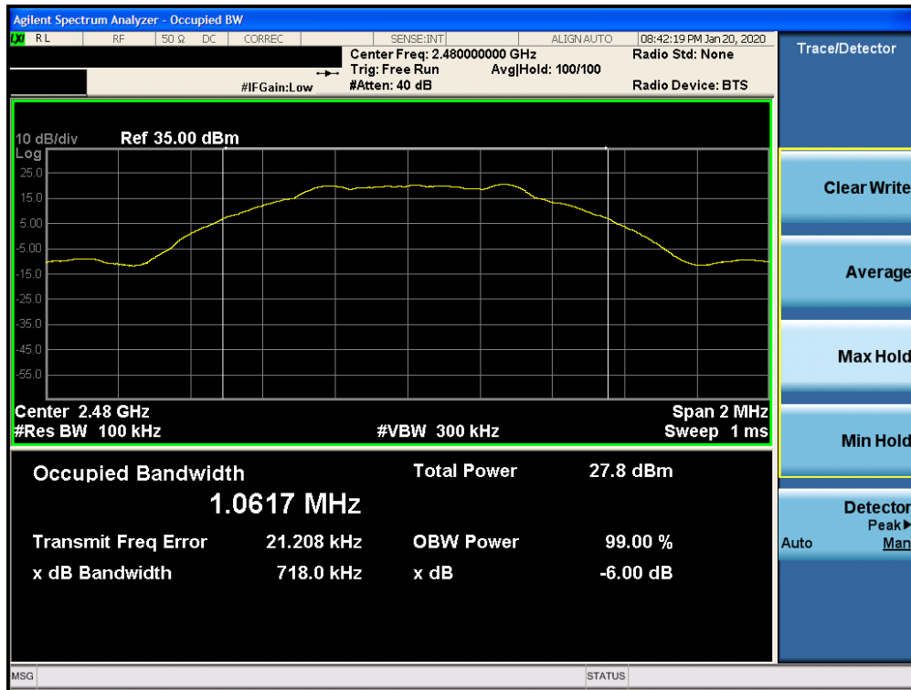
Plot 7-3. 6dB Bandwidth Plot Ant WF8 (Bluetooth (LE), 1Mbps, ePA – Ch. 39)
