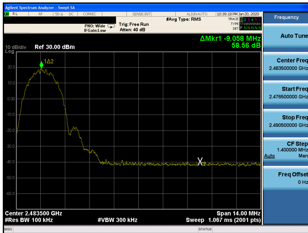
Plot 7-64. Band Edge Plot Ant WF8 (Bluetooth (LE), 2Mbps ePA – Ch. 38)
