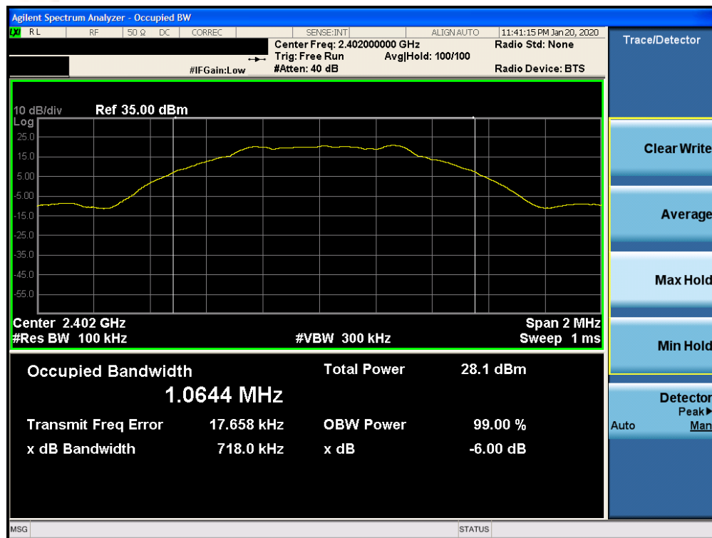
Plot 7-7. 6dB Bandwidth Plot Ant WF7 (Bluetooth (LE), 1Mbps, ePA – Ch. 0)
