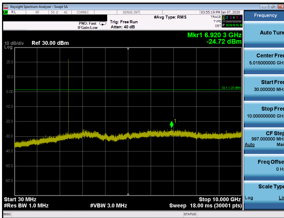
Plot 7-45. Conducted Spurious Plot Ant WF8 (Bluetooth, GFSK, ePA – Ch. 0)
