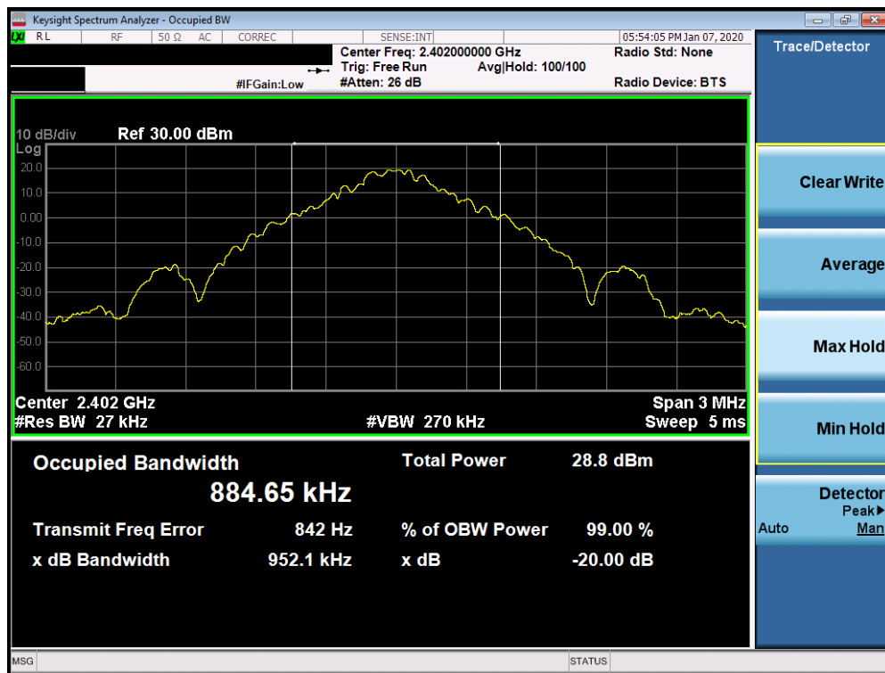
Plot 7-7. 20dB Bandwidth Plot Ant WF7 (Bluetooth, GFSK, ePA – Ch. 0)
