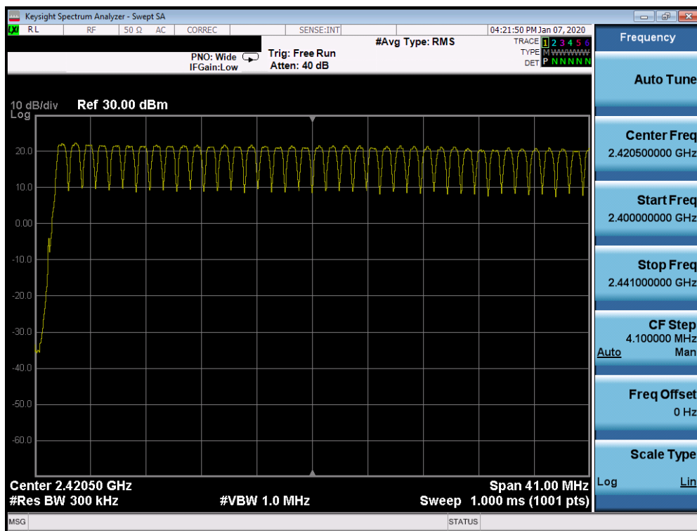
Plot 7-37. Low End Spectrum Channel Hopping Plot Ant WF8 (Bluetooth, GFSK, ePA)
