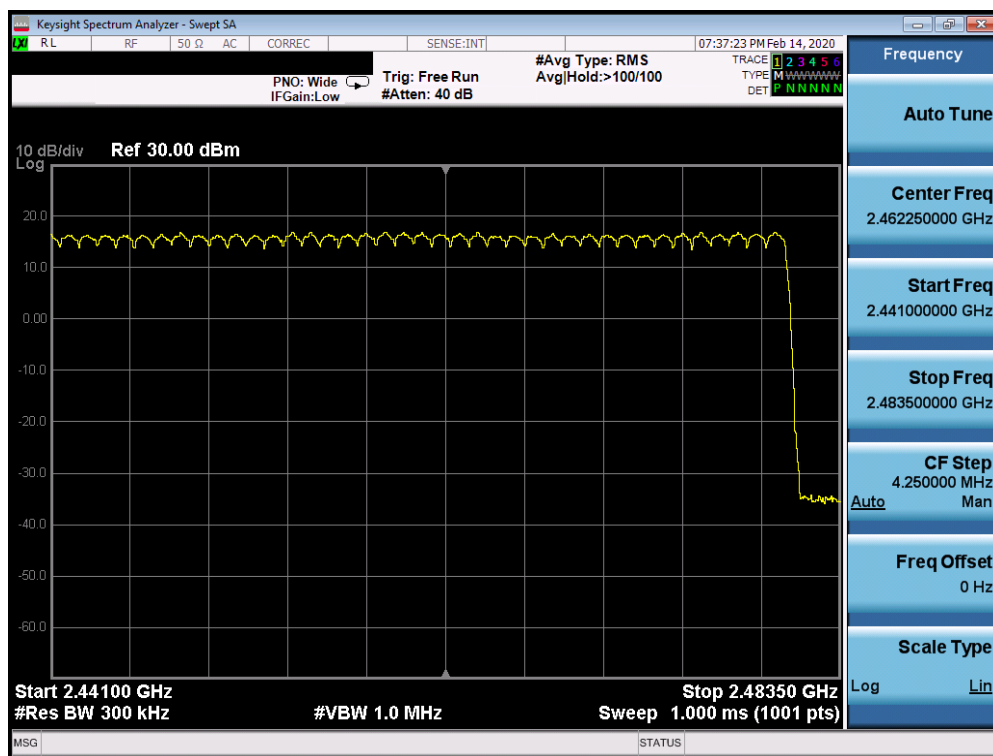
Plot 7-44. High End Spectrum Channel Hopping Plot Ant WF7 (Bluetooth, 8DPSK, ePA)
