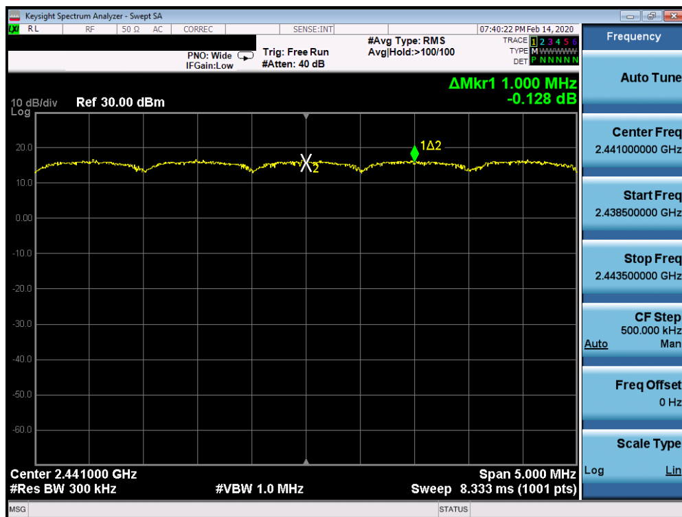
Plot 7-32. Channel Spacing Plot Ant WF7 (Bluetooth, 8DPSK, ePA)
