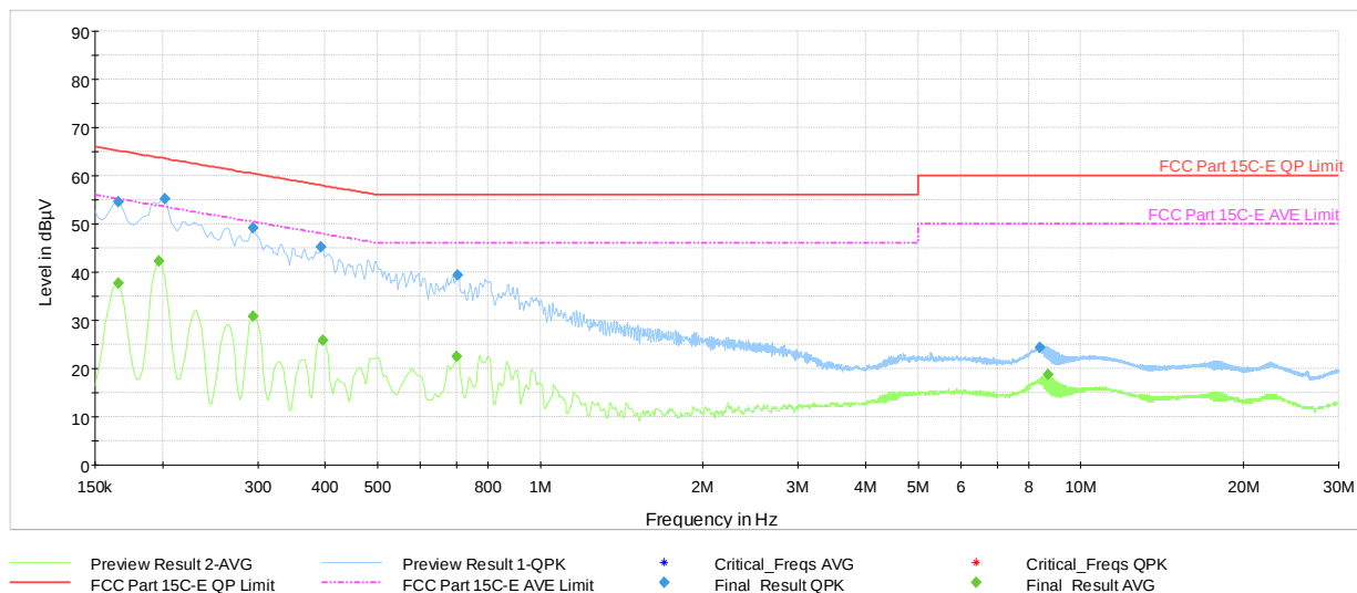
Plot 7-81. Line-Conducted Test Plot- Ch.39 TxBF (L1, with AC/DC Adapter)
