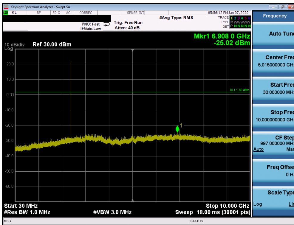
Plot 7-51. Conducted Spurious Plot Ant WF7 (Bluetooth, GFSK, ePA – Ch. 0)
