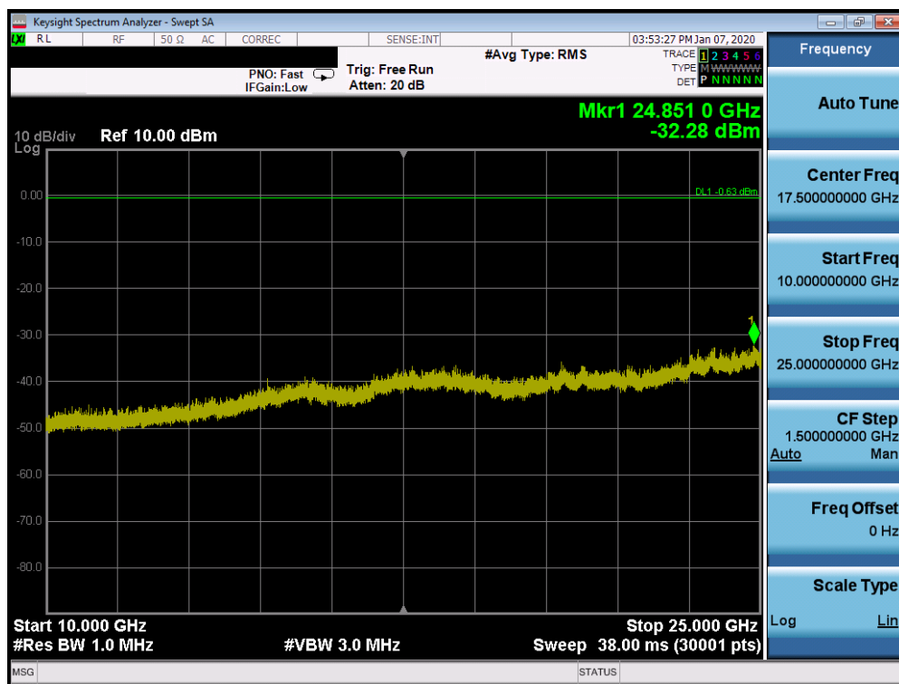
Plot 7-48. Conducted Spurious Plot Ant WF8 (Bluetooth, GFSK, ePA Ch. 39)
