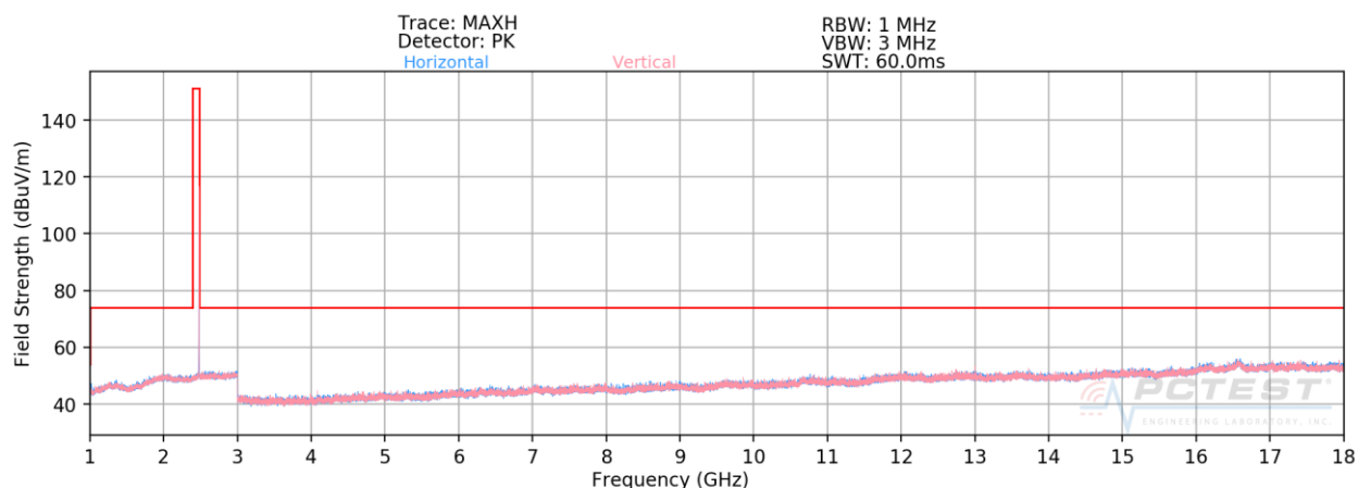
Plot 7-62. Radiated Spurious Plot above 1GHz Ant WF7 (BT GFSK ePA – Ch. 78)
