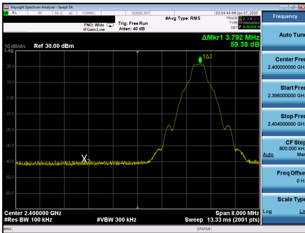
Plot 7-13. Band Edge Plot Ant WF8 (Bluetooth with Hopping Disabled, GFSK, ePA – Ch. 0)
