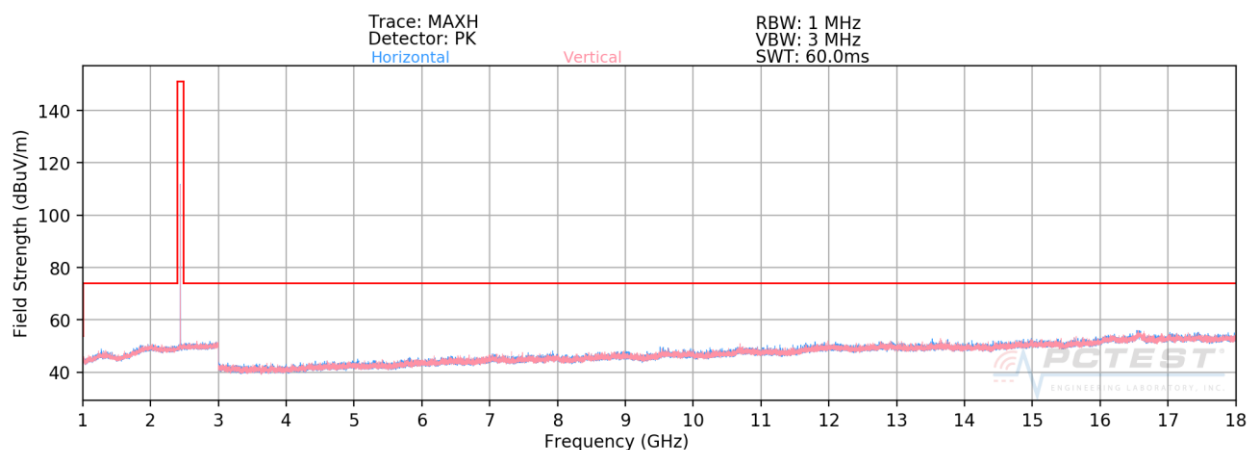
Plot 7-61. Radiated Spurious Plot above 1GHz Ant WF7 (BT GFSK ePA – Ch. 39)
