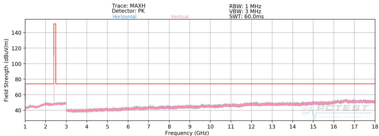
Plot 7-60. Radiated Spurious Plot above 1GHz Ant WF7 (BT GFSK ePA – Ch. 0)
