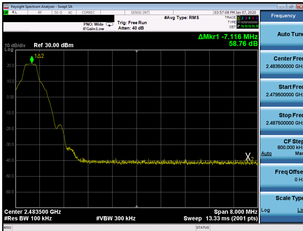
Plot 7-14. Band Edge Plot Ant WF8 (Bluetooth with Hopping Disabled, GFSK, ePA – Ch. 78)
