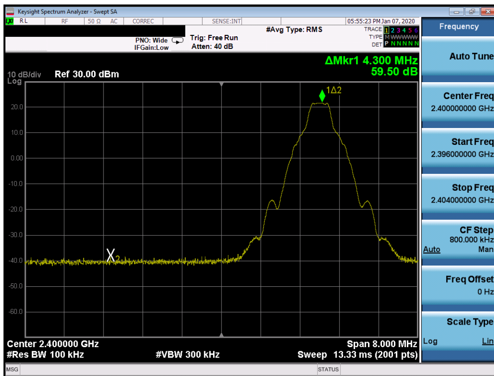
Plot 7-21. Band Edge Plot Ant WF7 (Bluetooth with Hopping Disabled, GFSK, ePA – Ch. 0)
