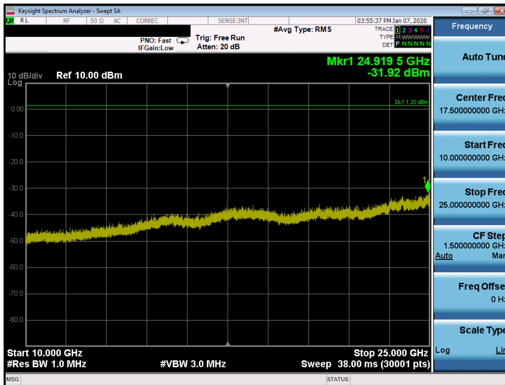
Plot 7-46. Conducted Spurious Plot Ant WF8 (Bluetooth, GFSK, ePA – Ch. 0)
