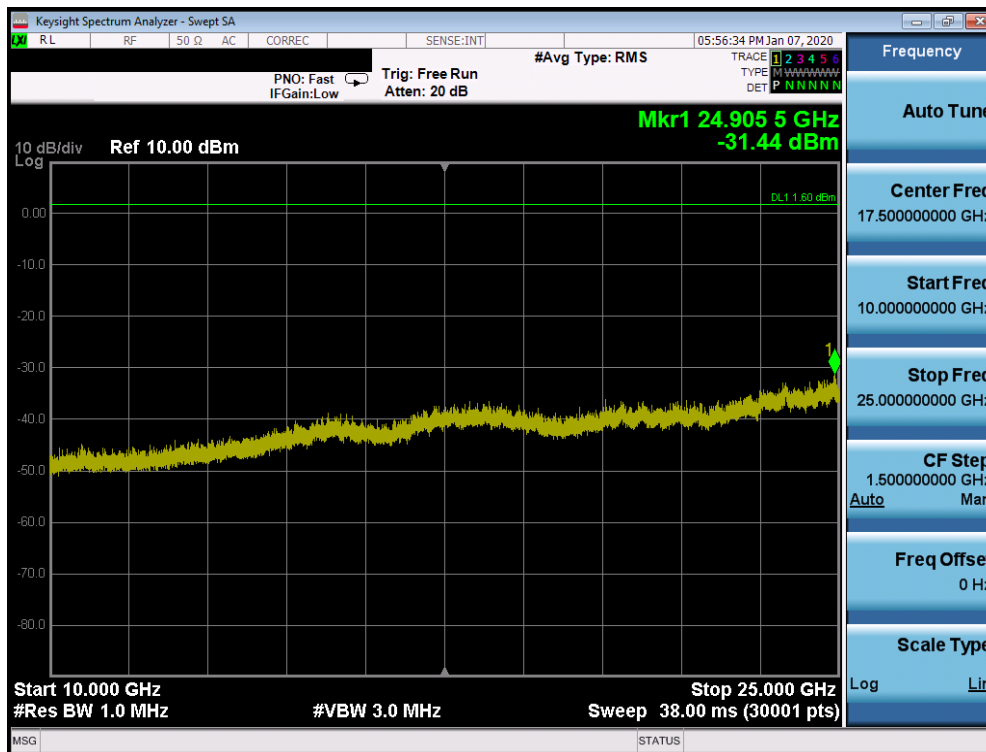
Plot 7-52. Conducted Spurious Plot Ant WF7 (Bluetooth, GFSK, ePA – Ch. 0)
