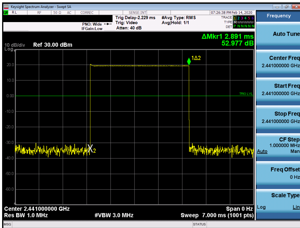
Plot 7-36. Time of Occupancy Plot Ant WF7 (Bluetooth, 8DPSK, ePA)
