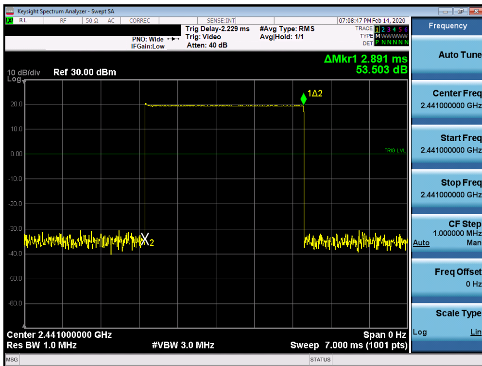
Plot 7-35. Time of Occupancy Plot Ant WF7 (Bluetooth, GFSK, ePA)
