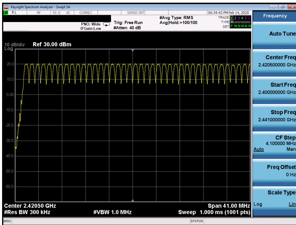
Plot 7-41. Low End Spectrum Channel Hopping Plot Ant WF7 (Bluetooth, GFSK, ePA)
