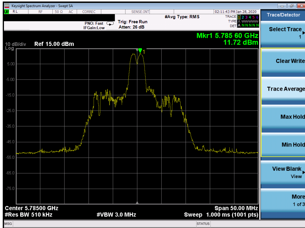
Plot 7-314. Power Spectral Density Plot SISO CORE 0 (20MHz BW 802.11ax Index 4 – RU26 (UNII Band 3) – Ch. 157)
