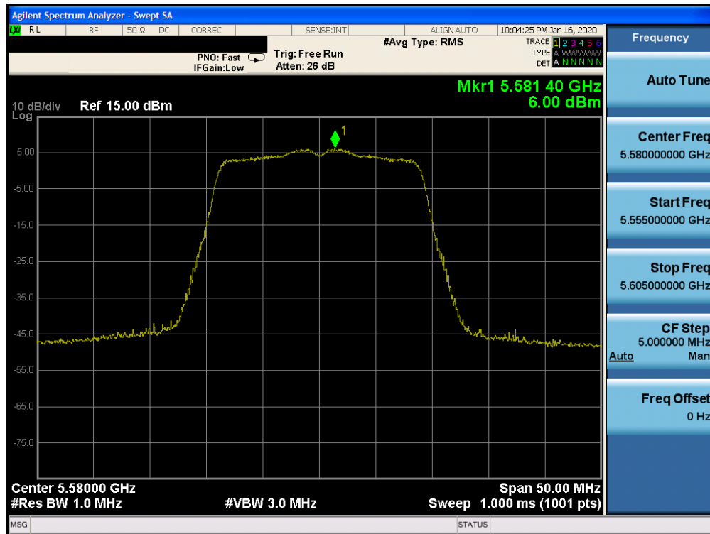
Plot 7-142. Power Spectral Density Plot CDD CORE 0 (20MHz BW 802.11n (UNII Band 2C) – Ch. 116)
