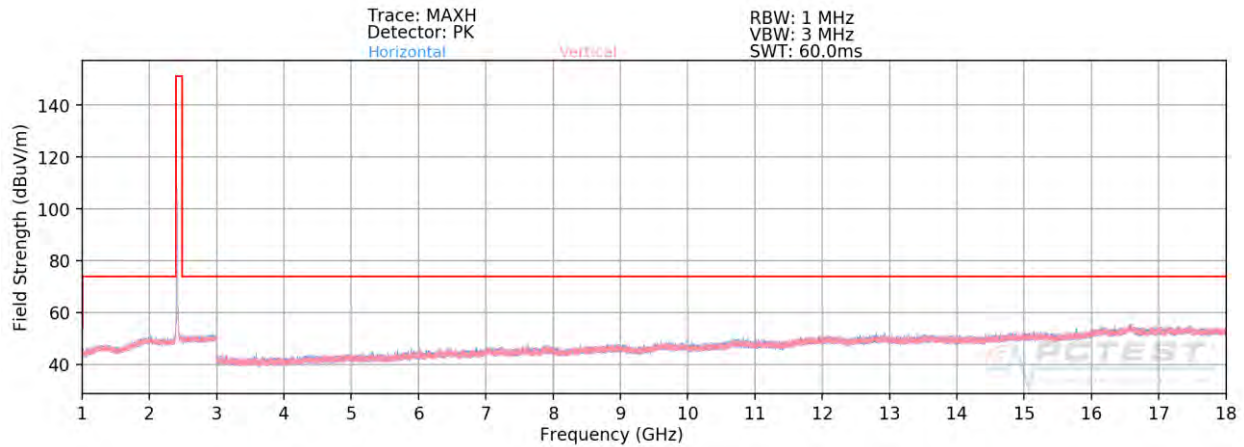
Plot 7-96. Radiated Spurious Plot above 1GHz SISO CORE 1 (802.11b – Ch. 1)
