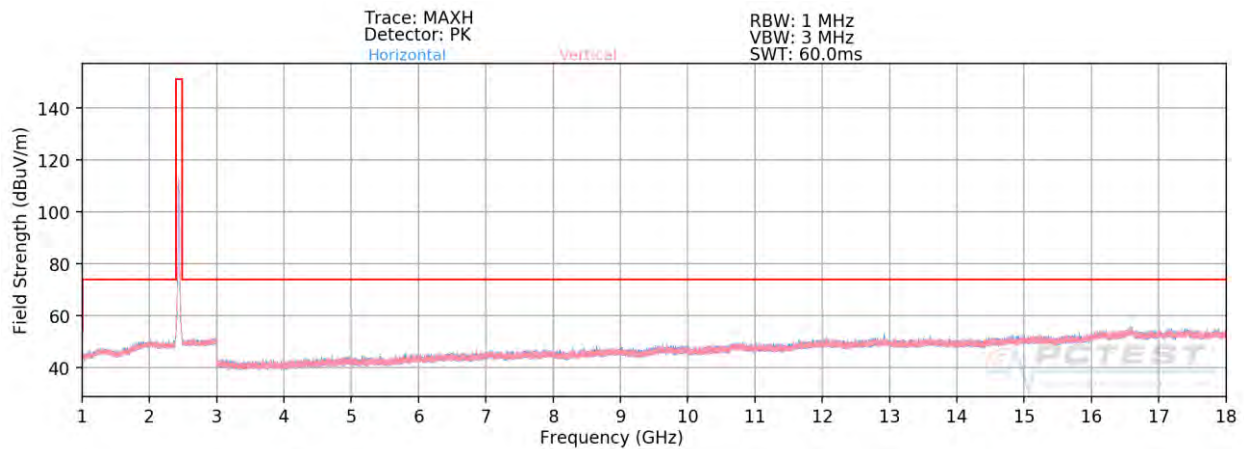
Plot 7-100. Radiated Spurious Plot above 1GHz CDD (802.11n – Ch. 6)
