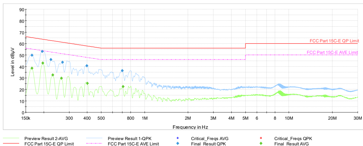
Plot 7-132. Line Conducted Plot with 802.11n CDD Ch.6 (L1, with AC/DC Adapter)
