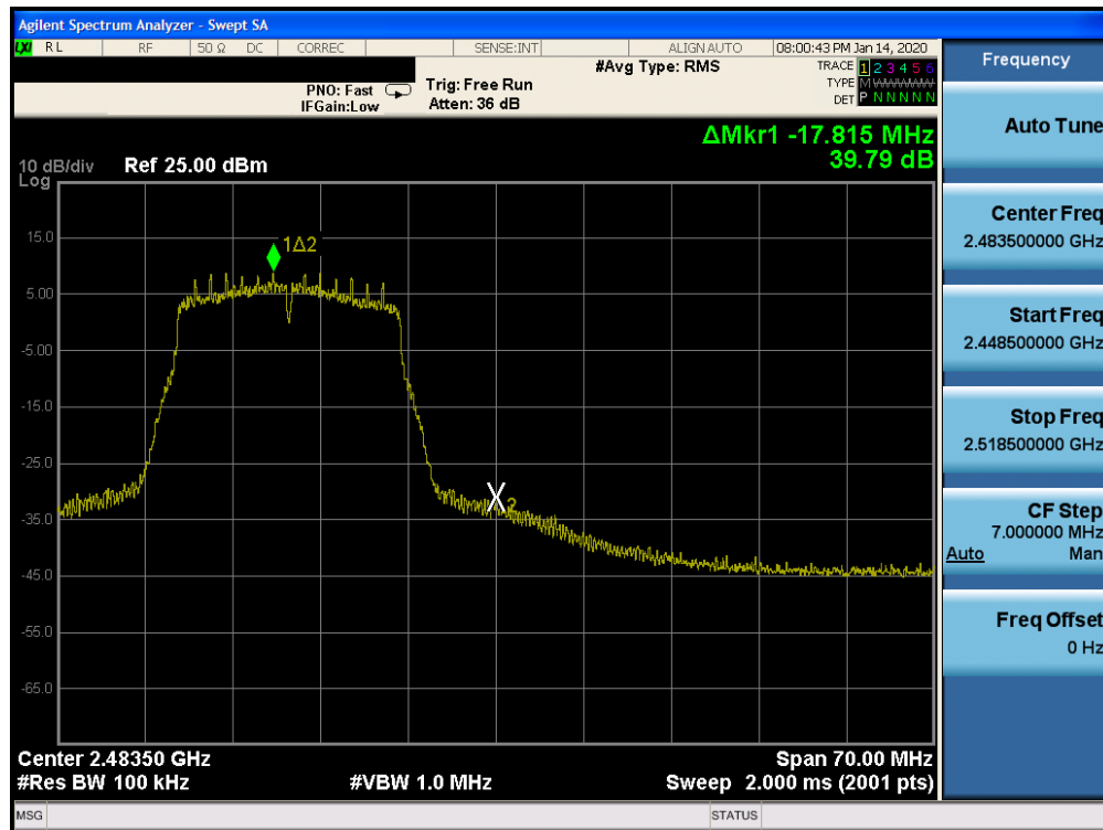
Plot 7-63. Band Edge Plot SISO CORE 0 (802.11n – Ch. 12)
