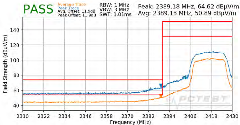
Plot 7-119. Radiated Restricted Lower Band Edge Measurement SISO CORE 1
