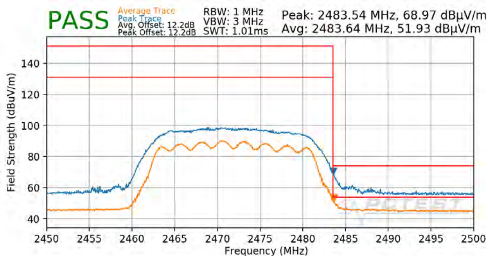
Plot 7-130. Radiated Restricted Upper Band Edge Measurement CDD
