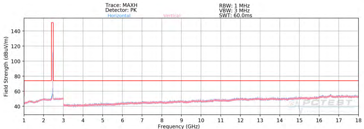
Plot 7-95. Radiated Spurious Plot above 1GHz SISO CORE 0 (802.11b – Ch. 11)
