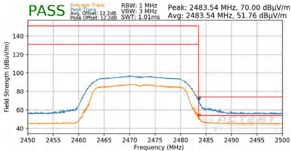
Plot 7-113. Radiated Restricted Upper Band Edge Measurement SISO CORE0
