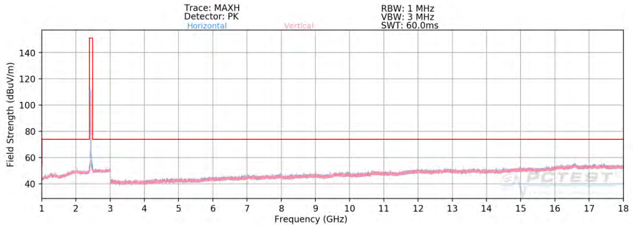
Plot 7-94. Radiated Spurious Plot above 1GHz SISO CORE 0 (802.11b – Ch. 6)
