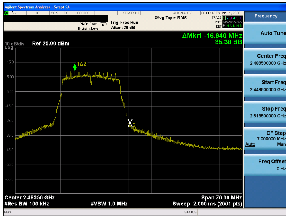
Plot 7-64. Band Edge Plot SISO CORE 0 (802.11n – Ch. 13)
