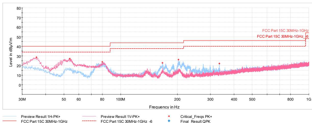
Plot 7-131. Radiated Spurious Plot below 1GHz CDD Ch.6, with AC/DC Adapter
