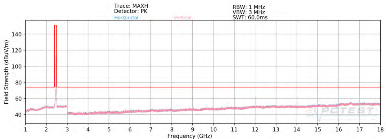
Plot 7-101. Radiated Spurious Plot above 1GHz CDD (802.11n – Ch. 11)
