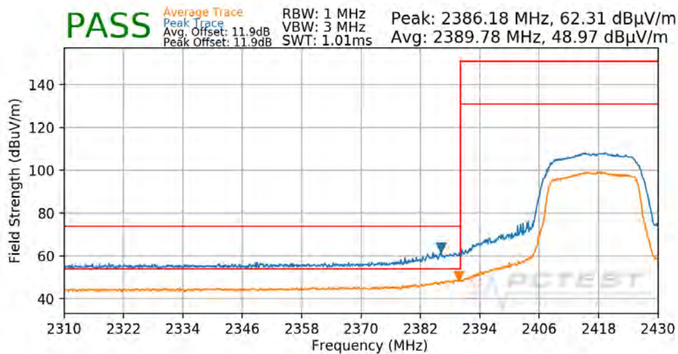
Plot 7-109. Radiated Restricted Lower Band Edge Measurement SISO CORE0
