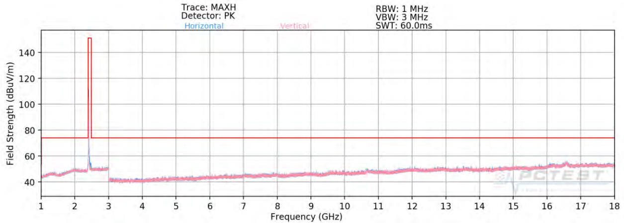
Plot 7-93. Radiated Spurious Plot above 1GHz SISO CORE 0 (802.11b – Ch. 1)
