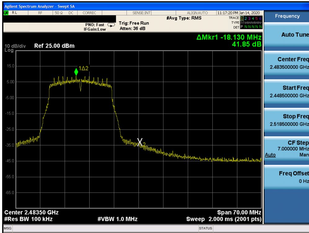
Plot 7-79. Band Edge Plot SISO CORE 1 (802.11n - Ch. 12)
