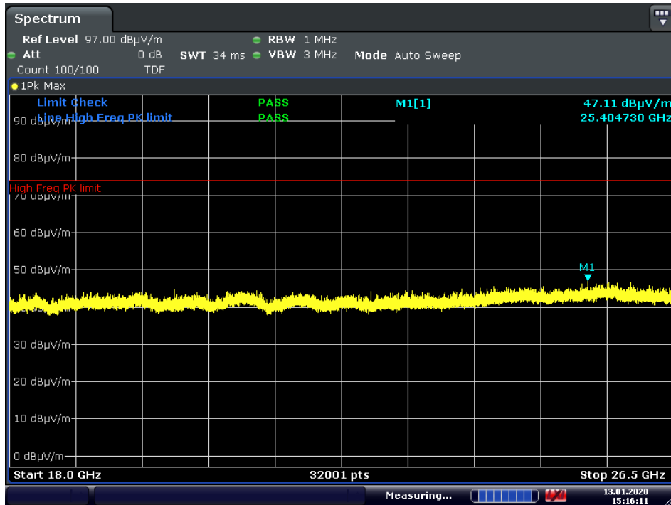
Plot 7-102. Radiated Spurious Plot above 18GHz CDD (802.11n, Pol. H)
