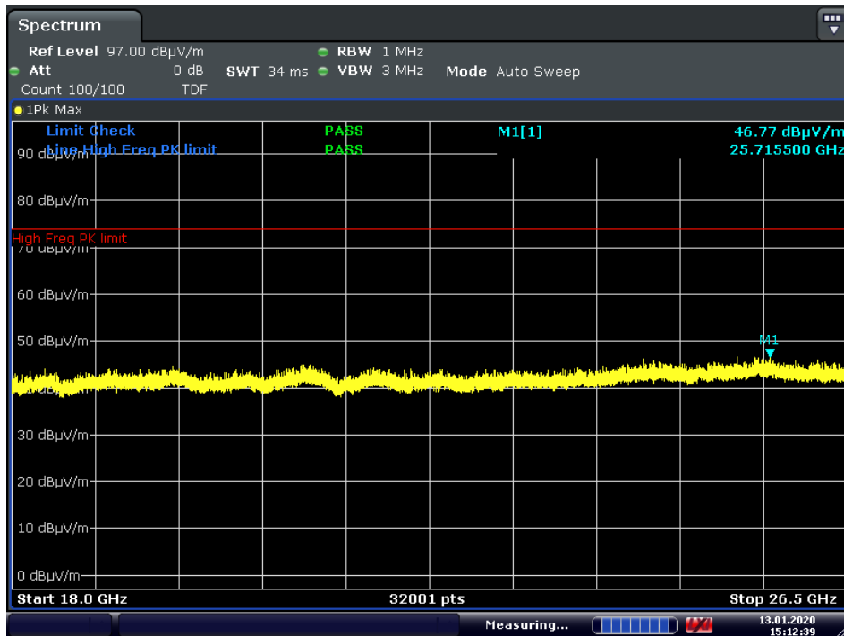
Plot 7-103. Radiated Spurious Plot above 18GHz CDD (802.11n, Pol. V)
