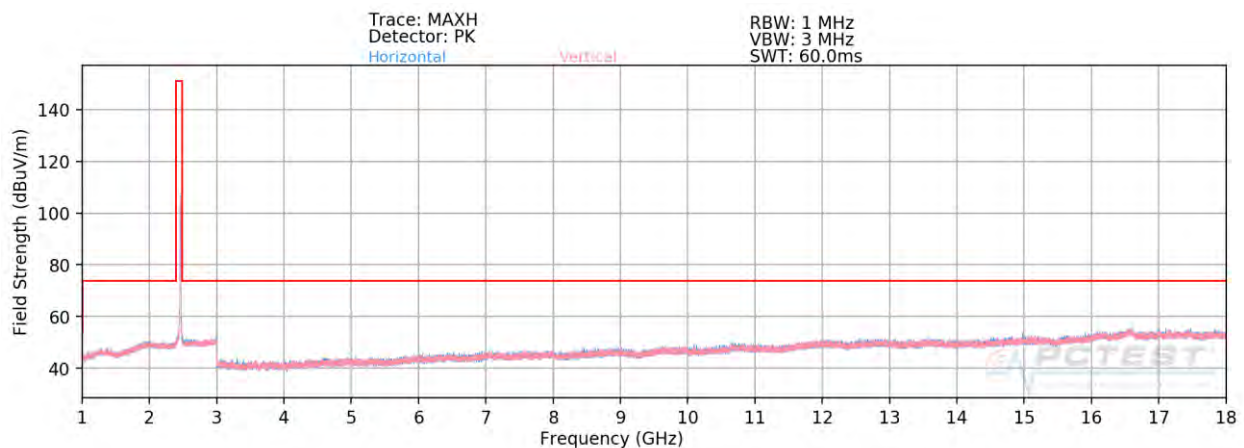
Plot 7-98. Radiated Spurious Plot above 1GHz SISO CORE 1 (802.11b – Ch. 11)
