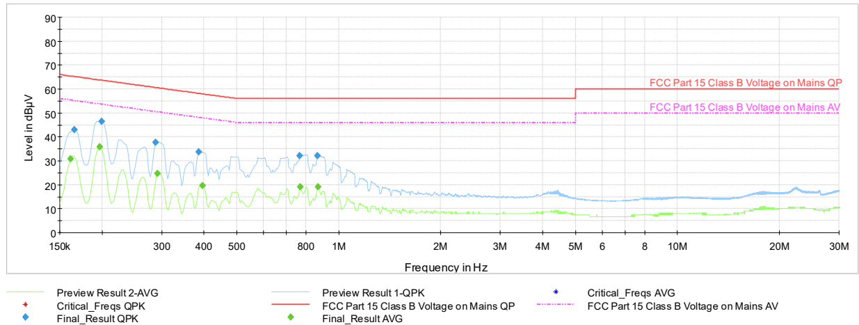
Plot 7-133. Line Conducted Plot with 802.11n CDD Ch.6 (N, with AC/DC Adapter)
