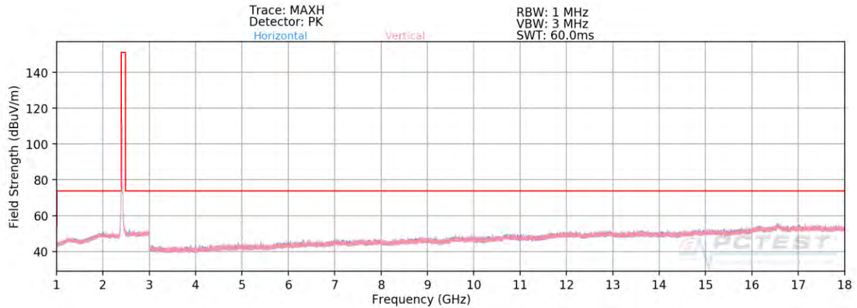
Plot 7-99. Radiated Spurious Plot above 1GHz CDD (802.11n – Ch. 1)
