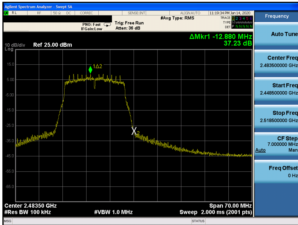
Plot 7-80. Band Edge Plot SISO CORE 1 (802.11n - Ch. 13)
