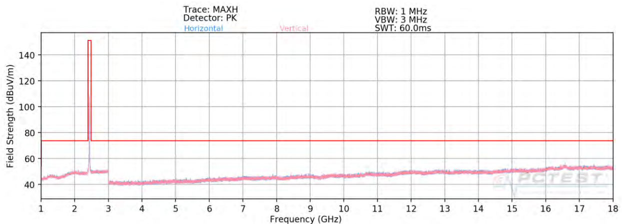
Plot 7-97. Radiated Spurious Plot above 1GHz SISO CORE 1 (802.11b – Ch. 6)
