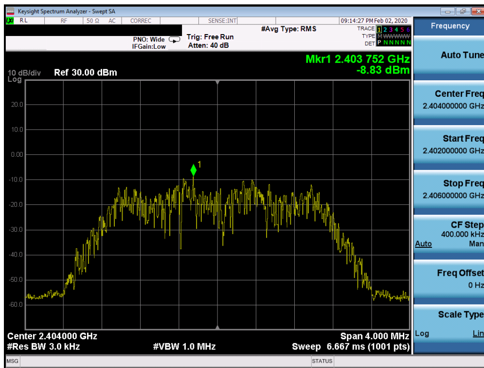
Plot 7-44. Power Spectral Density Plot TxBF Ant WF7 (Bluetooth (HDR4), 4Mbps, iPA – Ch. 1)
