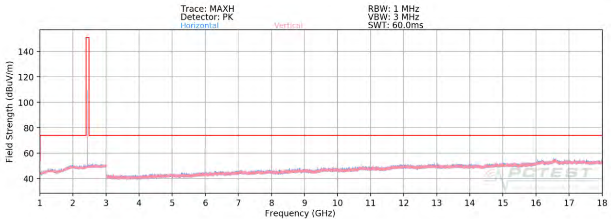
Plot 7-82. Radiated Spurious Plot Above 1GHz Ant WF8 (4Mbps, HDR4 ePA – Ch. 38, Ant. Pol. H & V)
