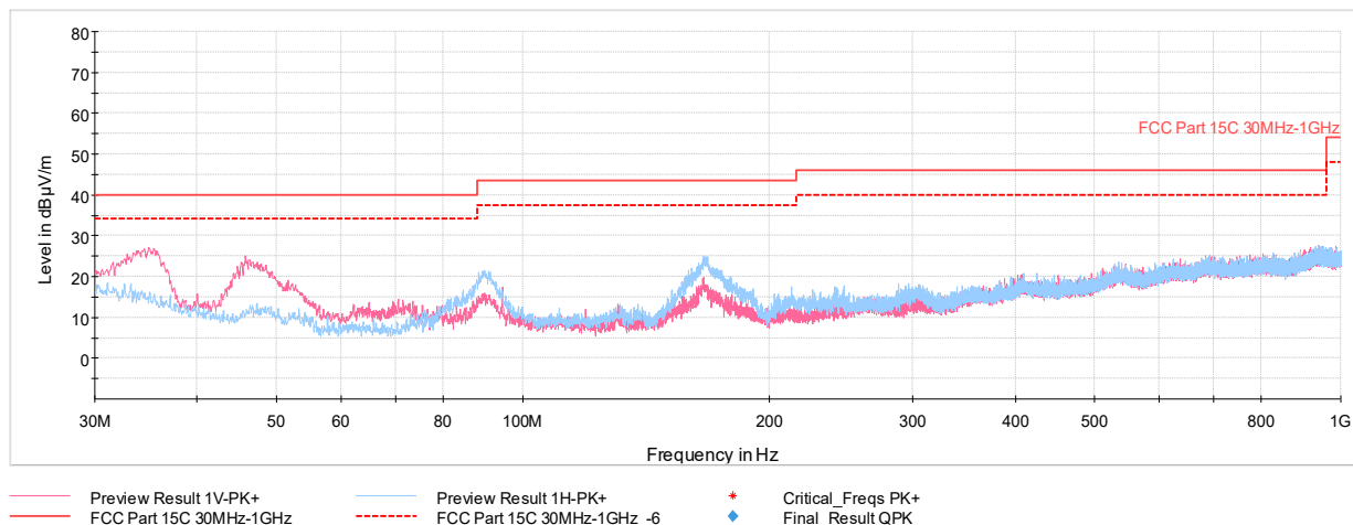
Plot 7-104. Radiated Spurious Plot below 1GHz (4Mbps, ePA – Ch.38 with AC/DC Adapter)
