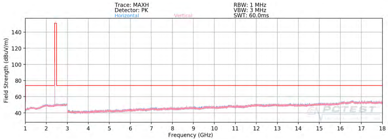
Plot 7-81. Radiated Spurious Plot Above 1GHz Ant WF8 (4Mbps, HDR4 ePA – Ch. 1, Ant. Pol. H & V)
