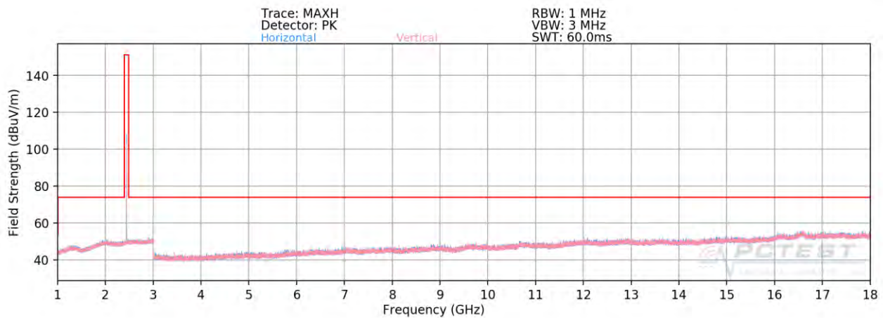
Plot 7-85. Radiated Spurious Plot Above 1GHz Ant WF7 (4Mbps, HDR4 ePA – Ch. 38, Ant. Pol. H & V)
