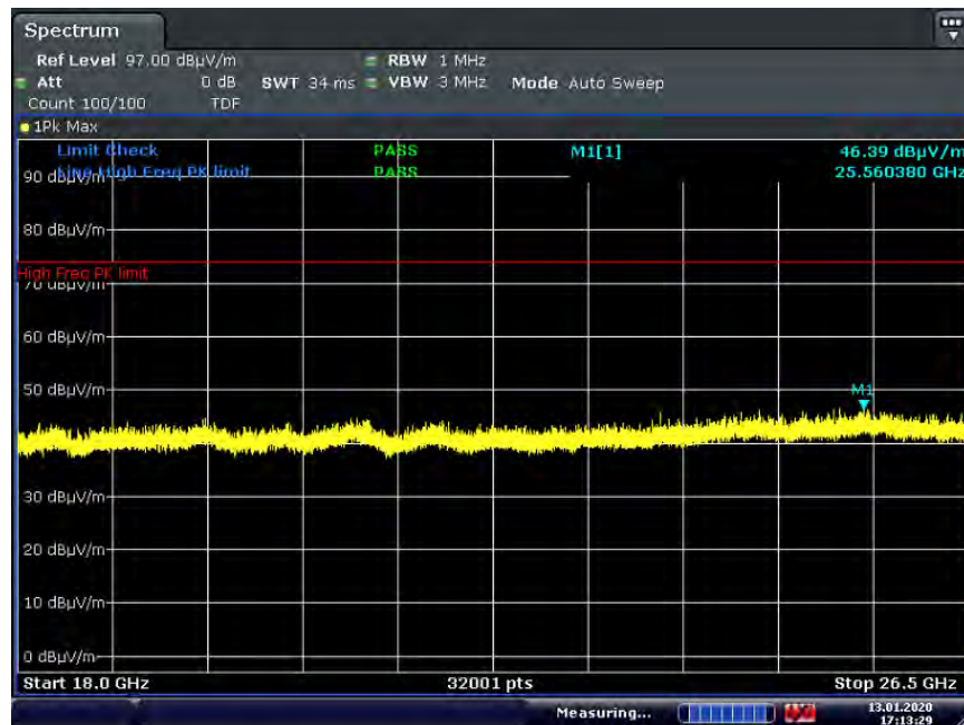
Plot 7-91. Radiated Spurious Plot Above 18GHz Ant WF8 (1Mbps, ePA, Ant. Pol. V)
