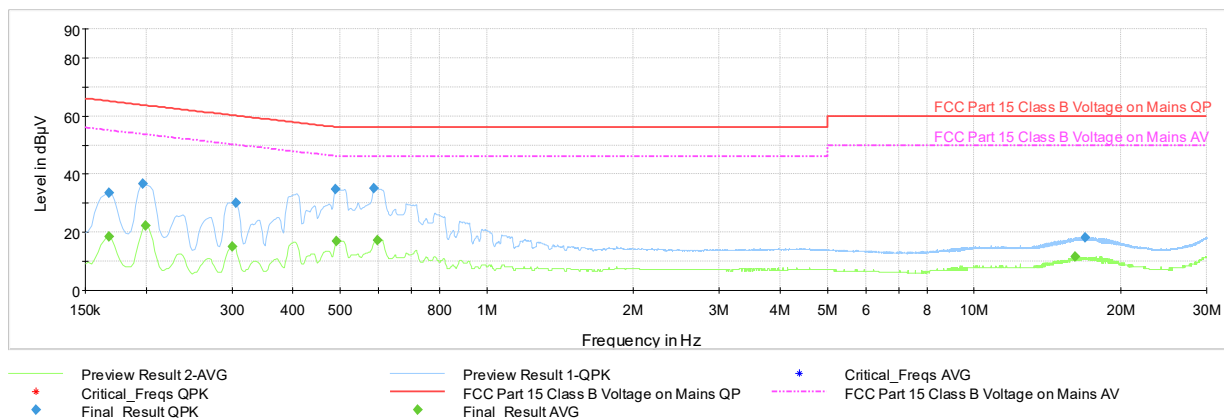
Plot 7-106. Line Conducted Plot with Bluetooth LE (N – 1Mbps, ePA, Ch.19 with AC/DC Adapter)
