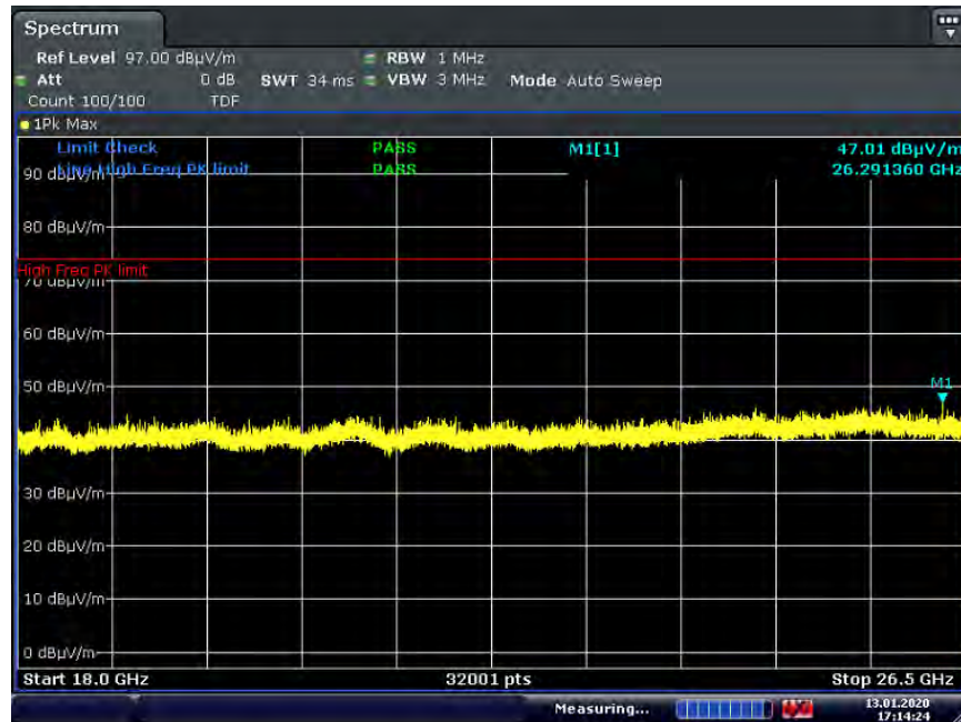
Plot 7-90. Radiated Spurious Plot Above 18GHz Ant WF8 (1Mbps, ePA, Ant. Pol. H)
