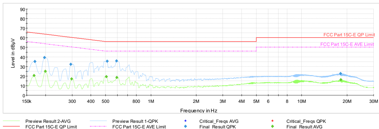
Plot 7-105. Line Conducted Plot with Bluetooth LE (L1 – 1Mbps, ePA, Ch.19, with AC/DC Adapter)
