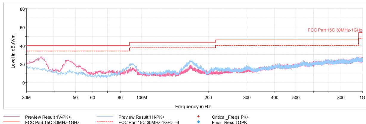
Plot 7-104. Radiated Spurious Plot below 1GHz (1Mbps, ePA Ch.19 with AC/DC Adapter)
