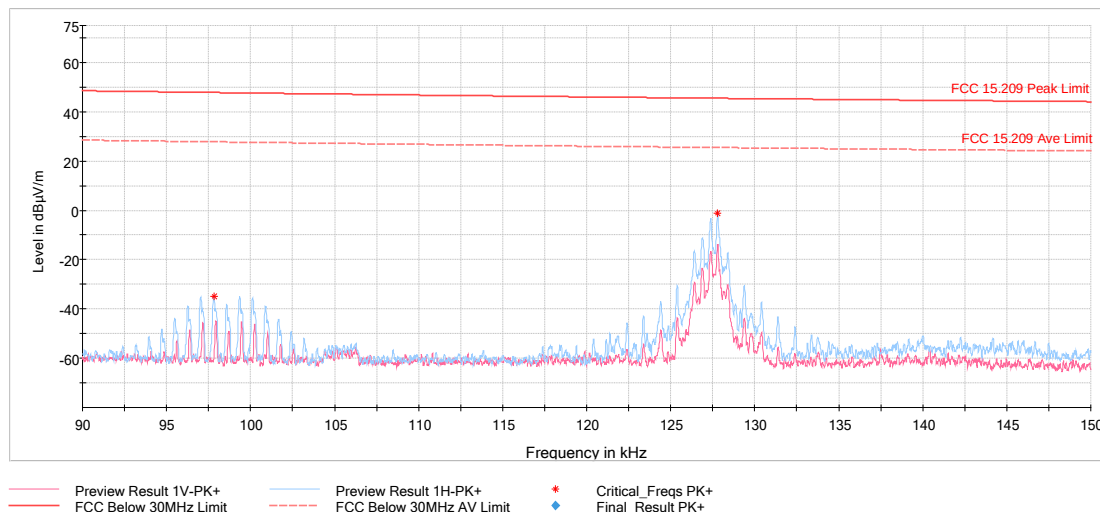
Plot 6-2. Radiated Restricted Lower Band Edge Measurement (Peak)
