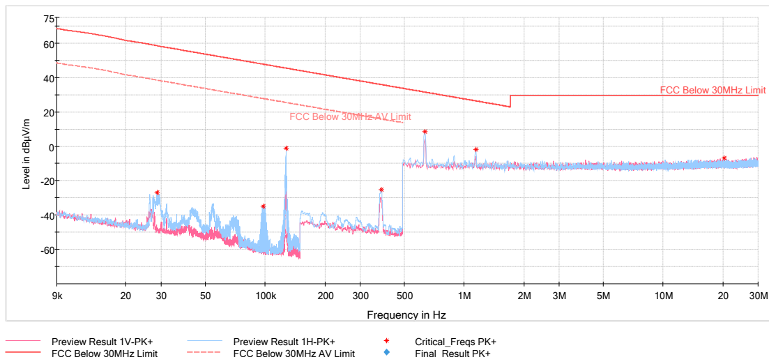
Plot 6-3. Radiated Spurious Plot 9kHz-30MHz with AC/DC Adapter
