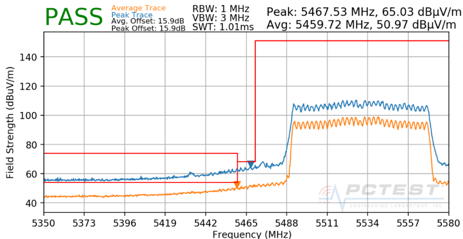
Plot 7-920. Radiated Lower Band Edge Plot CDD (Peak & Average - UNII Band 2C - RU996)
