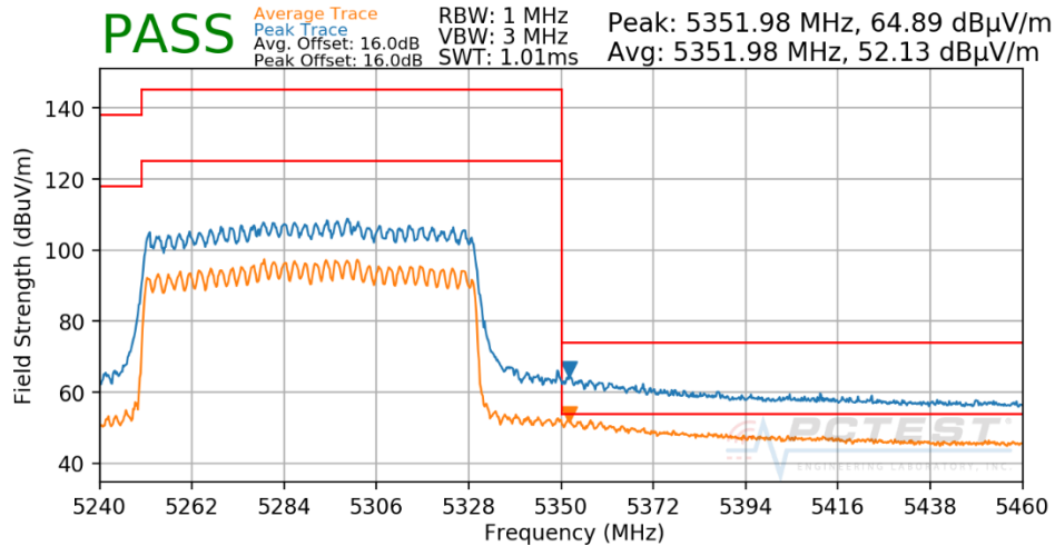
Plot 7-919. Radiated Upper Band Edge Plot CDD (Peak & Average - UNII Band 2A - RU996)
