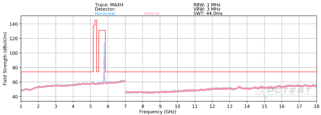
Plot 7-743. Radiated Spurious Plot above 1GHz SISO CORE 0 (802.11ax – U3 Ch. 157 – RU242)
