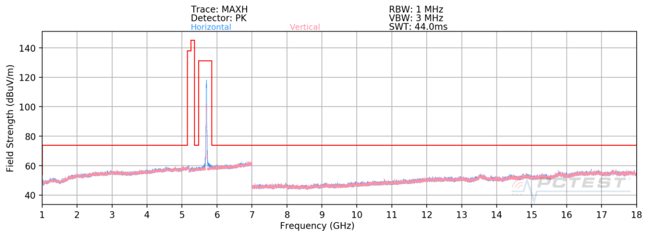
Plot 7-200. Radiated Spurious Plot above 1GHz CDD (802.11n – U2C Ch. 144)
