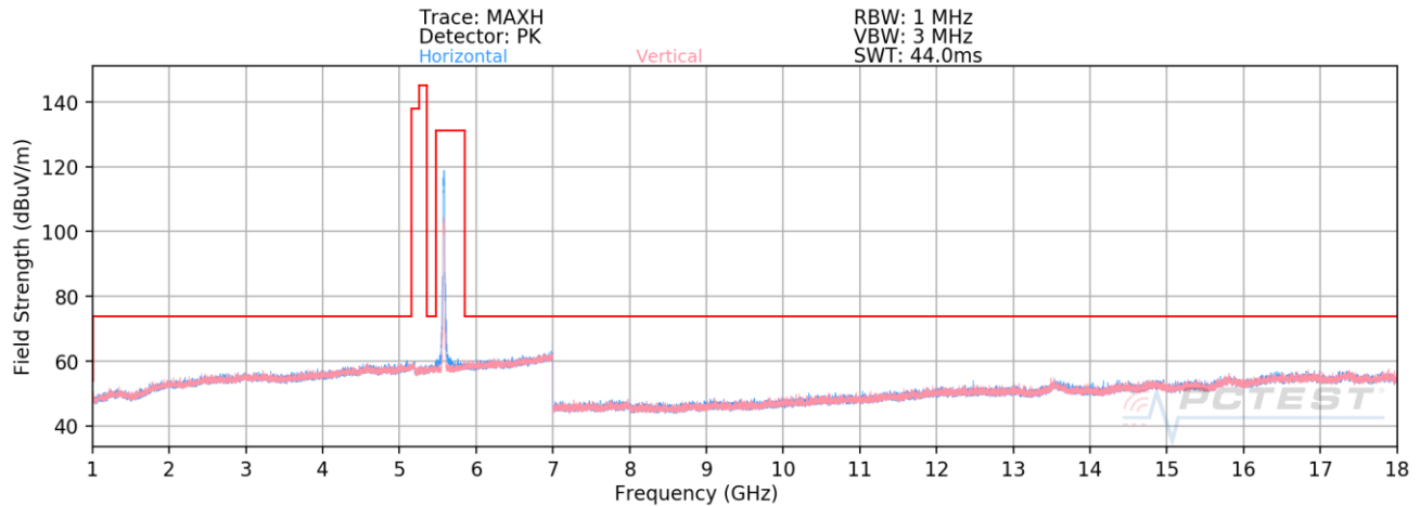
Plot 7-199. Radiated Spurious Plot above 1GHz CDD (802.11n – U2C Ch. 116)
