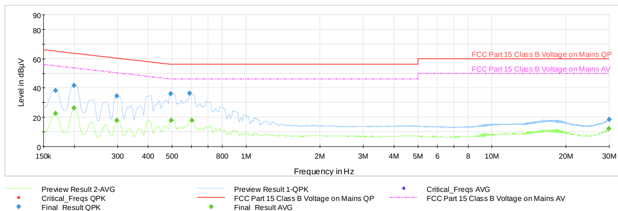
Plot 7-281. Line Conducted Plot with 802.11n UNII Band 1 (N)
