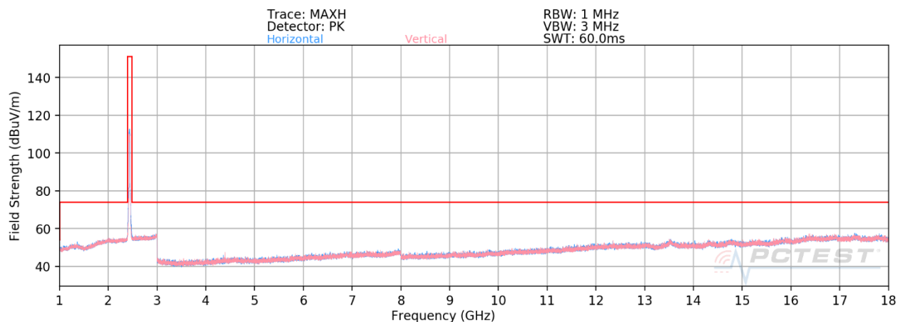
Plot 7-133. Radiated Spurious Plot above 1GHz SISO CORE 1 (802.11ax OFDMA – RU242 – Ch. 6)
