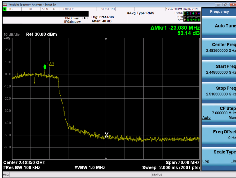
Plot 7-81. Band Edge Plot SISO CORE1 (802.11n (2.4GHz) – Ch. 10)
