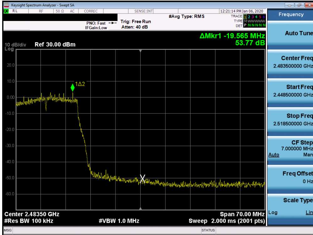
Plot 7-63. Band Edge Plot SISO CORE0 (802.11n (2.4GHz) – Ch. 10)
