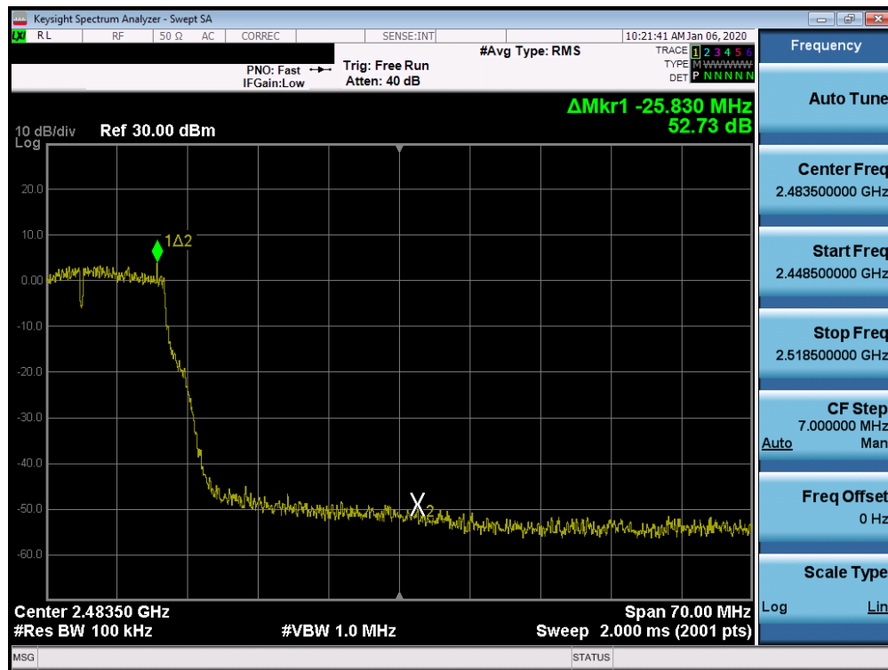
Plot 7-55. Band Edge Plot SISO CORE0 (802.11g – Ch. 9)
