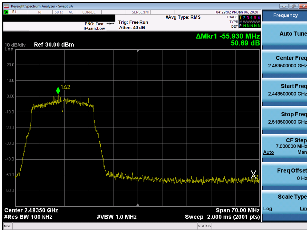
Plot 7-64. Band Edge Plot SISO CORE0 (802.11n (2.4GHz) – Ch. 11)
