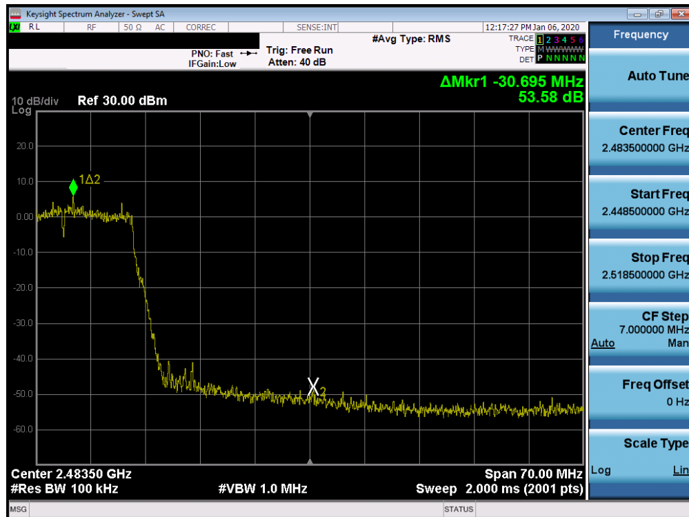
Plot 7-62. Band Edge Plot SISO CORE0 (802.11n (2.4GHz) – Ch. 9)
