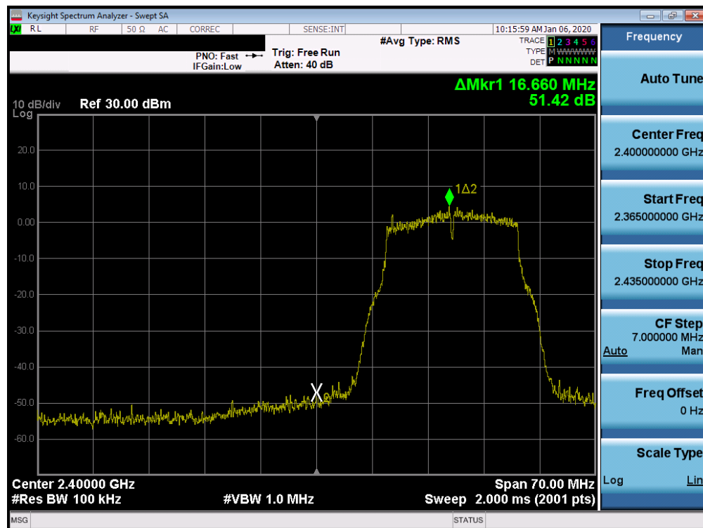
Plot 7-54. Band Edge Plot SISO CORE0 (802.11g- Ch. 2)
