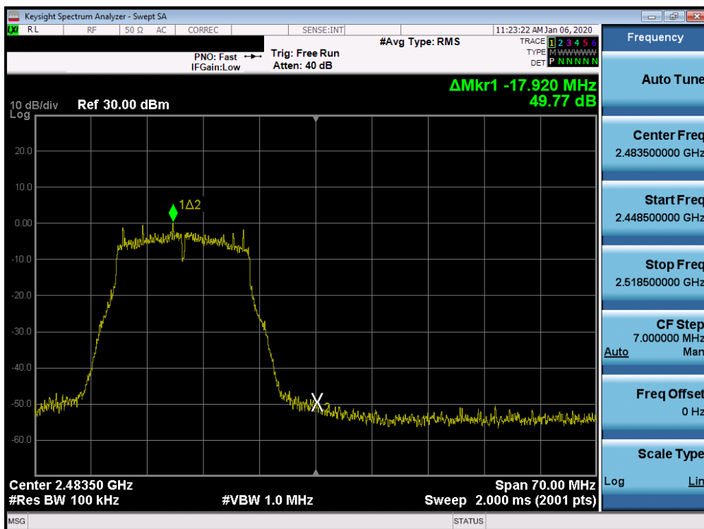
Plot 7-76. Band Edge Plot SISO CORE1 (802.11g - Ch. 12)
