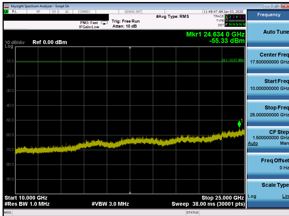
Plot 7-86. Conducted Spurious Plot SISO CORE0 (802.11b – Ch. 1)
