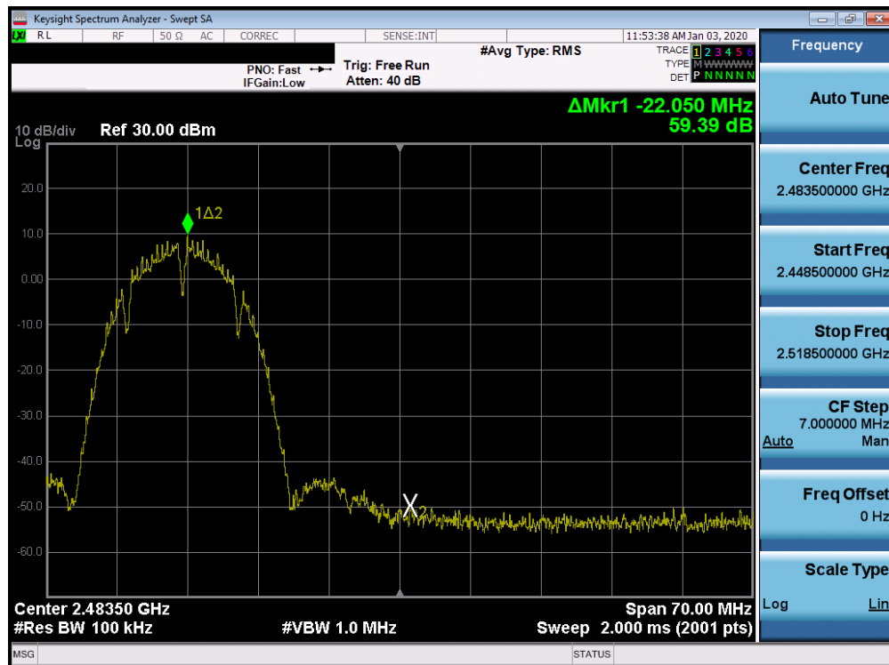
Plot 7-68. Band Edge Plot SISO CORE1 (802.11b – Ch. 11)
