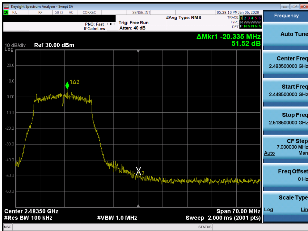
Plot 7-75. Band Edge Plot SISO CORE1 (802.11g - Ch. 11)
