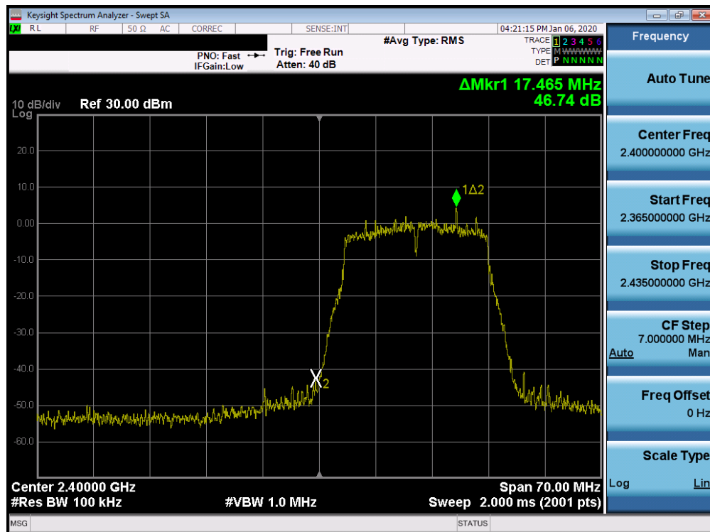
Plot 7-60. Band Edge Plot SISO CORE0 (802.11n (2.4GHz) – Ch. 1)
