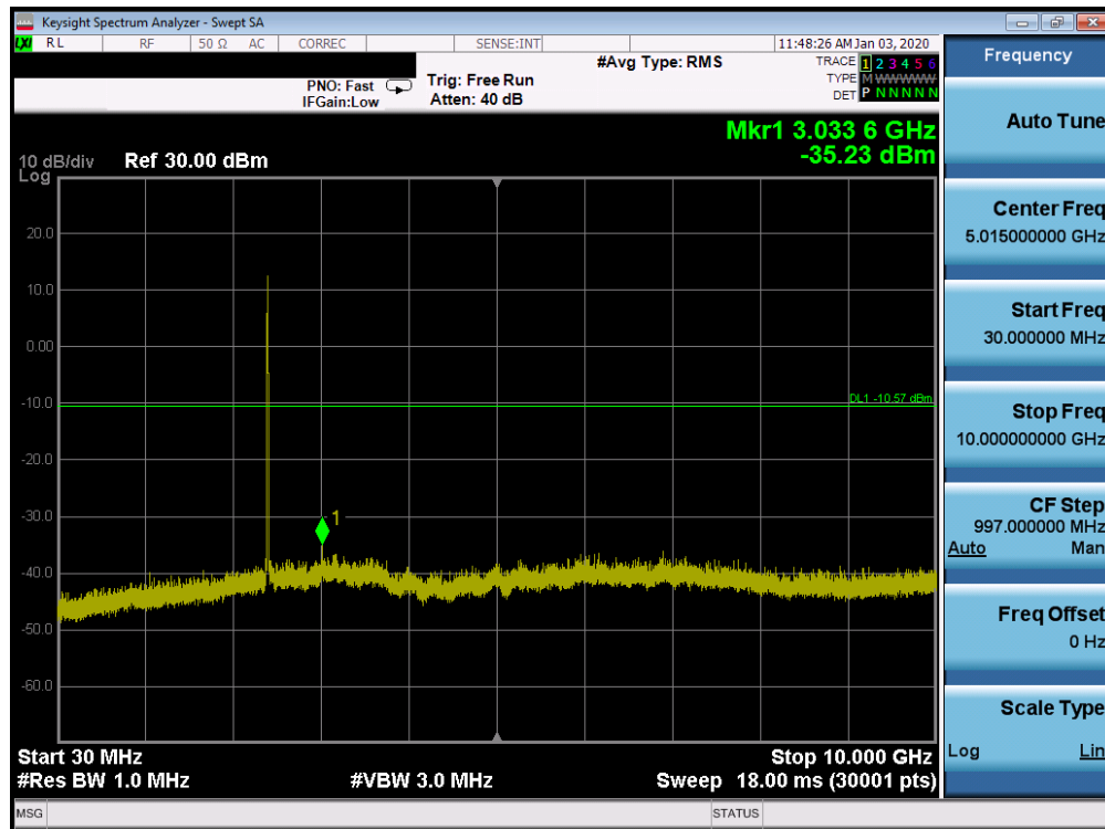
Plot 7-85. Conducted Spurious Plot SISO CORE0 (802.11b – Ch. 1)
