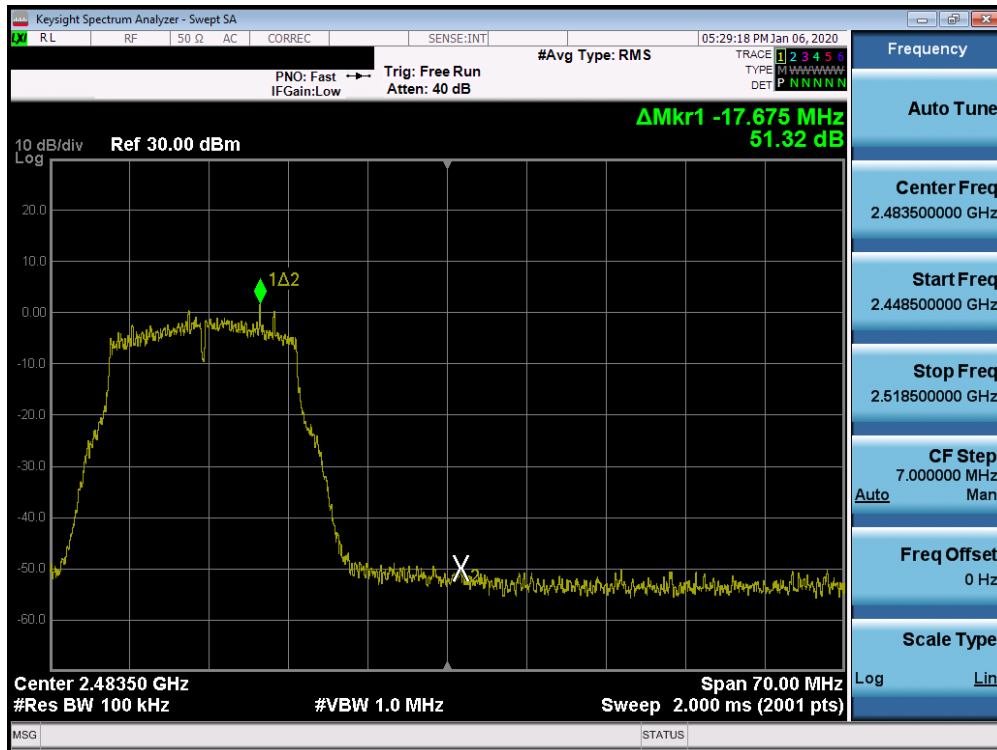
Plot 7-57. Band Edge Plot SISO CORE0 (802.11g – Ch. 11)
