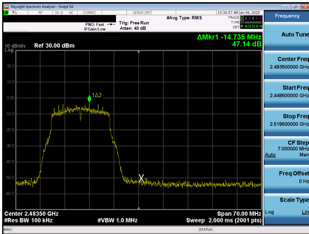
Plot 7-58. Band Edge Plot SISO CORE0 (802.11g – Ch. 12)
