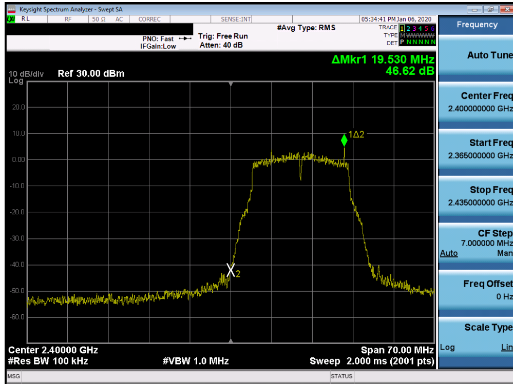
Plot 7-71. Band Edge Plot SISO CORE1 (802.11g- Ch. 1)
