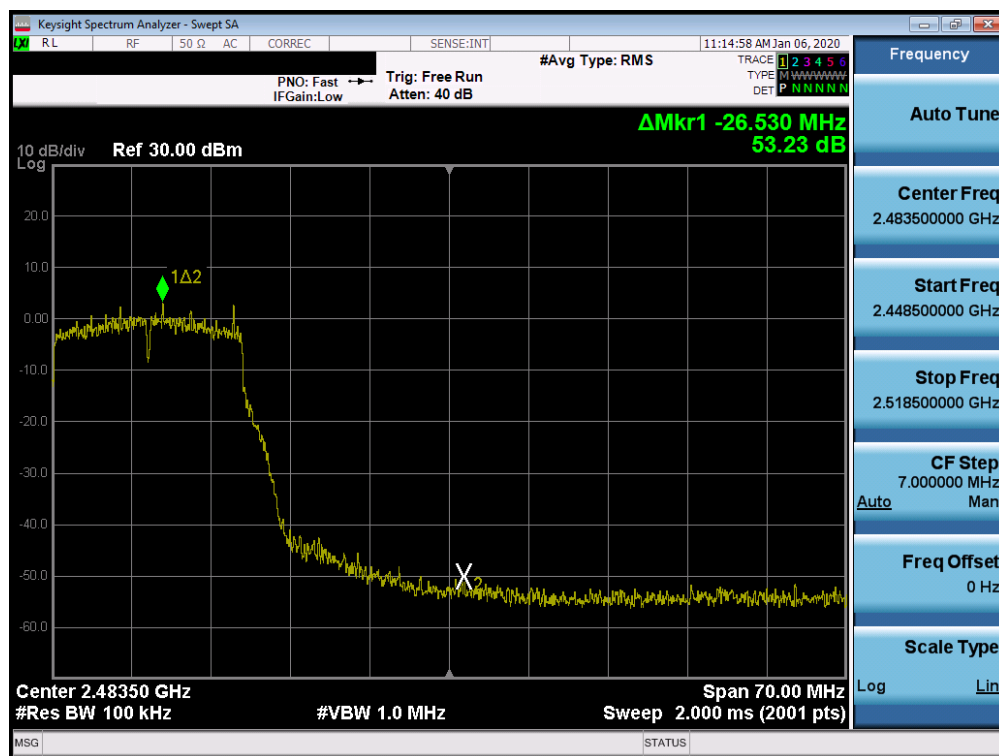
Plot 7-74. Band Edge Plot SISO CORE1 (802.11g – Ch. 10)
