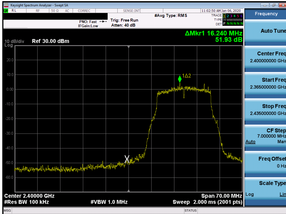
Plot 7-72. Band Edge Plot SISO CORE1 (802.11g- Ch. 2)
