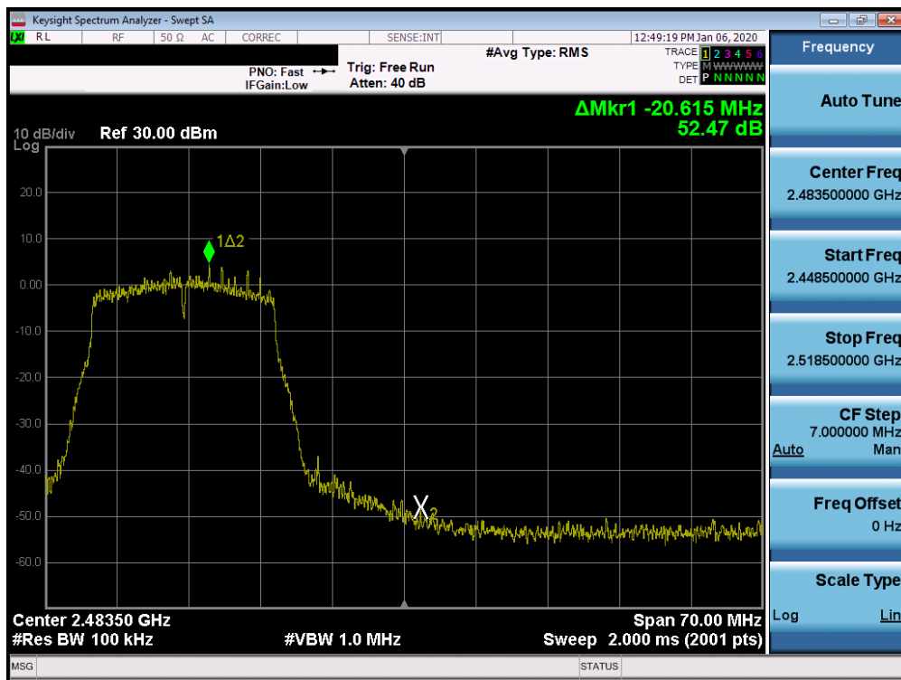
Plot 7-82. Band Edge Plot SISO CORE1 (802.11n (2.4GHz) – Ch. 11)
