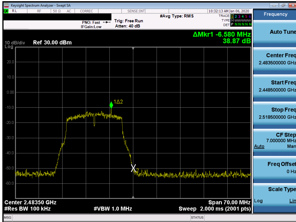
Plot 7-59. Band Edge Plot SISO CORE0 (802.11g – Ch. 13)
