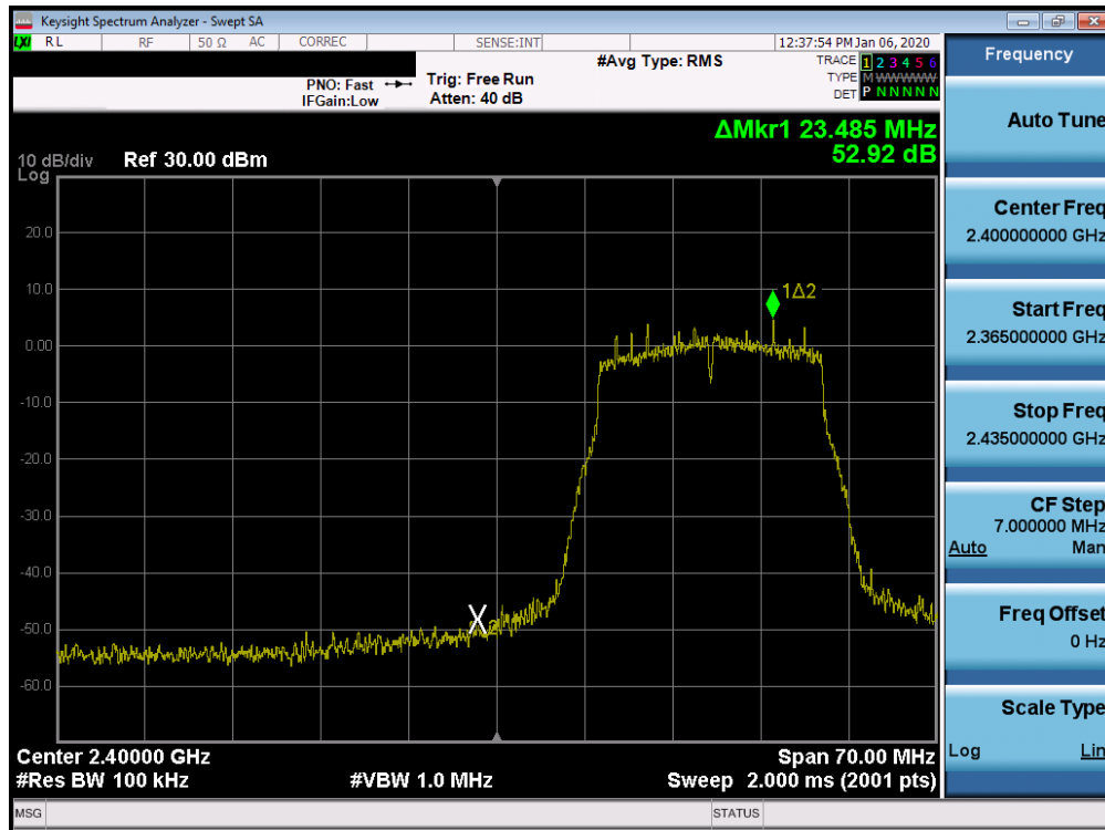
Plot 7-79. Band Edge Plot SISO CORE1 (802.11n (2.4GHz) – Ch. 2)
