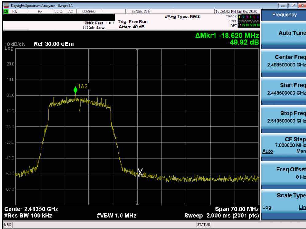
Plot 7-83. Band Edge Plot SISO CORE1 (802.11n – Ch. 12)
