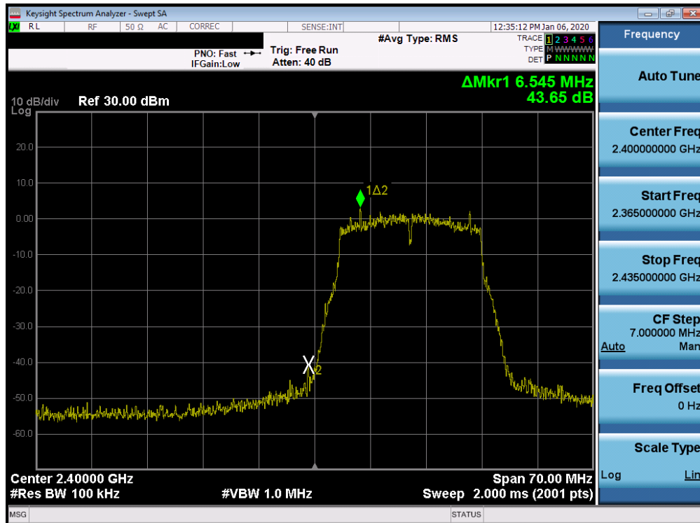
Plot 7-78. Band Edge Plot SISO CORE1 (802.11n (2.4GHz) – Ch. 1)
