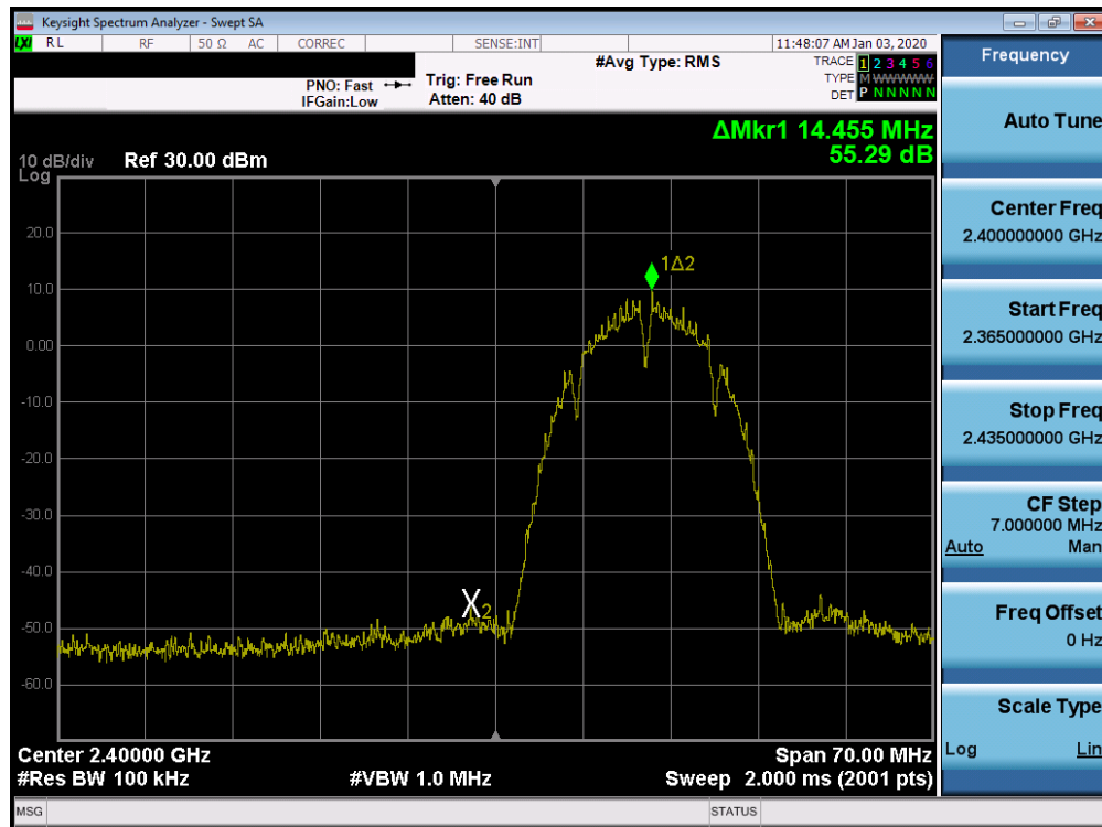
Plot 7-67. Band Edge Plot SISO CORE1 (802.11b – Ch. 1)
