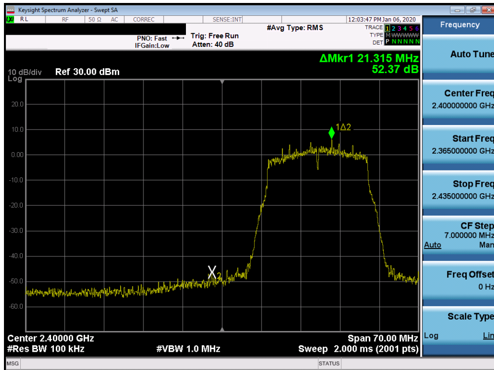
Plot 7-61. Band Edge Plot SISO CORE0 (802.11n (2.4GHz) – Ch. 2)
