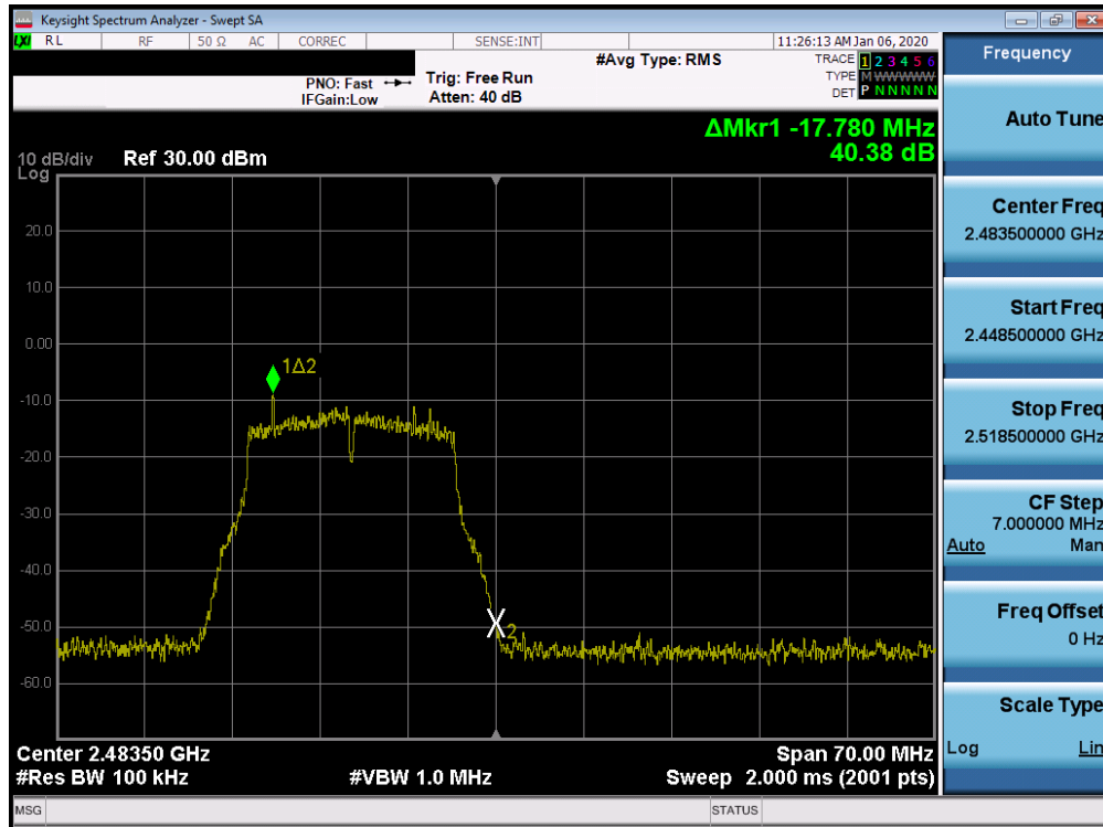
Plot 7-77. Band Edge Plot SISO CORE1 (802.11g – Ch. 13)
