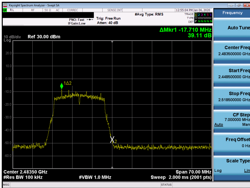
Plot 7-84. Band Edge Plot SISO CORE1 (802.11n – Ch. 13)
