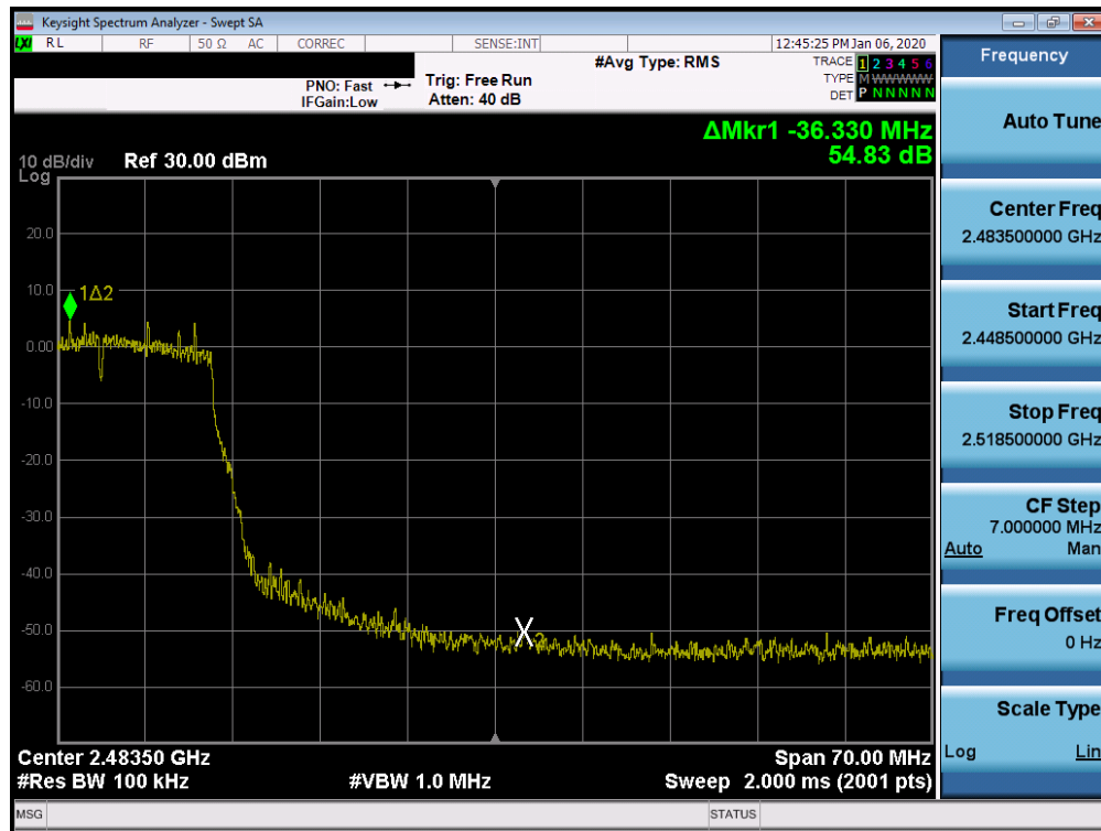
Plot 7-80. Band Edge Plot SISO CORE1 (802.11n (2.4GHz) – Ch. 9)
