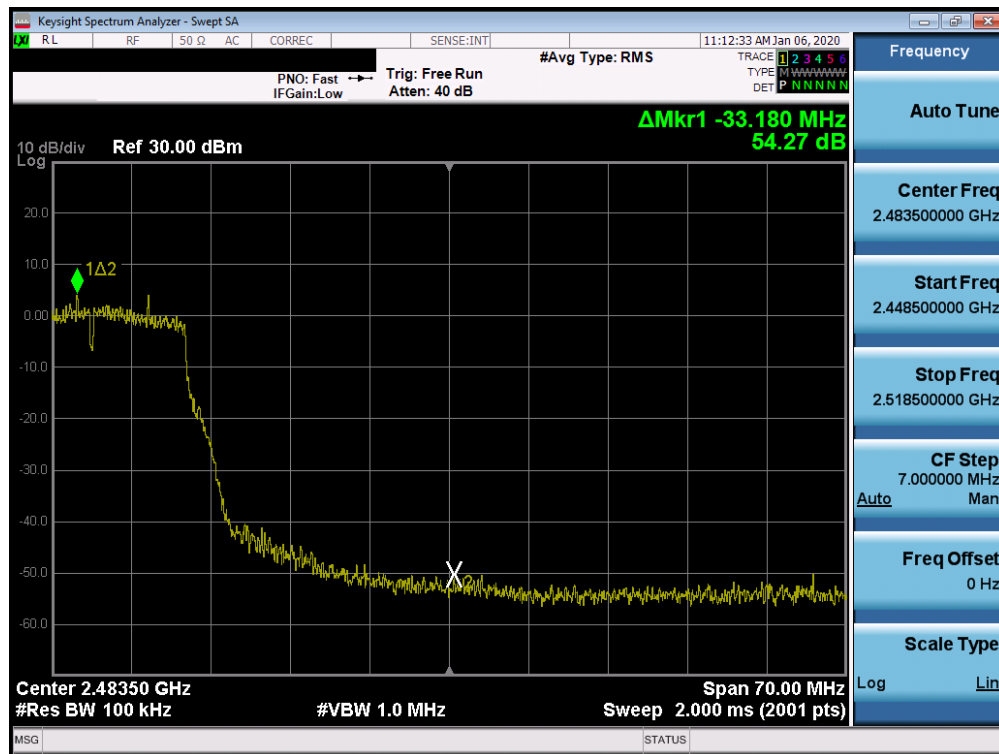
Plot 7-73. Band Edge Plot SISO CORE1 (802.11g – Ch. 9)
