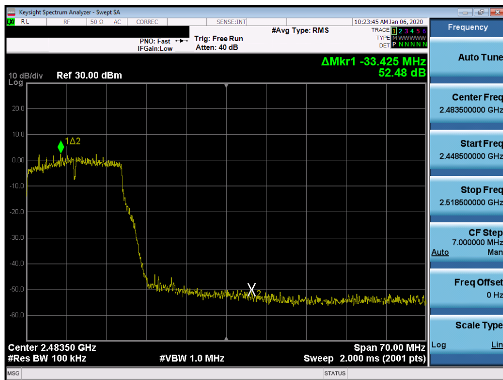
Plot 7-56. Band Edge Plot SISO CORE0 (802.11g – Ch. 10)
