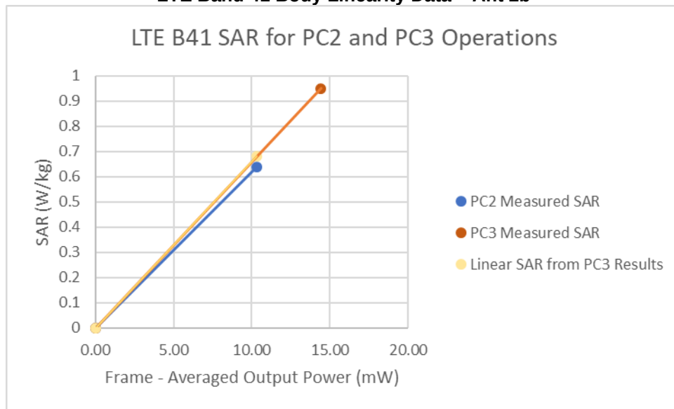
Figure 13-7 LTE Band 41 Body Linearity Data – Ant 2b
