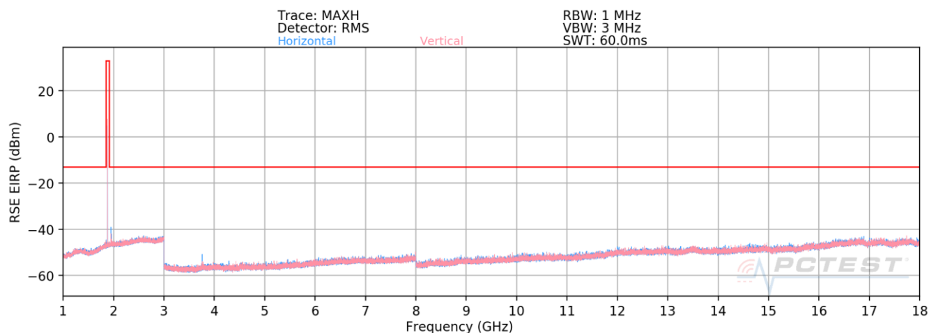
Plot 7-80. Radiated Spurious Plot Above 1GHz (PCS GPRS Mode)
