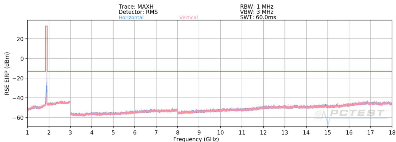
Plot 7-81. Radiated Spurious Plot Above 1GHz (PCS WCDMA Mode)
