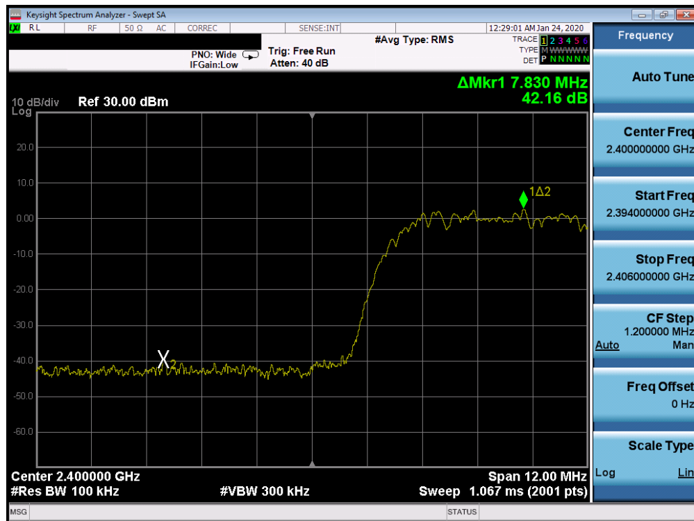
Plot 7-67. Band Edge Plot Ant 2a (Bluetooth (HDR8), ePA – Ch. 1)
