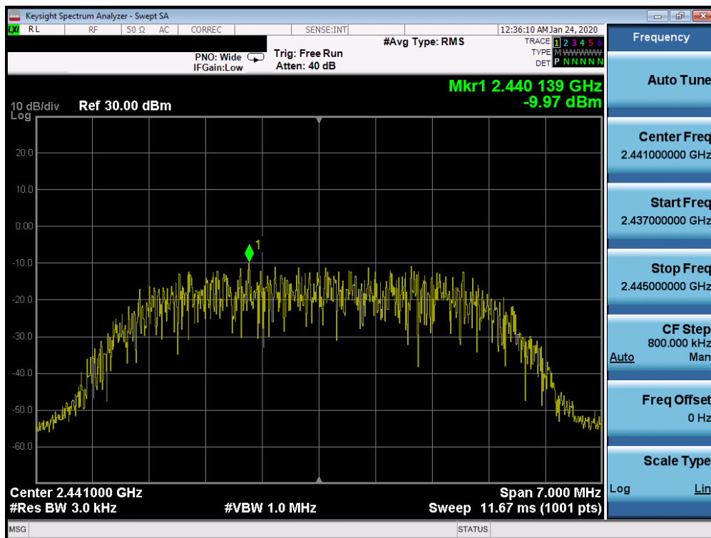
Plot 7-32. Power Spectral Density Plot Ant 2a (Bluetooth (HDR8), 8Mbps, ePA – Ch. 38)
