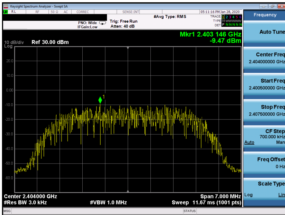
Plot 7-56. Power Spectral Density Plot Tx BF Ant 2a (Bluetooth (HDR8), 8Mbps, iPA – Ch. 1)
