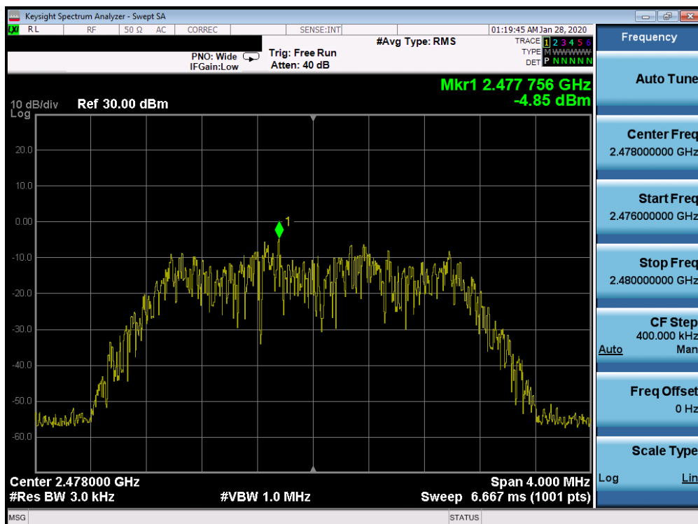
Plot 7-18. Power Spectral Density Plot Ant 4a (Bluetooth (HDR4), 4Mbps, iPA – Ch. 75)
