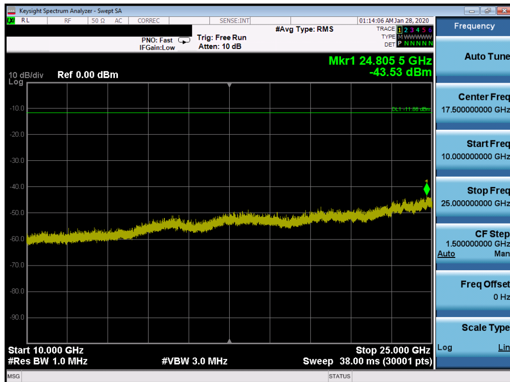
Plot 7-74. Conducted Spurious Plot Ant 4a (Bluetooth (HDR4), 4Mbps, ePA – Ch. 75)
