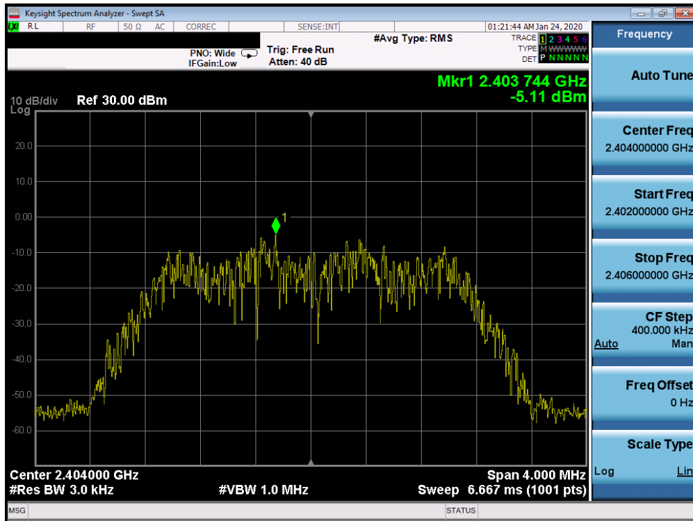
Plot 7-19. Power Spectral Density Plot Ant 4a (Bluetooth (HDR8), 8Mbps, ePA – Ch. 1)
