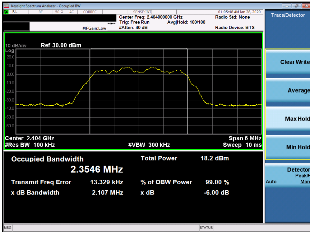
Plot 7-1. 6dB Bandwidth Plot Ant 4a (Bluetooth (HDR4), 4Mbps, ePA – Ch. 1)
