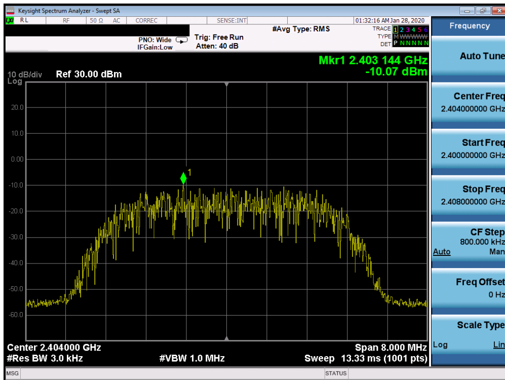
Plot 7-34. Power Spectral Density Plot Ant 2a (Bluetooth (HDR8), 8Mbps, iPA – Ch. 1)
