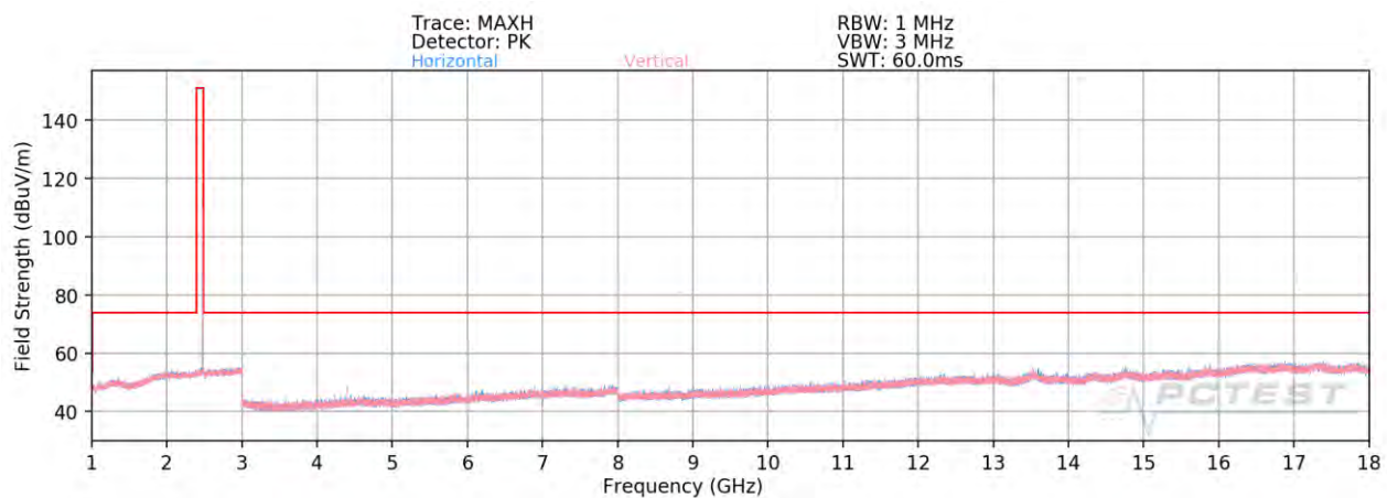
Plot 7-83. Radiated Spurious Plot Above 1GHz Ant 4a (4Mbps, HDR4 ePA – Ch. 75, Ant. Pol. H & V)
