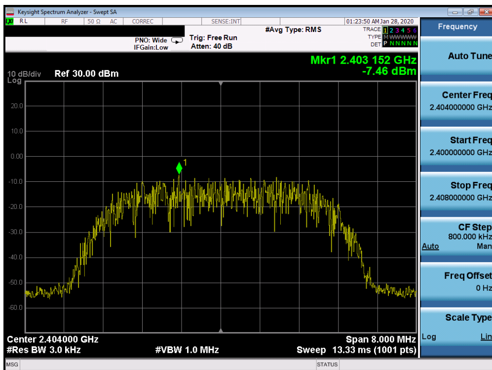
Plot 7-22. Power Spectral Density Plot Ant 4a (Bluetooth (HDR8), 8Mbps, iPA – Ch. 1)
