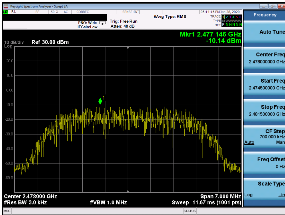
Plot 7-54. Power Spectral Density Plot Tx BF Ant 2a (Bluetooth (HDR8), 8Mbps, ePA – Ch. 75)
