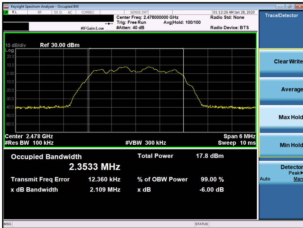
Plot 7-3. 6dB Bandwidth Plot Ant 4a (Bluetooth (HDR4), 4Mbps, ePA – Ch. 75)
