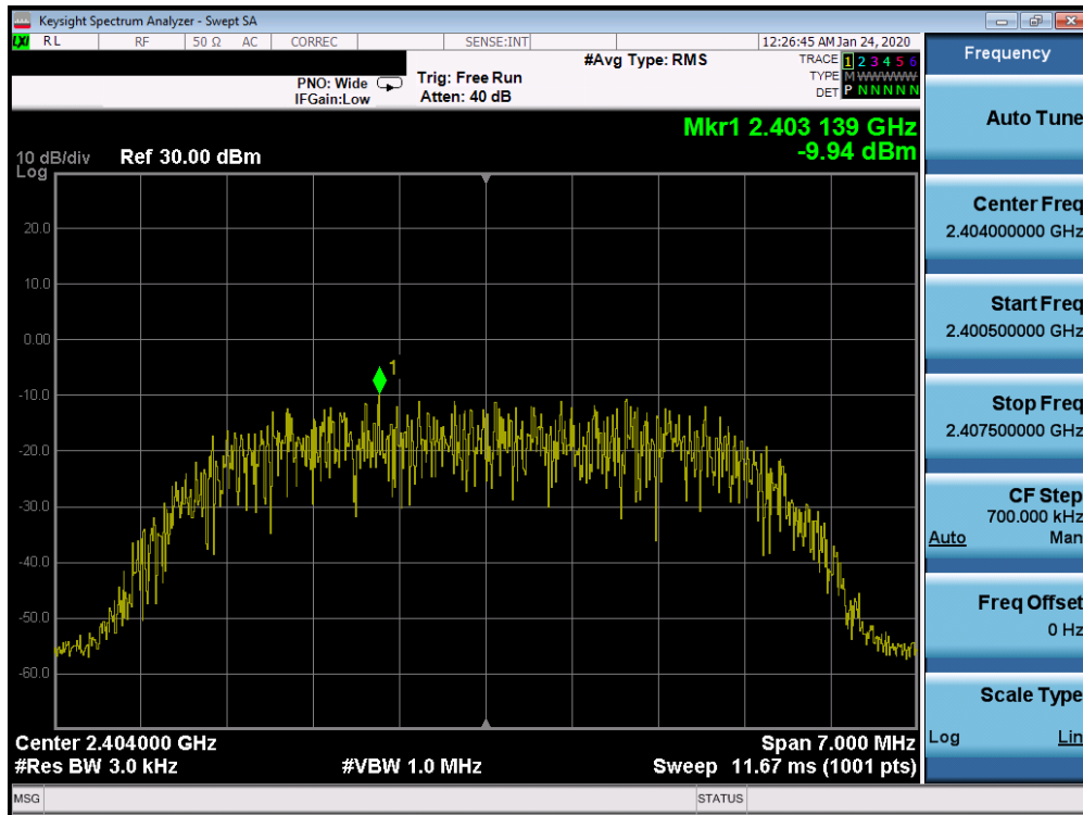
Plot 7-31. Power Spectral Density Plot Ant 2a (Bluetooth (HDR8), 8Mbps, ePA – Ch. 1)
