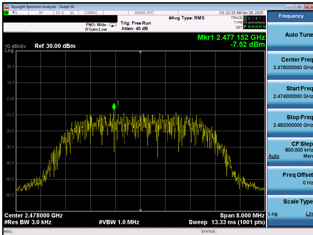
Plot 7-24. Power Spectral Density Plot Ant 4a (Bluetooth (HDR8), 8Mbps, iPA – Ch. 75)
