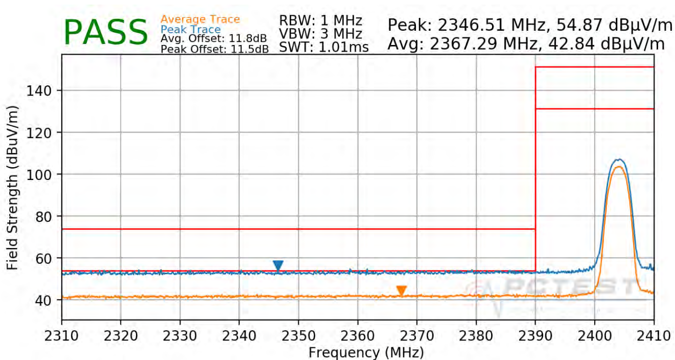
Plot 7-96. Radiated Restricted Lower Band Edge Measurement Ant 2a (Average & Peak)
