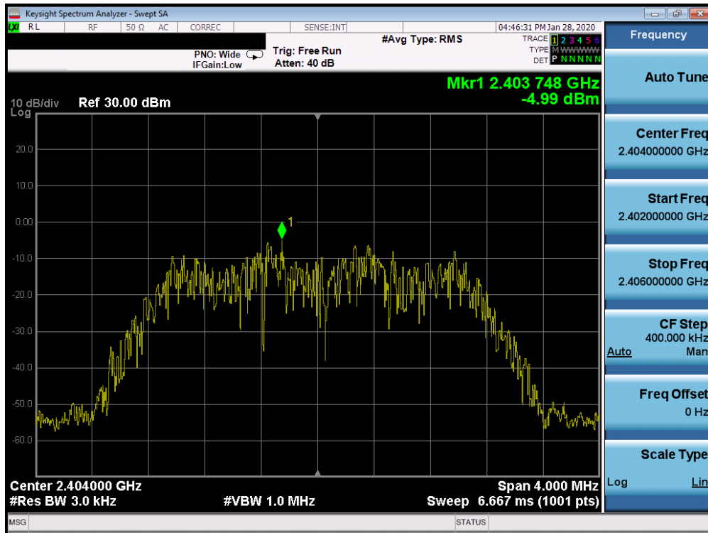
Plot 7-37. Power Spectral Density Plot TxBF Ant 4a (Bluetooth (HDR4), 4Mbps, ePA – Ch. 1)
