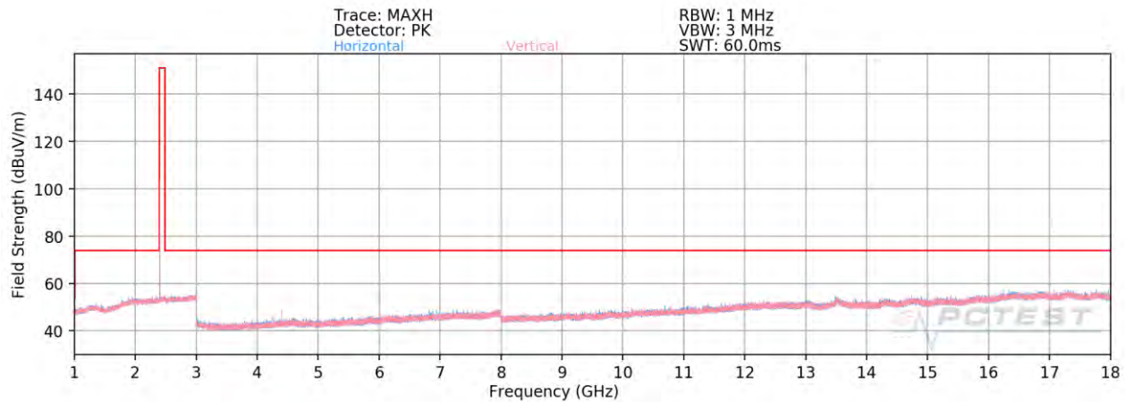
Plot 7-87. Radiated Spurious Plot Above 1GHz TXBF (4Mbps, HDR4 ePA – Ch. 1, Ant. Pol. H & V)
