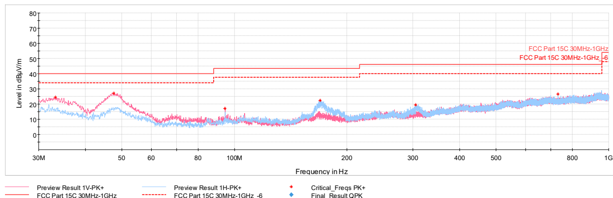
Plot 7-104. Radiated Spurious Plot below 1GHz (4Mbps, ePA – Ch.38 with AC/DC Adapter)
