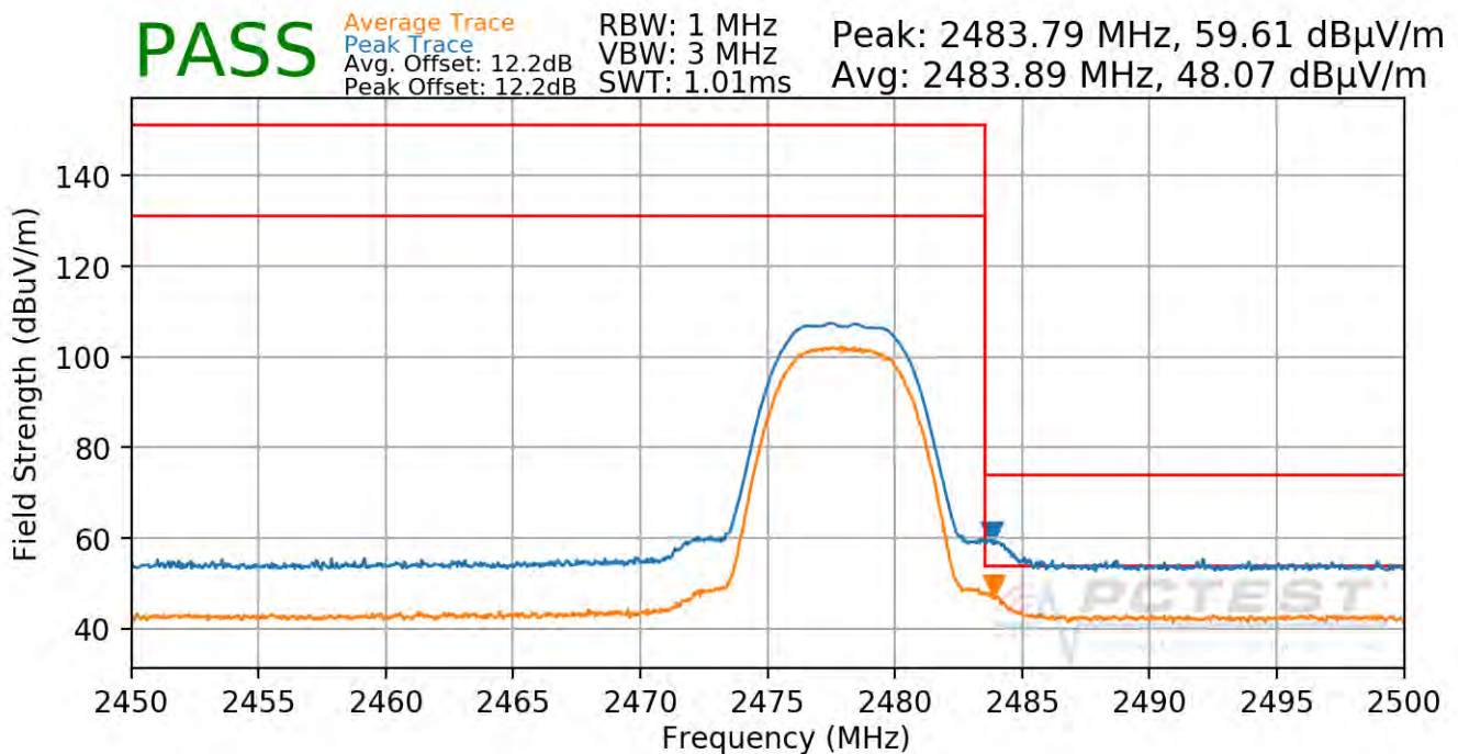
Plot 7-95. Radiated Restricted Upper Band Edge Measurement Ant 4a (Average & Peak)
