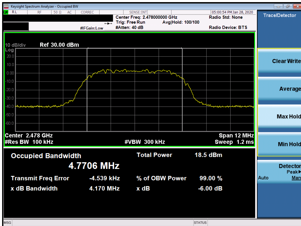
Plot 7-6. 6dB Bandwidth Plot Ant 4a (Bluetooth (HDR8), 8Mbps, ePA – Ch. 75)
