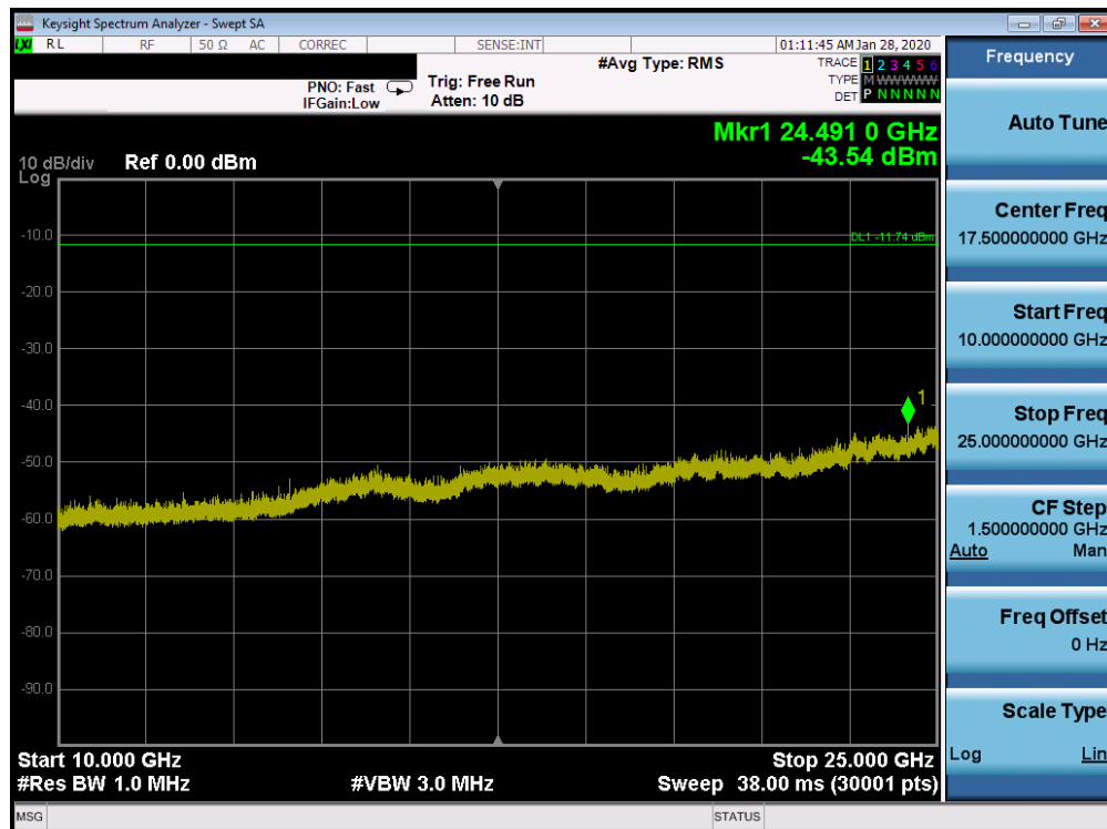
Plot 7-72. Conducted Spurious Plot Ant 4a (Bluetooth (HDR4), 4Mbps, ePA – Ch. 38)
