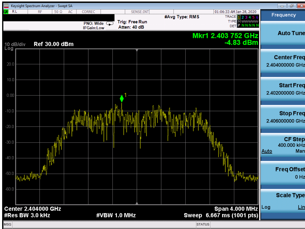
Plot 7-13. Power Spectral Density Plot Ant 4a (Bluetooth (HDR4), 4Mbps, ePA – Ch. 1)
