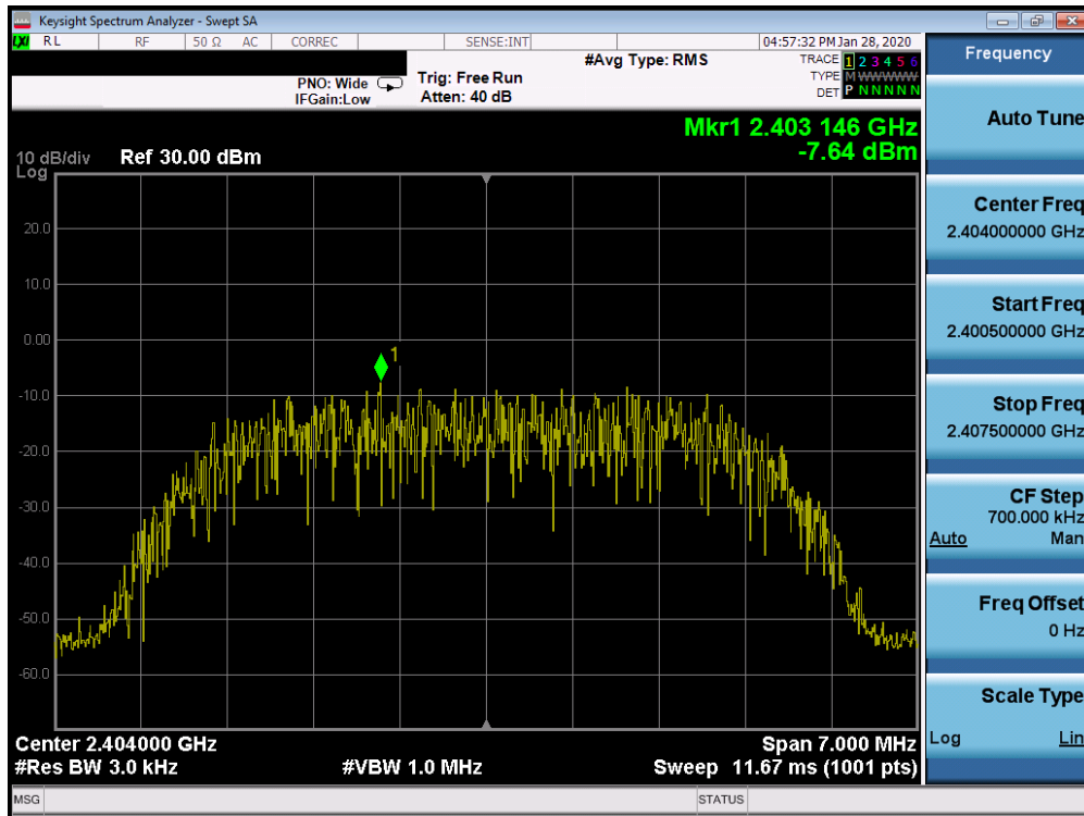
Plot 7-49. Power Spectral Density Plot TxBF Ant 4a (Bluetooth (HDR8), 8Mbps, ePA – Ch. 1)
