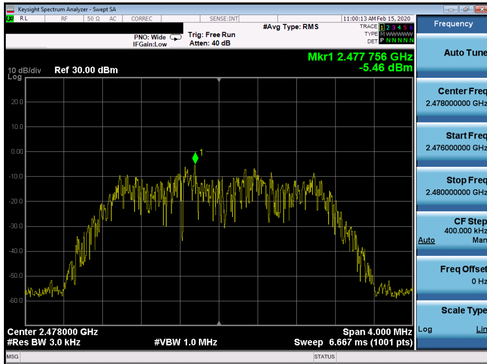
Plot 7-41. Power Spectral Density Plot TxBF Ant 4a (Bluetooth (HDR4), 4Mbps, ePA – Ch. 75)
