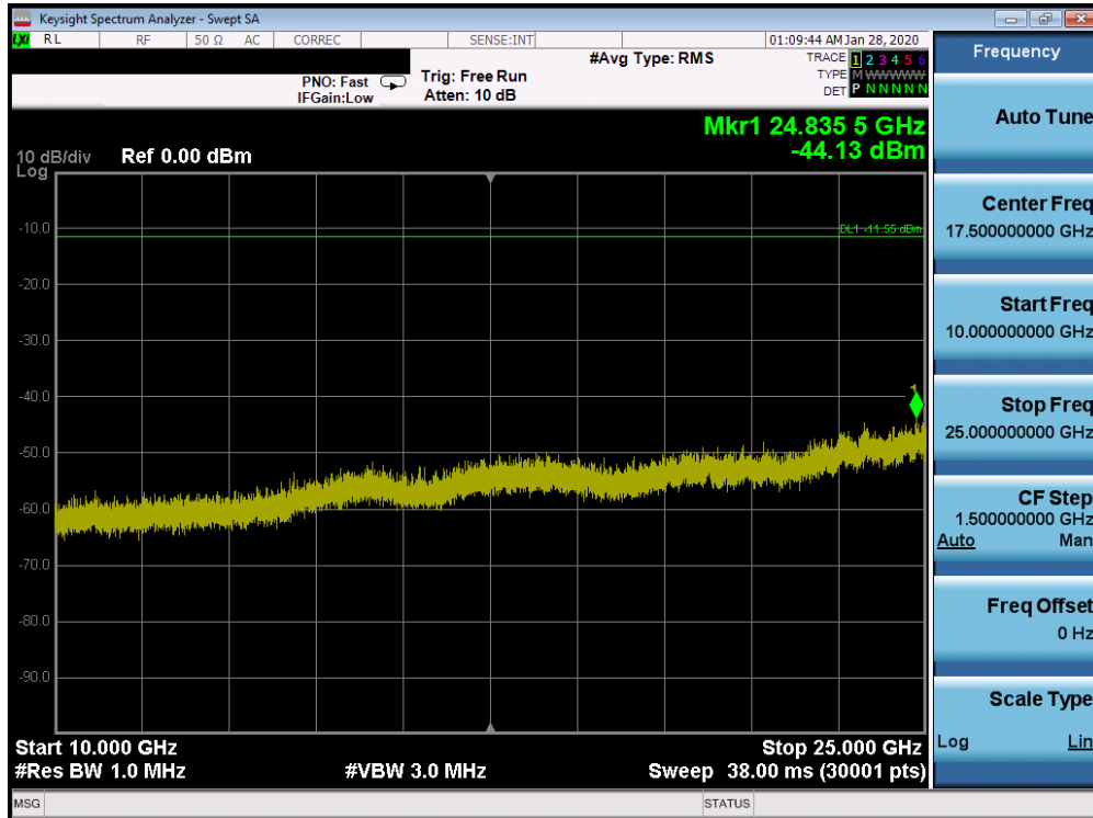
Plot 7-70. Conducted Spurious Plot Ant 4a (Bluetooth (HDR4), 4Mbps, ePA – Ch. 1)
