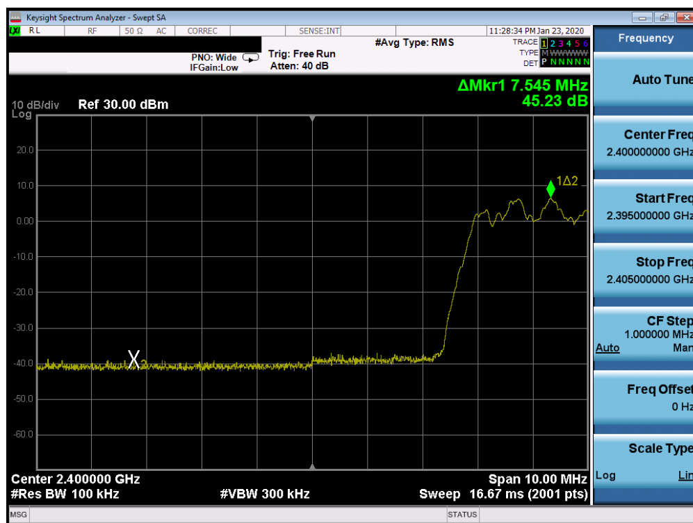
Plot 7-65. Band Edge Plot Ant 2a (Bluetooth (HDR4), ePA – Ch. 1)
