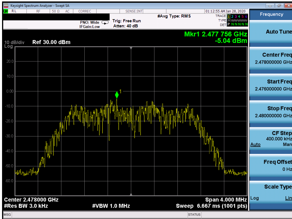
Plot 7-15. Power Spectral Density Plot Ant 4a (Bluetooth (HDR4), 4Mbps, ePA – Ch. 75)
