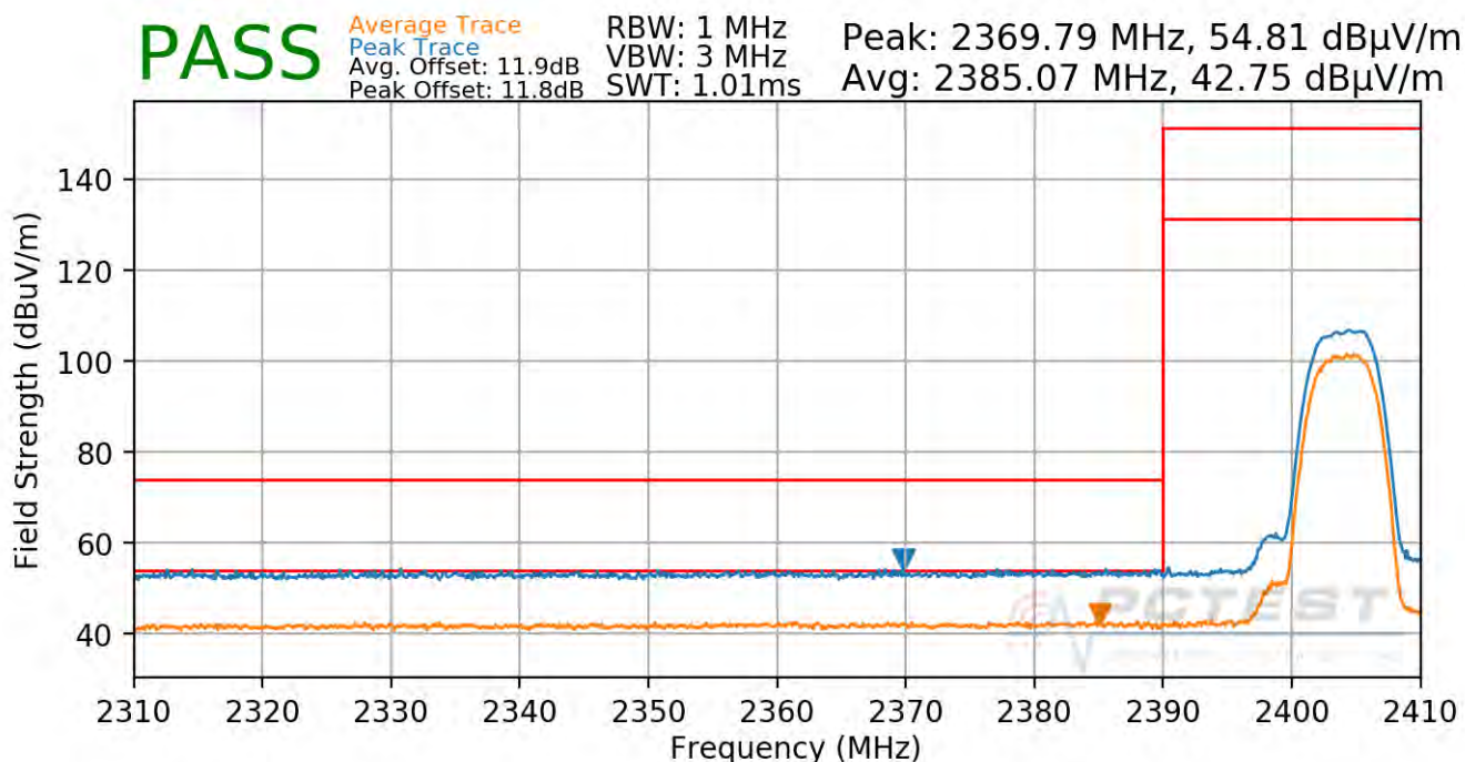
Plot 7-97. Radiated Restricted Lower Band Edge Measurement Ant 2a (Average & Peak)
