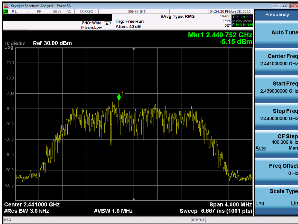
Plot 7-45. Power Spectral Density Plot TxBF Ant 4a (Bluetooth (HDR4), 4Mbps, iPA – Ch. 38)
