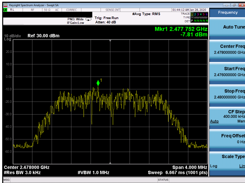
Plot 7-48. Power Spectral Density Plot TxBF Ant 2a (Bluetooth (HDR4), 4Mbps, iPA – Ch. 75)
