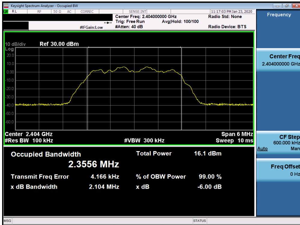
Plot 7-7. 6dB Bandwidth Plot Ant 2a (Bluetooth (HDR4), 4Mbps, ePA – Ch. 1)
