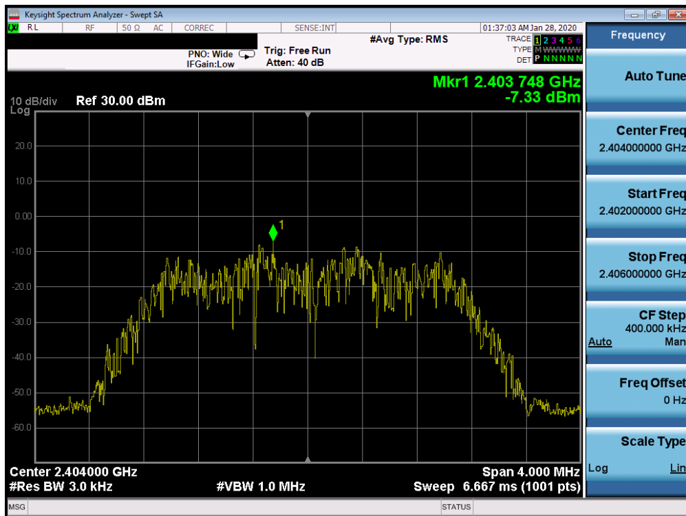
Plot 7-44. Power Spectral Density Plot Tx BF Ant 2a (Bluetooth (HDR4), 4Mbps, iPA – Ch. 1)
