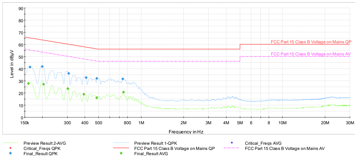
Plot 7-106. Line Conducted Plot with Bluetooth HDR (N, 4Mbps ePA – Ch.38 with AC/DC Adapter)
