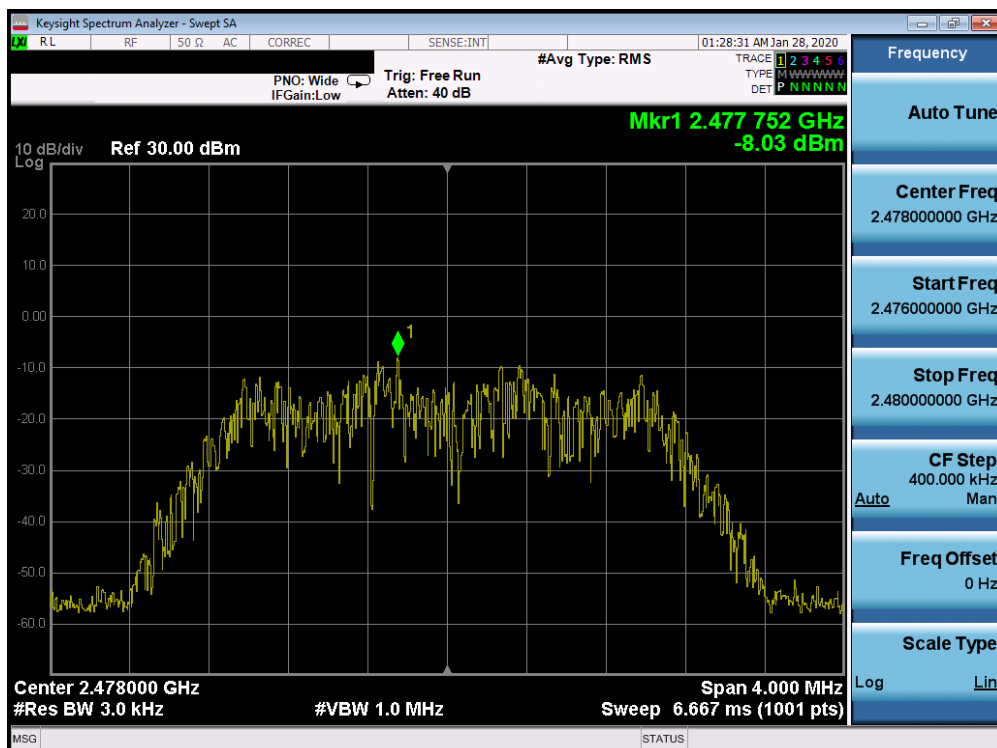
Plot 7-30. Power Spectral Density Plot Ant 2a (Bluetooth (HDR4), 4Mbps, iPA – Ch. 75)
