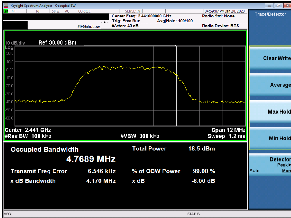
Plot 7-5. 6dB Bandwidth Plot Ant 4a (Bluetooth (HDR8), 8Mbps, ePA – Ch. 38)
