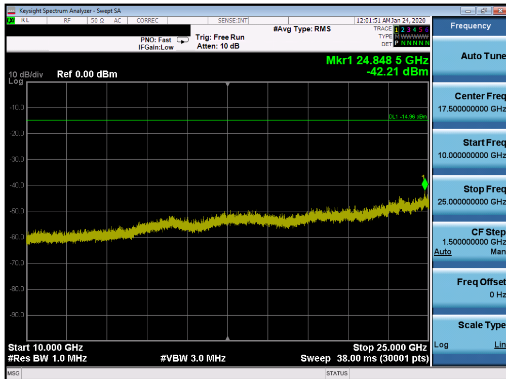
Plot 7-80. Conducted Spurious Plot Ant 2a (Bluetooth (HDR4), 4Mbps, ePA – Ch. 75)
