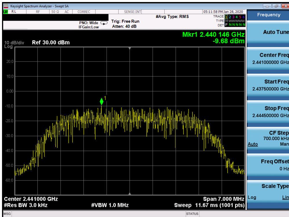
Plot 7-58. Power Spectral Density Plot TxBF Ant 2a (Bluetooth (HDR8), 8Mbps, iPA – Ch. 38)
