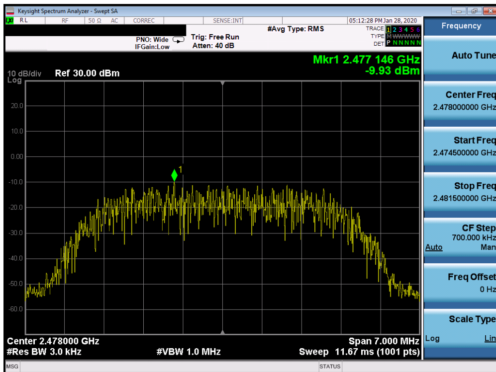
Plot 7-60. Power Spectral Density Plot TxBF Ant 2a (Bluetooth (HDR8), 8Mbps, iPA – Ch. 75)
