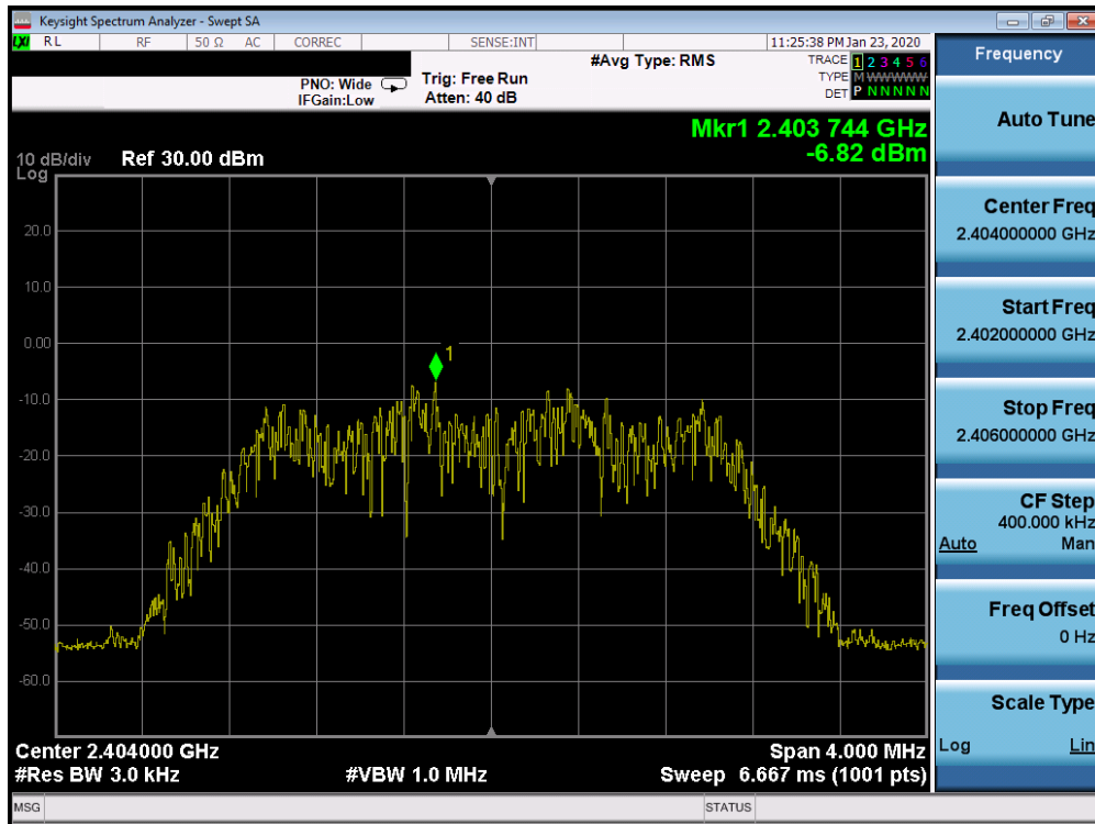
Plot 7-25. Power Spectral Density Plot Ant 2a (Bluetooth (HDR4), 4Mbps, ePA – Ch. 1)
