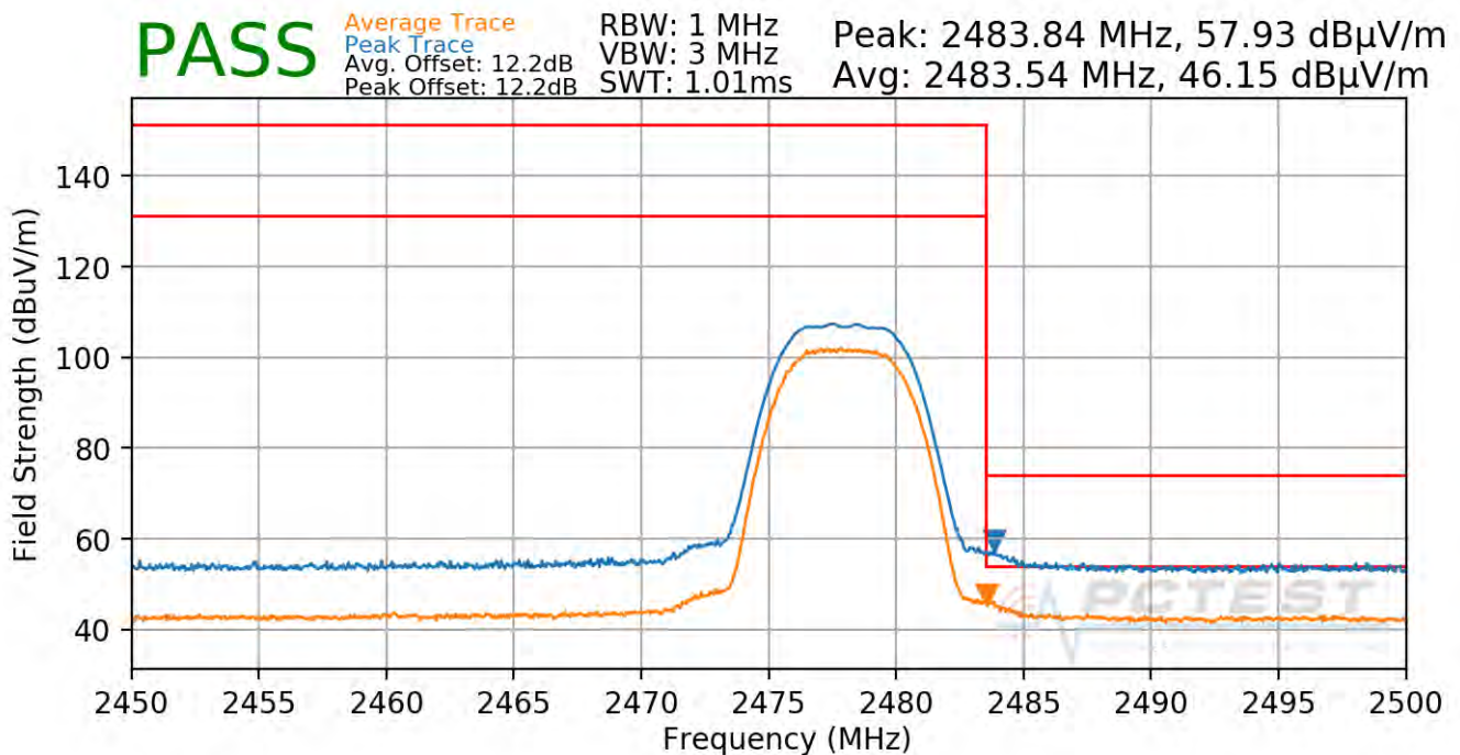
Plot 7-99. Radiated Restricted Upper Band Edge Measurement Ant 2a (Average & Peak)
