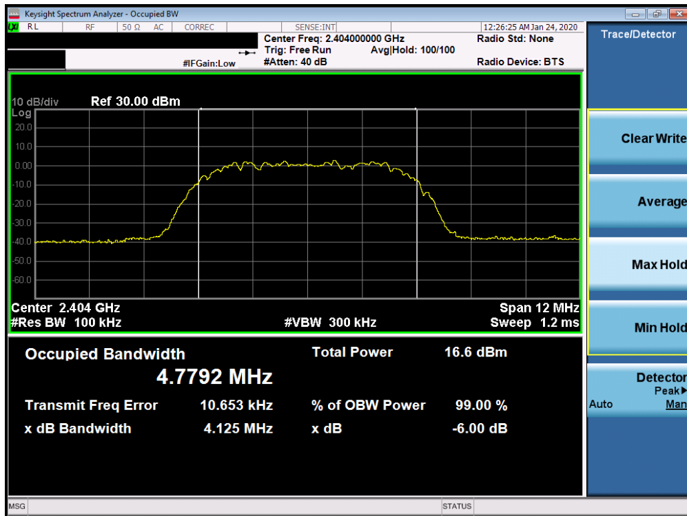
Plot 7-10. 6dB Bandwidth Plot Ant 2a (Bluetooth (HDR8), 8Mbps, ePA – Ch. 1)
