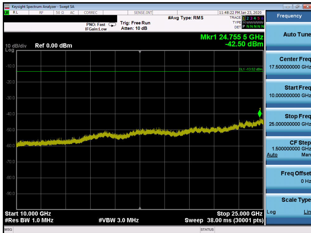
Plot 7-78. Conducted Spurious Plot Ant 2a (Bluetooth (HDR4), 4Mbps, ePA – Ch. 38)
