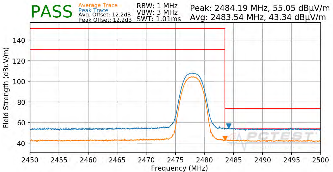
Plot 7-94. Radiated Restricted Upper Band Edge Measurement Ant 4a (Average & Peak)
