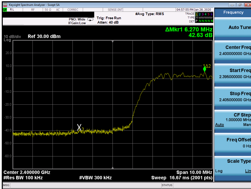
Plot 7-63. Band Edge Plot Ant 4a (Bluetooth (HDR8), ePA - Ch. 1)
