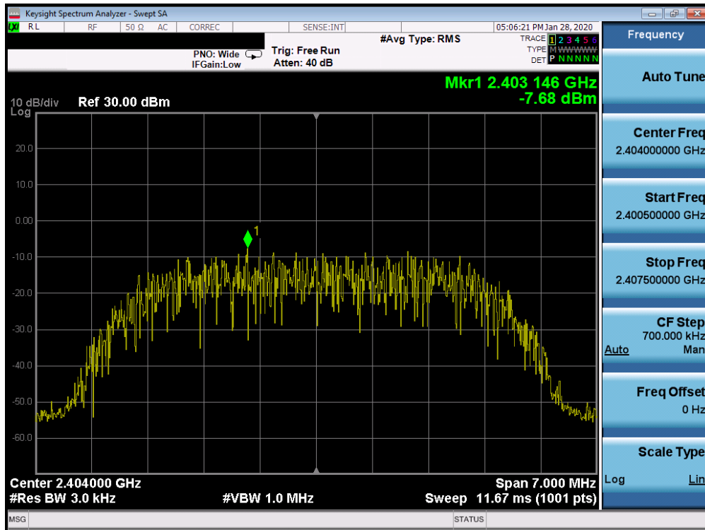
Plot 7-55. Power Spectral Density Plot Tx BF Ant 4a (Bluetooth (HDR8), 8Mbps, iPA – Ch. 1)
