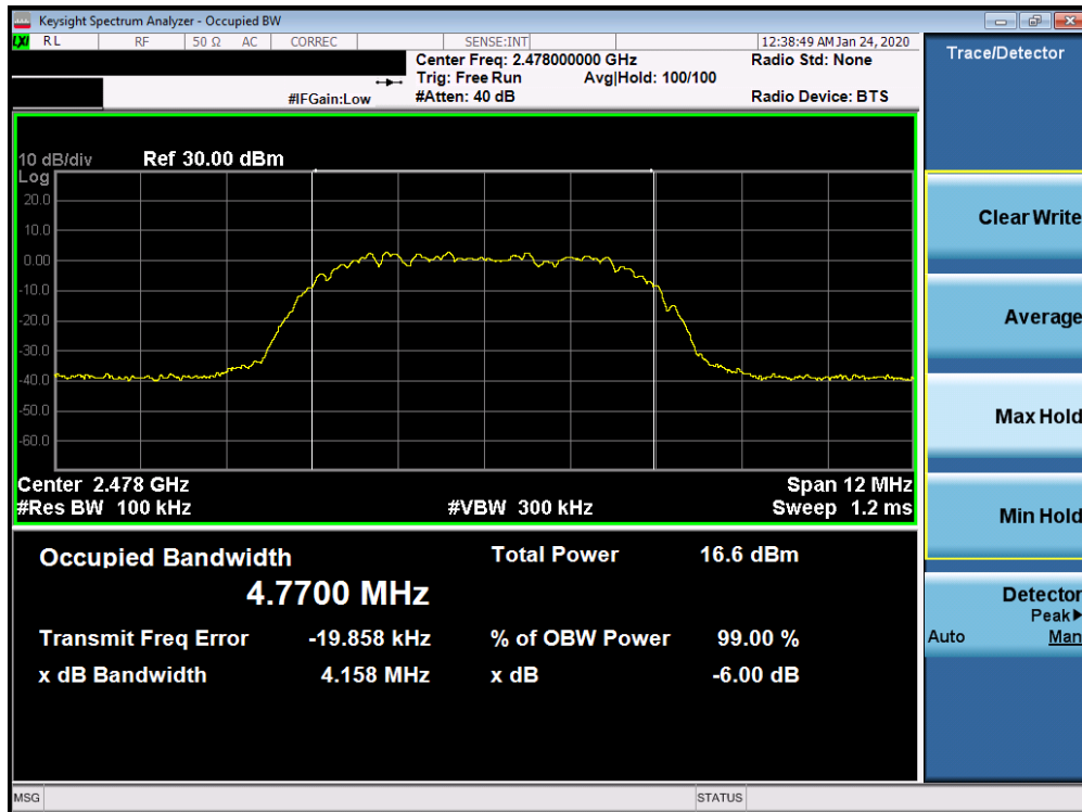
Plot 7-12. 6dB Bandwidth Plot Ant 2a (Bluetooth (HDR8), 8Mbps, ePA – Ch. 75)
