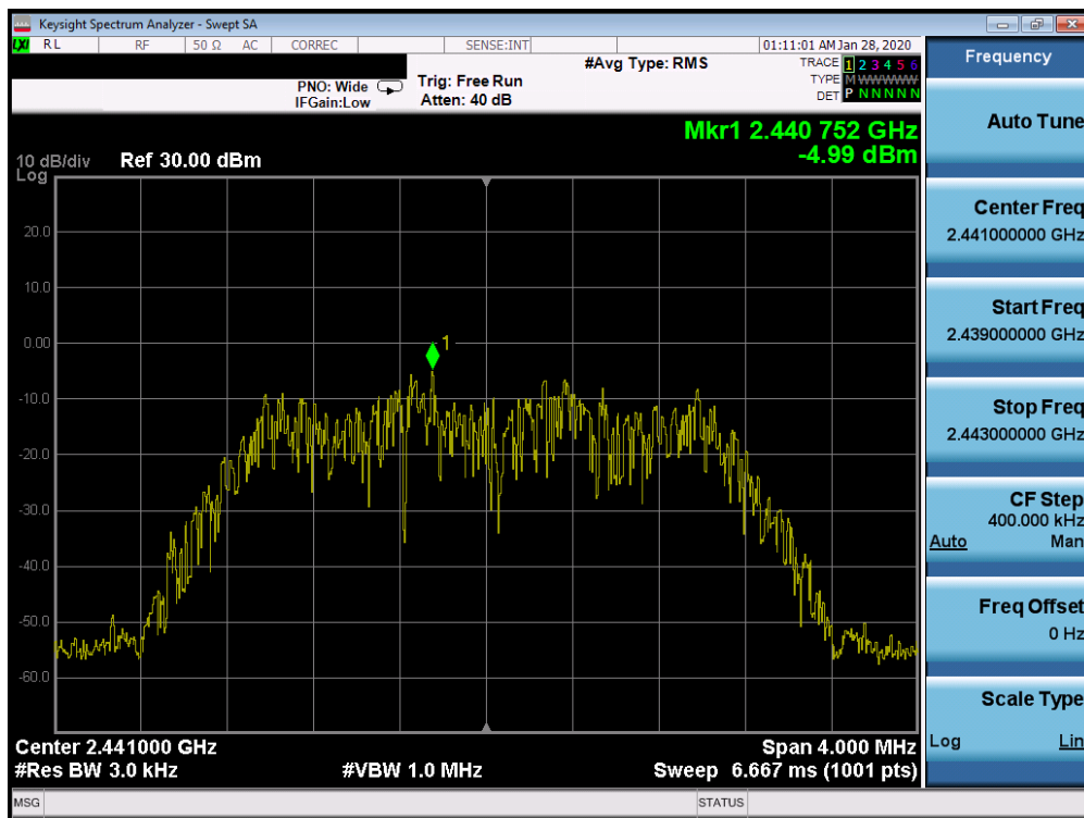
Plot 7-14. Power Spectral Density Plot Ant 4a (Bluetooth (HDR4), 4Mbps, ePA – Ch. 38)
