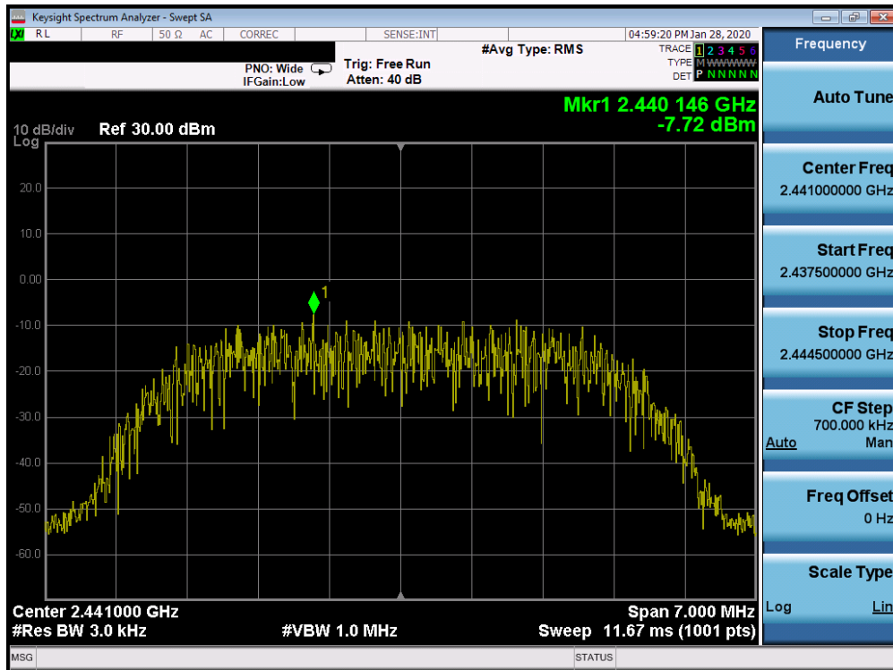
Plot 7-51. Power Spectral Density Plot TxBF Ant 4a (Bluetooth (HDR8), 8Mbps, ePA – Ch. 38)
