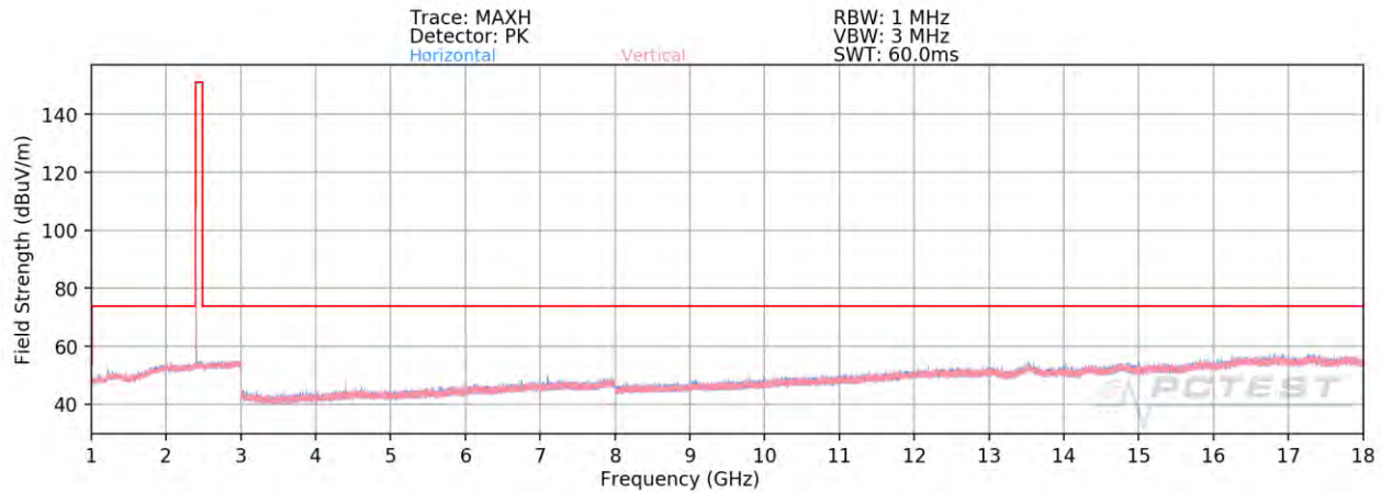
Plot 7-81. Radiated Spurious Plot Above 1GHz Ant 4a (4Mbps, HDR4 ePA – Ch. 1, Ant. Pol. H & V)
