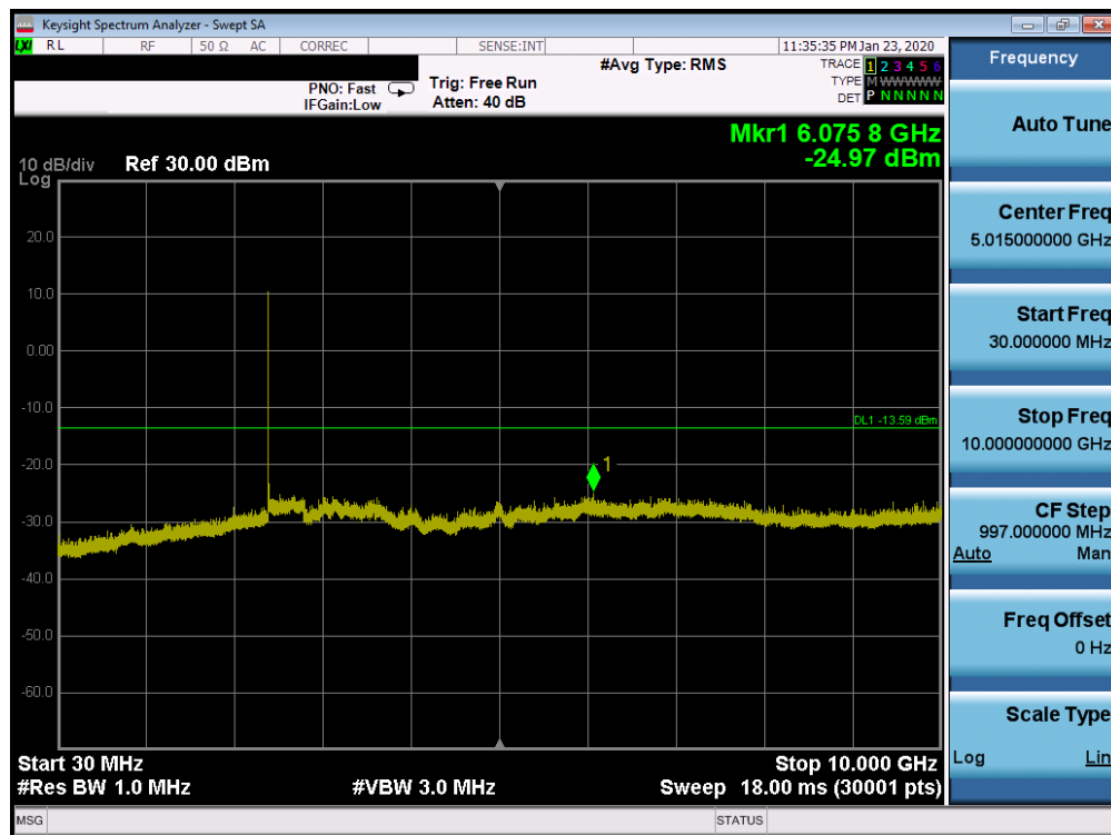
Plot 7-75. Conducted Spurious Plot Ant 2a (Bluetooth (HDR4), 4Mbps, ePA – Ch. 1)
