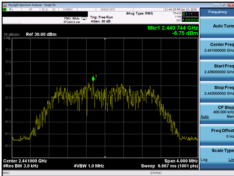
Plot 7-26. Power Spectral Density Plot Ant 2a (Bluetooth (HDR4), 4Mbps, ePA – Ch. 38)
