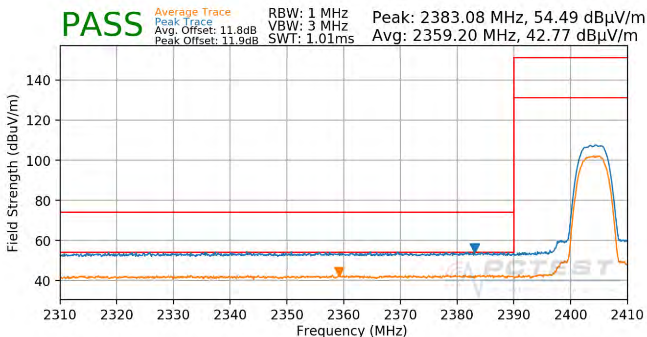
Plot 7-93. Radiated Restricted Lower Band Edge Measurement Ant 4a (Average & Peak)
