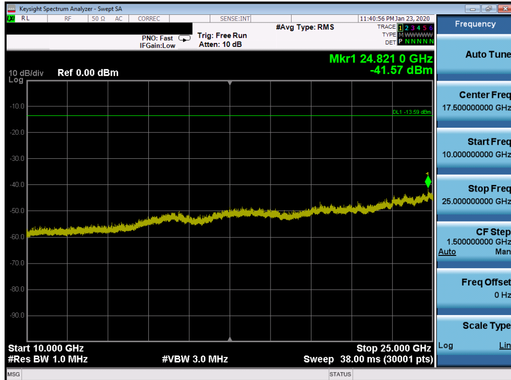
Plot 7-76. Conducted Spurious Plot Ant 2a (Bluetooth (HDR4), 4Mbps, ePA – Ch. 1)
