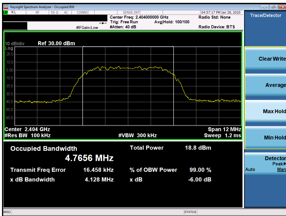
Plot 7-4. 6dB Bandwidth Plot Ant 4a (Bluetooth (HDR8), 8Mbps, ePA – Ch. 1)
