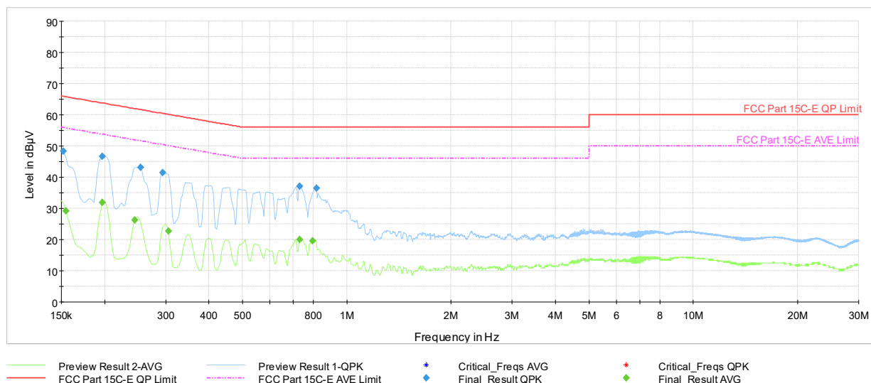
Plot 7-105. Line Conducted Plot with Bluetooth HDR (L1, 4Mbps ePA – Ch.38 with AC/DC Adapter)
