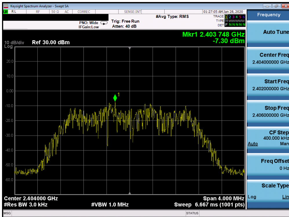
Plot 7-28. Power Spectral Density Plot Ant 2a (Bluetooth (HDR4), 4Mbps, iPA – Ch. 1)
