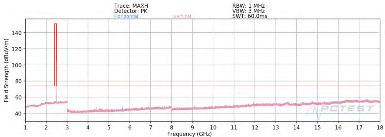
Plot 7-89. Radiated Spurious Plot Above 1GHz TXBF (4Mbps, HDR4 ePA – Ch. 75, Ant. Pol. H & V)
