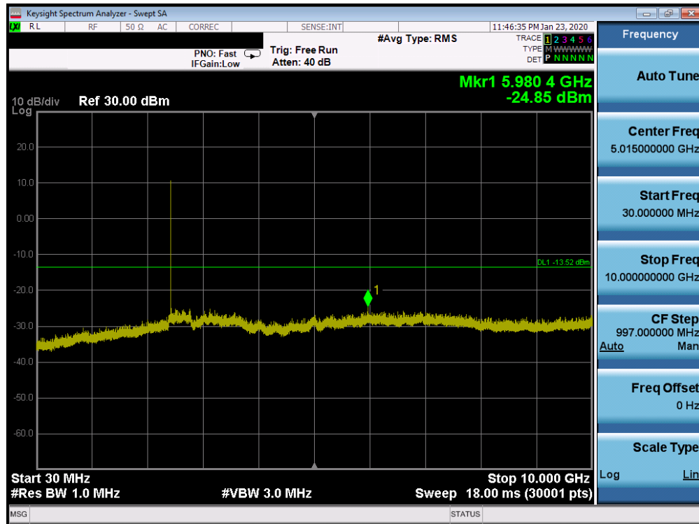
Plot 7-77. Conducted Spurious Plot Ant 2a (Bluetooth (HDR4), 4Mbps, ePA – Ch. 38)
