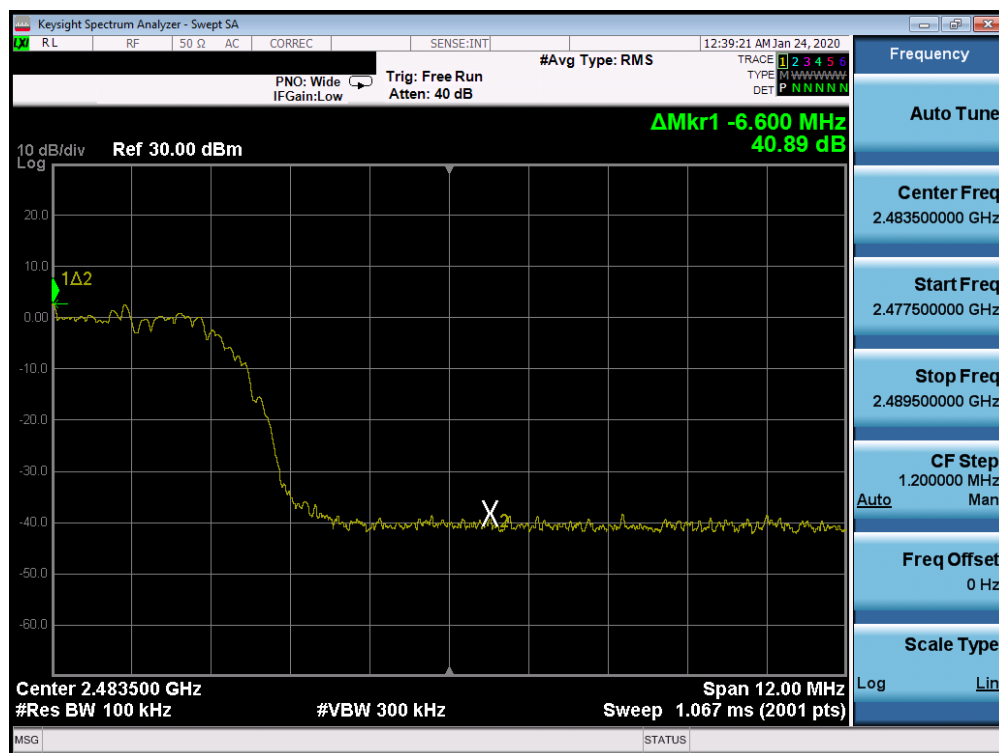
Plot 7-68. Band Edge Plot Ant 2a (Bluetooth (HDR8), ePA – Ch. 75)
