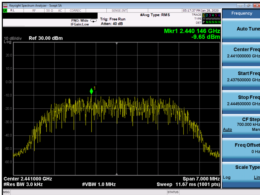
Plot 7-52. Power Spectral Density Plot TxBF Ant 2a (Bluetooth (HDR8), 8Mbps, ePA – Ch. 38)
