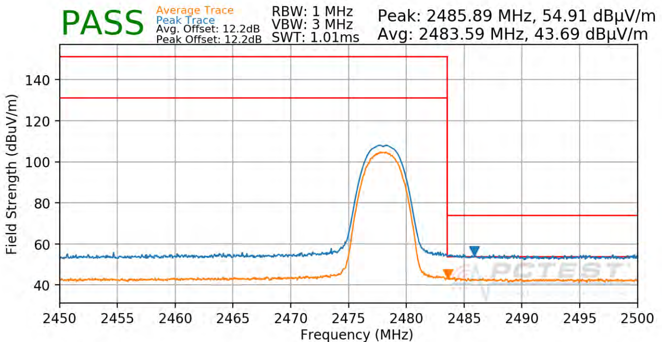
Plot 7-98. Radiated Restricted Upper Band Edge Measurement Ant 2a (Average & Peak)
