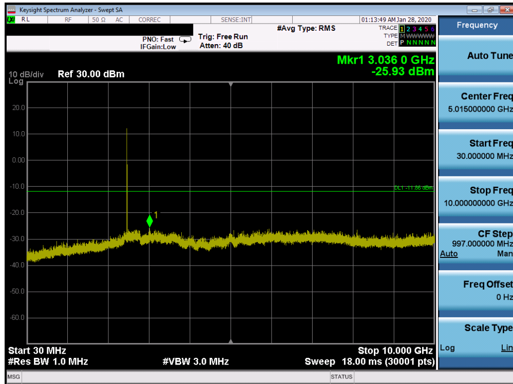
Plot 7-73. Conducted Spurious Plot Ant 4a (Bluetooth (HDR4), 4Mbps, ePA – Ch. 75)
