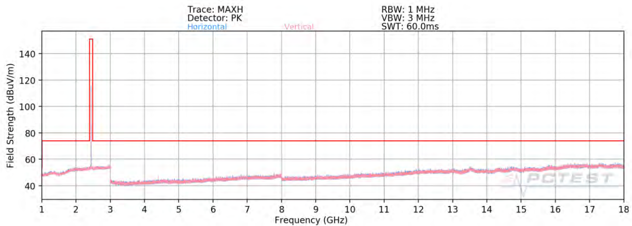
Plot 7-82. Radiated Spurious Plot Above 1GHz Ant 4a (4Mbps, HDR4 ePA – Ch. 38, Ant. Pol. H & V)
