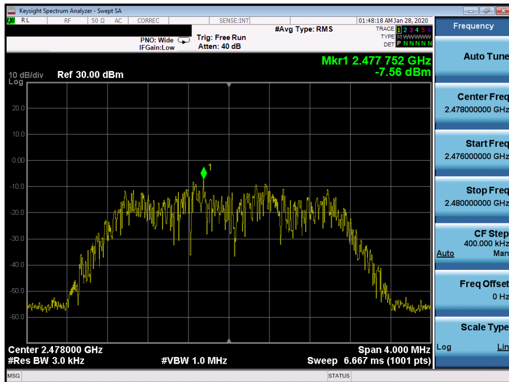
Plot 7-42. Power Spectral Density Plot TxBF Ant 2a (Bluetooth (HDR4), 4Mbps, ePA – Ch. 75)
