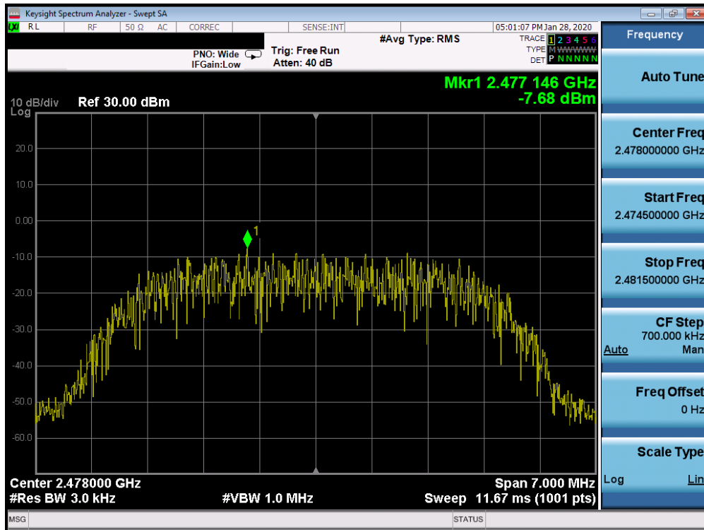
Plot 7-53. Power Spectral Density Plot Tx BF Ant 4a (Bluetooth (HDR8), 8Mbps, ePA – Ch. 75)
