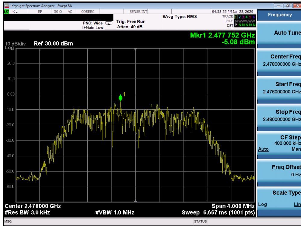
Plot 7-47. Power Spectral Density Plot TxBF Ant 4a (Bluetooth (HDR4), 4Mbps, iPA – Ch. 75)
