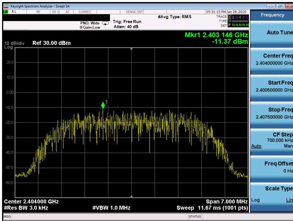
Plot 7-50. Power Spectral Density Plot TxBF Ant 2a (Bluetooth (HDR8), 8Mbps, ePA – Ch. 1)
