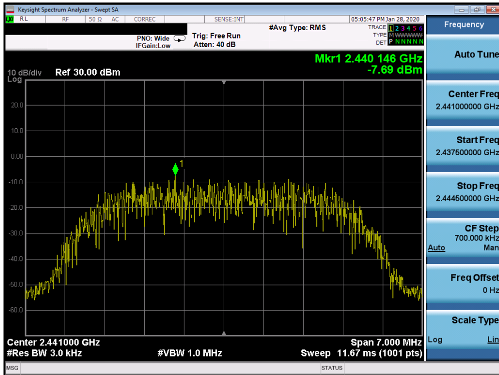
Plot 7-57. Power Spectral Density Plot TxBF Ant 4a (Bluetooth (HDR8), 8Mbps, iPA – Ch. 38)
