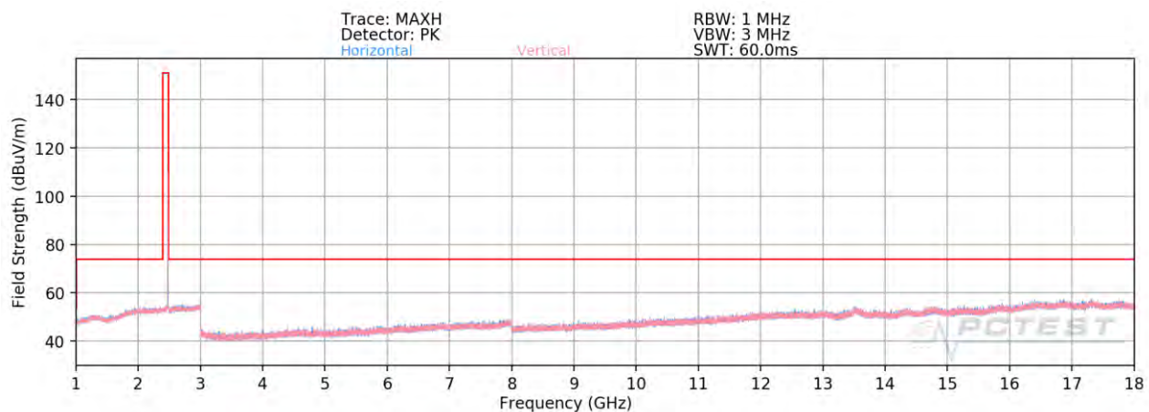
Plot 7-86. Radiated Spurious Plot Above 1GHz Ant 2a (4Mbps, HDR4 ePA – Ch. 75, Ant. Pol. H & V)
