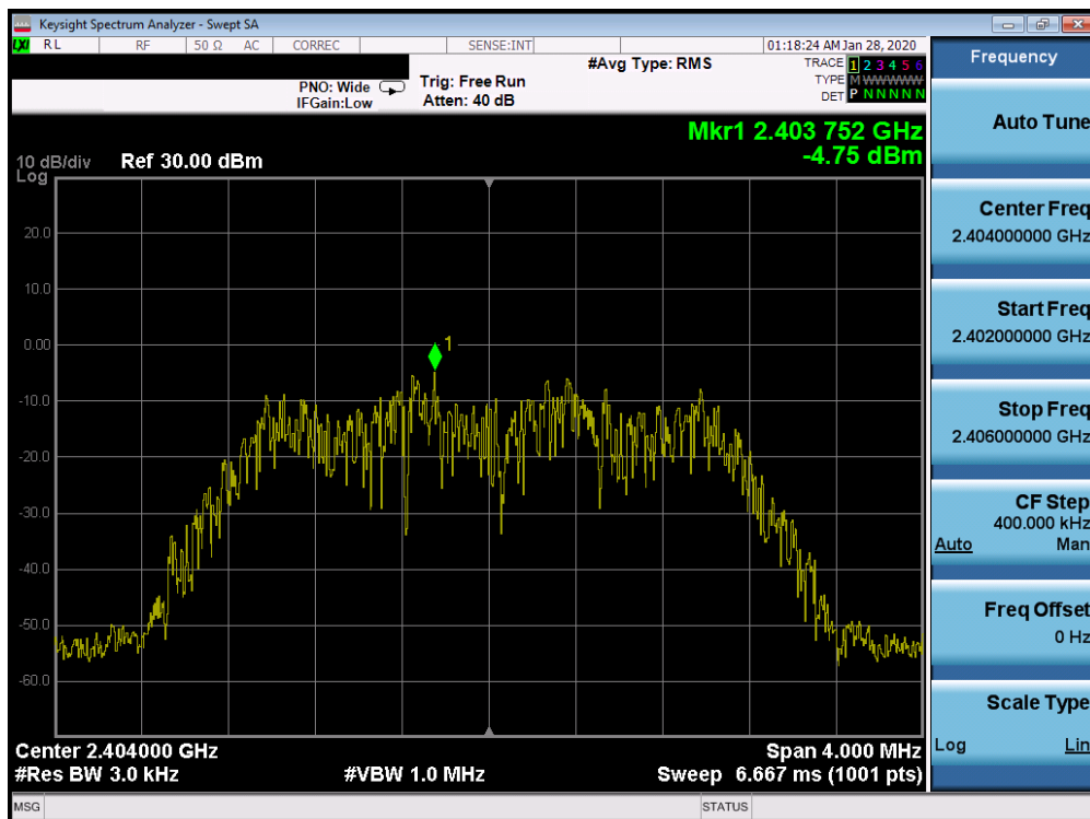
Plot 7-16. Power Spectral Density Plot Ant 4a (Bluetooth (HDR4), 4Mbps, iPA – Ch. 1)
