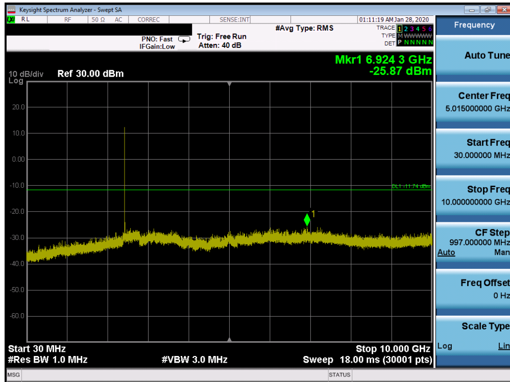
Plot 7-71. Conducted Spurious Plot Ant 4a (Bluetooth (HDR4), 4Mbps, ePA – Ch. 38)
