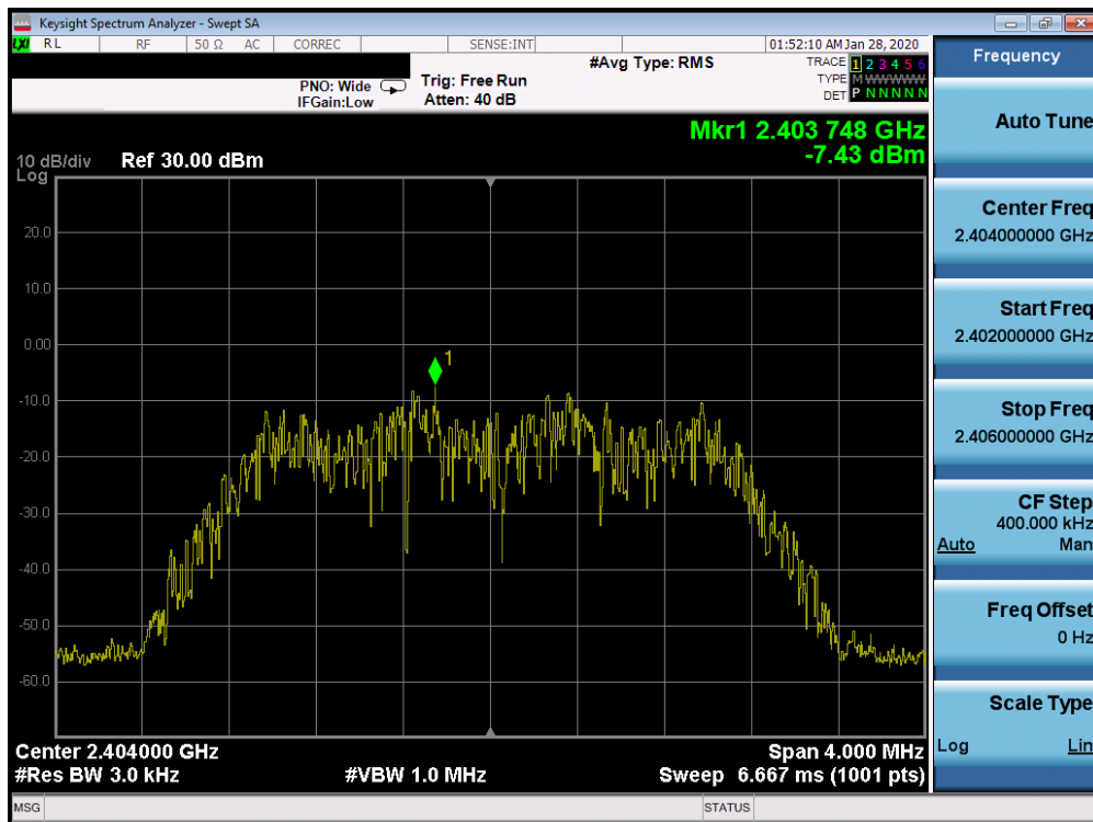
Plot 7-38. Power Spectral Density Plot TxBF Ant 2a (Bluetooth (HDR4), 4Mbps, ePA – Ch. 1)
