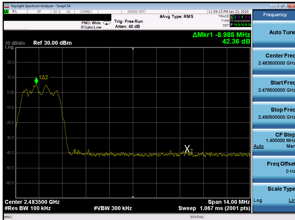
Plot 7-66. Band Edge Plot Ant 2a (Bluetooth (HDR4), ePA – Ch. 75)
