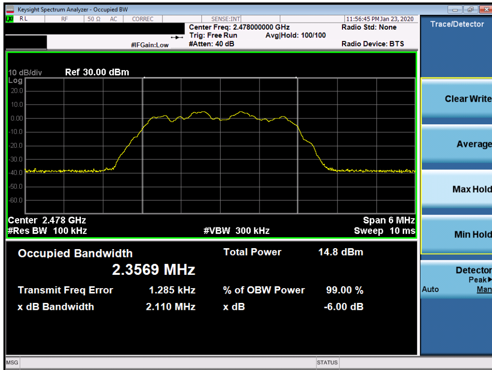
Plot 7-9. 6dB Bandwidth Plot Ant 2a (Bluetooth (HDR4), 4Mbps, ePA – Ch. 75)
