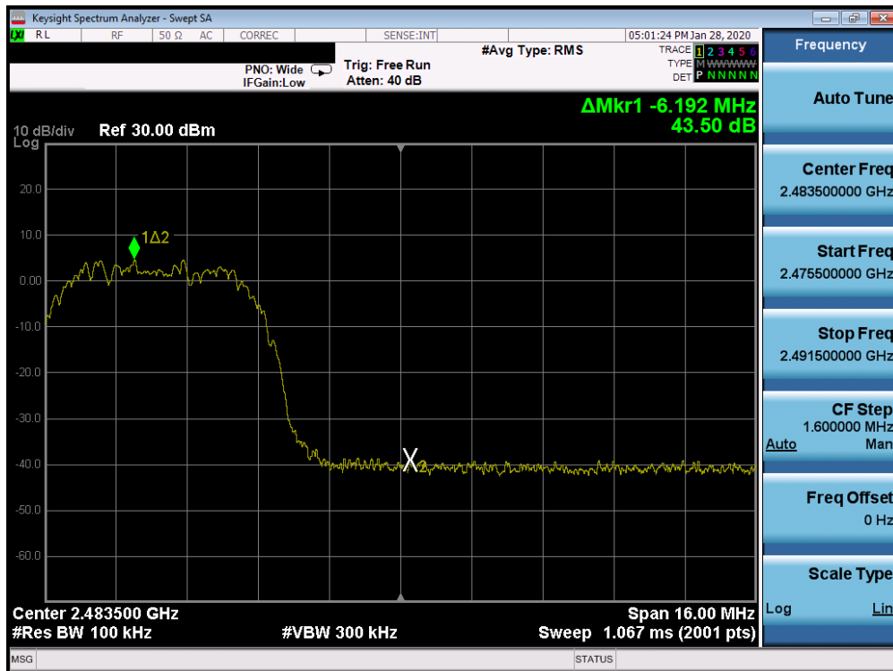
Plot 7-64. Band Edge Plot Ant 4a (Bluetooth (HDR8), ePA - Ch. 75)
