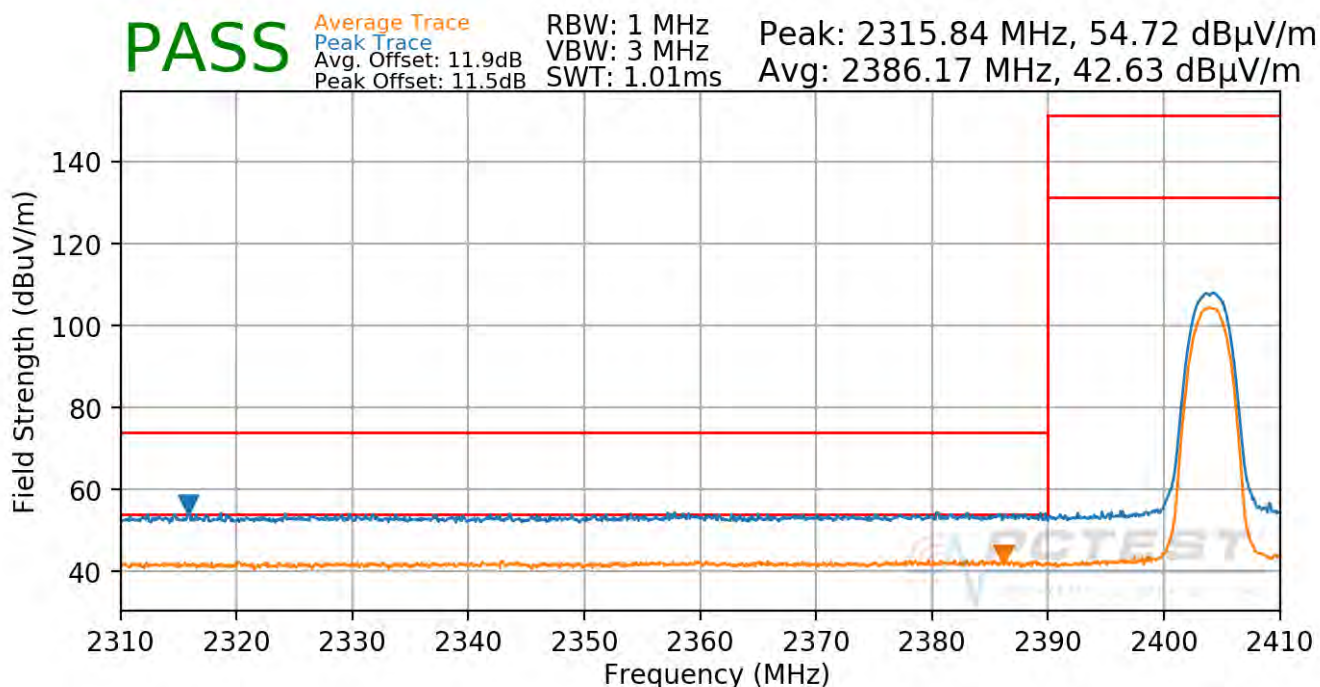
Plot 7-92. Radiated Restricted Lower Band Edge Measurement Ant 4a (Average & Peak)
