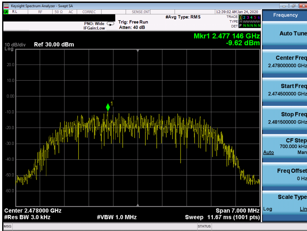
Plot 7-33. Power Spectral Density Plot Ant 2a (Bluetooth (HDR8), 8Mbps, ePA – Ch. 75)
