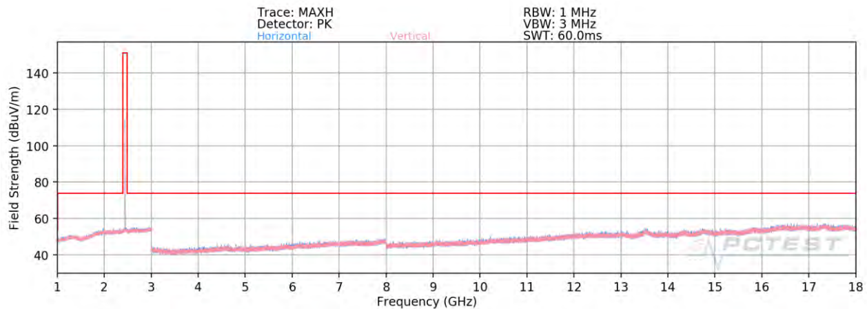
Plot 7-85. Radiated Spurious Plot Above 1GHz Ant 2a (4Mbps, HDR4 ePA – Ch. 38, Ant. Pol. H & V)
