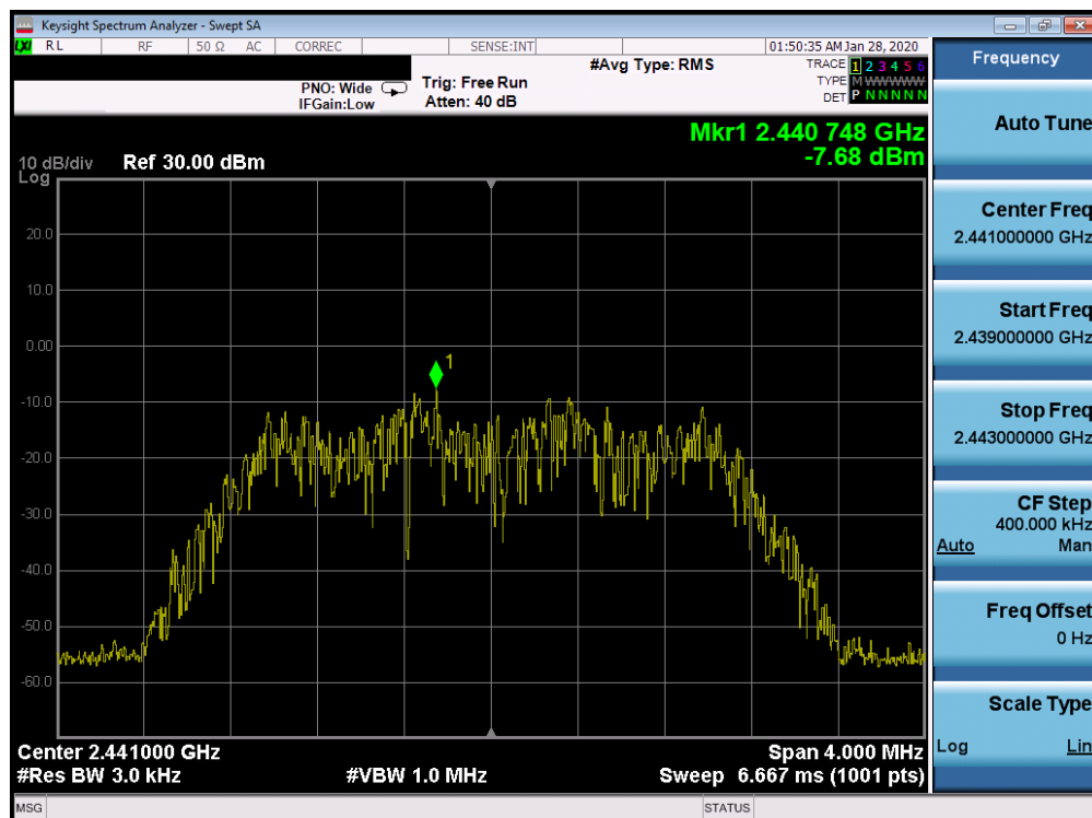
Plot 7-40. Power Spectral Density Plot TxBF Ant 2a (Bluetooth (HDR4), 4Mbps, ePA – Ch. 38)
