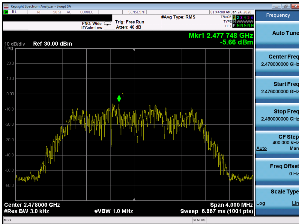
Plot 7-21. Power Spectral Density Plot Ant 4a (Bluetooth (HDR8), 8Mbps, ePA – Ch. 75)
