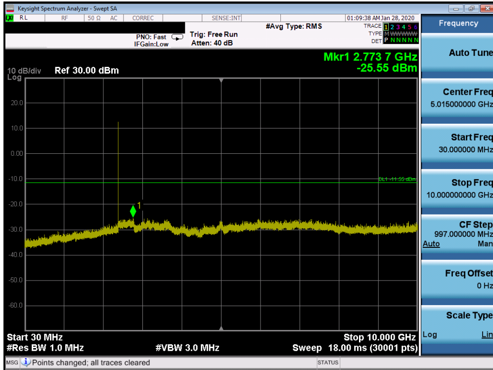
Plot 7-69. Conducted Spurious Plot Ant 4a (Bluetooth (HDR4), 4Mbps, ePA – Ch. 1)
