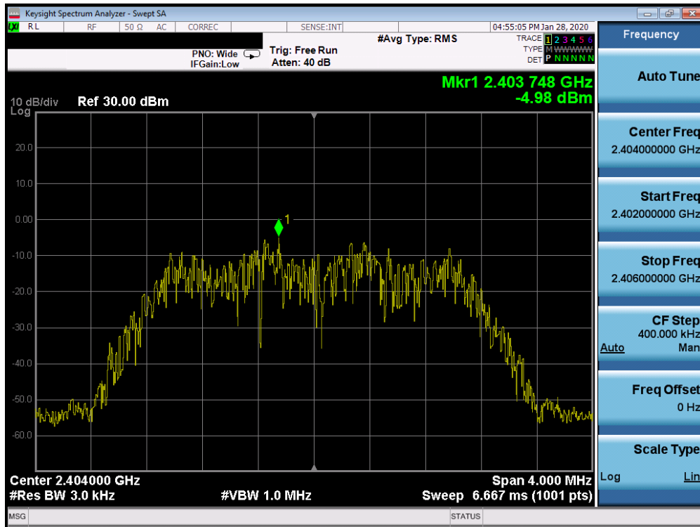
Plot 7-43. Power Spectral Density Plot Tx BF Ant 4a (Bluetooth (HDR4), 4Mbps, iPA – Ch. 1)
