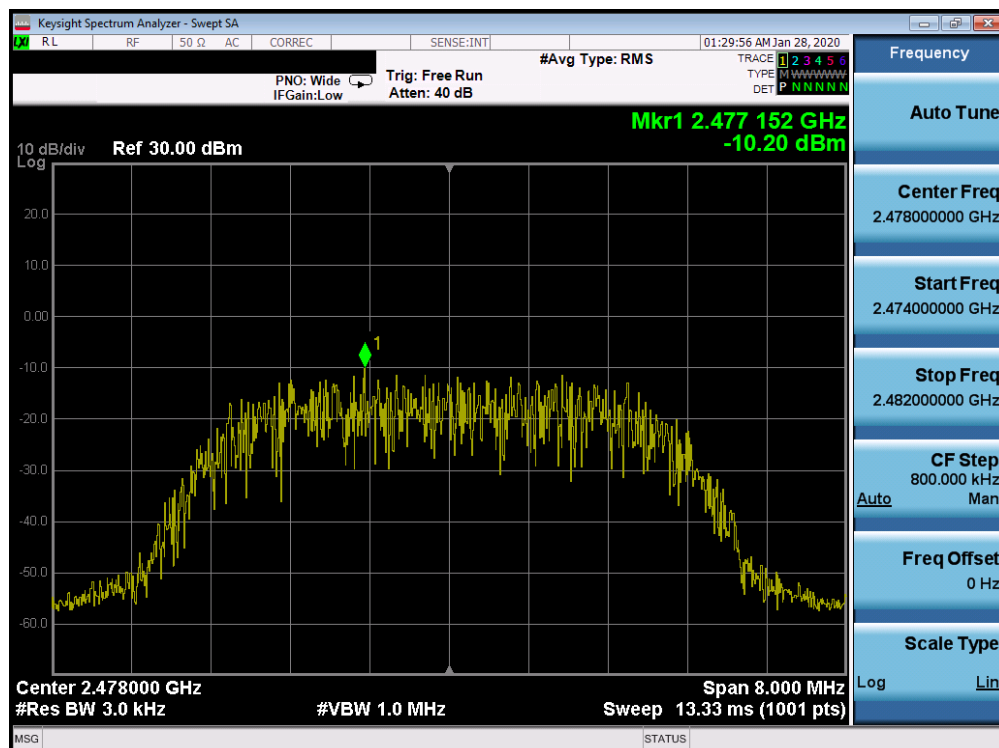
Plot 7-36. Power Spectral Density Plot Ant 2a (Bluetooth (HDR8), 8Mbps, iPA – Ch. 75)
