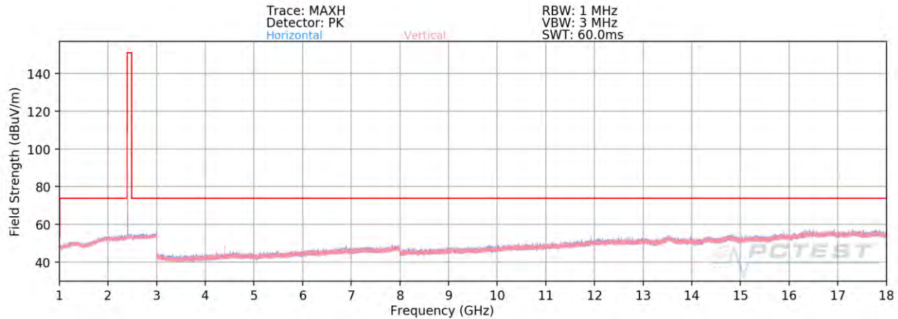
Plot 7-84. Radiated Spurious Plot Above 1GHz Ant 2a (4Mbps, HDR4 ePA – Ch. 1, Ant. Pol. H & V)
