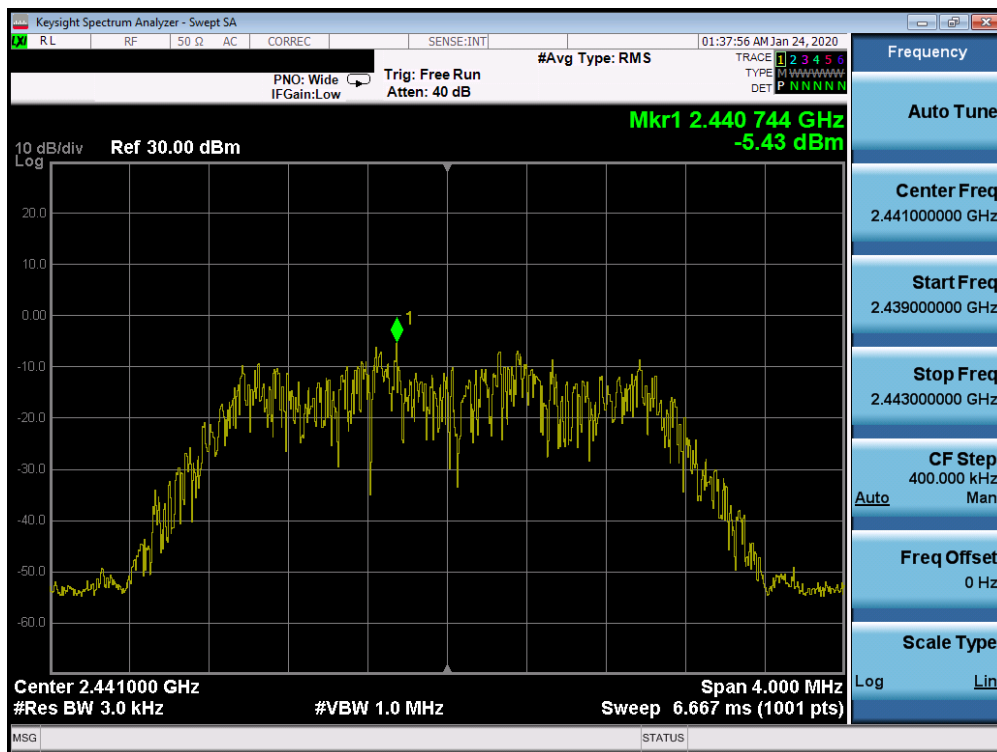
Plot 7-20. Power Spectral Density Plot Ant 4a (Bluetooth (HDR8), 8Mbps, ePA – Ch. 38)
