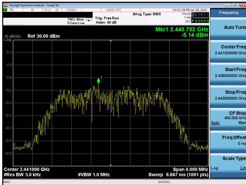
Plot 7-39. Power Spectral Density Plot TxBF Ant 4a (Bluetooth (HDR4), 4Mbps, ePA – Ch. 38)
