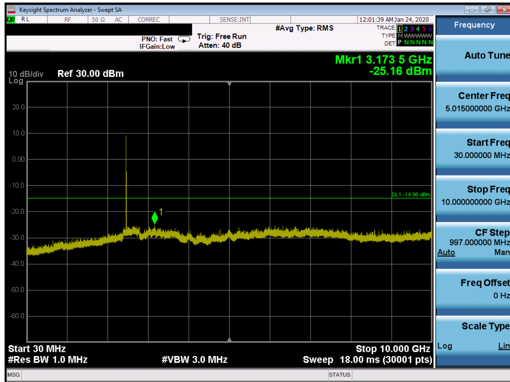
Plot 7-79. Conducted Spurious Plot Ant 2a (Bluetooth (HDR4), 4Mbps, ePA – Ch. 75)
