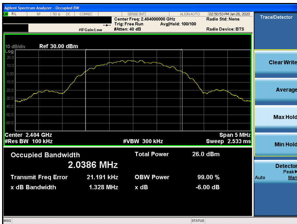
Plot 7-10. 6dB Bandwidth Plot Ant 2a (Bluetooth (LE), 2Mbps, ePA – Ch. 0)
