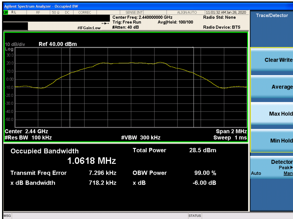
Plot 7-2. 6dB Bandwidth Plot Ant 4a (Bluetooth (LE), 1Mbps, ePA – Ch. 19)
