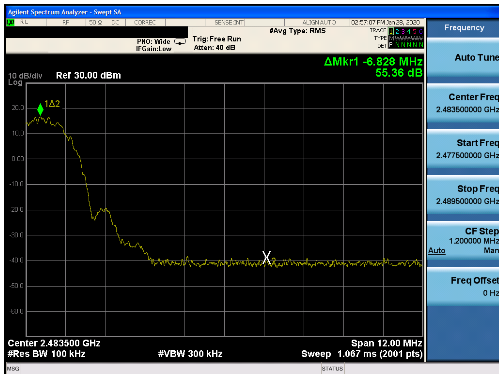
Plot 7-68. Band Edge Plot Ant 2a (Bluetooth (LE), 2Mbps ePA – Ch. 38)
