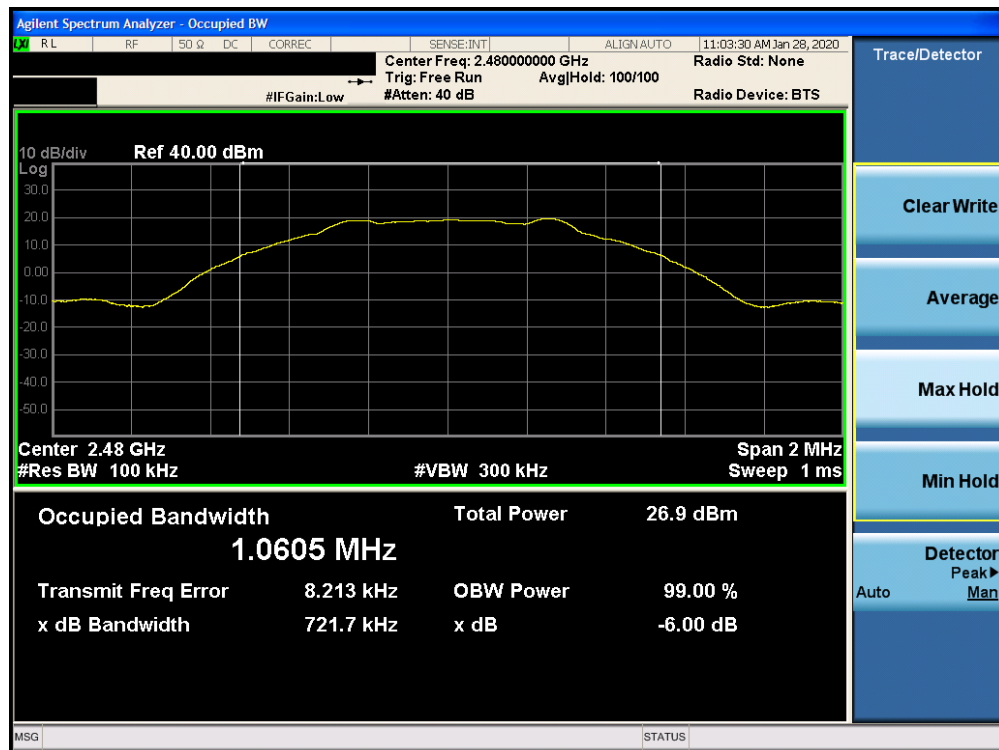
Plot 7-3. 6dB Bandwidth Plot Ant 4a (Bluetooth (LE), 1Mbps, ePA – Ch. 39)
