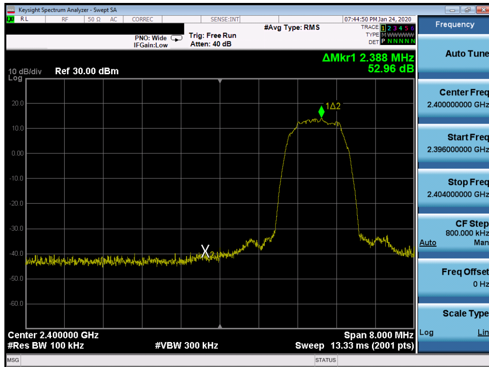
Plot 7-17. Band Edge Plot Ant 4a (Bluetooth with Hopping Disabled, 8DPSK, ePA – Ch. 0)
