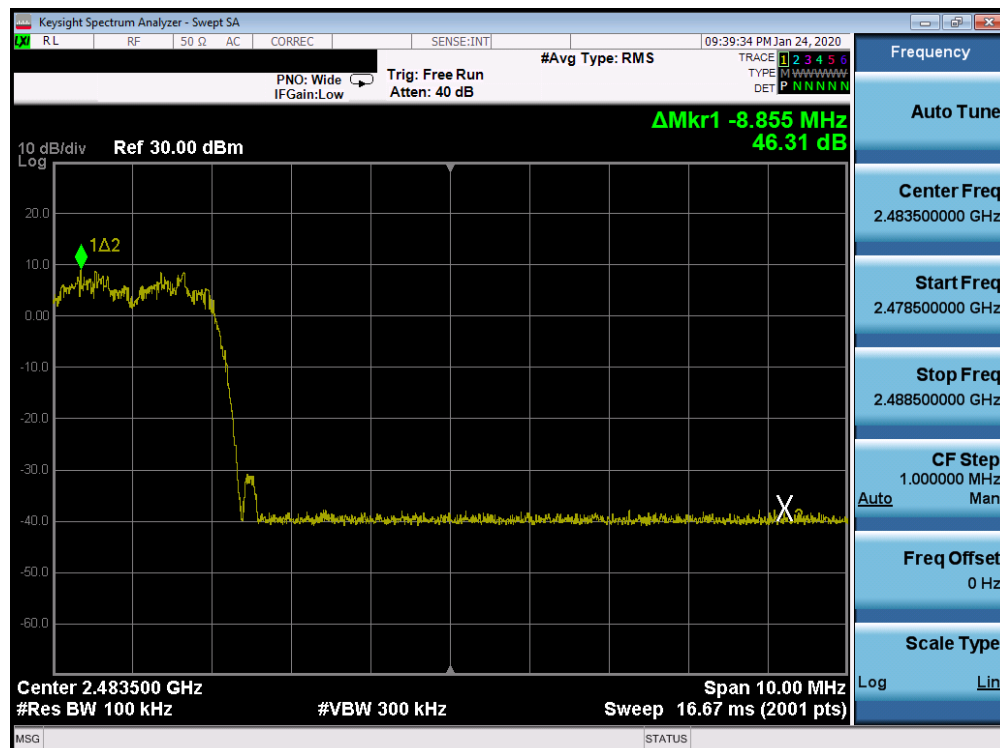
Plot 7-28. Band Edge Plot Ant 2a (Bluetooth with Hopping Enabled, 8DPSK, ePA)
