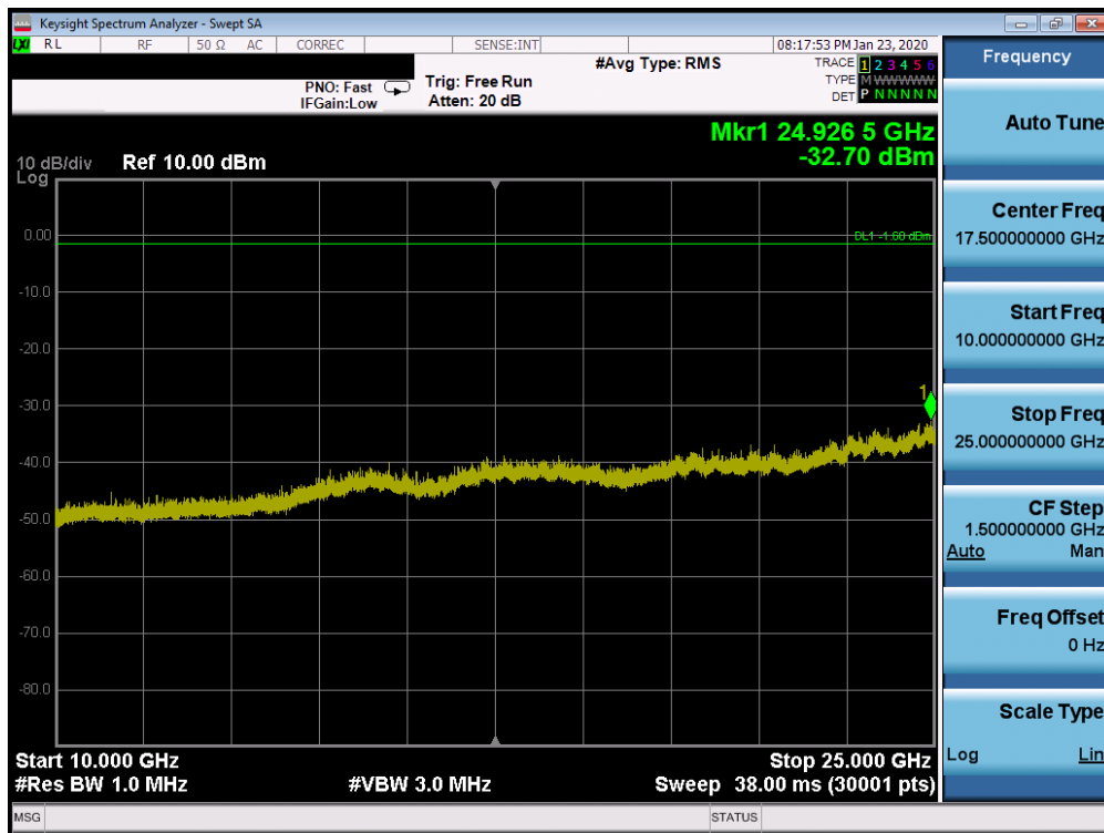
Plot 7-48. Conducted Spurious Plot Ant 4a (Bluetooth, GFSK, ePA Ch. 39)
