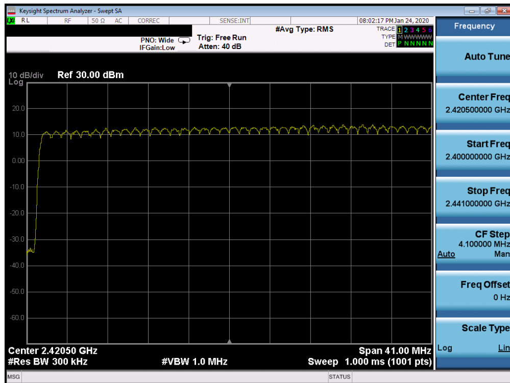
Plot 7-39. Low End Spectrum Channel Hopping Plot Ant 4a (Bluetooth, 8DPSK, ePA)
