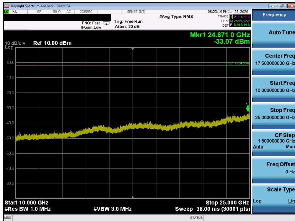
Plot 7-50. Conducted Spurious Plot Ant 4a (Bluetooth, GFSK, ePA – Ch. 78)
