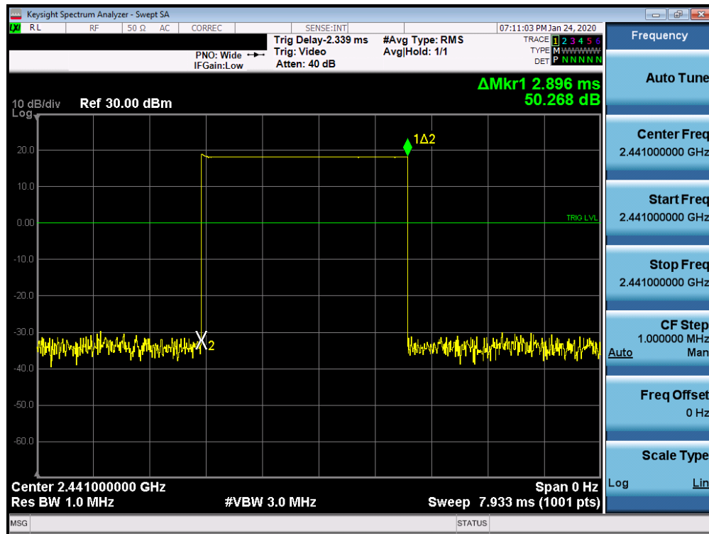
Plot 7-35. Time of Occupancy Plot Ant 2a (Bluetooth, GFSK, ePA)
