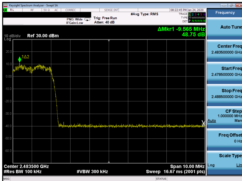
Plot 7-20. Band Edge Plot Ant 4a (Bluetooth with Hopping Enabled, 8DPSK, ePA)
