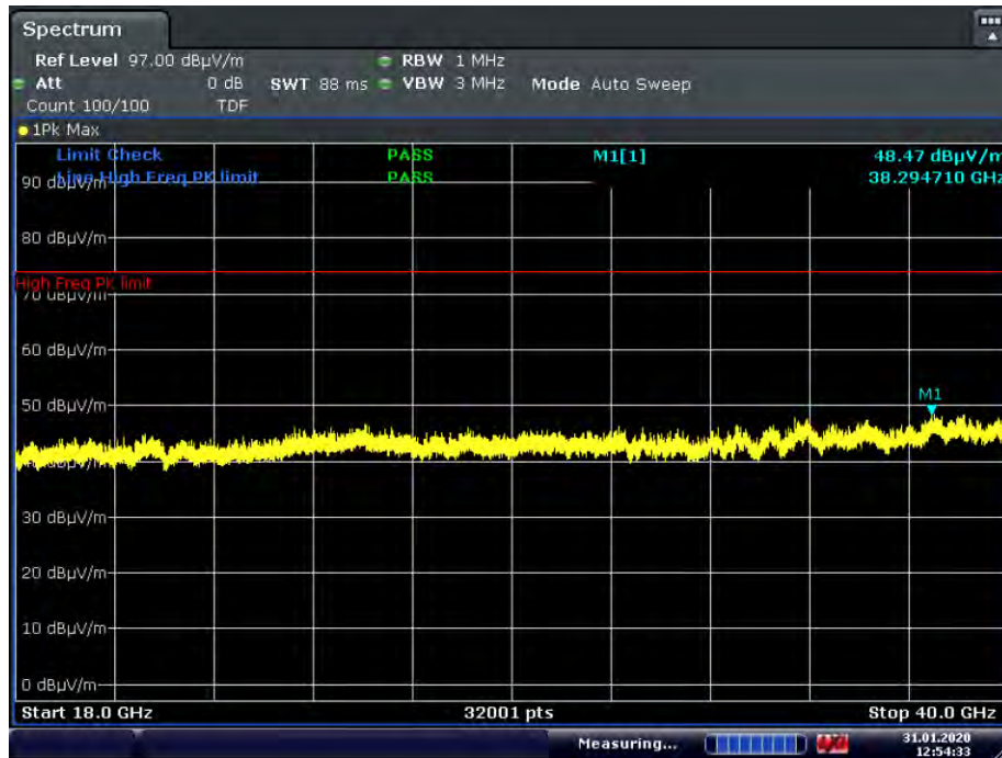
Plot 7-69. Radiated Spurious Plot 18GHz Simultaneous Tx – 40GHz Pol. H
