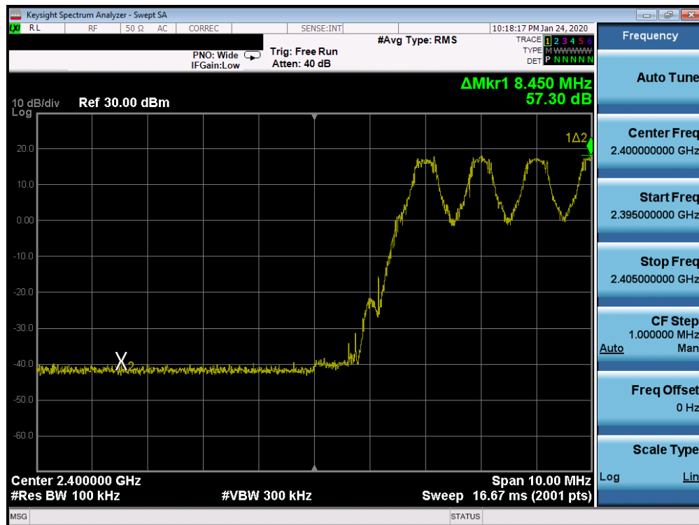
Plot 7-23. Band Edge Plot Ant 2a (Bluetooth with Hopping Enabled, GFSK, ePA)
