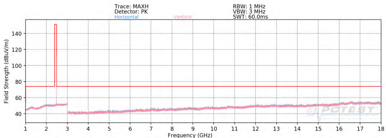
Plot 7-59. Radiated Spurious Plot above 1GHz Ant 4a (BT GFSK ePA – Ch. 78)
