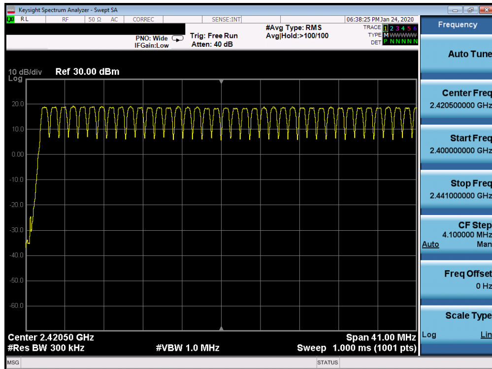
Plot 7-41. Low End Spectrum Channel Hopping Plot Ant 2a (Bluetooth, GFSK, ePA)
