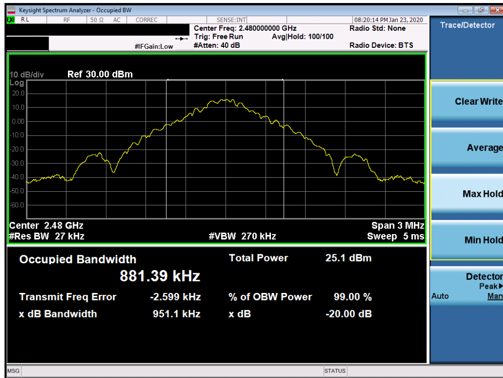
Plot 7-3. 20dB Bandwidth Plot Ant 4a (Bluetooth, GFSK, ePA – Ch. 78)
