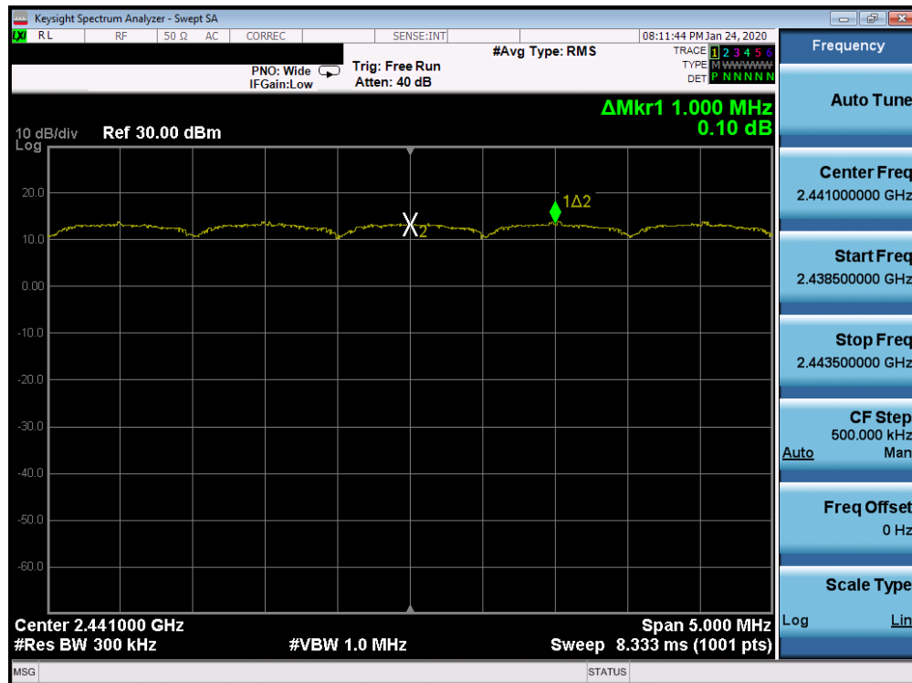
Plot 7-30. Channel Spacing Plot Ant 4a (Bluetooth, 8DPSK, ePA)
