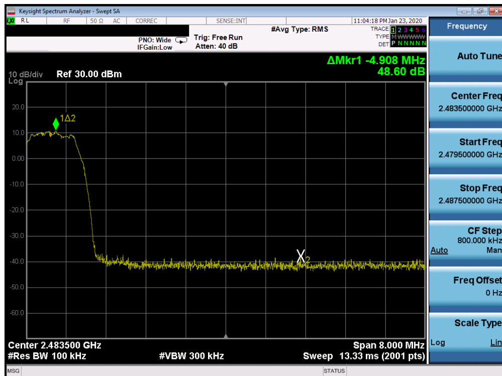
Plot 7-26. Band Edge Plot Ant 2a (Bluetooth with Hopping Disabled, 8DPSK, ePA – Ch. 78)
