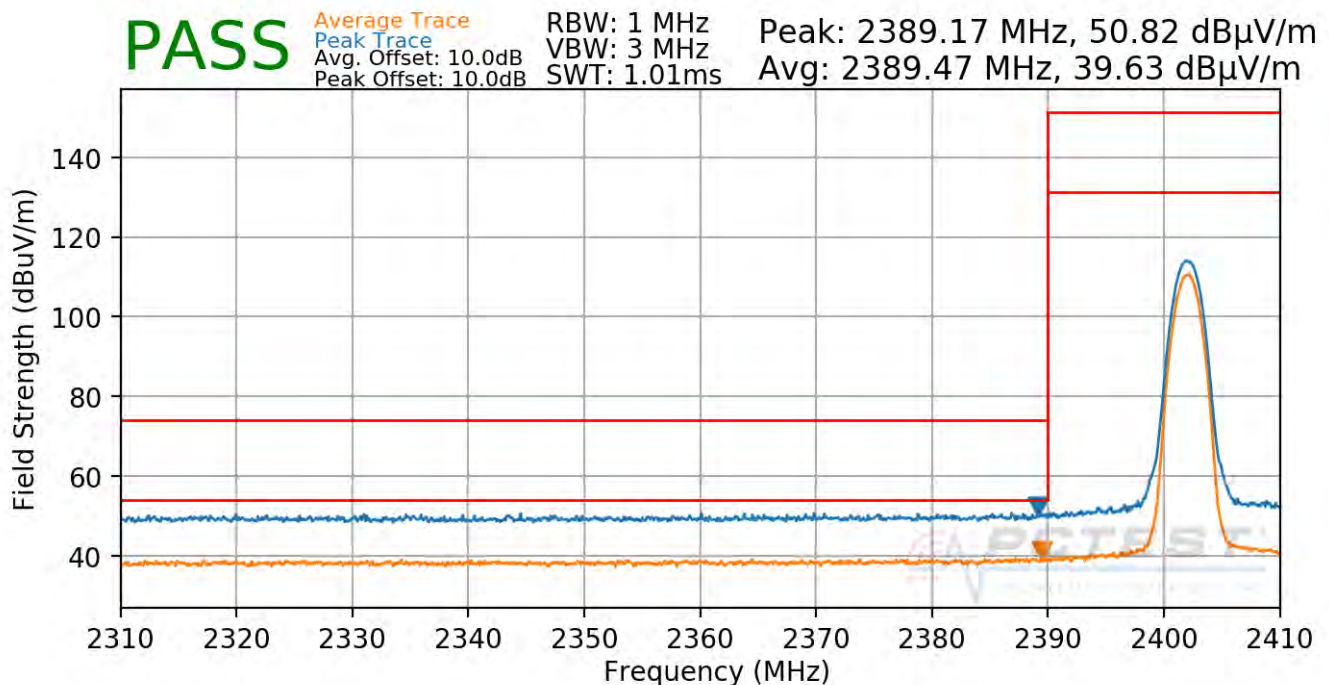
Plot 7-72. Radiated Restricted Lower Band Edge Measurement Ant 4a (Average & Peak)
