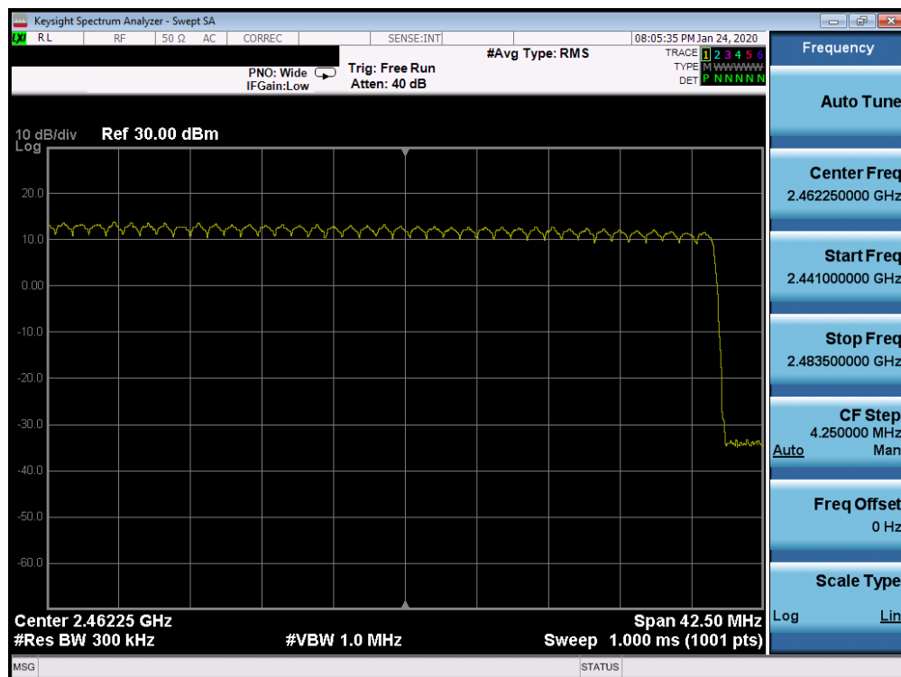
Plot 7-40. High End Spectrum Channel Hopping Plot Ant 4a (Bluetooth, 8DPSK, ePA)
