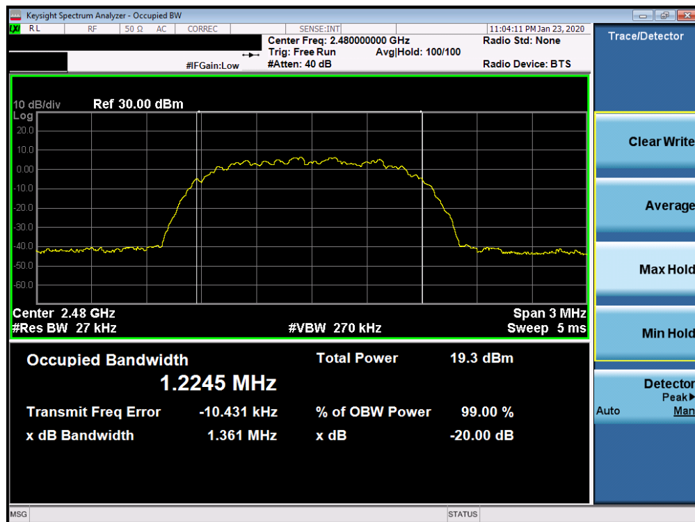
Plot 7-12. 20dB Bandwidth Plot Ant 2a (Bluetooth, 8DPSK, ePA – Ch. 78)
