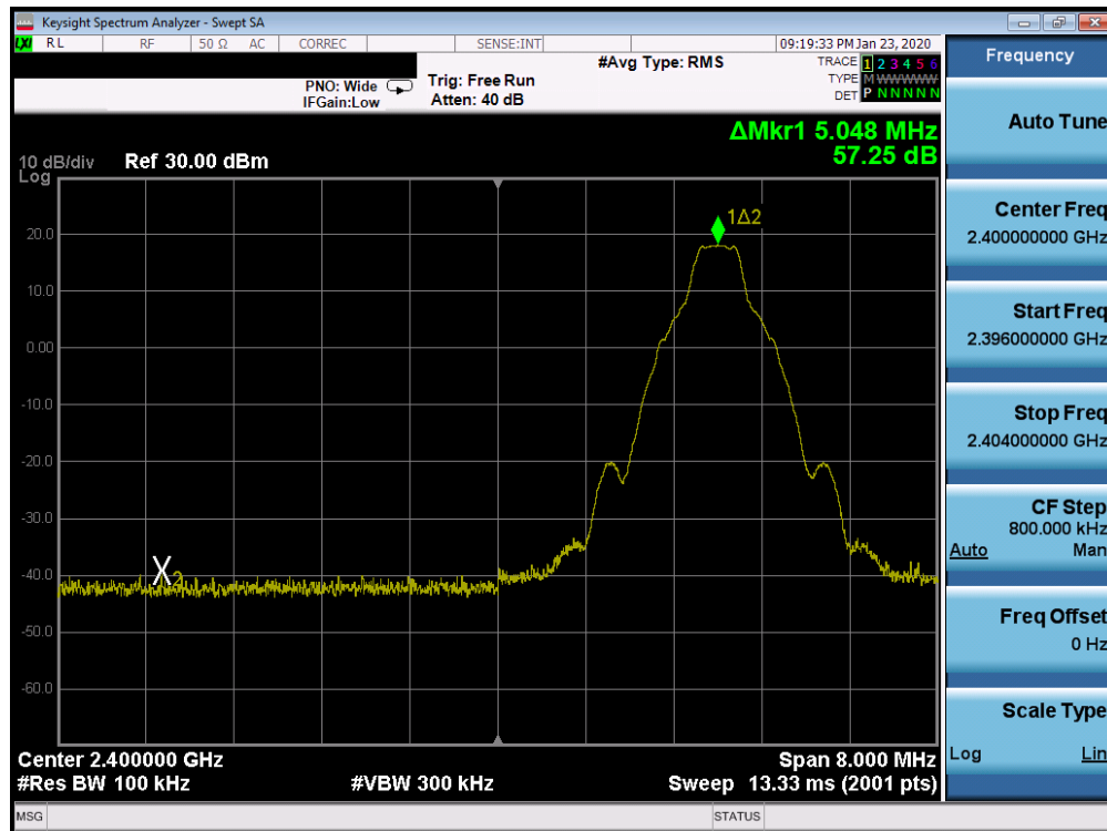
Plot 7-21. Band Edge Plot Ant 2a (Bluetooth with Hopping Disabled, GFSK, ePA – Ch. 0)
