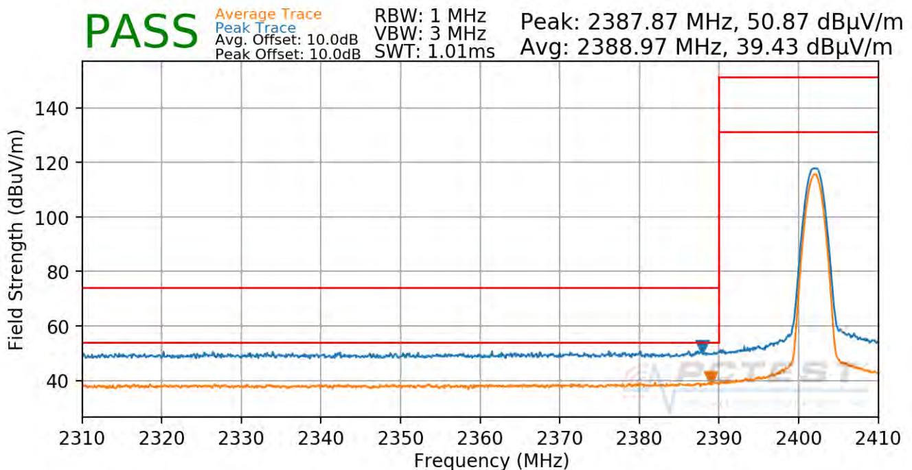
Plot 7-75. Radiated Restricted Lower Band Edge Measurement Ant 2a (Average & Peak)
