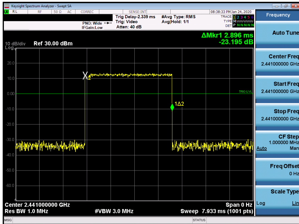
Plot 7-36. Time of Occupancy Plot Ant 2a (Bluetooth, 8DPSK, ePA)
