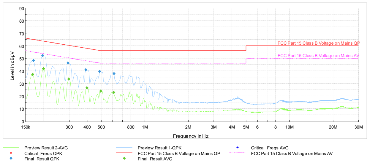
Plot 7-86. Line-Conducted Test Plot- Ch.39 TxBF (N, with AC/DC Adapter)
