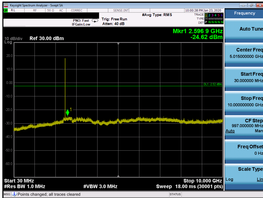
Plot 7-55. Conducted Spurious Plot Ant 2a (Bluetooth, GFSK, ePA – Ch. 78)
