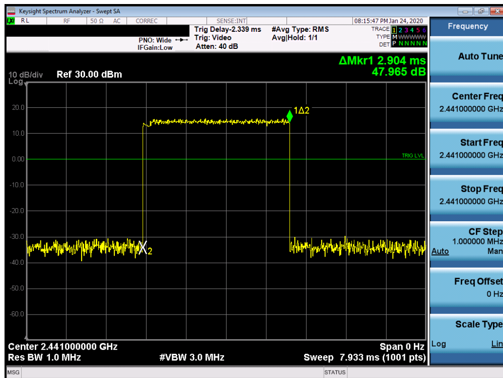
Plot 7-34. Time of Occupancy Plot Ant 4a (Bluetooth, 8DPSK, ePA)
