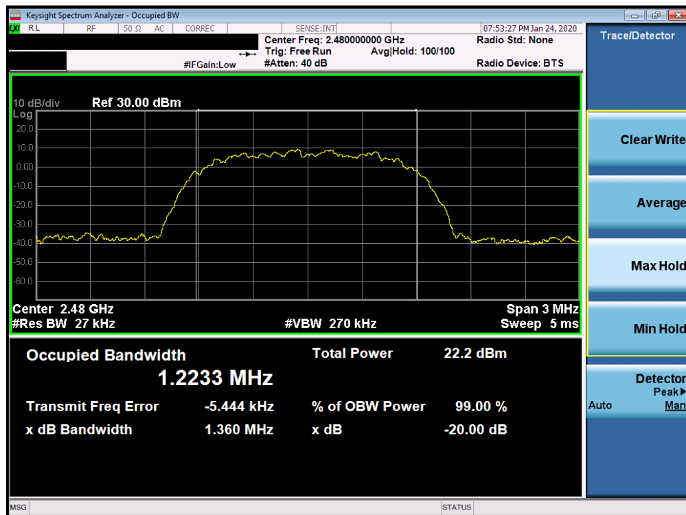
Plot 7-6. 20dB Bandwidth Plot Ant 4a (Bluetooth, 8DPSK, ePA – Ch. 78)
