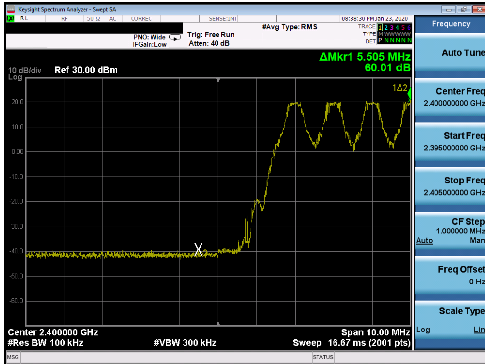
Plot 7-15. Band Edge Plot Ant 4a (Bluetooth with Hopping Enabled, GFSK, ePA)
