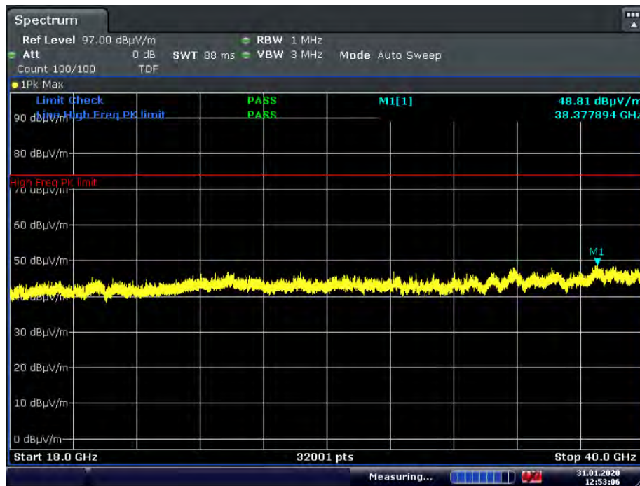
Plot 7-70. Radiated Spurious Plot 18GHz Simultaneous Tx – 40GHz Pol. V
