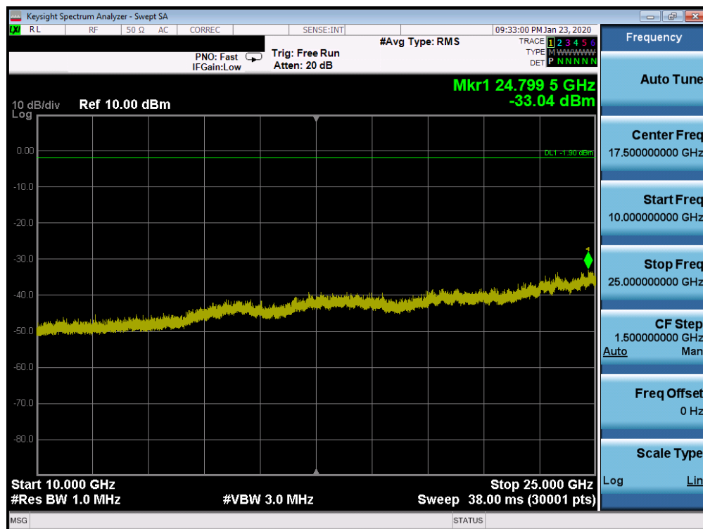
Plot 7-54. Conducted Spurious Plot Ant 2a (Bluetooth, GFSK, ePA Ch. 39)
