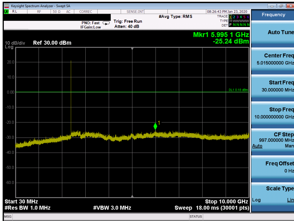
Plot 7-45. Conducted Spurious Plot Ant 4a (Bluetooth, GFSK, ePA – Ch. 0)
