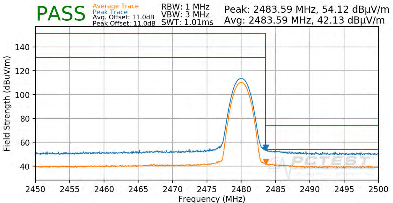
Plot 7-78. Radiated Restricted Upper Band Edge Measurement Ant 2a (Average & Peak)
