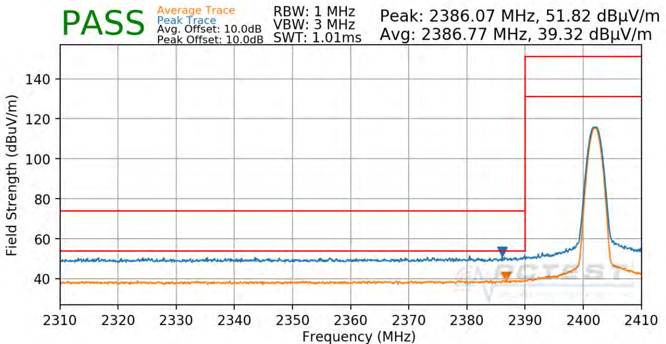
Plot 7-71. Radiated Restricted Lower Band Edge Measurement Ant 4a (Average & Peak)
