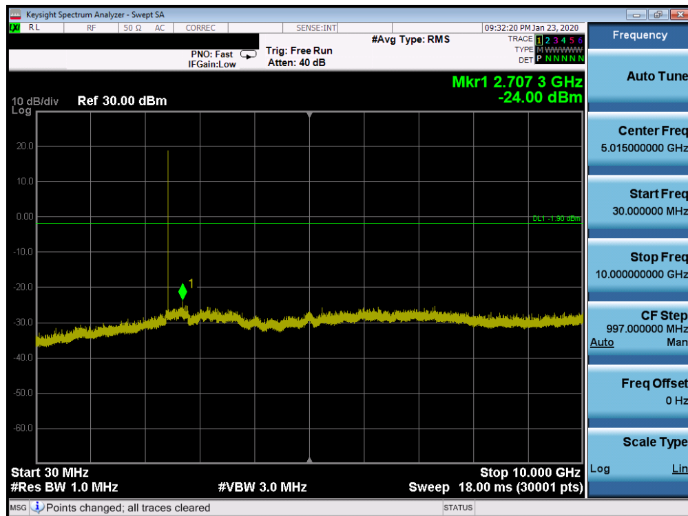
Plot 7-53. Conducted Spurious Plot Ant 2a (Bluetooth, GFSK, ePA – Ch. 39)
