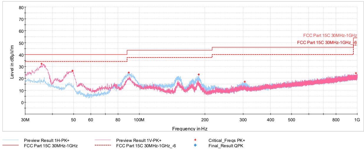
Plot 7-84. Radiated Spurious Plot below 1GHz Simultaneous Tx, with AC/DC Adapter
