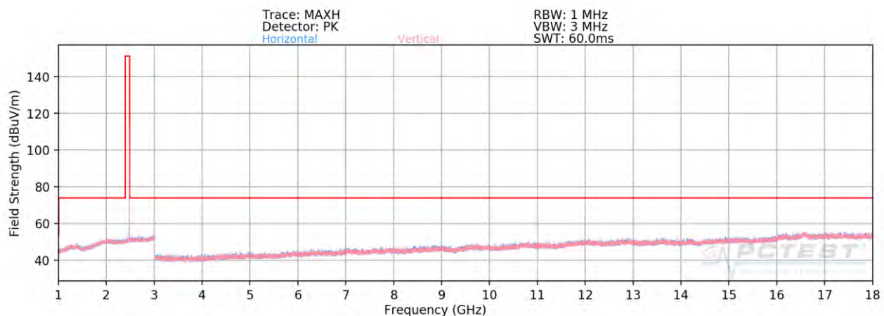
Plot 7-65. Radiated Spurious Plot above 1GHz TXBF (BT GFSK ePA – Ch. 78)
