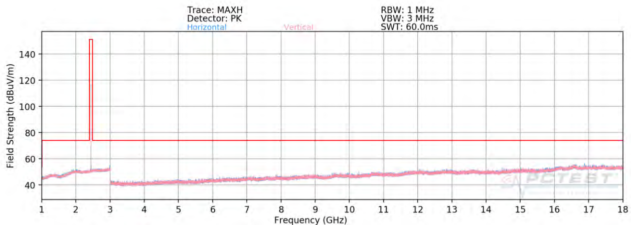
Plot 7-58. Radiated Spurious Plot above 1GHz Ant 4a (BT GFSK ePA – Ch. 39)
