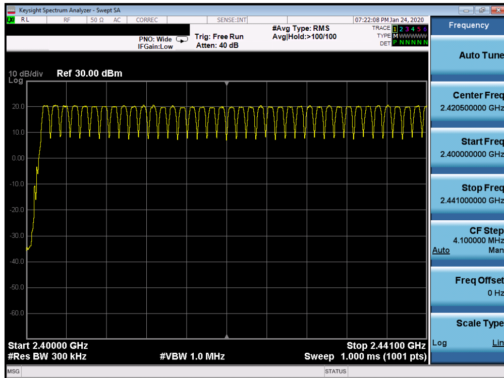
Plot 7-37. Low End Spectrum Channel Hopping Plot Ant 4a (Bluetooth, GFSK, ePA)
