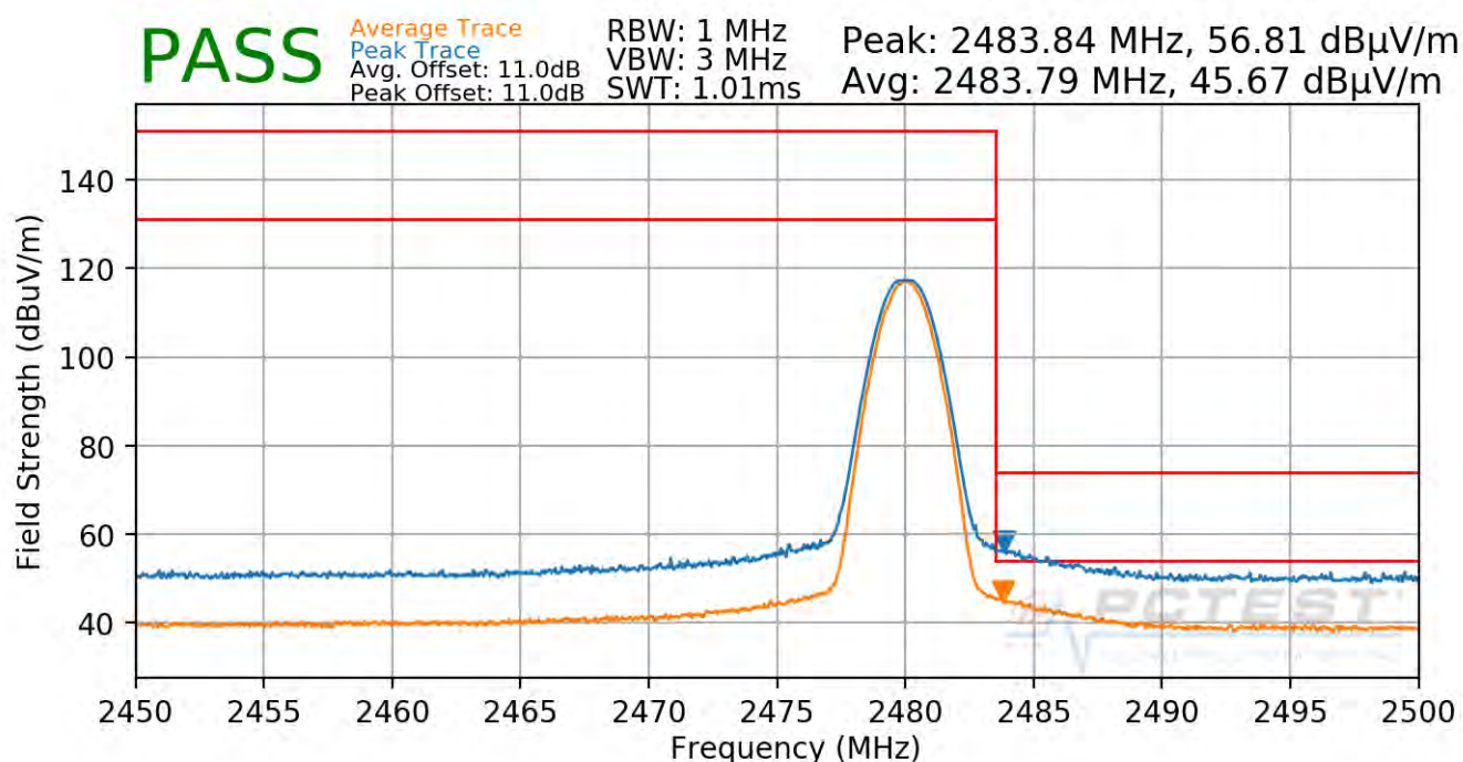
Plot 7-73. Radiated Restricted Upper Band Edge Measurement Ant 4a (Average & Peak)
