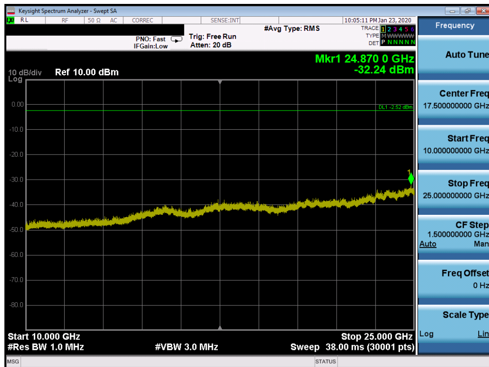
Plot 7-56. Conducted Spurious Plot Ant 2a (Bluetooth, GFSK, ePA – Ch. 78)
