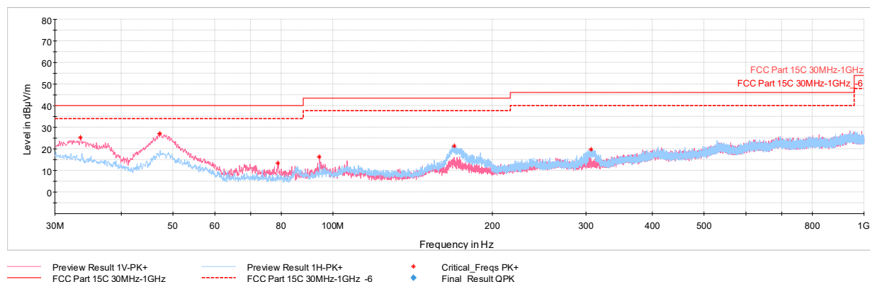
Plot 7-83. Radiated Spurious Plot below 1GHz GFSK ePA TxBF – Ch.39 , with AC/DC Adapter)
