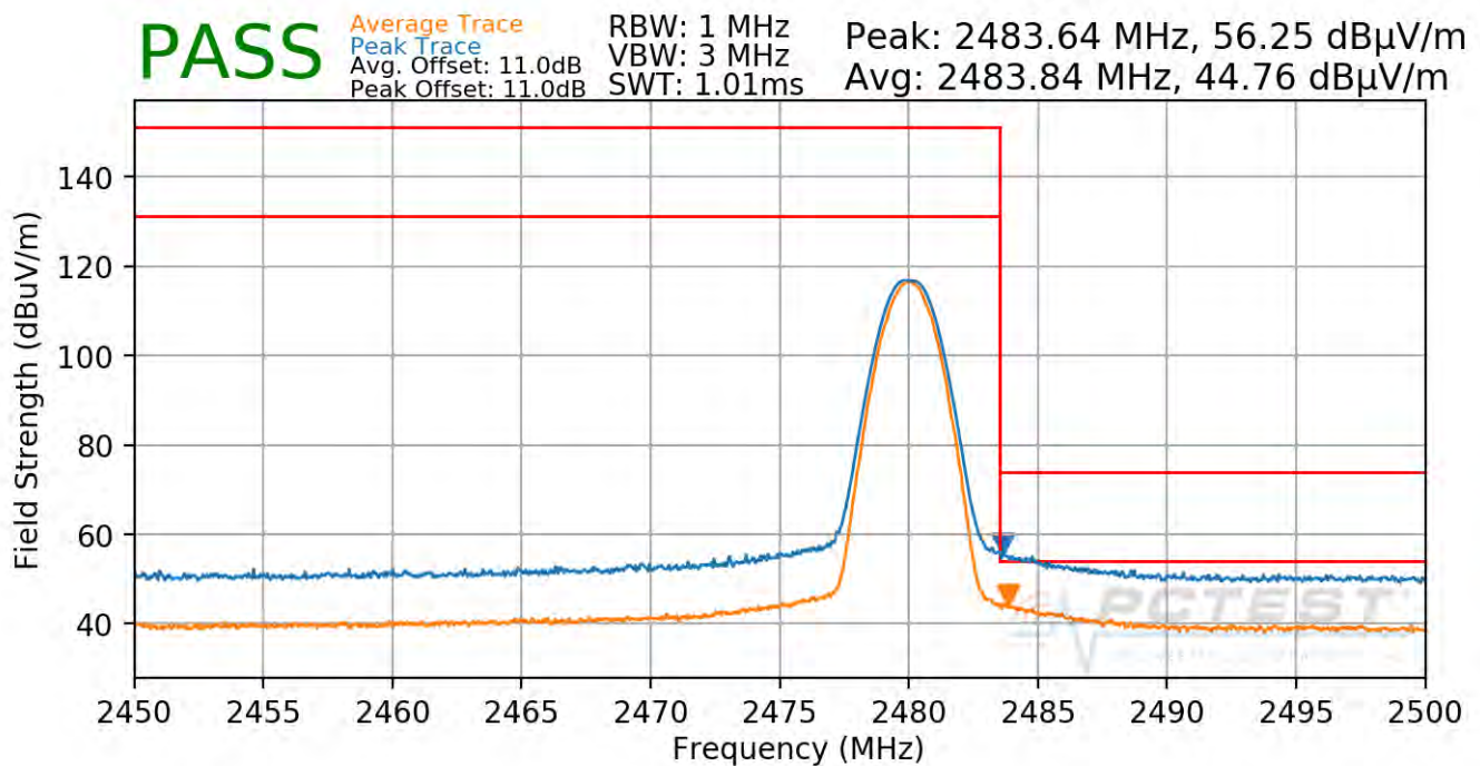
Plot 7-77. Radiated Restricted Upper Band Edge Measurement Ant 2a (Average & Peak)
