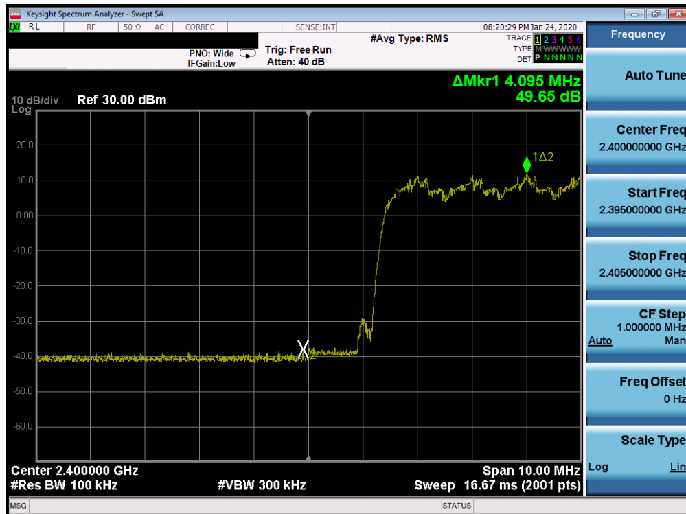
Plot 7-19. Band Edge Plot Ant 4a (Bluetooth with Hopping Enabled, 8DPSK, ePA)
