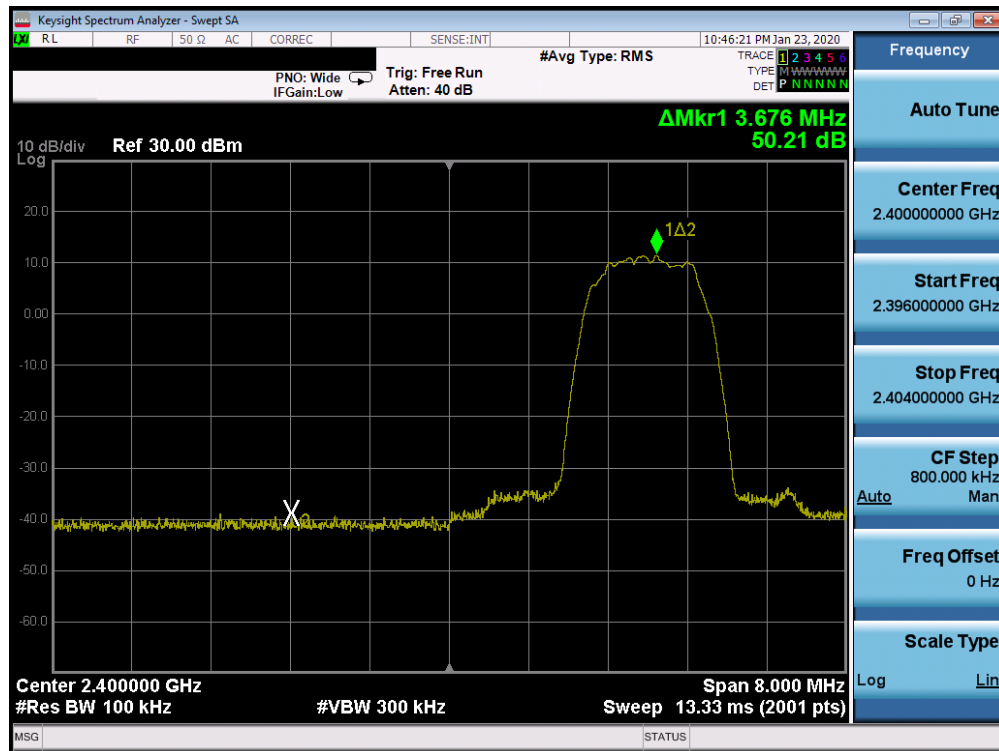
Plot 7-25. Band Edge Plot Ant 2a (Bluetooth with Hopping Disabled, 8DPSK, ePA – Ch. 0)
