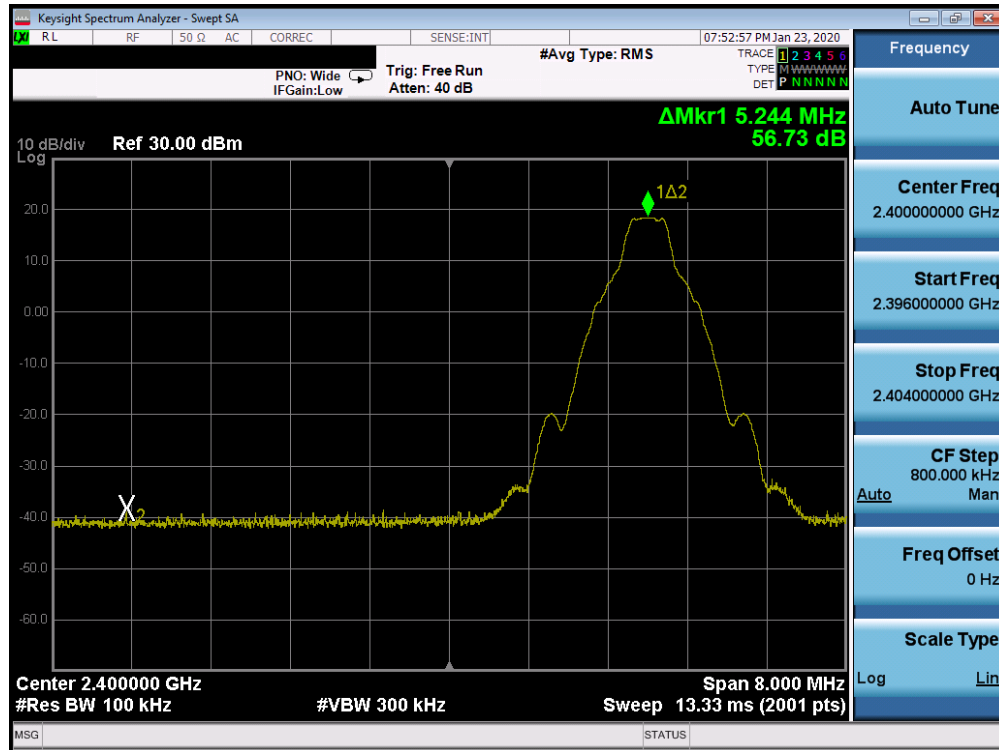
Plot 7-13. Band Edge Plot Ant 4a (Bluetooth with Hopping Disabled, GFSK, ePA – Ch. 0)
