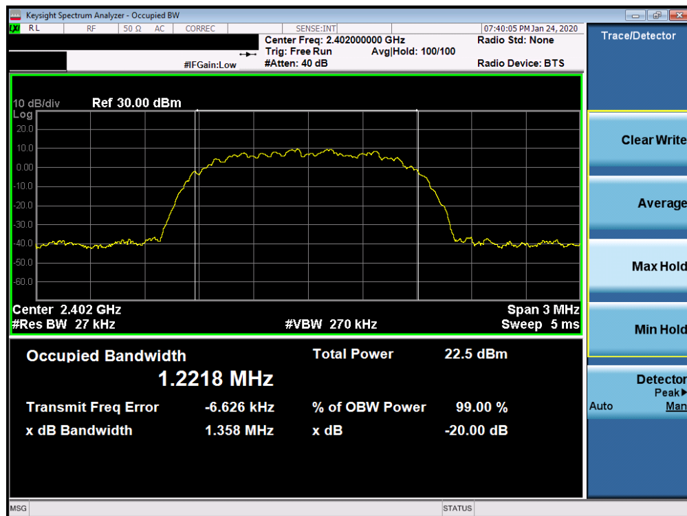
Plot 7-4. 20dB Bandwidth Plot Ant 4a (Bluetooth, 8DPSK, ePA – Ch. 0)
