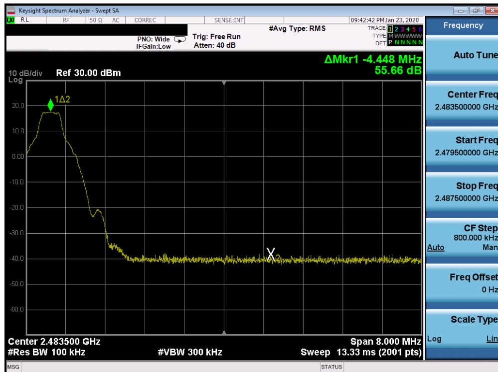
Plot 7-22. Band Edge Plot Ant 2a (Bluetooth with Hopping Disabled, GFSK, ePA – Ch. 78)
