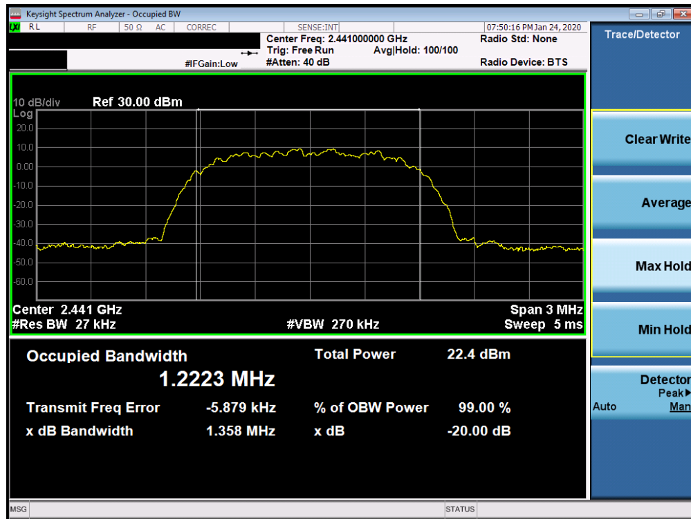
Plot 7-5. 20dB Bandwidth Plot Ant 4a (Bluetooth, 8DPSK, ePA – Ch. 39)
