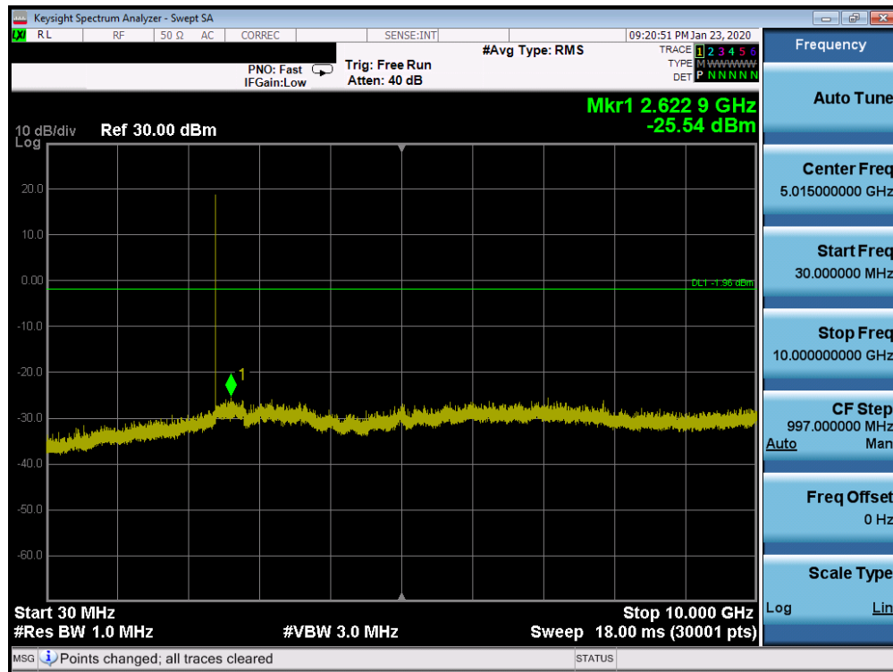
Plot 7-51. Conducted Spurious Plot Ant 2a (Bluetooth, GFSK, ePA – Ch. 0)
