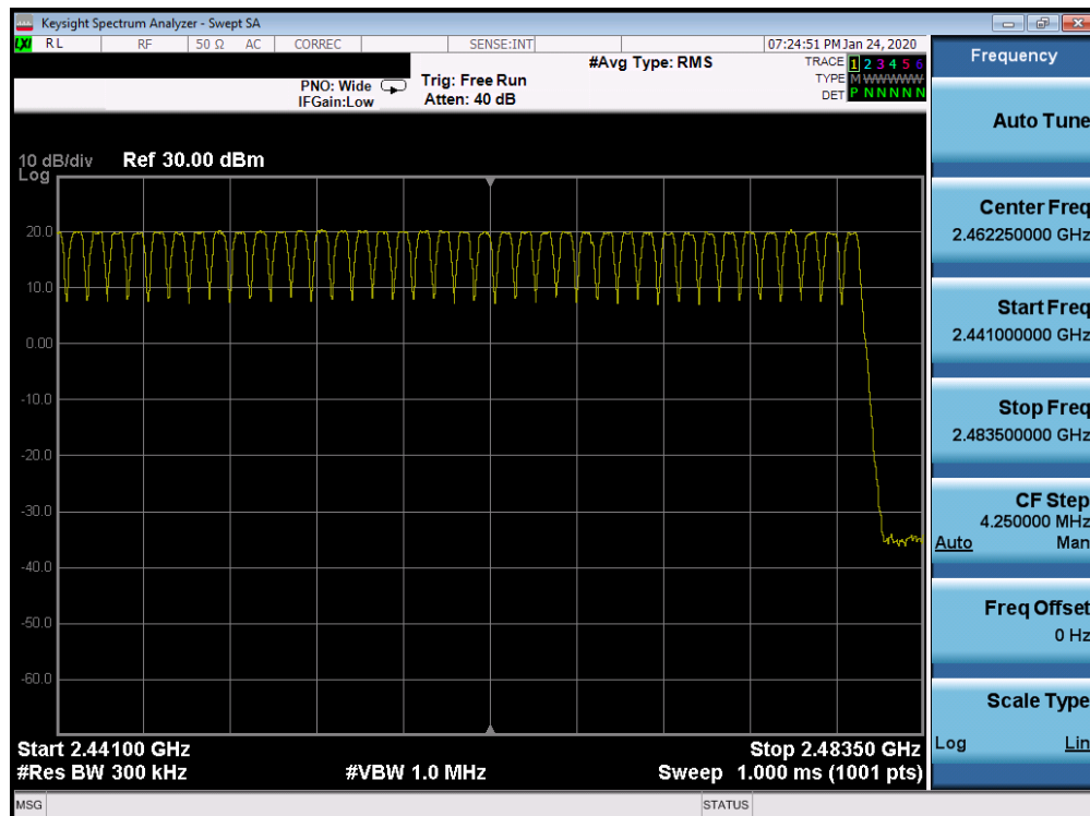
Plot 7-38. High End Spectrum Channel Hopping Plot Ant 4a (Bluetooth, GFSK, ePA)
