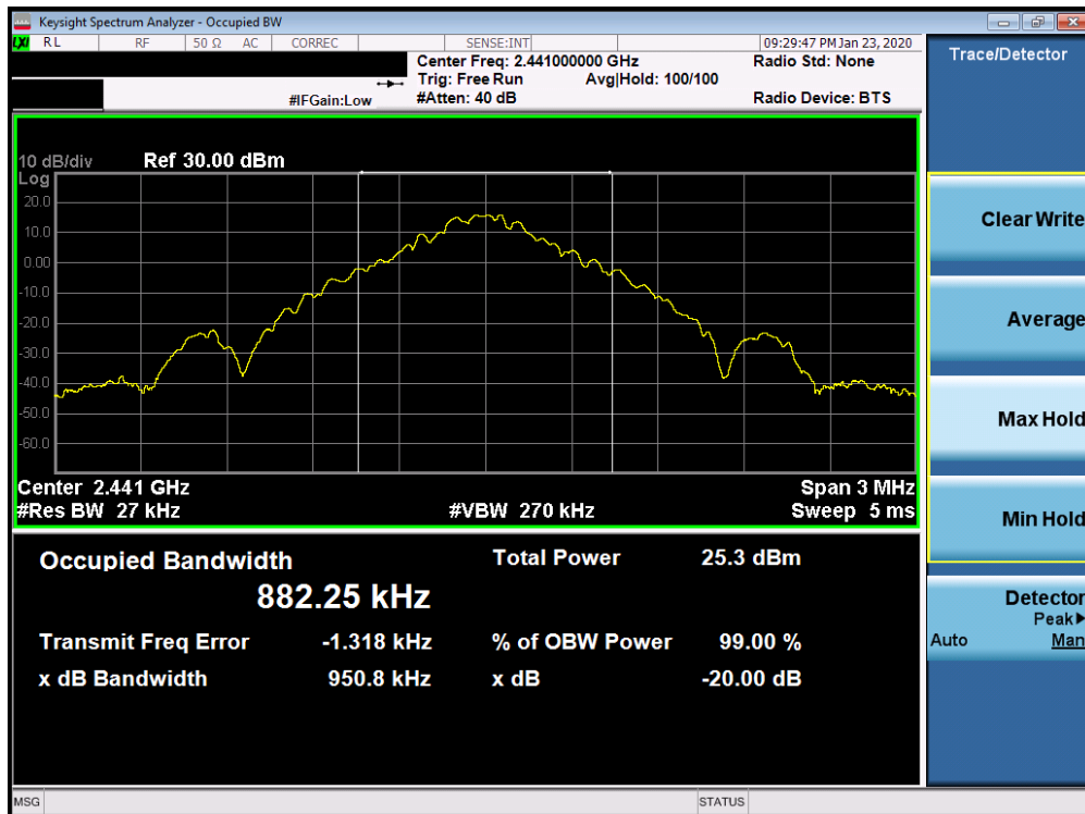
Plot 7-8. 20dB Bandwidth Plot Ant 2a (Bluetooth, GFSK, ePA – Ch. 39)
