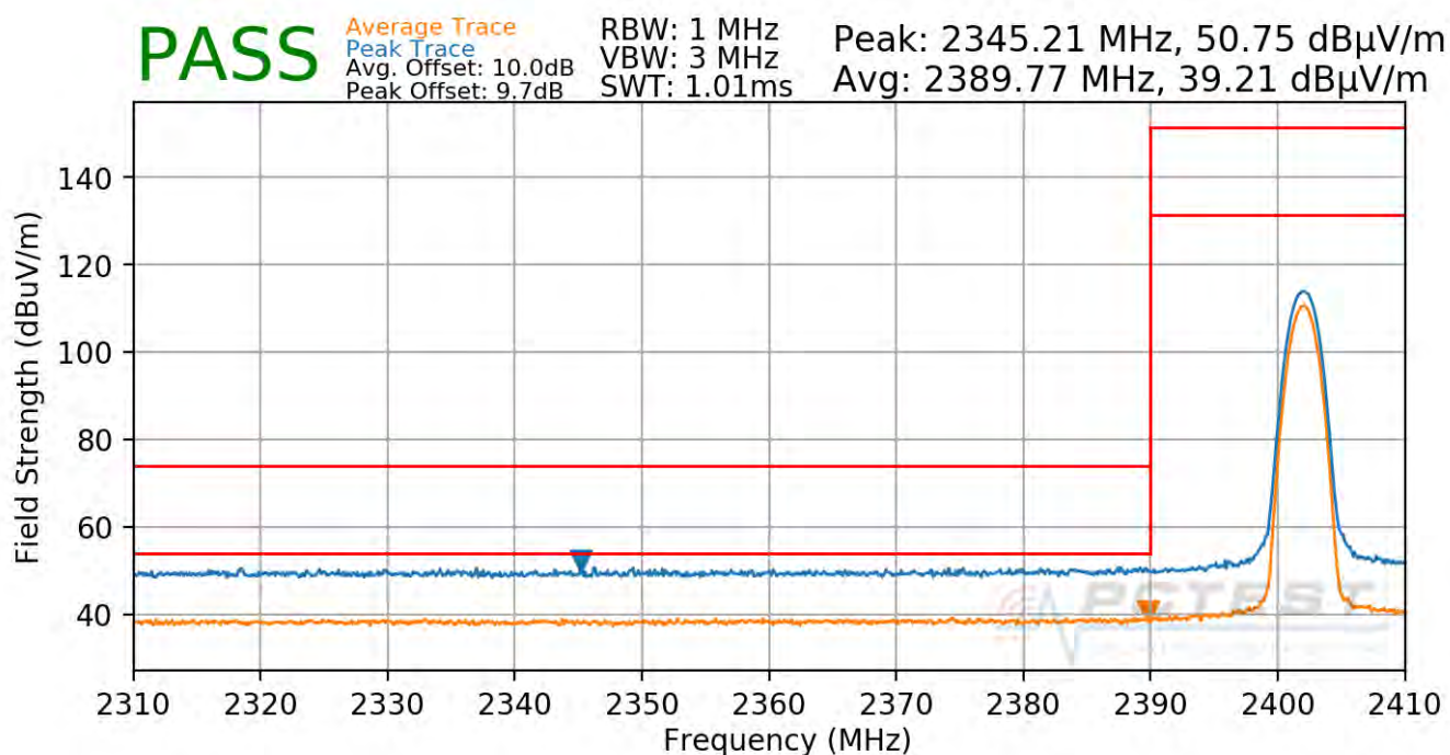
Plot 7-76. Radiated Restricted Lower Band Edge Measurement Ant 2a (Average & Peak)
