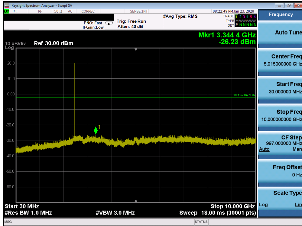
Plot 7-49. Conducted Spurious Plot Ant 4a (Bluetooth, GFSK, ePA – Ch. 78)
