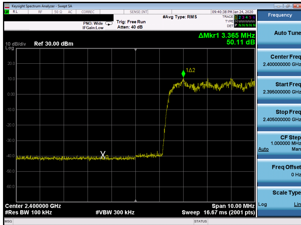
Plot 7-27. Band Edge Plot Ant 2a (Bluetooth with Hopping Enabled, 8DPSK, ePA)
