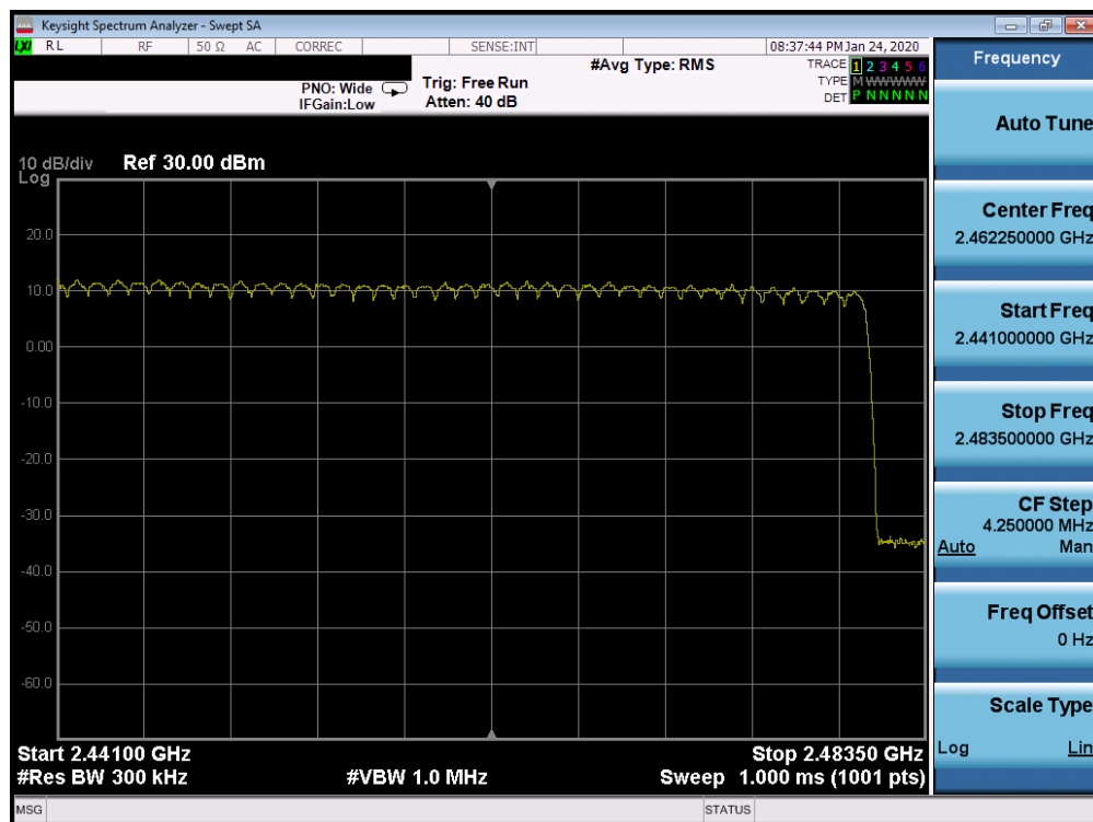
Plot 7-44. High End Spectrum Channel Hopping Plot Ant 2a (Bluetooth, 8DPSK, ePA)
