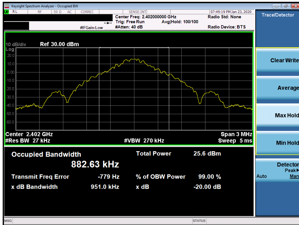
Plot 7-1. 20dB Bandwidth Plot Ant 4a (Bluetooth, GFSK, ePA – Ch. 0)
