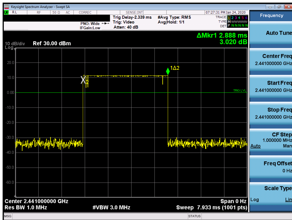
Plot 7-33. Time of Occupancy Plot Ant 4a (Bluetooth, GFSK, ePA)
