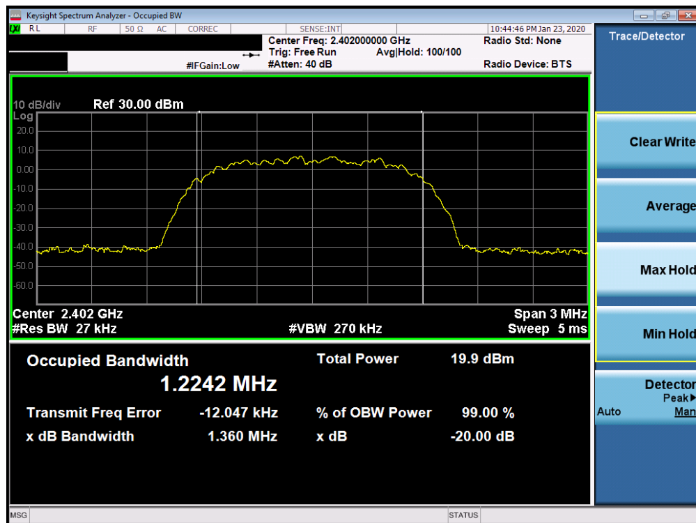
Plot 7-10. 20dB Bandwidth Plot Ant 2a (Bluetooth, 8DPSK, ePA – Ch. 0)
