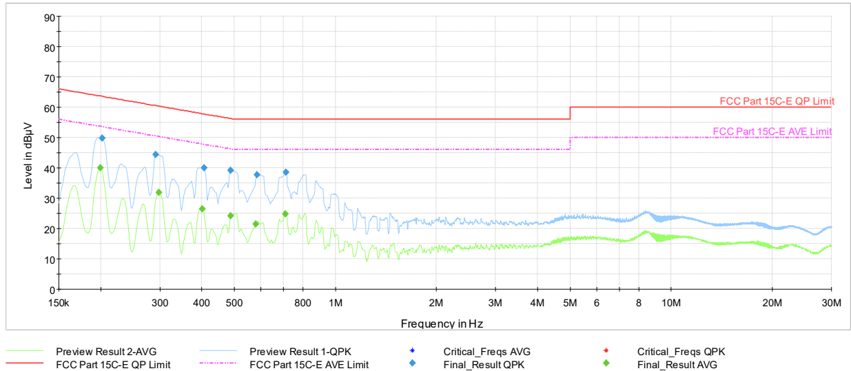
Plot 7-85. Line-Conducted Test Plot- Ch.39 TxBF (L1, with AC/DC Adapter)
