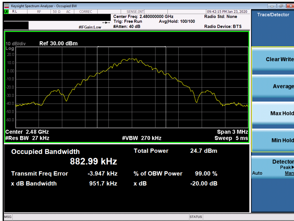
Plot 7-9. 20dB Bandwidth Plot Ant 2a (Bluetooth, GFSK, ePA – Ch. 78)
