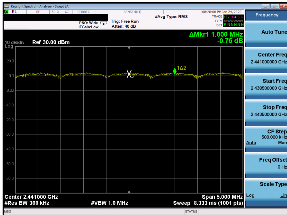
Plot 7-32. Channel Spacing Plot Ant 2a (Bluetooth, 8DPSK, ePA)
