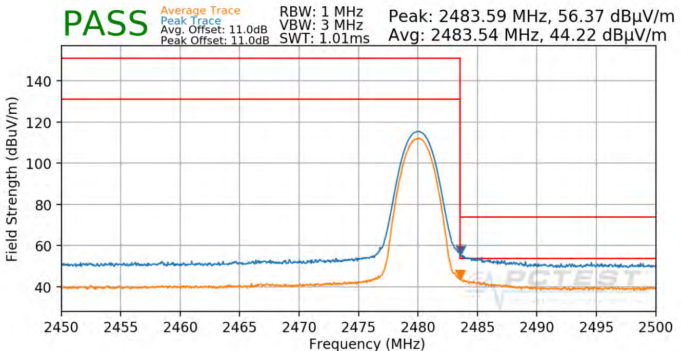
Plot 7-74. Radiated Restricted Upper Band Edge Measurement Ant 4a (Average & Peak)
