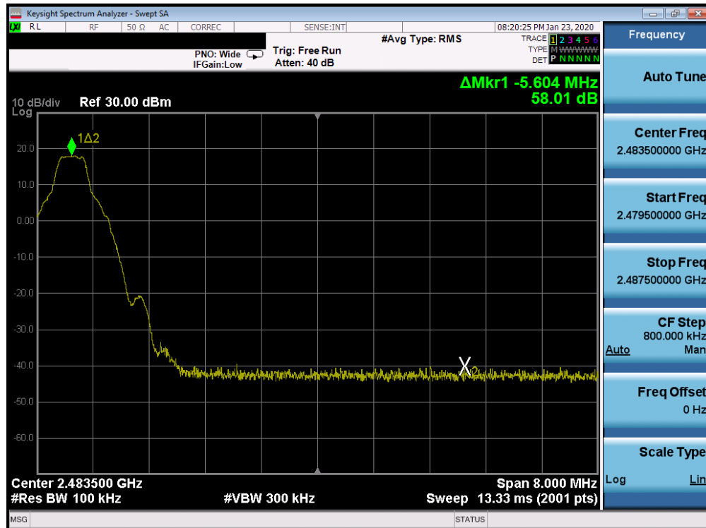
Plot 7-14. Band Edge Plot Ant 4a (Bluetooth with Hopping Disabled, GFSK, ePA – Ch. 78)
