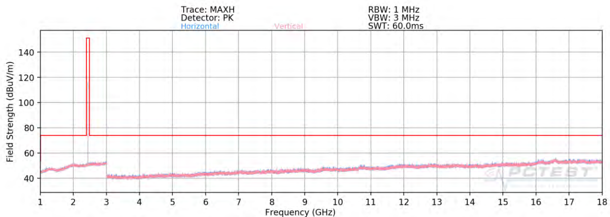
Plot 7-61. Radiated Spurious Plot above 1GHz Ant 2a (BT GFSK ePA – Ch. 39)
