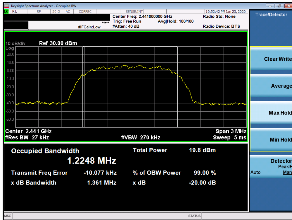
Plot 7-11. 20dB Bandwidth Plot Ant 2a (Bluetooth, 8DPSK, ePA – Ch. 39)
