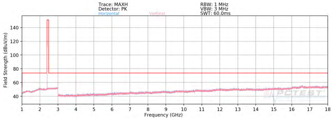
Plot 7-60. Radiated Spurious Plot above 1GHz Ant 2a (BT GFSK ePA – Ch. 0)
