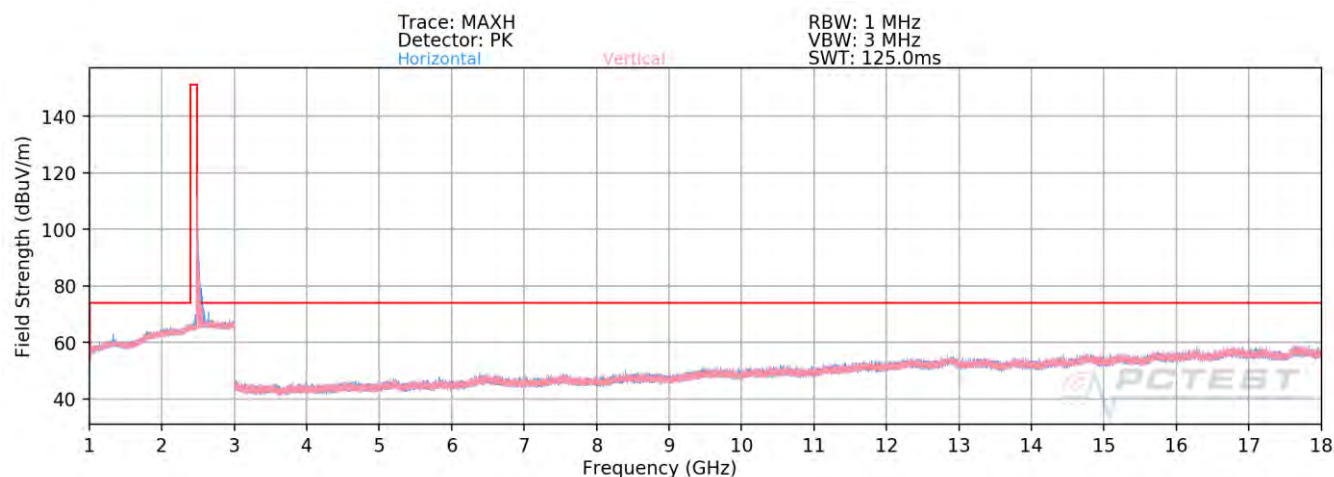
Plot 7-68. Radiated Spurious Plot above 1GHz Simultaneous Tx
