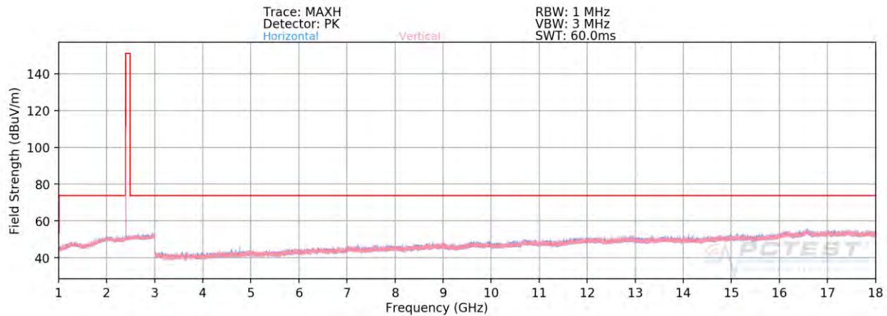
Plot 7-57. Radiated Spurious Plot above 1GHz Ant 4a (BT GFSK ePA – Ch. 0)
