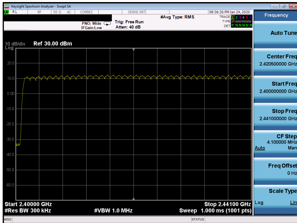
Plot 7-43. Low End Spectrum Channel Hopping Plot Ant 2a (Bluetooth, 8DPSK, ePA)
