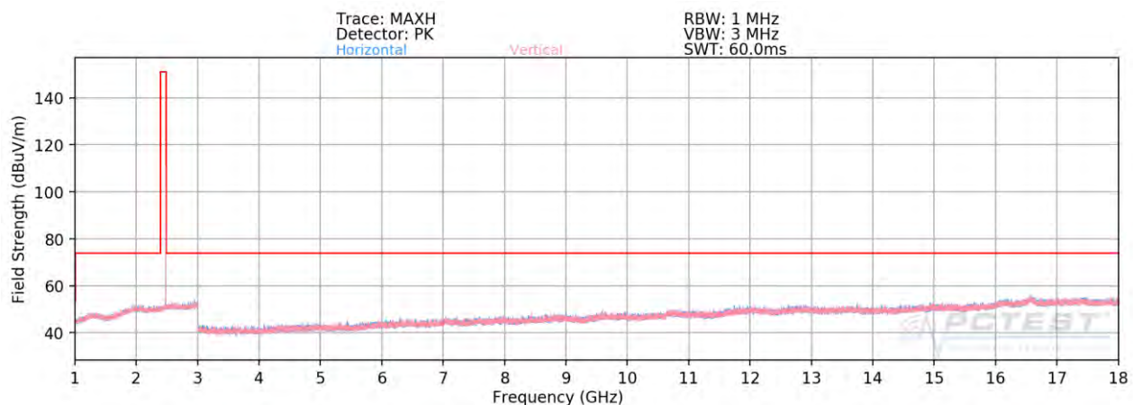
Plot 7-62. Radiated Spurious Plot above 1GHz Ant 2a (BT GFSK ePA – Ch. 78)
