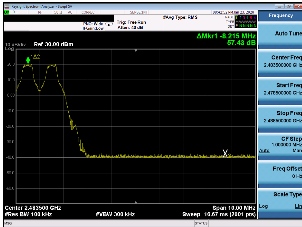
Plot 7-16. Band Edge Plot Ant 4a (Bluetooth with Hopping Enabled, GFSK, ePA)
