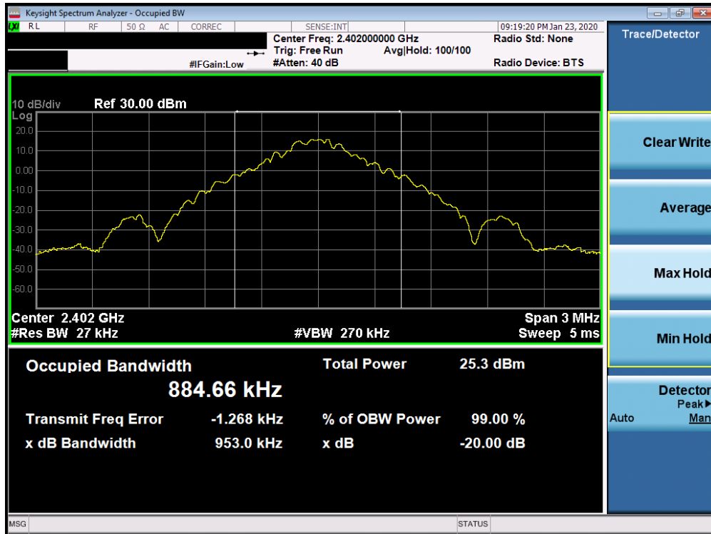
Plot 7-7. 20dB Bandwidth Plot Ant 2a (Bluetooth, GFSK, ePA – Ch. 0)
