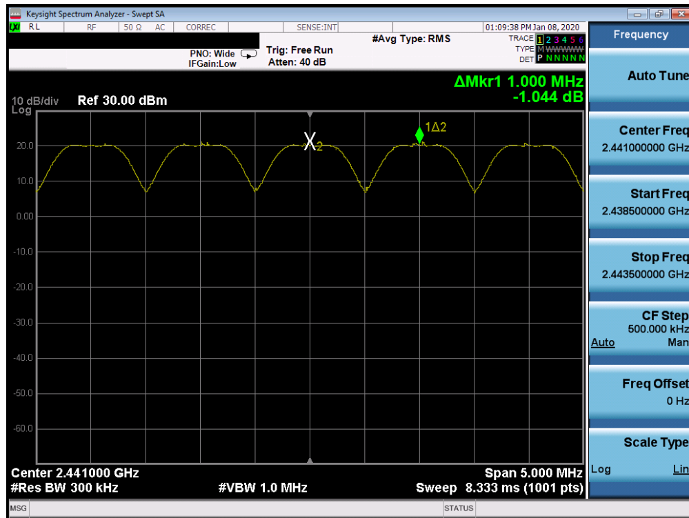
Plot 7-31. Channel Spacing Plot Ant 2a (Bluetooth, GFSK, ePA)
