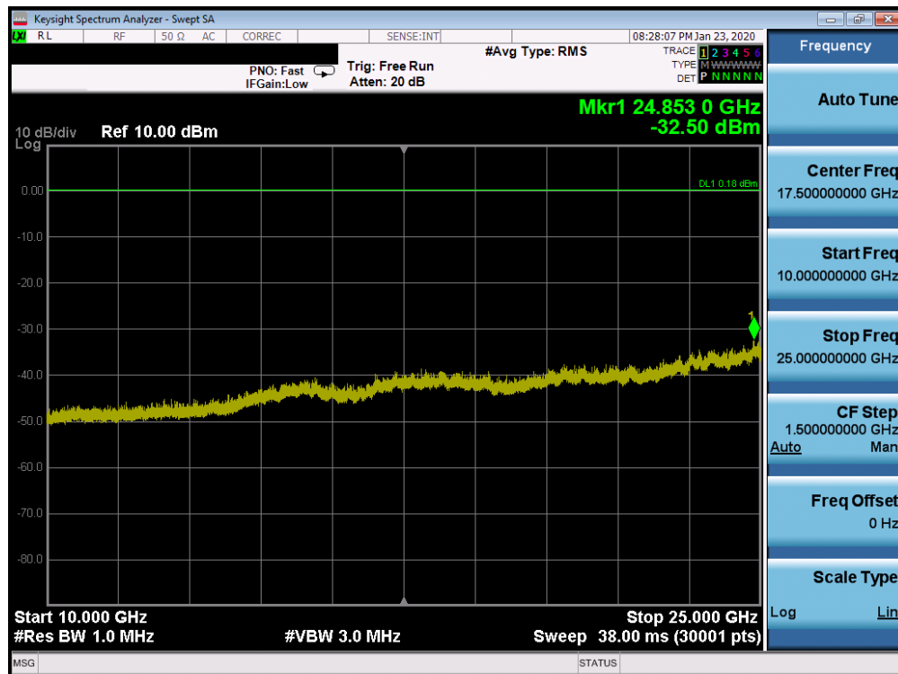
Plot 7-46. Conducted Spurious Plot Ant 4a (Bluetooth, GFSK, ePA – Ch. 0)
