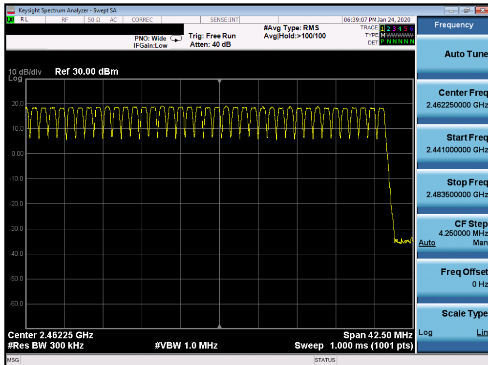
Plot 7-42. High End Spectrum Channel Hopping Plot Ant 2a (Bluetooth, GFSK, ePA)
