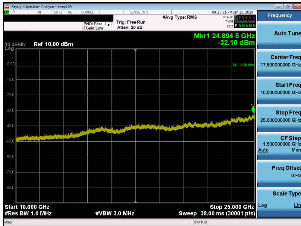
Plot 7-52. Conducted Spurious Plot Ant 2a (Bluetooth, GFSK, ePA – Ch. 0)
