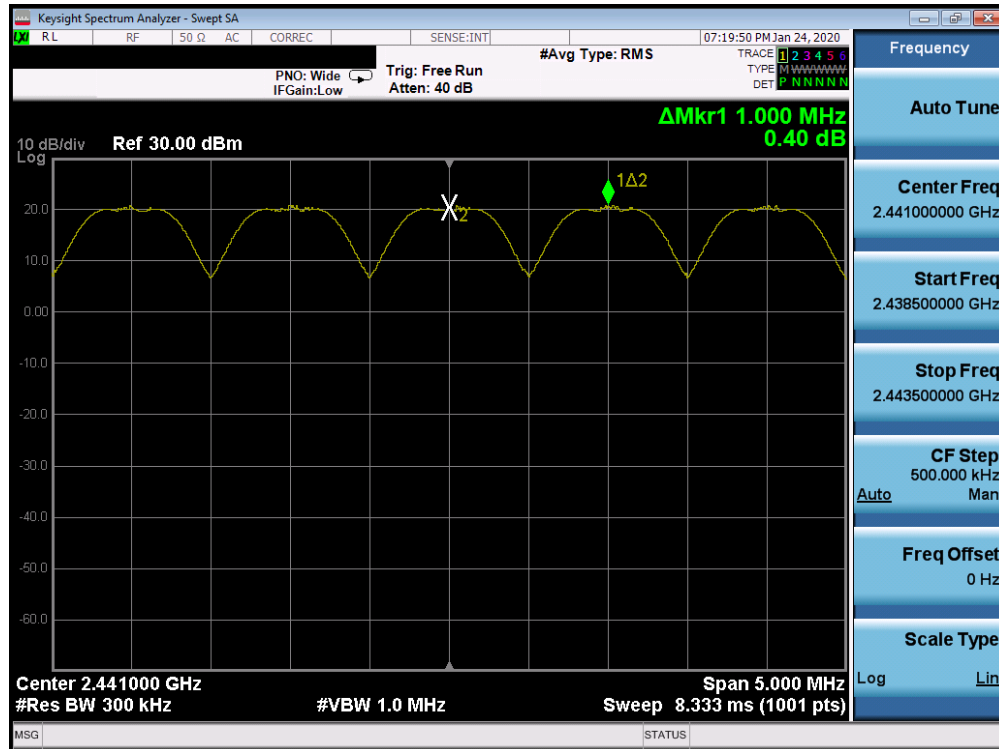
Plot 7-29. Channel Spacing Plot Ant 4a (Bluetooth, GFSK, ePA)
