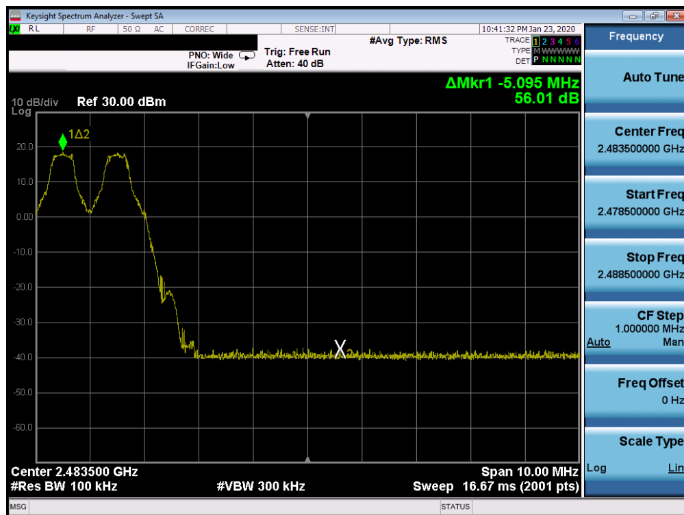
Plot 7-24. Band Edge Plot Ant 2a (Bluetooth with Hopping Enabled, GFSK, ePA)
