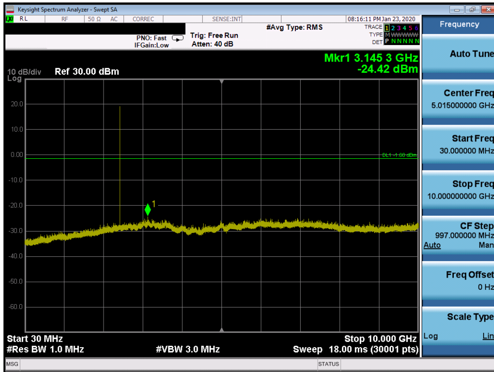
Plot 7-47. Conducted Spurious Plot Ant 4a (Bluetooth, GFSK, ePA – Ch. 39)
