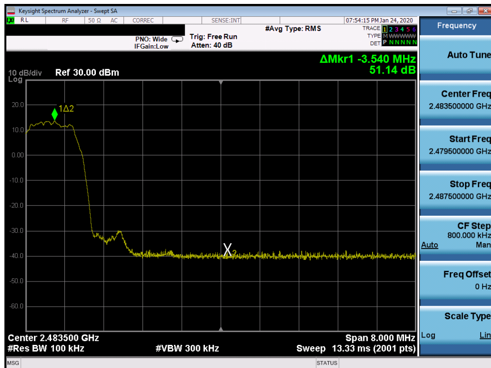
Plot 7-18. Band Edge Plot Ant 4a (Bluetooth with Hopping Disabled, 8DPSK, ePA – Ch. 78)
