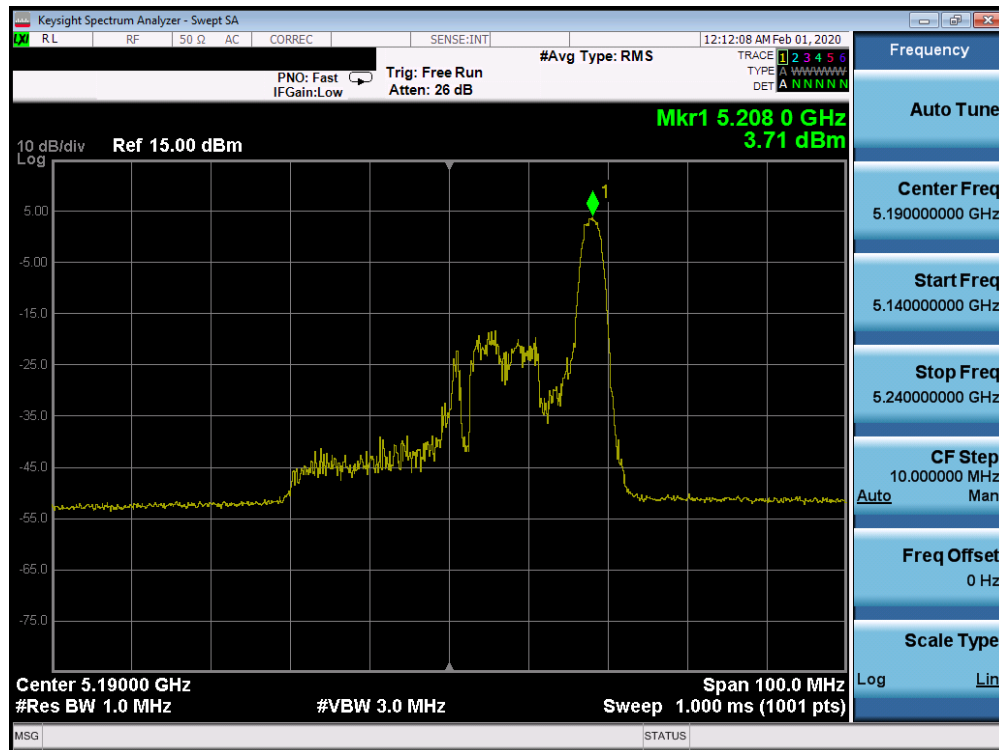
Plot 7-431. Power Spectral Density Plot ISD SISO CORE 1 (40MHz BW 802.11ax Index 17 – RU26 (UNII Band 1) – Ch. 38)
