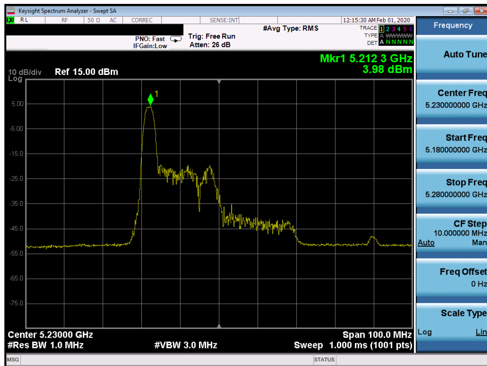
Plot 7-432. Power Spectral Density Plot ISD SISO CORE 1 (40MHz BW 802.11ax Index 0 – RU26 (UNII Band 1) – Ch. 46)
