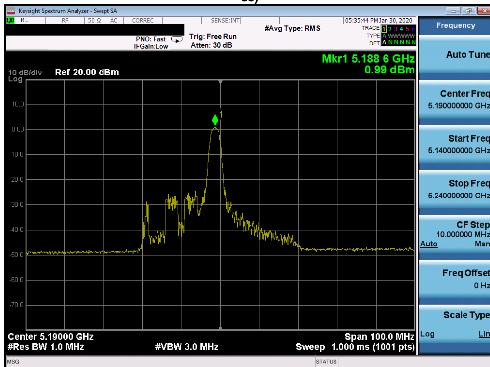
Plot 7-652. Power Spectral Density Plot ISCED CDD CORE 1 (40MHz BW 802.11ax Index 8 – RU26 (UNII Band 1) – Ch. 38)
