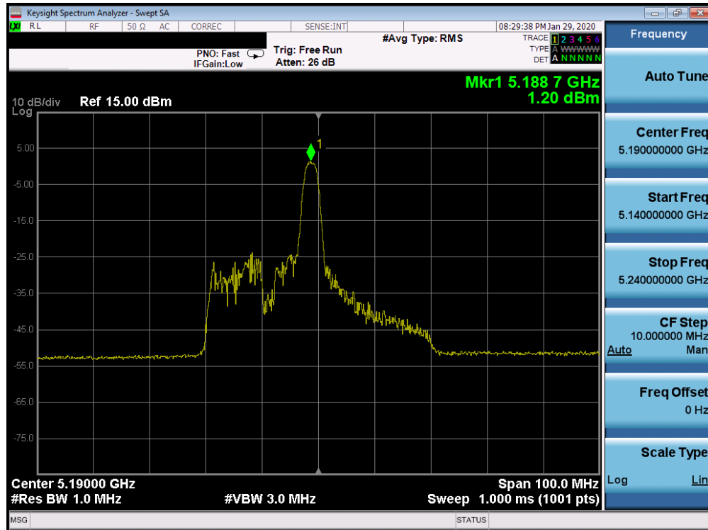
Plot 7-651. Power Spectral Density Plot ISCED CDD CORE 0 (40MHz BW 802.11ax Index 8 – RU26 (UNII Band 1) – Ch. 38)
