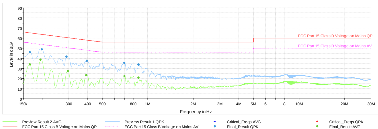
Plot 7-283. Line Conducted Plot with 802.11n UNII Band 1 – Ch.36 (N), with AC/DC Adapter)
