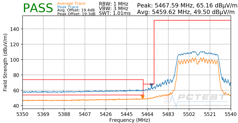
Plot 7-271. Radiated Lower Band Edge Plot CDD (UNII Band 2C)
