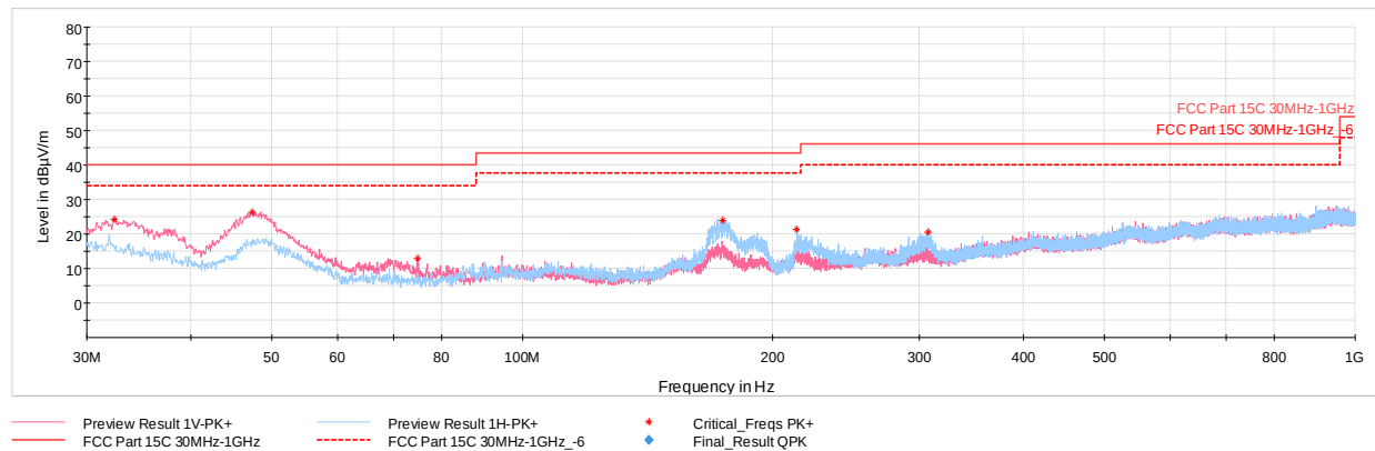
Plot 7-281. Radiated Spurious Plot below 1GHz CDD – Ch.36 with AC/DC Adapter
