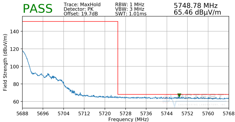
Plot 7-263. Radiated Upper Band Edge Plot CDD (Peak – UNII Band 2C)
