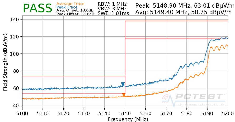
Plot 7-257. Radiated Lower Band Edge Plot CDD (UNII Band 1)
