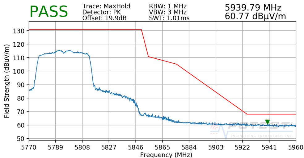
Plot 7-250. Radiated Upper Band Edge Plot SISO CORE1 (Peak – UNII Band 3)
