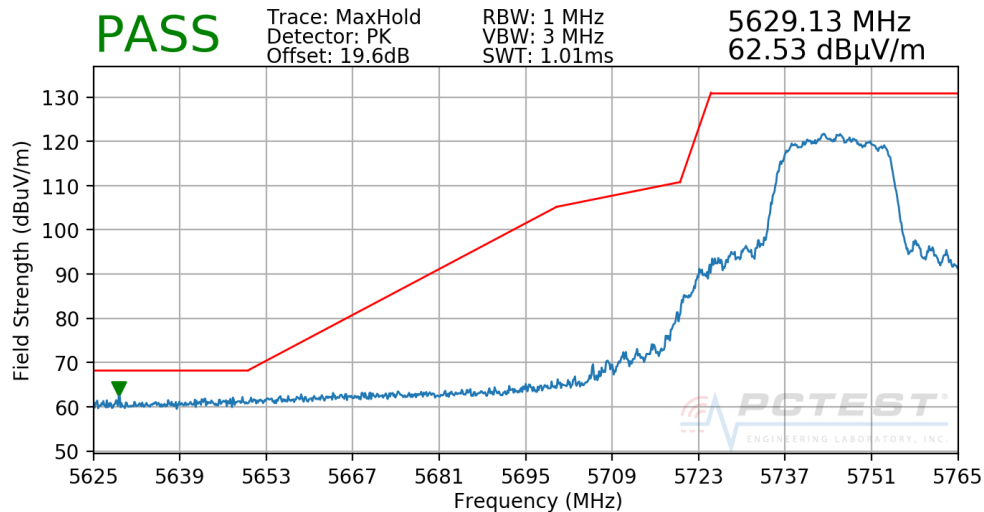
Plot 7-265. Radiated Lower Band Edge Plot CDD (Peak – UNII Band 3)
