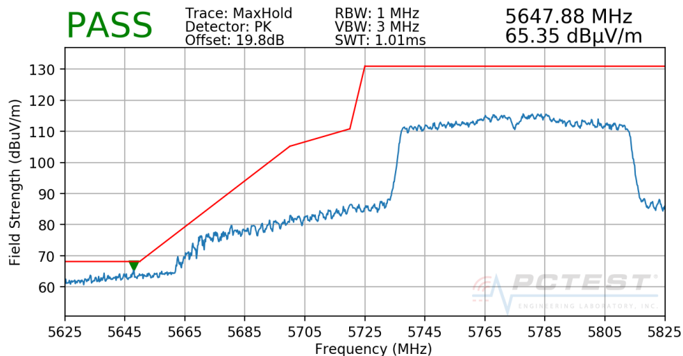
Plot 7-279. Radiated Lower Band Edge Plot CDD (Peak - UNII Band 3)
