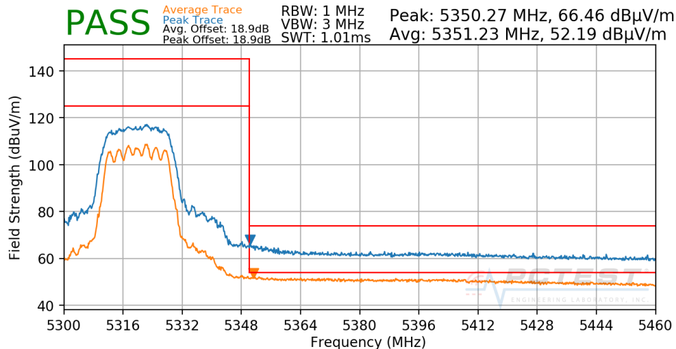
Plot 7-259. Radiated Upper Band Edge Plot CDD (UNII Band 2A)
