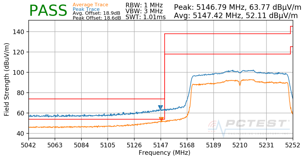
Plot 7-251. Radiated Lower Band Edge Plot SISO CORE1 (UNII Band 1)
