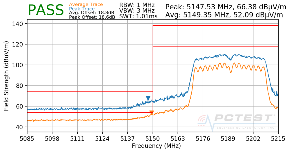
Plot 7-267. Radiated Lower Band Edge Plot CDD (UNII Band 1)
