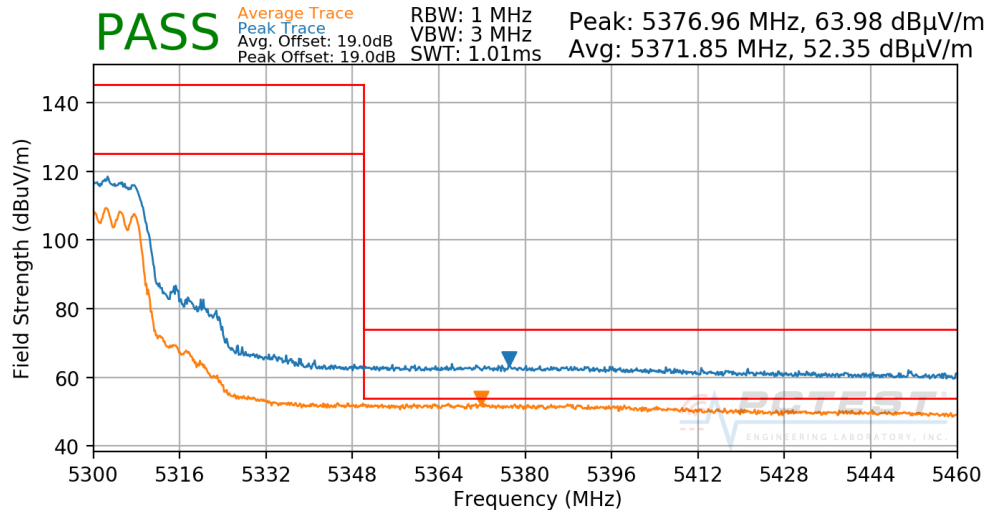
Plot 7-258. Radiated Upper Band Edge Plot CDD (UNII Band 2A)
