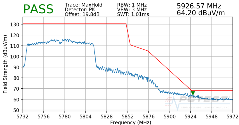
Plot 7-280. Radiated Upper Band Edge Plot CDD (Peak – UNII Band 3)
