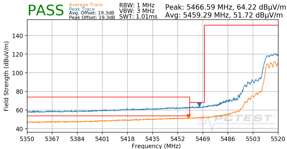
Plot 7-261. Radiated Lower Band Edge Plot CDD (Peak – UNII Band 2C)
