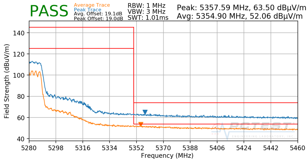
Plot 7-269. Radiated Upper Band Edge Plot CDD (UNII Band 2A)
