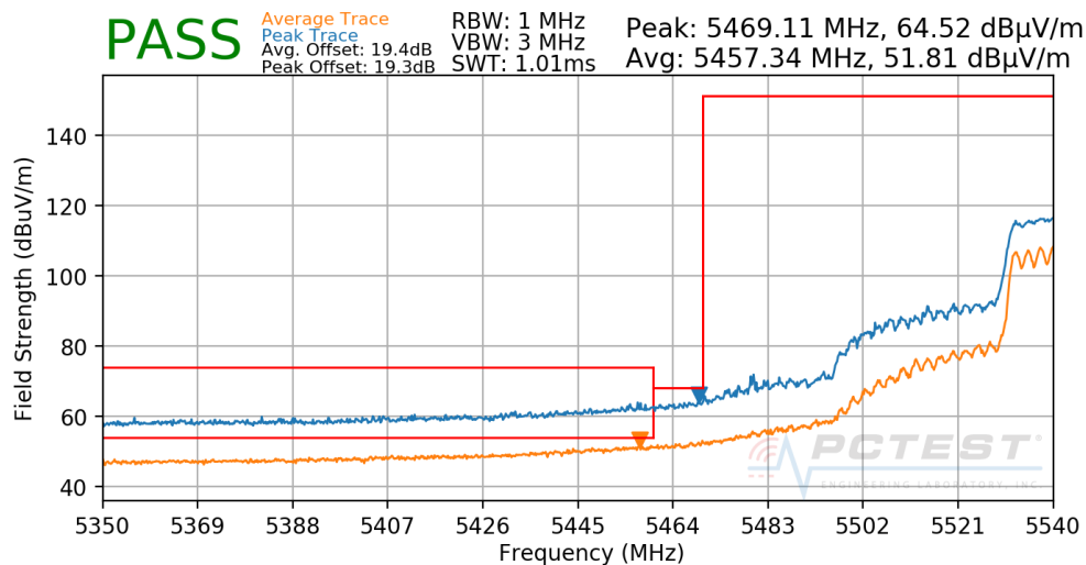
Plot 7-272. Radiated Lower Band Edge Plot CDD (Peak - UNII Band 2C)
