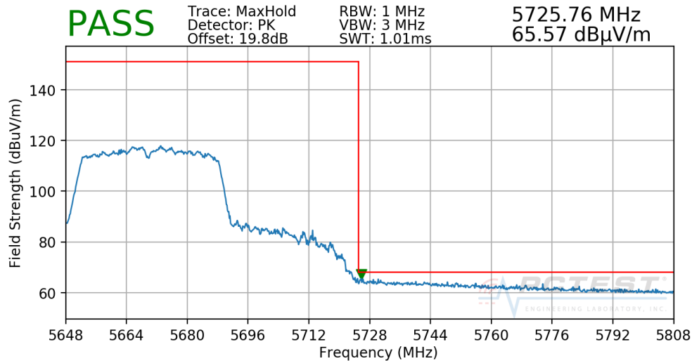
Plot 7-273. Radiated Upper Band Edge Plot CDD (Peak - UNII Band 2C)
