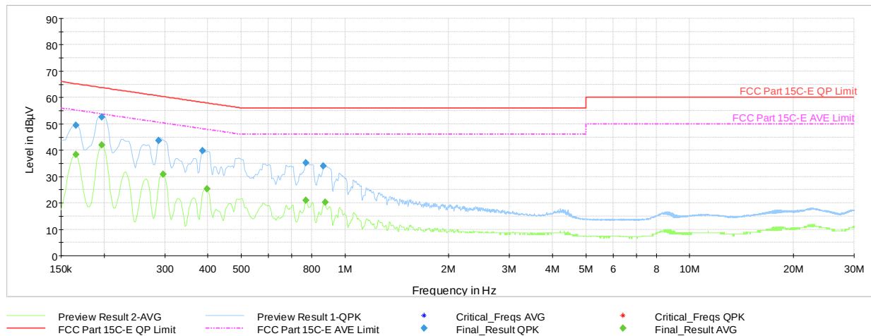
Plot 7-282. Line Conducted Plot with 802.11n UNII Band 1 – Ch.36 (L1), with AC/DC Adapter
