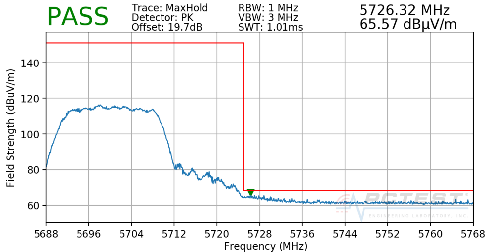
Plot 7-264. Radiated Upper Band Edge Plot CDD (Peak – UNII Band 2C)
