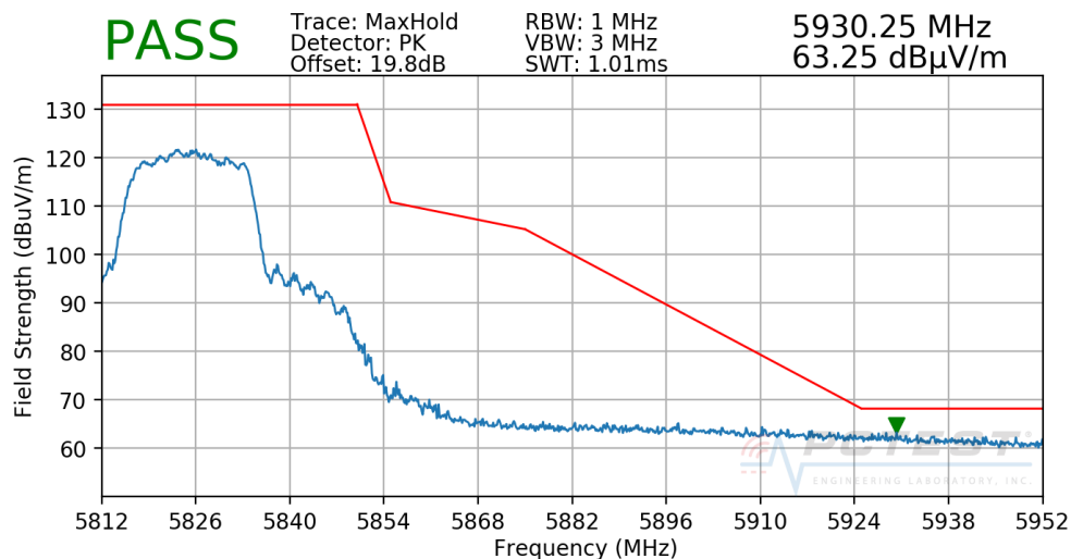
Plot 7-266. Radiated Upper Band Edge Plot CDD (Peak – UNII Band 3)
