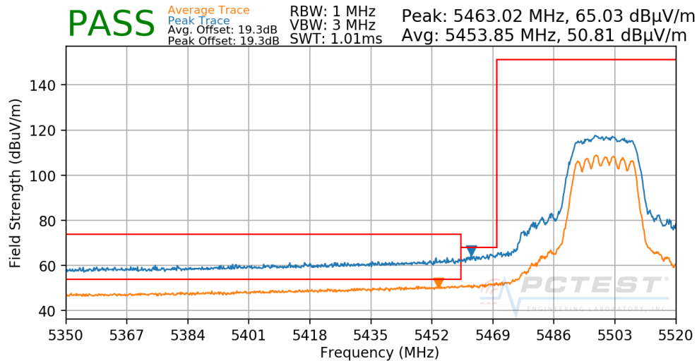
Plot 7-260. Radiated Lower Band Edge Plot CDD (UNII Band 2C)
