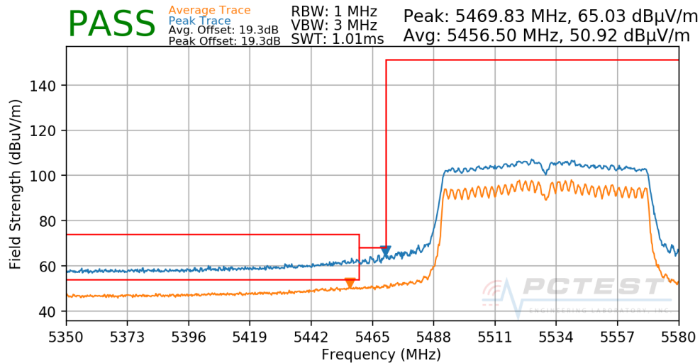
Plot 7-278. Radiated Lower Band Edge Plot CDD (UNII Band 2C)
