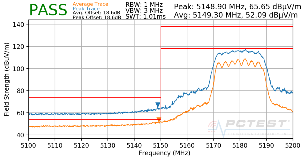
Plot 7-256. Radiated Lower Band Edge Plot CDD (UNII Band 1)
