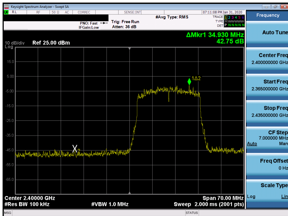
Plot 7-82. Band Edge SISO CORE 1 (802.11ax OFDMA – RU242 – Ch. 1)
