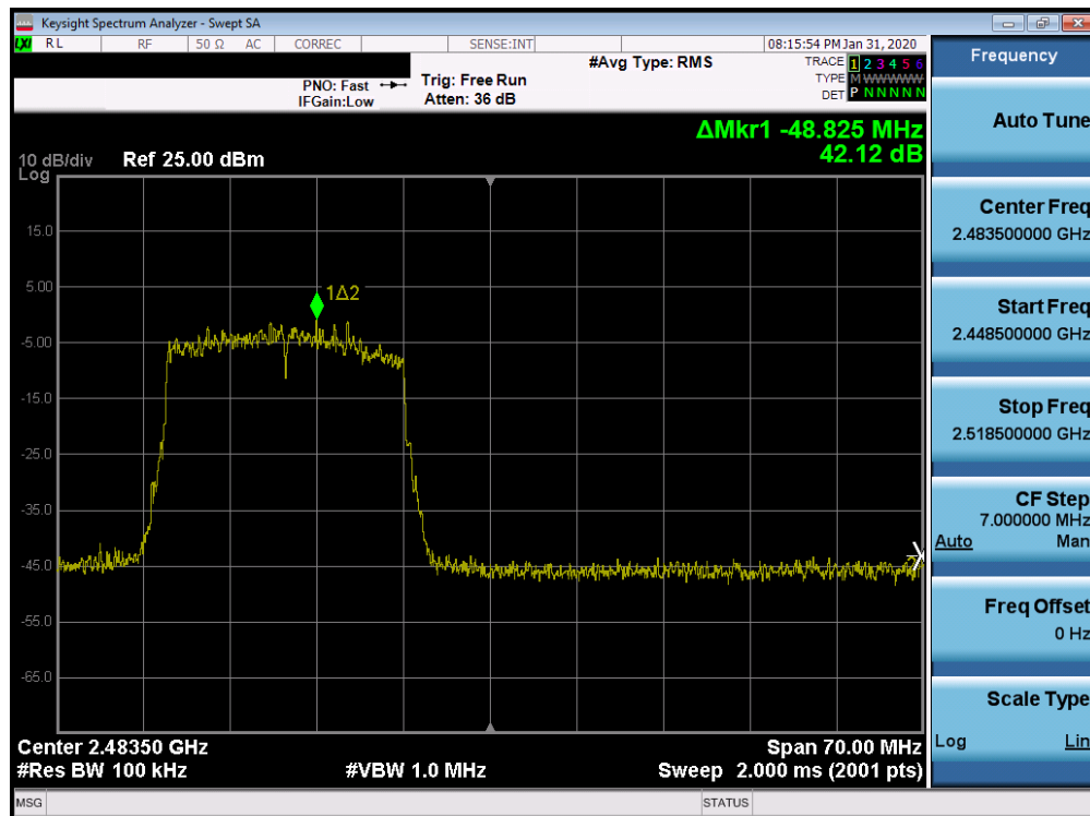
Plot 7-78. Band Edge SISO CORE 0 (802.11ax OFDMA – RU242 – Ch. 12)
