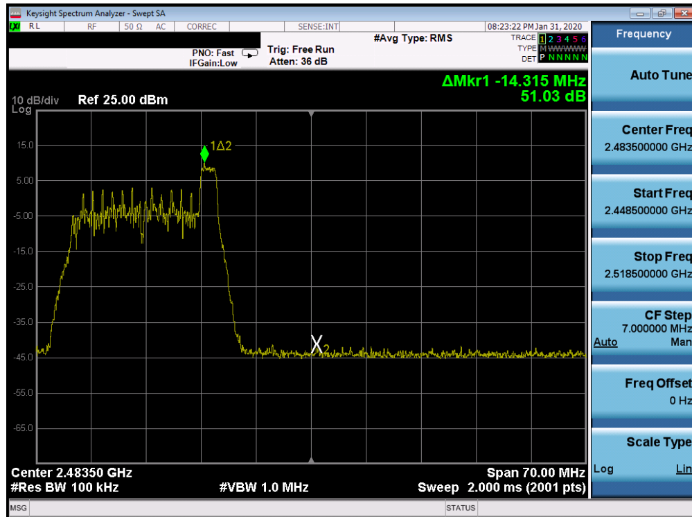
Plot 7-74. Band Edge SISO CORE 0 (802.11ax OFDMA – RU26 Index 8 – Ch. 11)
