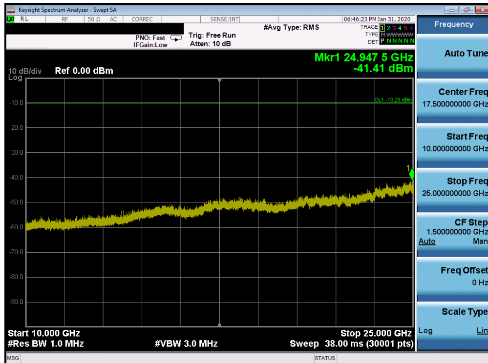
Plot 7-86. Conducted Spurious Plot SISO CORE 0 (802.11ax OFDMA – RU26 – Ch. 1)
