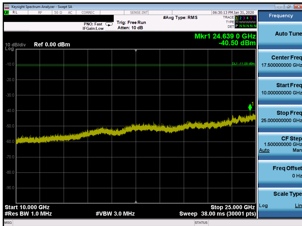
Plot 7-88. Conducted Spurious Plot SISO CORE 0 (802.11ax OFDMA – RU26 – Ch. 6)
