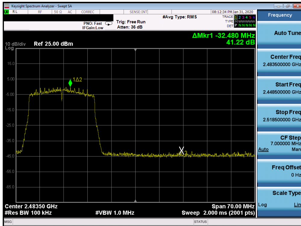
Plot 7-83. Band Edge SISO CORE 1 (802.11ax OFDMA – RU242 – Ch. 11)
