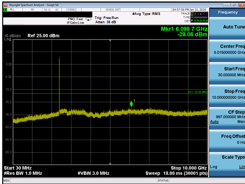
Plot 7-91. Conducted Spurious Plot SISO CORE 0 (802.11ax OFDMA – RU242 – Ch. 1)
