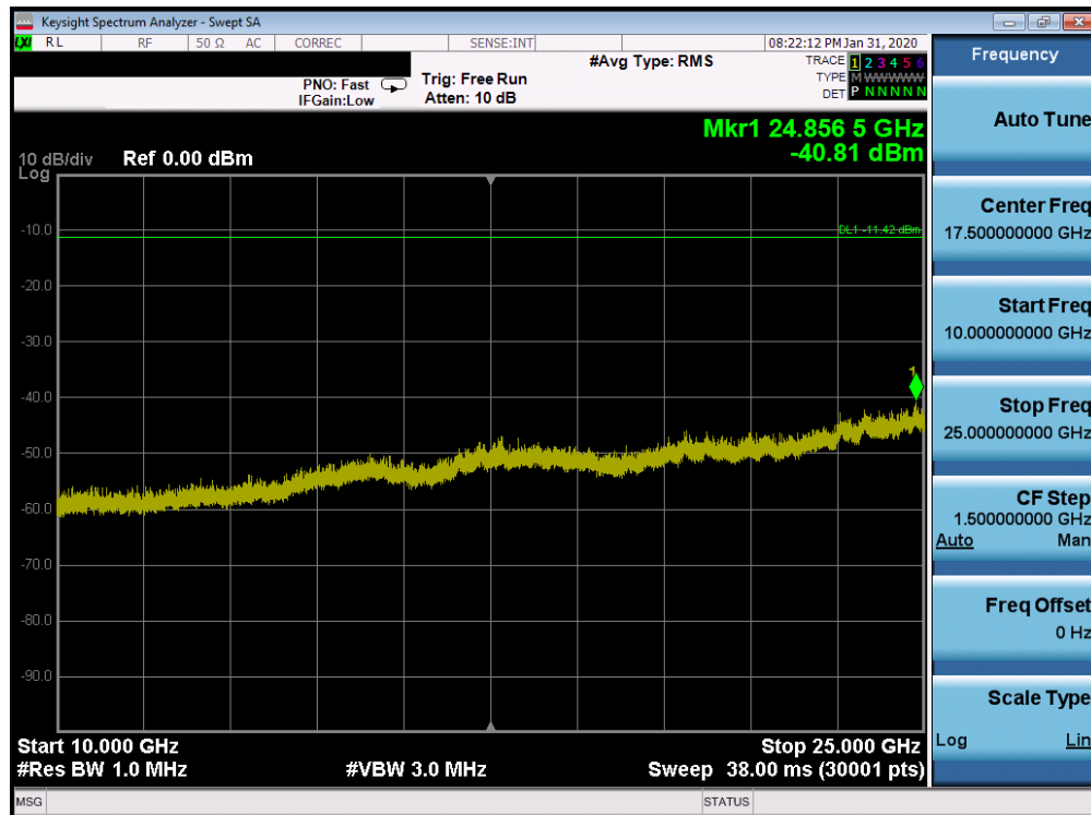
Plot 7-90. Conducted Spurious Plot SISO CORE 0 (802.11ax OFDMA – RU26 – Ch. 11)
