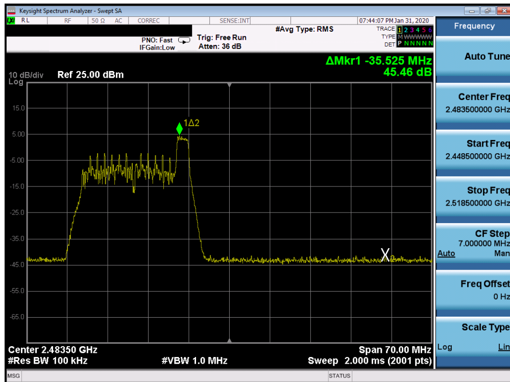
Plot 7-81. Band Edge SISO CORE 1 (802.11ax OFDMA – RU26 Index 8 – Ch. 12)
