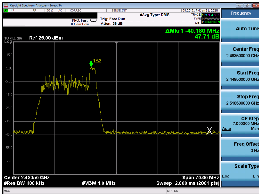
Plot 7-75. Band Edge SISO CORE 0 (802.11ax OFDMA – RU26 Index 8 – Ch. 12)
