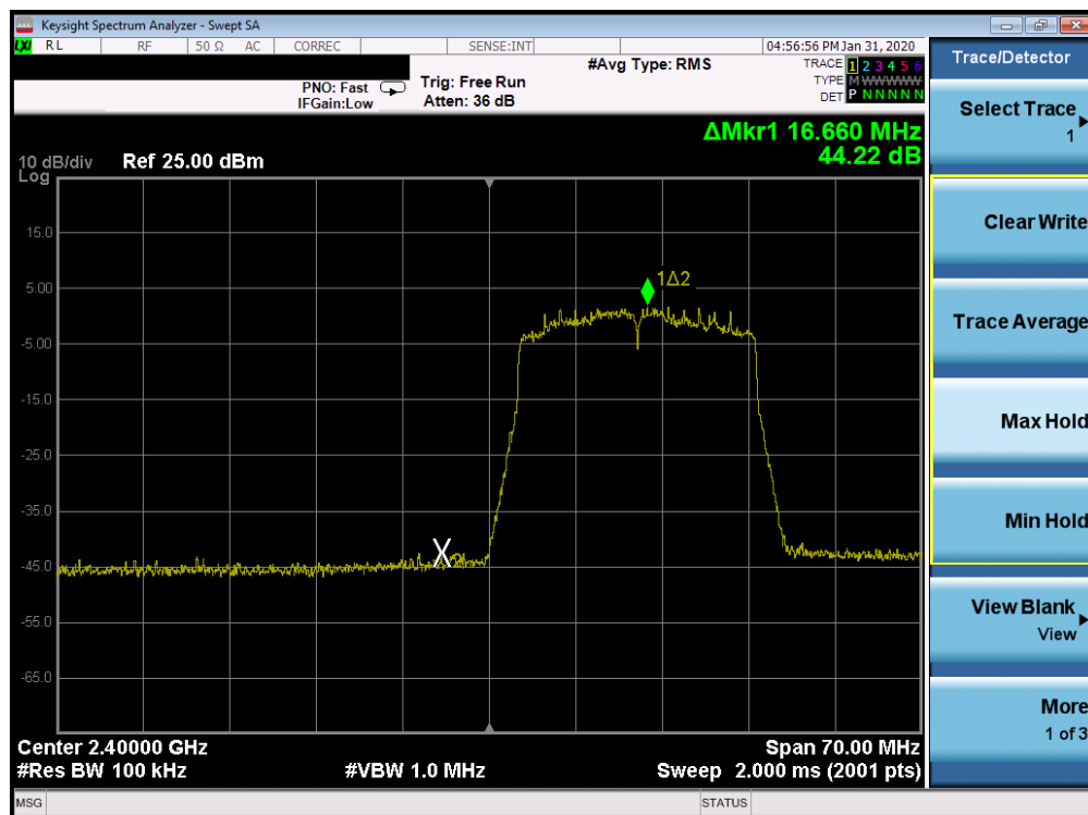
Plot 7-76. Band Edge SISO CORE 0 (802.11ax OFDMA – RU242 – Ch. 1)
