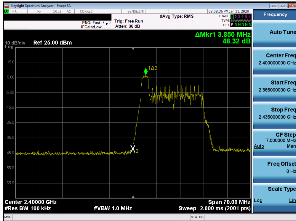
Plot 7-79. Band Edge SISO CORE 1 (802.11ax OFDMA – RU26 Index 0 – Ch. 1)
