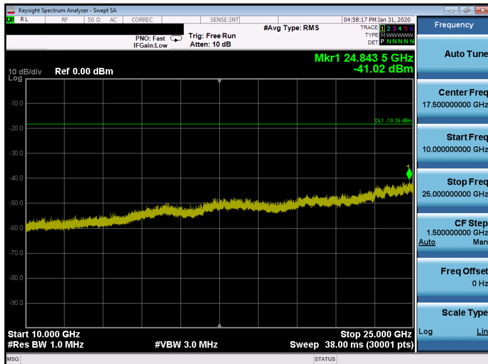
Plot 7-92. Conducted Spurious Plot SISO CORE 0 (802.11ax OFDMA – RU242 – Ch. 1)
