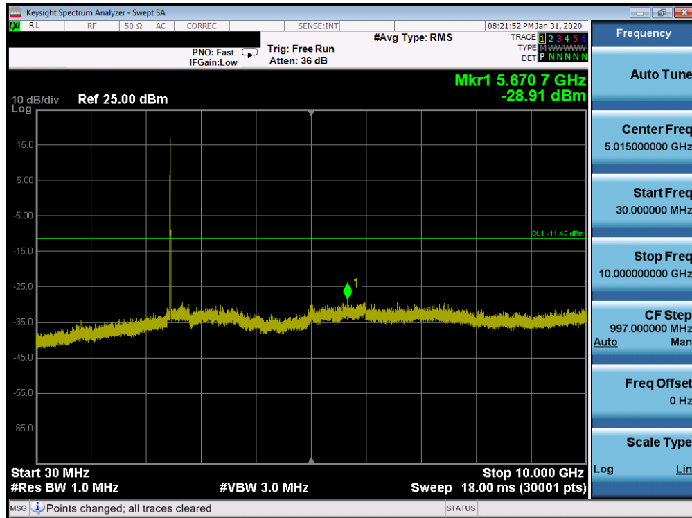
Plot 7-89. Conducted Spurious Plot SISO CORE 0 (802.11ax OFDMA – RU26 – Ch. 11)
