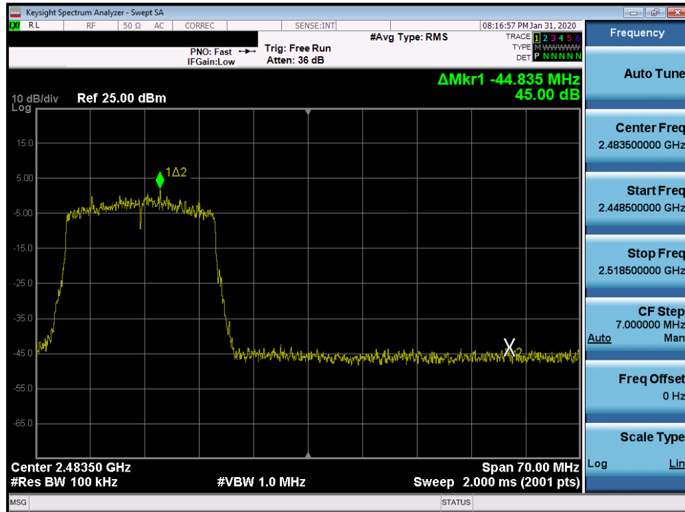
Plot 7-77. Band Edge SISO CORE 0 (802.11ax OFDMA – RU242 – Ch. 11)
