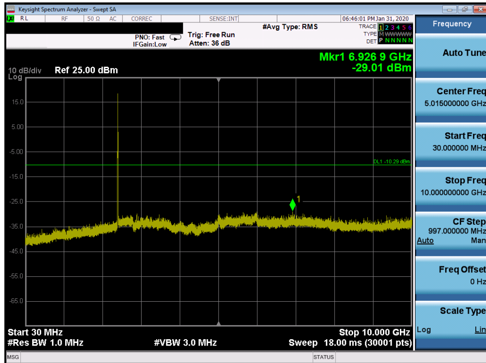
Plot 7-85. Conducted Spurious Plot SISO CORE 0 (802.11ax OFDMA – RU26 – Ch. 1)
