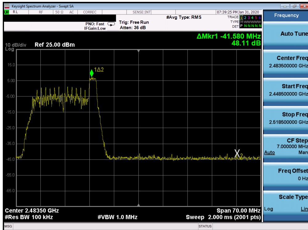
Plot 7-80. Band Edge SISO CORE 1 (802.11ax OFDMA – RU26 Index 8 – Ch. 11)
