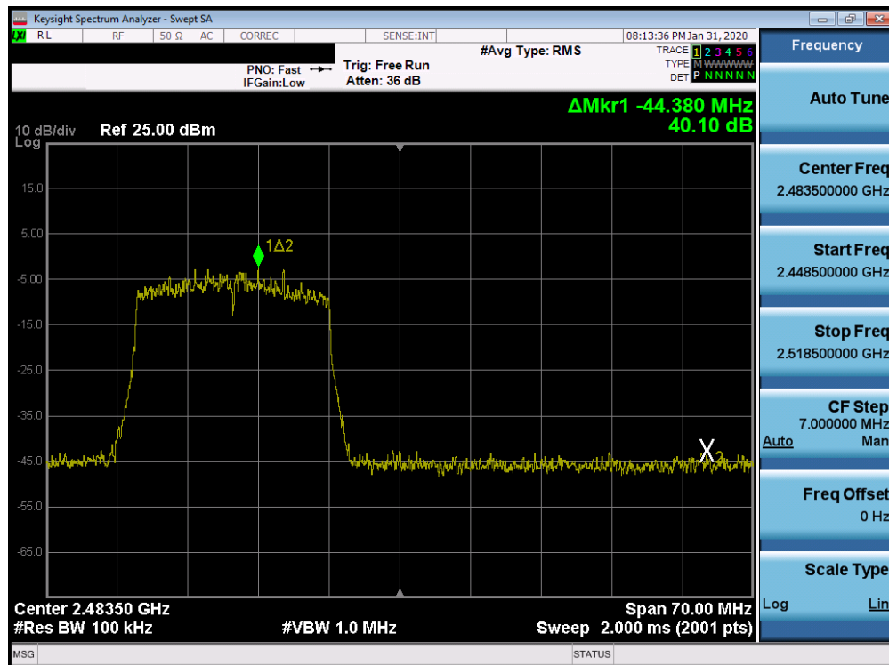
Plot 7-84. Band Edge SISO CORE 1 (802.11ax OFDMA – RU242 – Ch. 12)
