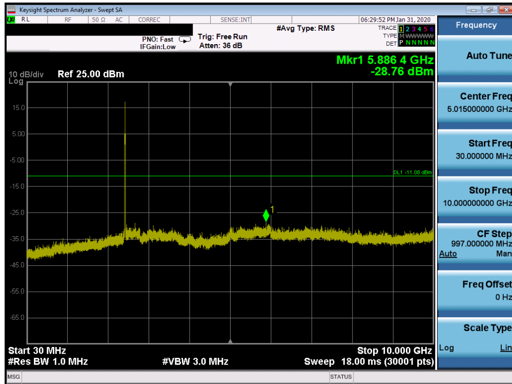
Plot 7-87. Conducted Spurious Plot SISO CORE 0 (802.11ax OFDMA – RU26 – Ch. 6)
