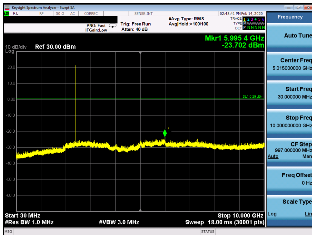
Plot 7-69. Conducted Spurious Plot Ant 4a (Bluetooth (LE), 1Mbps, ePA - Ch. 0)
