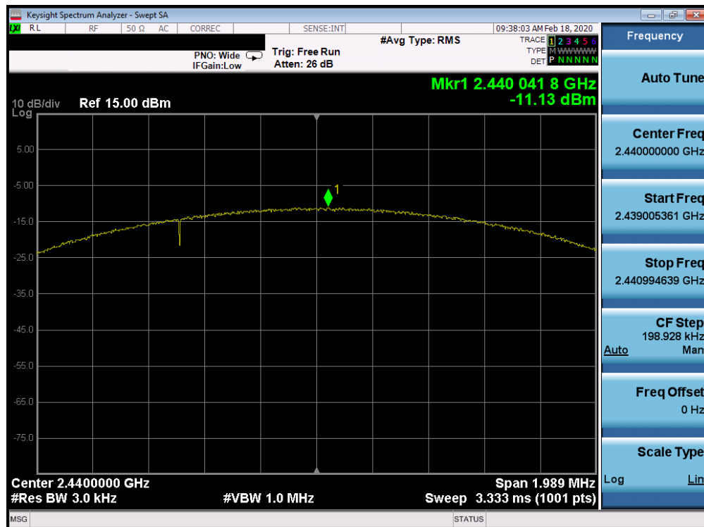
Plot 7-58. Power Spectral Density Plot TxBF Ant 2a (Bluetooth (LE), 2Mbps, iPA – Ch. 19)
