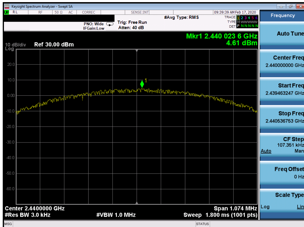
Plot 7-14. Power Spectral Density Plot Ant 4a (Bluetooth (LE), 1Mbps, ePA – Ch. 19)
