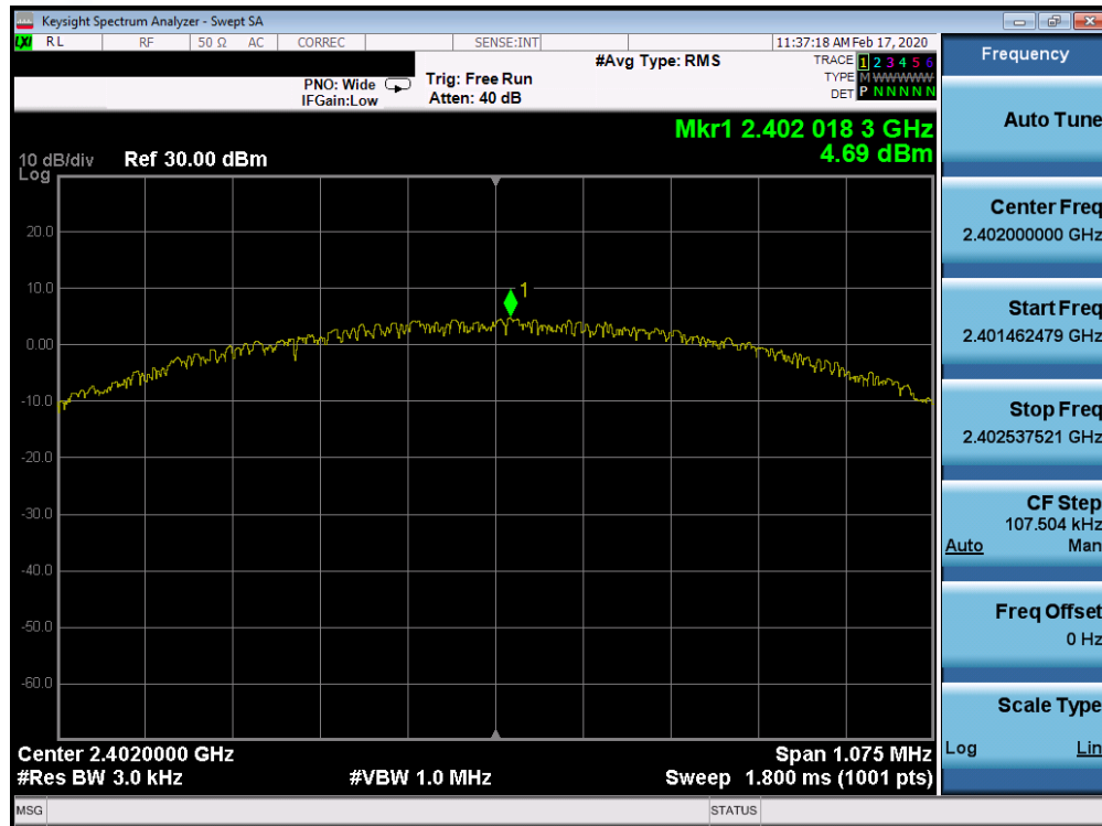
Plot 7-37. Power Spectral Density Plot TxBF Ant 4a (Bluetooth (LE), 1Mbps, ePA – Ch. 0)
