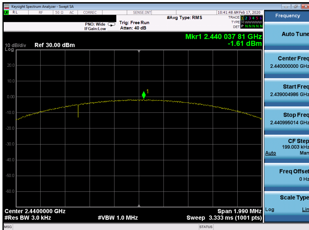
Plot 7-32. Power Spectral Density Plot Ant 2a (Bluetooth (LE), 2Mbps, ePA – Ch. 19)
