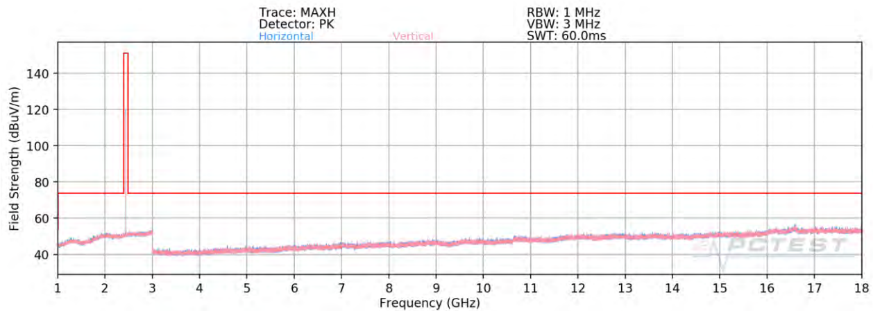
Plot 7-82. Radiated Spurious Plot Above 1GHz Ant 4a (1Mbps, ePA – Ch. 19)
