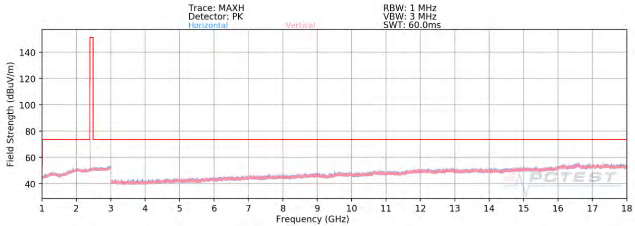
Plot 7-81. Radiated Spurious Plot Above 1GHz Ant 4a (1Mbps, ePA – Ch. 0)
