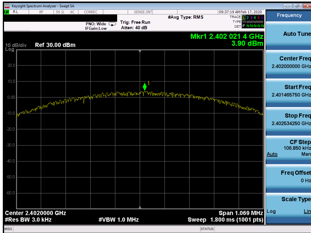
Plot 7-13. Power Spectral Density Plot Ant 4a (Bluetooth (LE), 1Mbps, ePA – Ch. 0)
