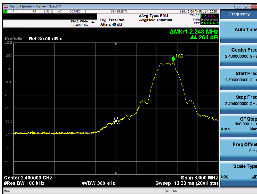
Plot 7-65. Band Edge Plot Ant 2a (Bluetooth (LE), 1Mbps ePA – Ch. 0)
