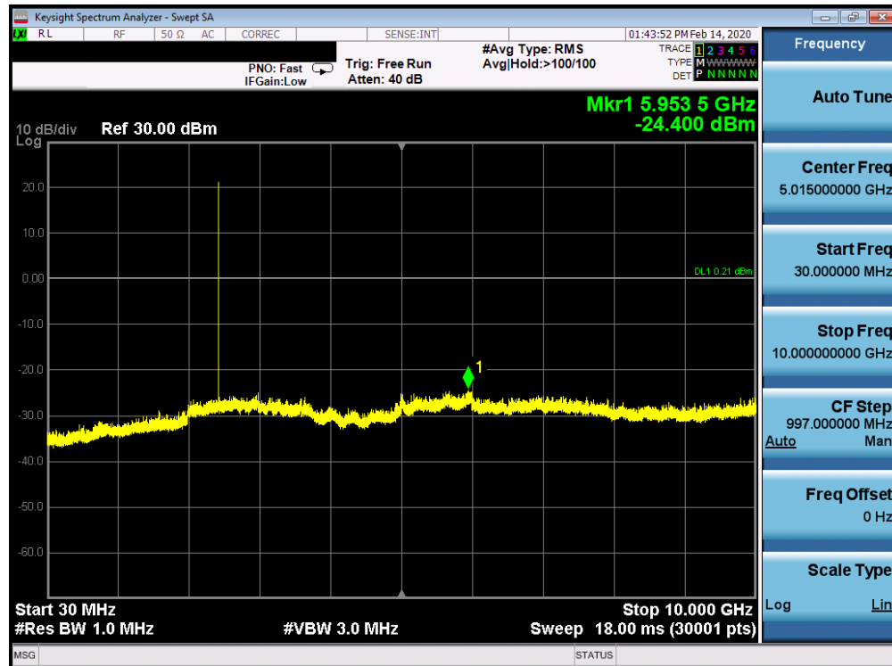
Plot 7-77. Conducted Spurious Plot Ant 2a (Bluetooth (LE), 1Mbps, ePA – Ch. 19)
