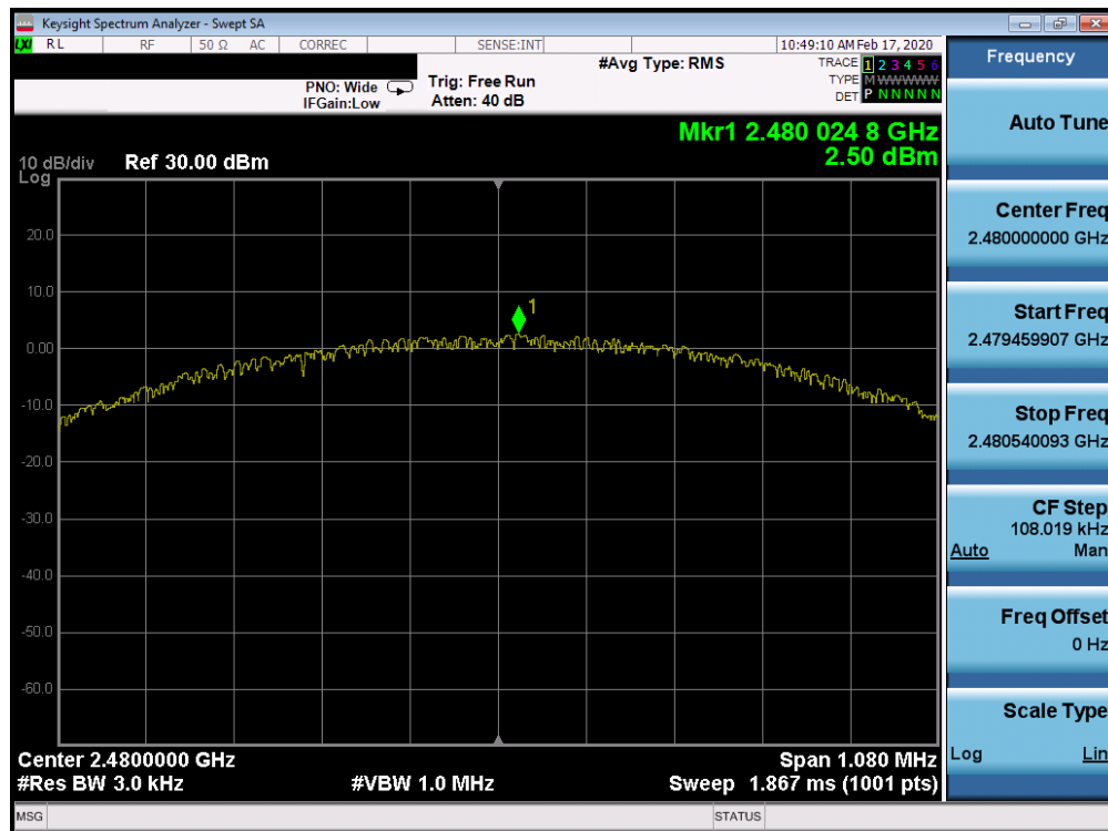
Plot 7-27. Power Spectral Density Plot Ant 2a (Bluetooth (LE), 1Mbps, ePA – Ch. 39)
