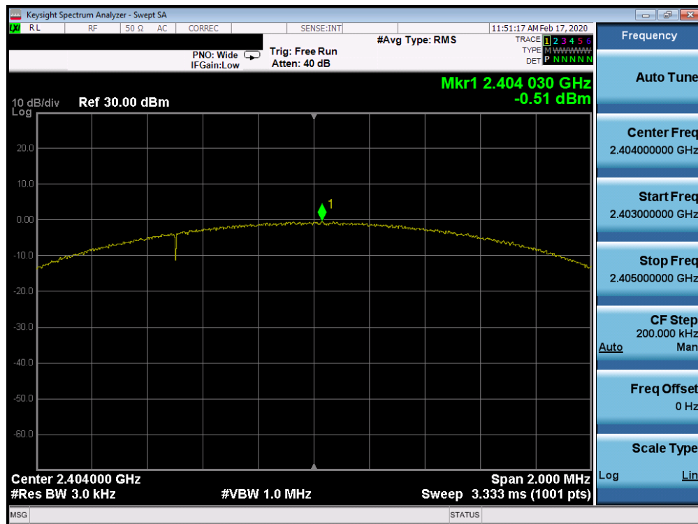
Plot 7-49. Power Spectral Density Plot Tx BF Ant 4a (Bluetooth (LE), 2Mbps, ePA – Ch. 1)
