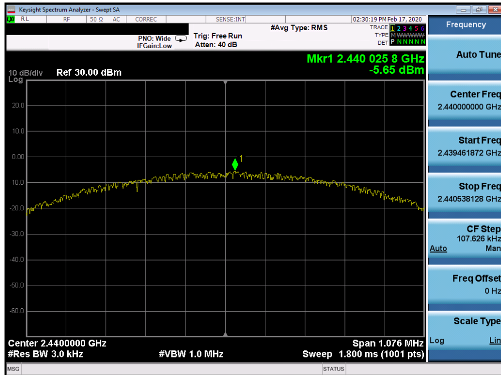
Plot 7-17. Power Spectral Density Plot Ant 4a (Bluetooth (LE), 1Mbps, iPA – Ch. 19)
