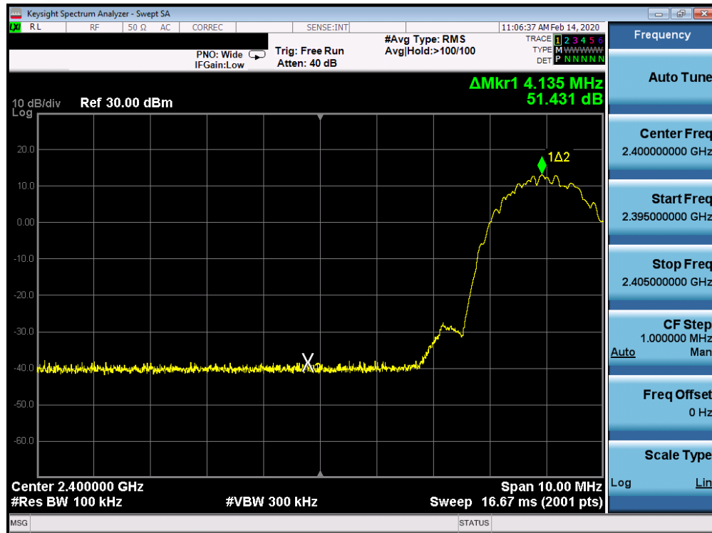
Plot 7-67. Band Edge Plot Ant 2a (Bluetooth (LE), 2Mbps ePA – Ch. 1)
