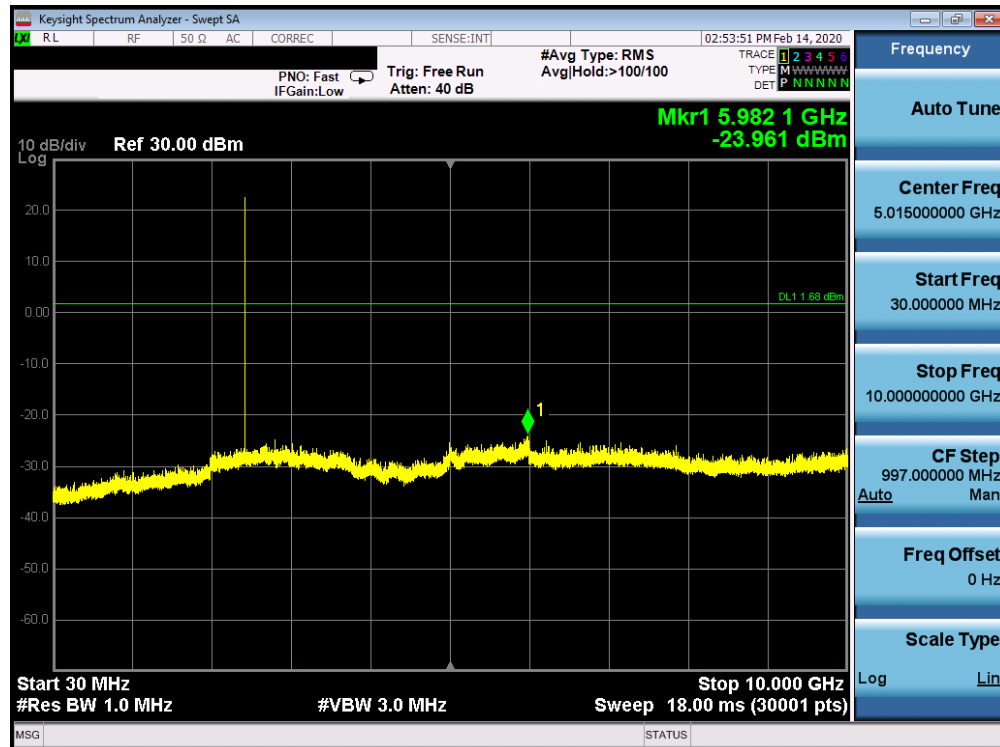
Plot 7-71. Conducted Spurious Plot Ant 4a (Bluetooth (LE), 1Mbps, ePA – Ch. 19)
