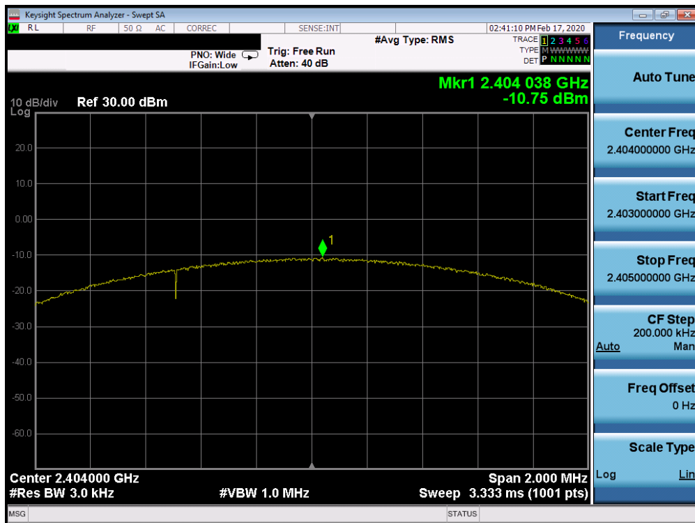
Plot 7-22. Power Spectral Density Plot Ant 4a (Bluetooth (LE), 2Mbps, iPA – Ch. 1)
