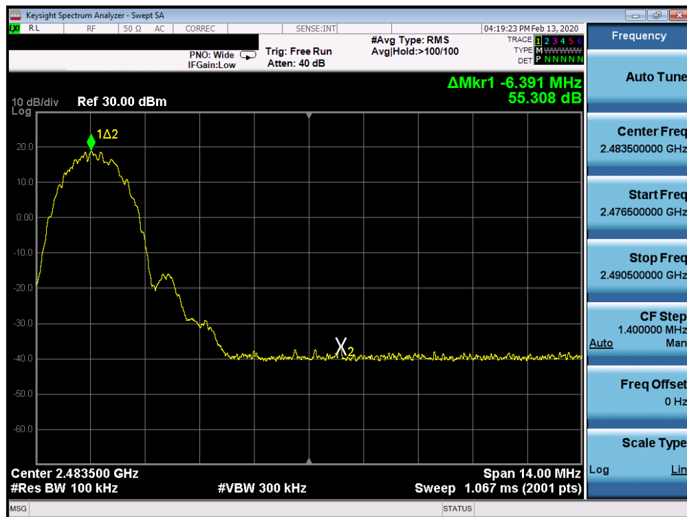
Plot 7-64. Band Edge Plot Ant 4a (Bluetooth (LE), 2Mbps ePA – Ch. 38)
