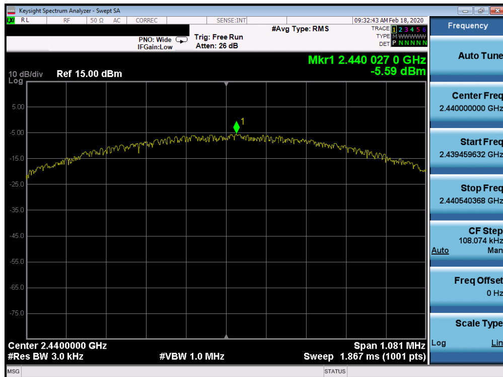
Plot 7-46. Power Spectral Density Plot TxBF Ant 2a (Bluetooth (LE), 1Mbps, iPA – Ch. 19)
