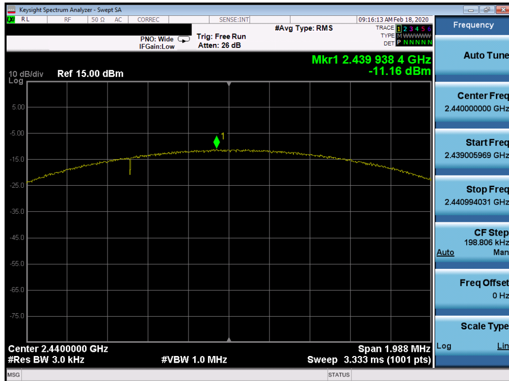
Plot 7-35. Power Spectral Density Plot Ant 2a (Bluetooth (LE), 2Mbps, iPA – Ch. 19)
