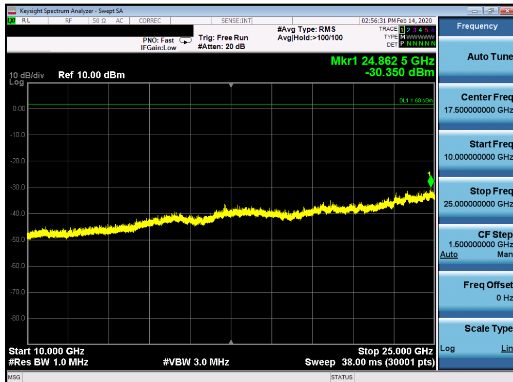
Plot 7-72. Conducted Spurious Plot Ant 4a (Bluetooth (LE), 1Mbps, ePA – Ch. 19)
