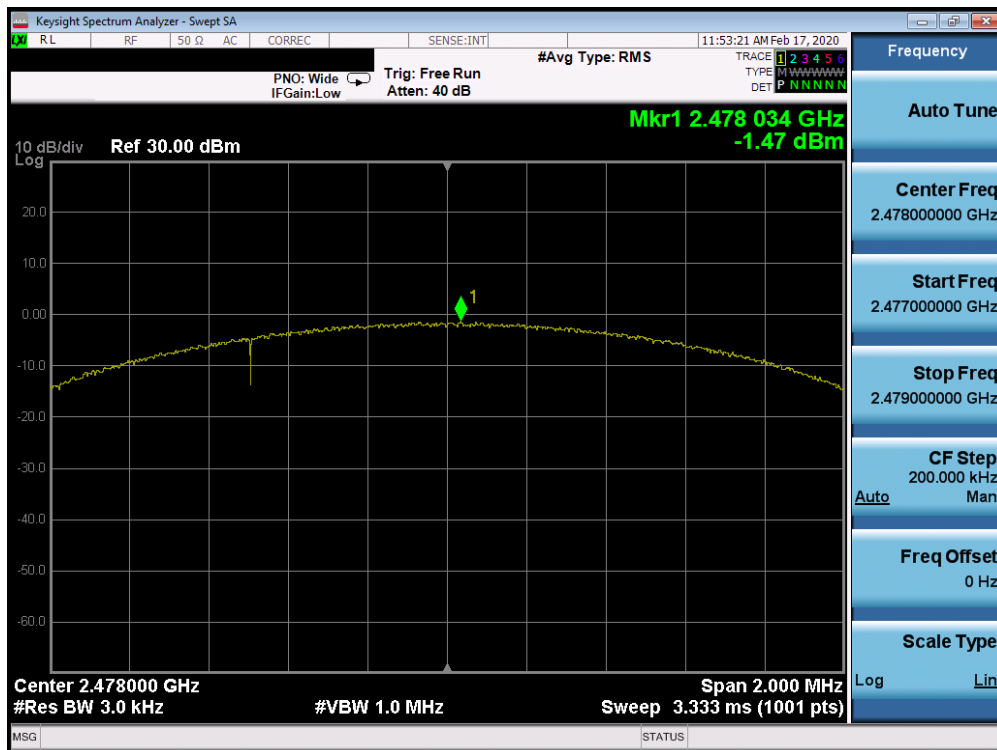
Plot 7-53. Power Spectral Density Plot Tx BF Ant 4a (Bluetooth (LE), 2Mbps, ePA – Ch. 38)
