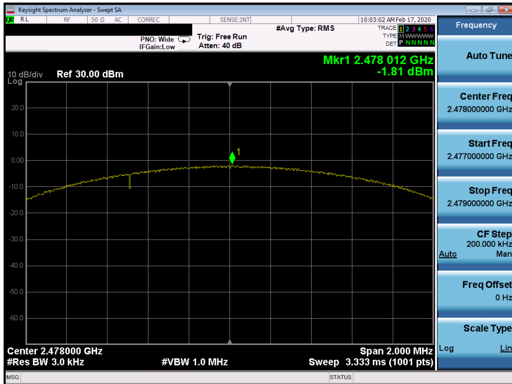
Plot 7-21. Power Spectral Density Plot Ant 4a (Bluetooth (LE), 2Mbps, ePA – Ch. 38)
