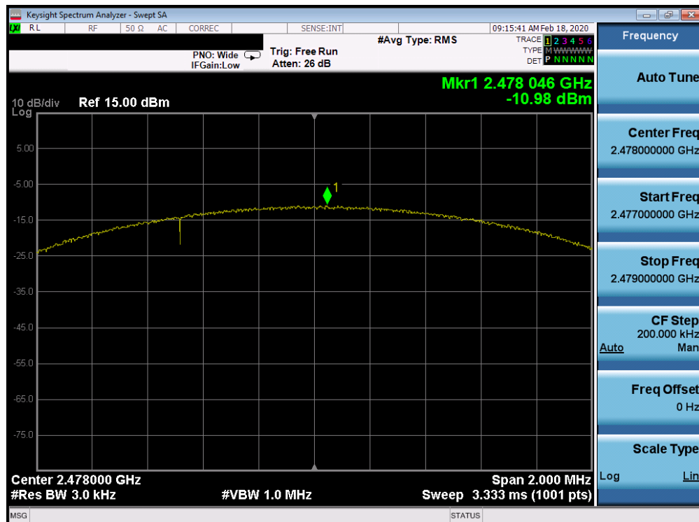
Plot 7-36. Power Spectral Density Plot Ant 2a (Bluetooth (LE), 2Mbps, iPA – Ch. 38)
