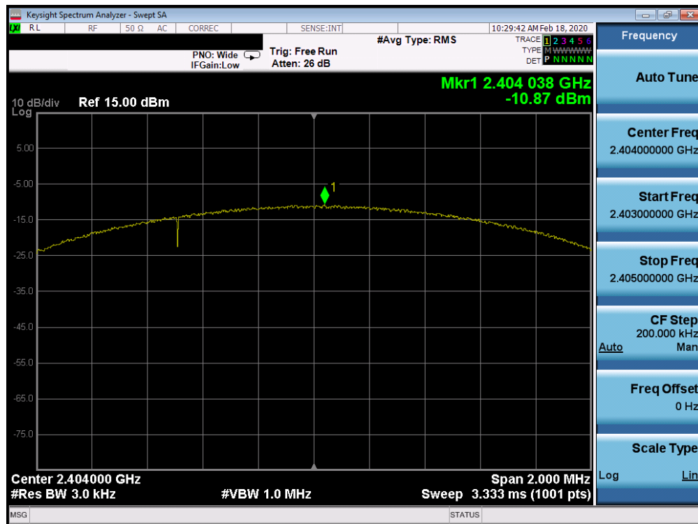
Plot 7-55. Power Spectral Density Plot Tx BF Ant 4a (Bluetooth (LE), 2Mbps, iPA – Ch. 1)
