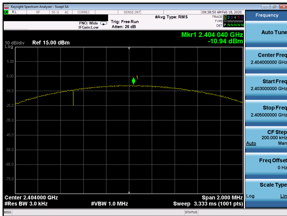
Plot 7-56. Power Spectral Density Plot Tx BF Ant 2a (Bluetooth (LE), 2Mbps, iPA – Ch. 1)
