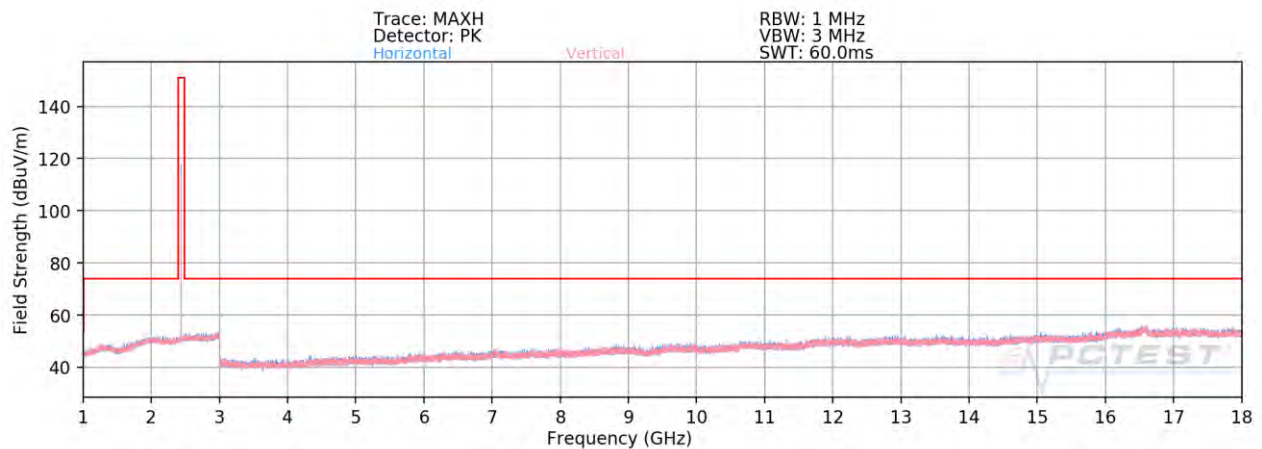
Plot 7-85. Radiated Spurious Plot Above 1GHz Ant 2a (1Mbps, ePA – Ch. 19)
