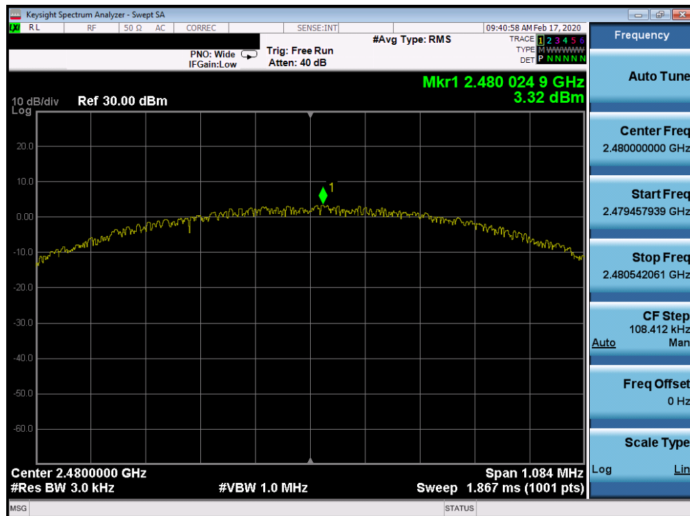
Plot 7-15. Power Spectral Density Plot Ant 4a (Bluetooth (LE), 1Mbps, ePA – Ch. 39)
