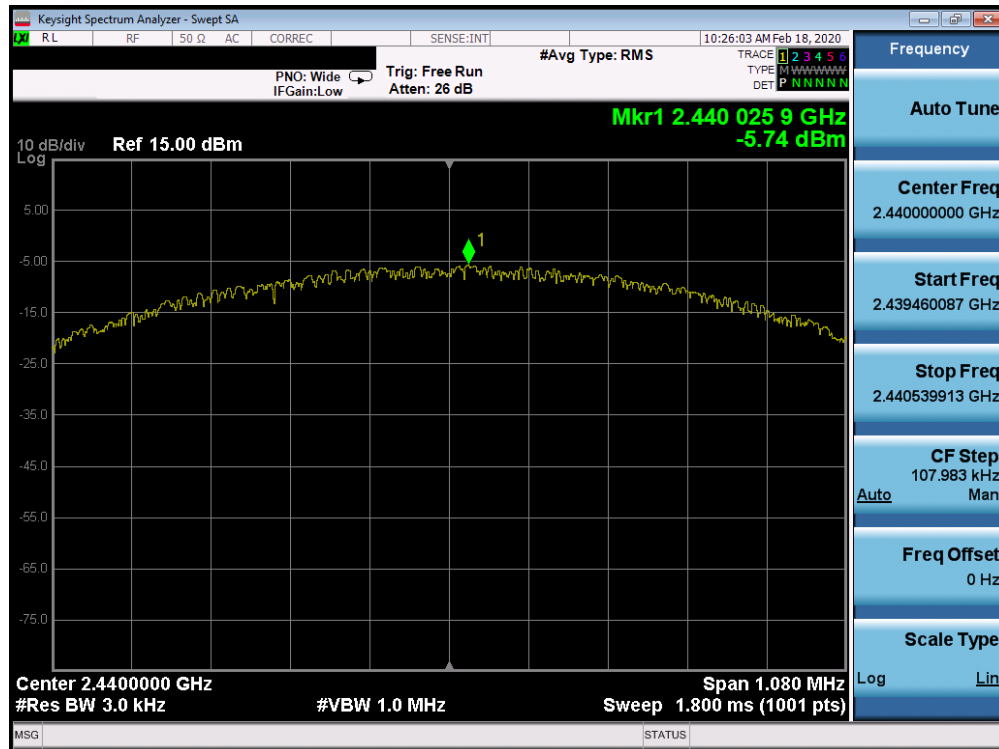
Plot 7-45. Power Spectral Density Plot TxBF Ant 4a (Bluetooth (LE), 1Mbps, iPA – Ch. 19)
