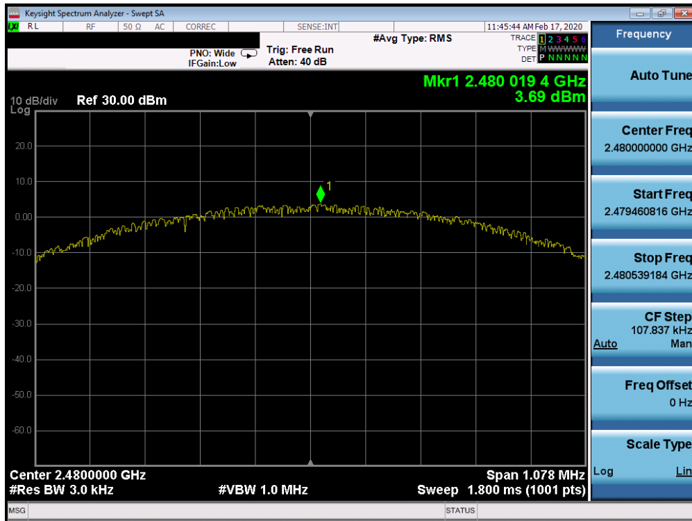
Plot 7-41. Power Spectral Density Plot TxBF Ant 4a (Bluetooth (LE), 1Mbps, ePA – Ch. 39)
