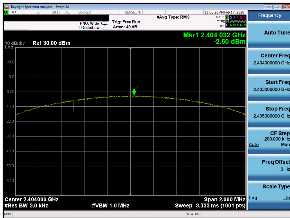
Plot 7-50. Power Spectral Density Plot Tx BF Ant 2a (Bluetooth (LE), 2Mbps, ePA – Ch. 1)
