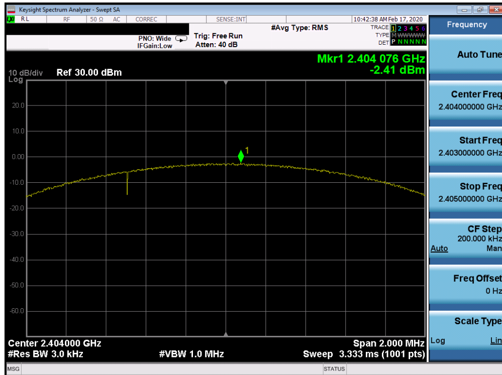
Plot 7-31. Power Spectral Density Plot Ant 2a (Bluetooth (LE), 2Mbps, ePA – Ch. 1)
