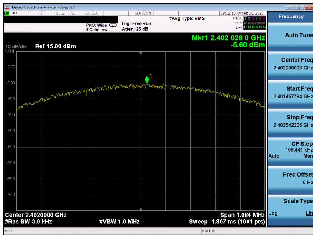
Plot 7-28. Power Spectral Density Plot Ant 2a (Bluetooth (LE), 1Mbps, iPA – Ch. 0)
