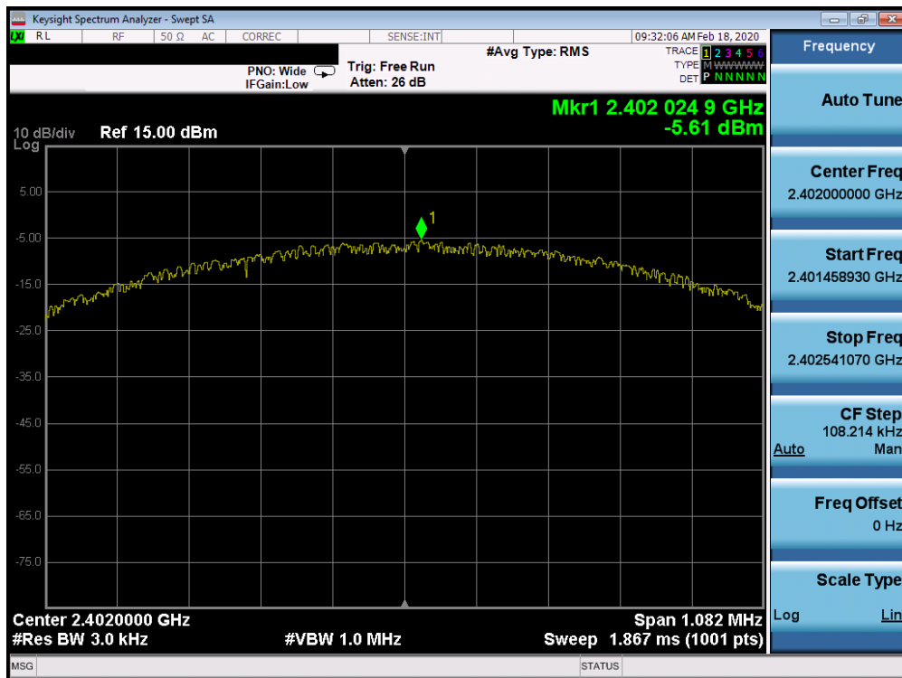
Plot 7-44. Power Spectral Density Plot Tx BF Ant 2a (Bluetooth (LE), 1Mbps, iPA – Ch. 0)
