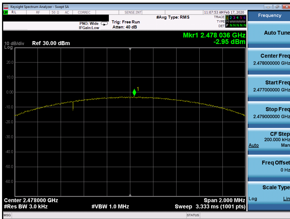
Plot 7-54. Power Spectral Density Plot Tx BF Ant 2a (Bluetooth (LE), 2Mbps, ePA – Ch. 38)
