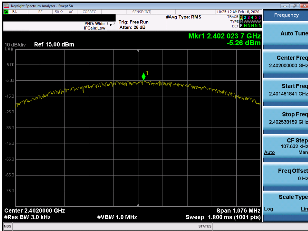
Plot 7-43. Power Spectral Density Plot Tx BF Ant 4a (Bluetooth (LE), 1Mbps, iPA – Ch. 0)
