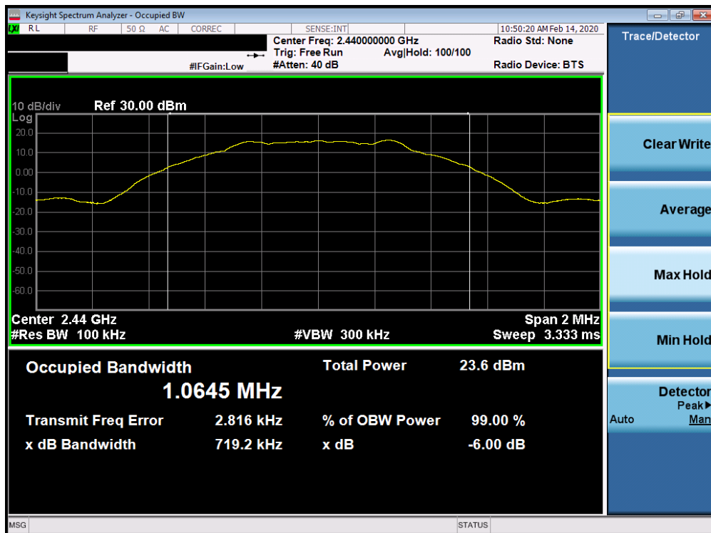
Plot 7-8. 6dB Bandwidth Plot Ant 2a (Bluetooth (LE), 1Mbps, ePA – Ch. 19)
