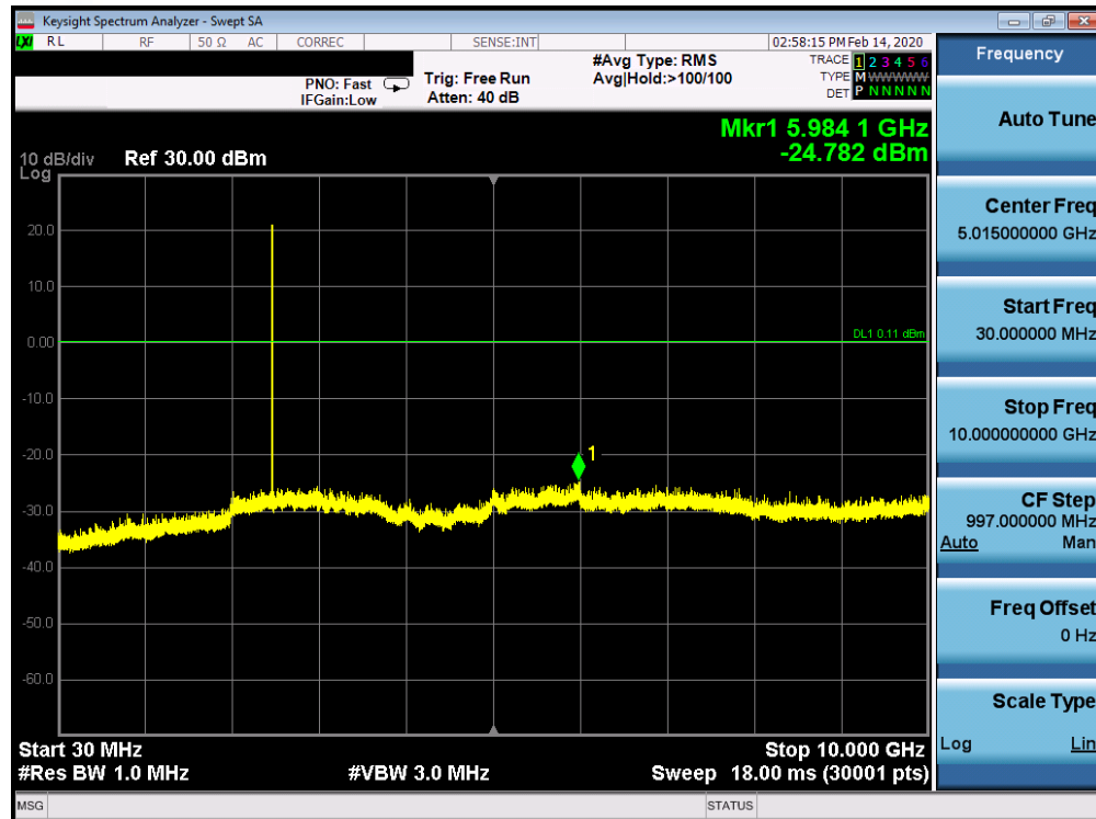
Plot 7-73. Conducted Spurious Plot Ant 4a (Bluetooth (LE), 1Mbps, ePA – Ch. 39)
