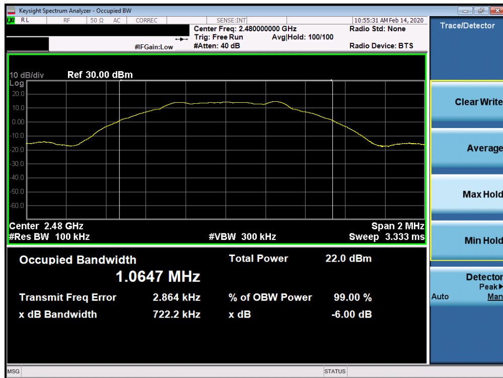
Plot 7-9. 6dB Bandwidth Plot Ant 2a (Bluetooth (LE), 1Mbps, ePA – Ch. 39)
