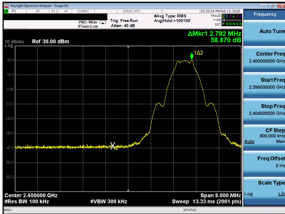
Plot 7-61. Band Edge Plot Ant 4a (Bluetooth (LE), 1Mbps ePA – Ch. 0)
