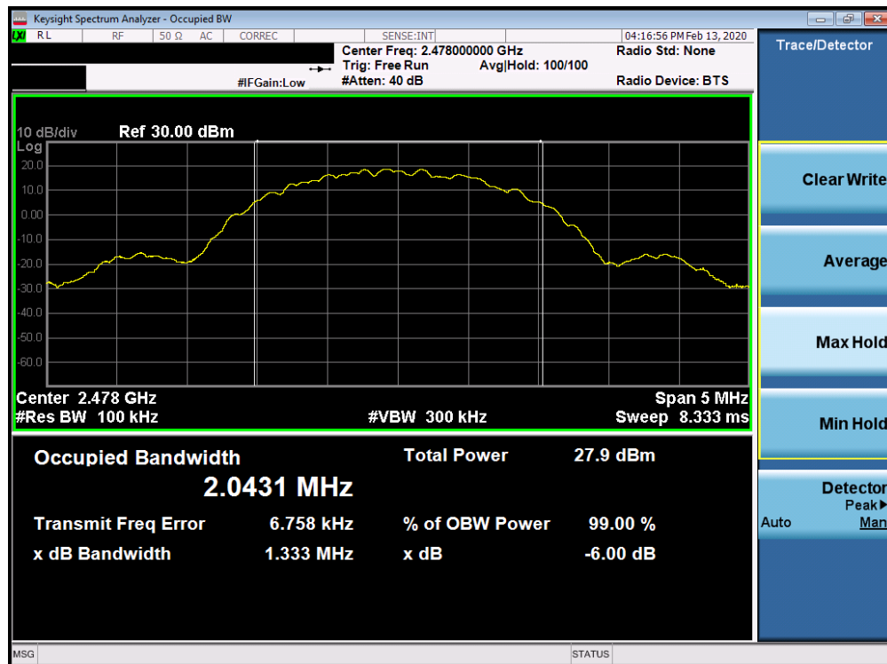
Plot 7-6. 6dB Bandwidth Plot Ant 4a (Bluetooth (LE), 2Mbps, ePA – Ch. 38)
