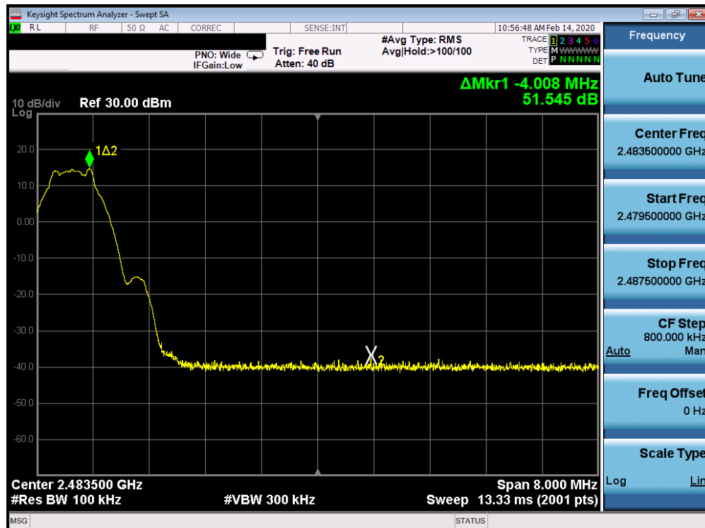
Plot 7-66. Band Edge Plot Ant 2a (Bluetooth (LE), 1Mbps ePA – Ch. 39)
