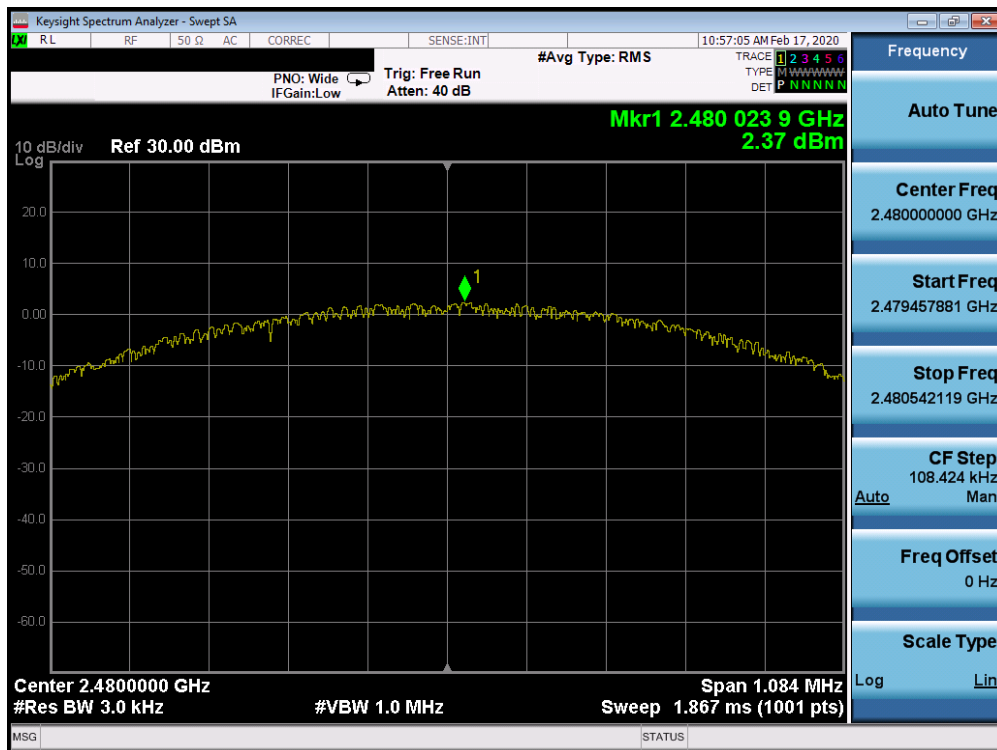
Plot 7-42. Power Spectral Density Plot TxBF Ant 2a (Bluetooth (LE), 1Mbps, ePA – Ch. 39)
