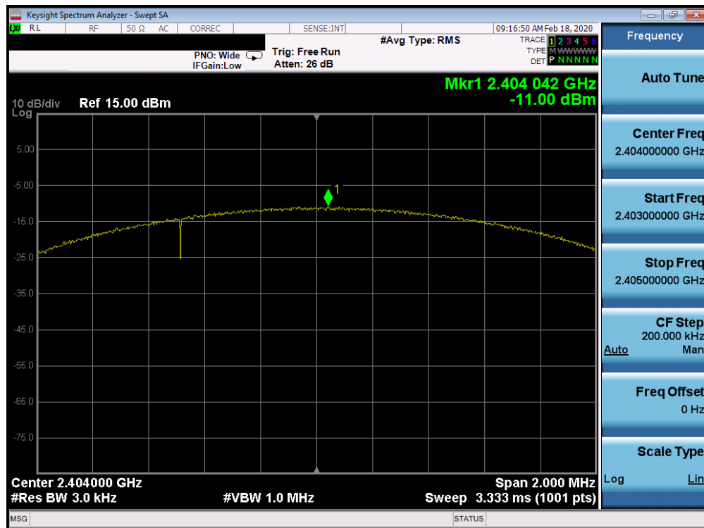
Plot 7-34. Power Spectral Density Plot Ant 2a (Bluetooth (LE), 2Mbps, iPA – Ch. 1)
