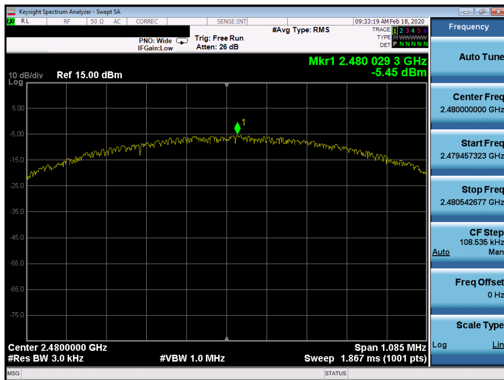
Plot 7-48. Power Spectral Density Plot TxBF Ant 2a (Bluetooth (LE), 1Mbps, iPA – Ch. 39)
