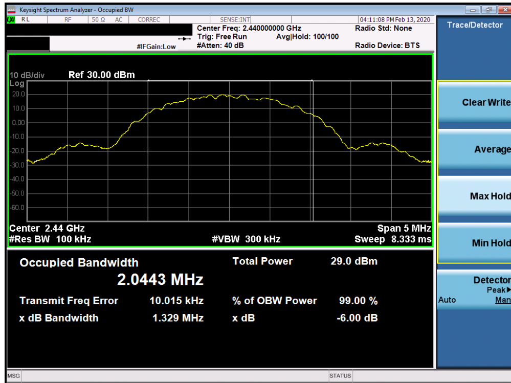
Plot 7-5. 6dB Bandwidth Plot Ant 4a (Bluetooth (LE), 2Mbps, ePA – Ch. 19)
