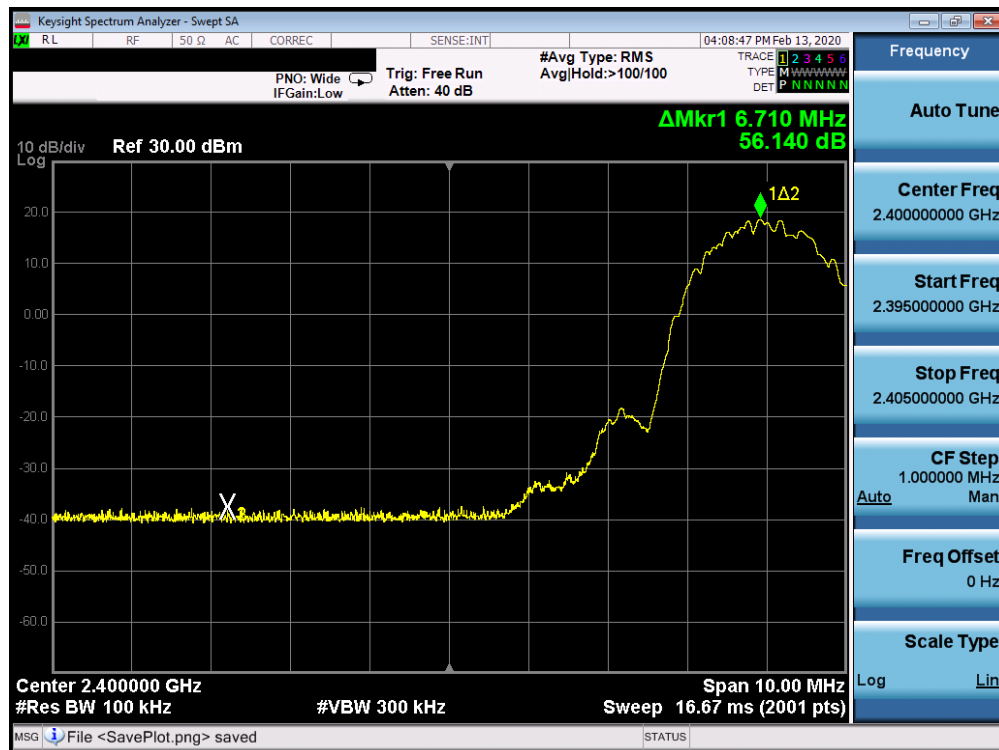
Plot 7-63. Band Edge Plot Ant 4a (Bluetooth (LE), 2Mbps ePA – Ch. 1)
