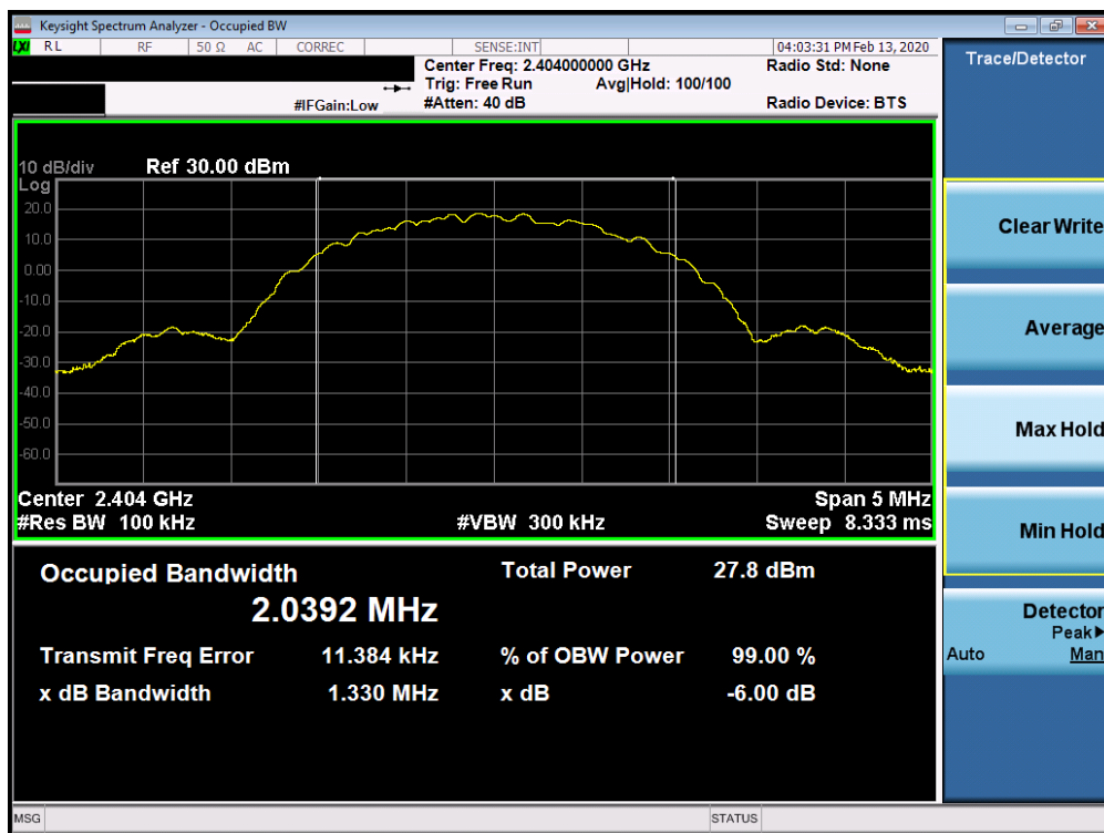
Plot 7-4. 6dB Bandwidth Plot Ant 4a (Bluetooth (LE), 2Mbps, ePA – Ch. 1)
