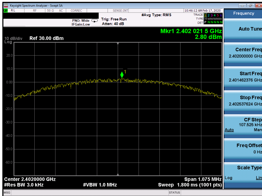
Plot 7-25. Power Spectral Density Plot Ant 2a (Bluetooth (LE), 1Mbps, ePA – Ch. 0)
