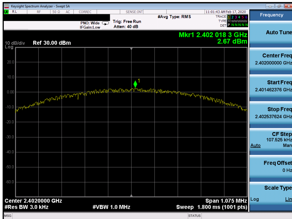
Plot 7-38. Power Spectral Density Plot TxBF Ant 2a (Bluetooth (LE), 1Mbps, ePA – Ch. 0)
