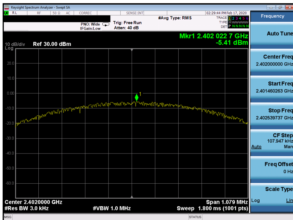
Plot 7-16. Power Spectral Density Plot Ant 4a (Bluetooth (LE), 1Mbps, iPA – Ch. 0)
