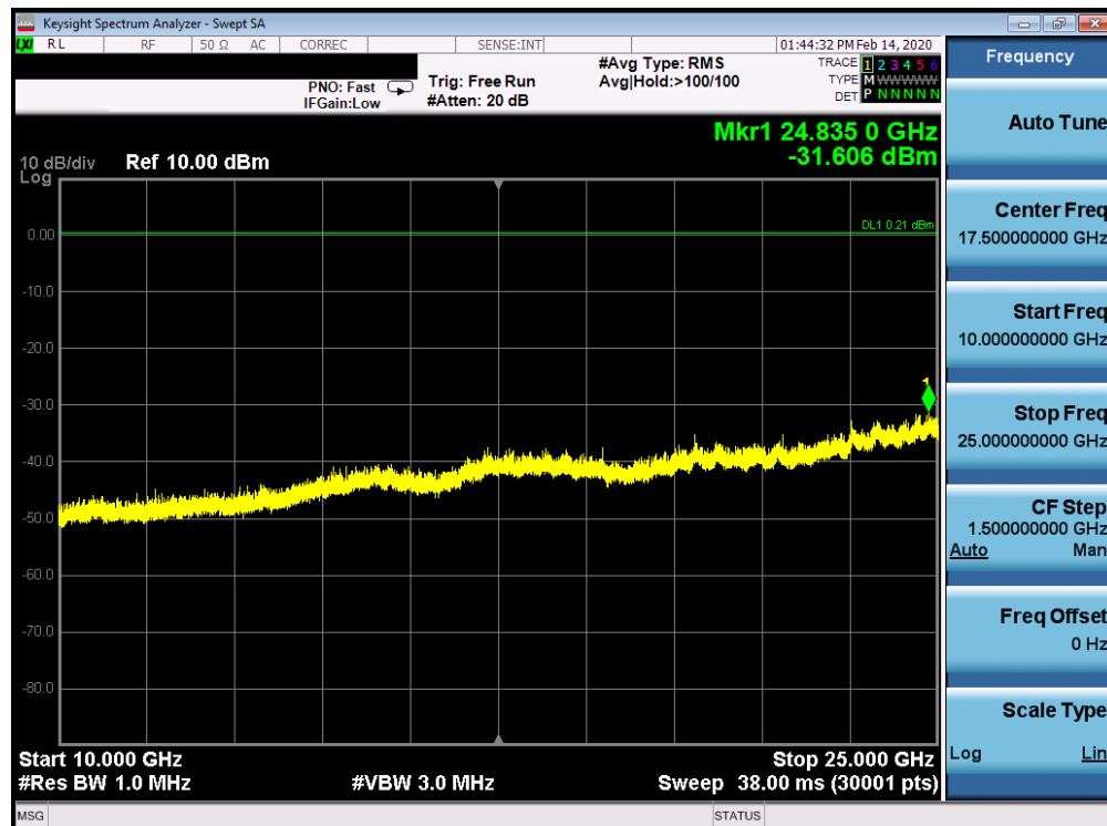
Plot 7-78. Conducted Spurious Plot Ant 2a (Bluetooth (LE), 1Mbps, ePA – Ch. 19)
