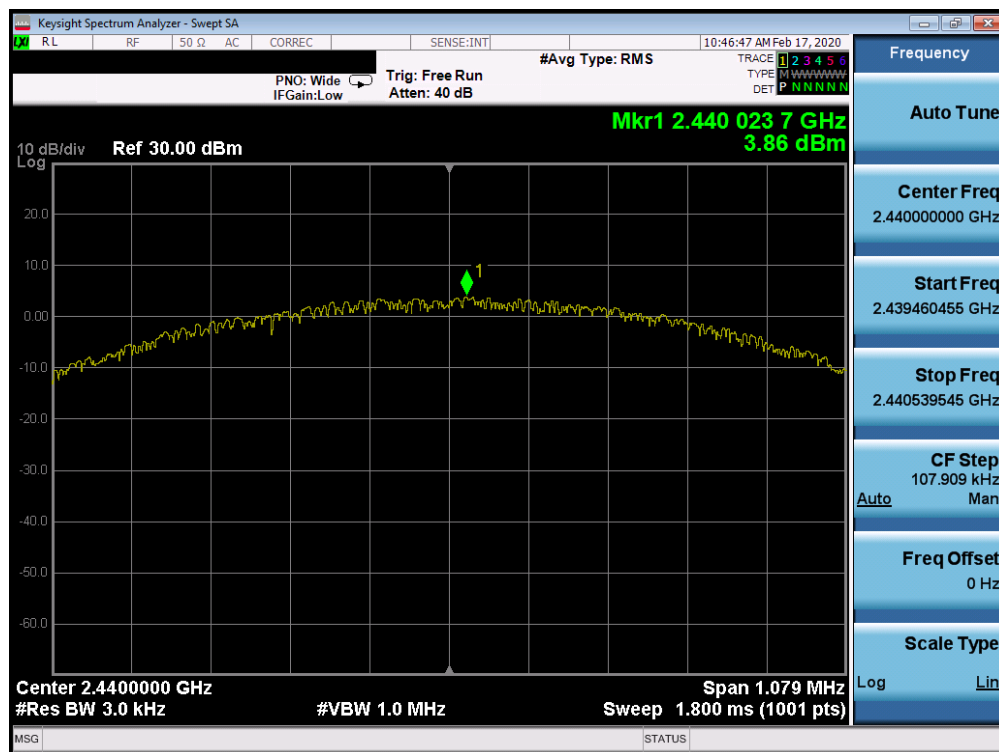
Plot 7-26. Power Spectral Density Plot Ant 2a (Bluetooth (LE), 1Mbps, ePA – Ch. 19)
