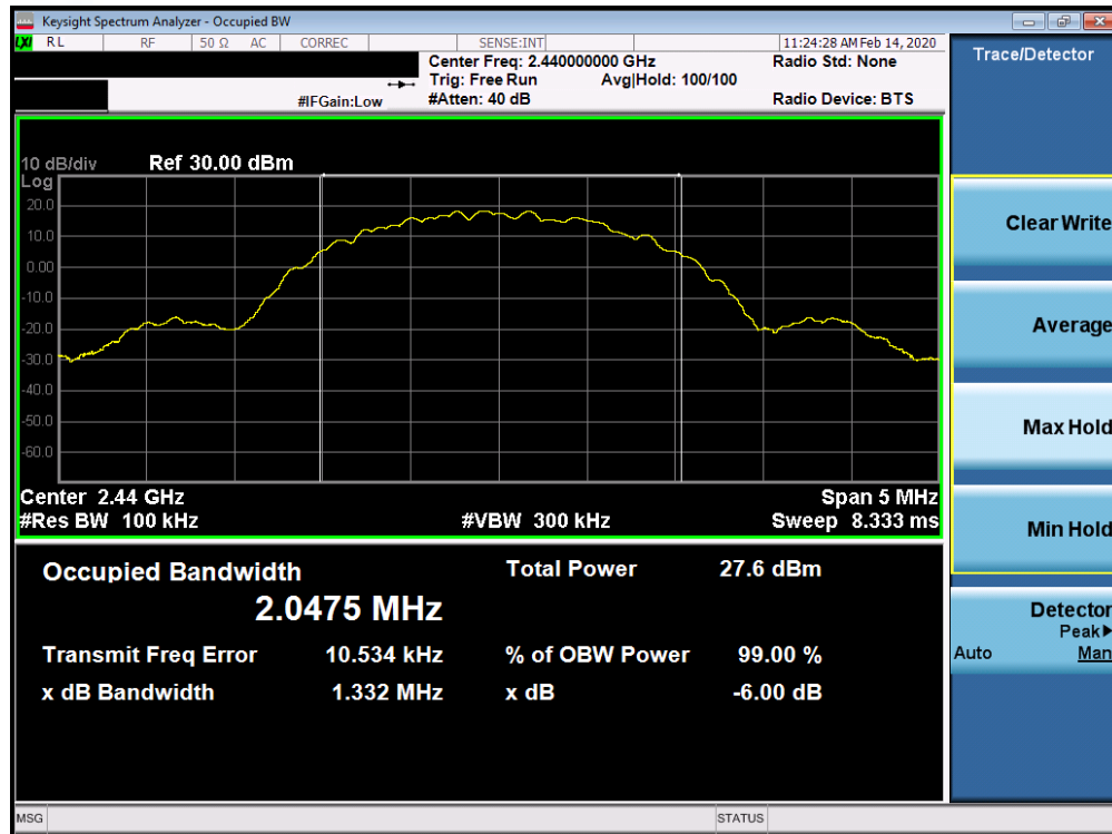
Plot 7-11. 6dB Bandwidth Plot Ant 2a (Bluetooth (LE), 2Mbps, ePA – Ch. 19)
