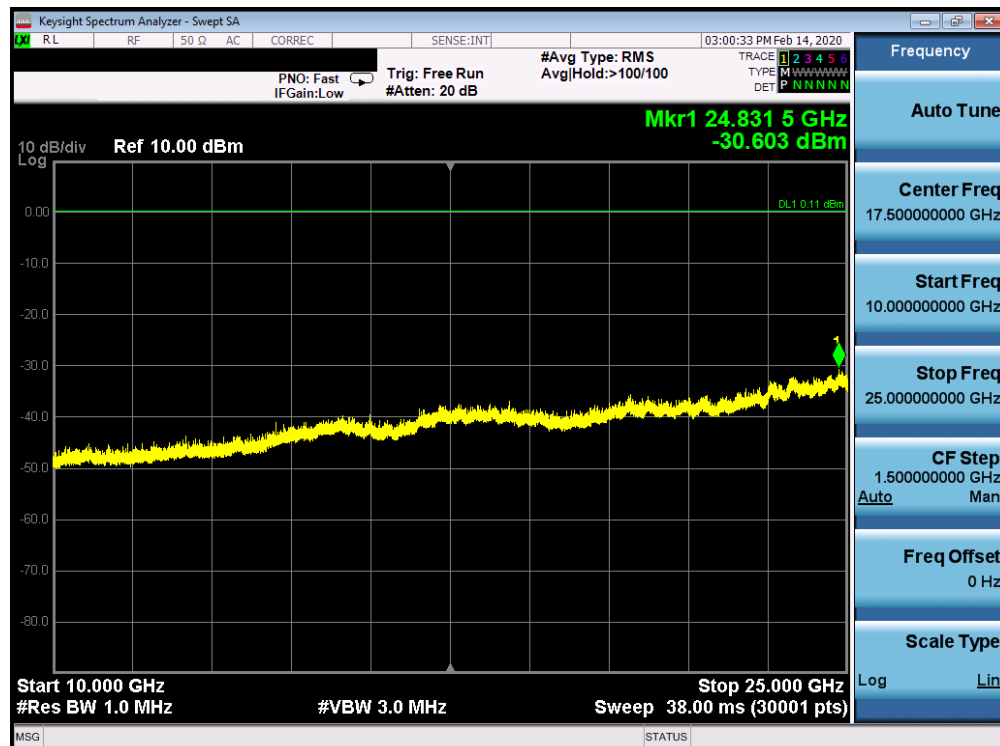
Plot 7-74. Conducted Spurious Plot Ant 4a (Bluetooth (LE), 1Mbps, ePA – Ch. 39)
