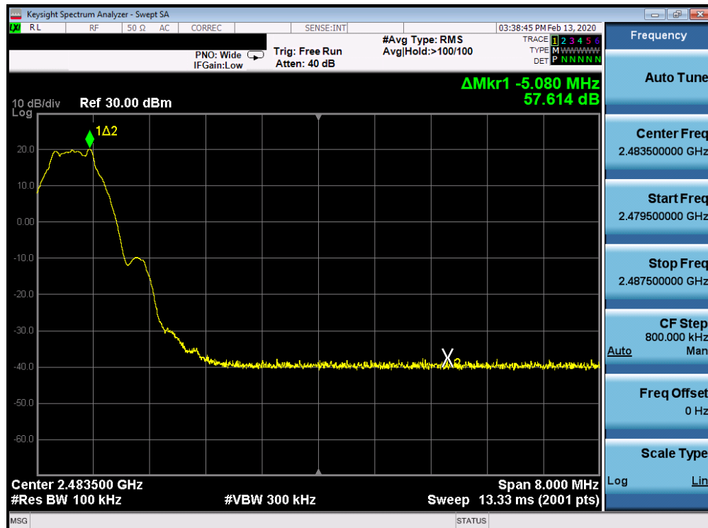
Plot 7-62. Band Edge Plot Ant 4a (Bluetooth (LE), 1Mbps ePA – Ch. 39)
