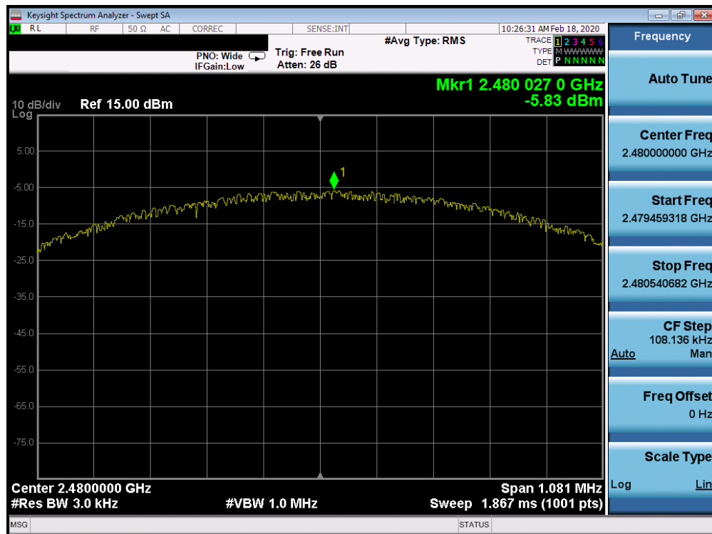
Plot 7-47. Power Spectral Density Plot TxBF Ant 4a (Bluetooth (LE), 1Mbps, iPA – Ch. 39)
