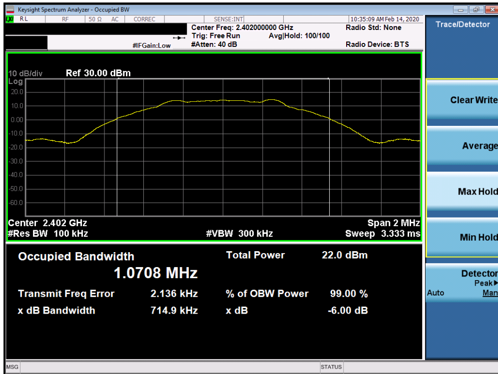
Plot 7-7. 6dB Bandwidth Plot Ant 2a (Bluetooth (LE), 1Mbps, ePA – Ch. 0)
