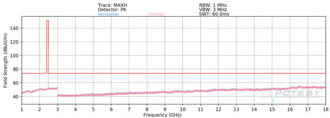
Plot 7-83. Radiated Spurious Plot Above 1GHz Ant 4a (1Mbps, ePA – Ch. 39)
