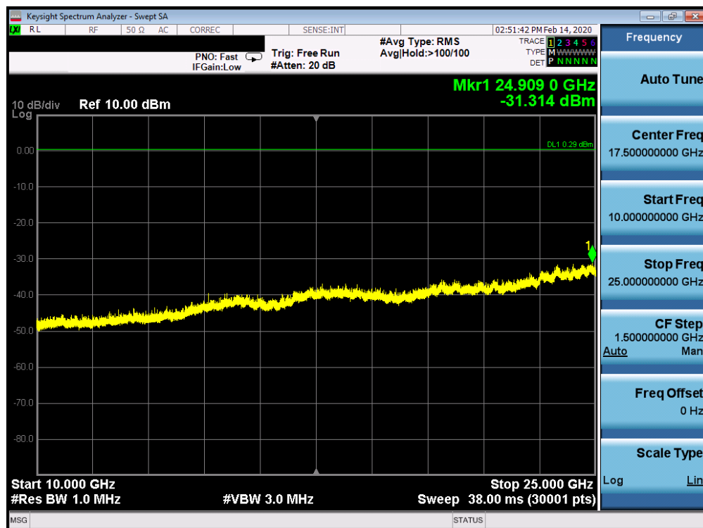
Plot 7-70. Conducted Spurious Plot Ant 4a (Bluetooth (LE), 1Mbps, ePA - Ch. 0)
