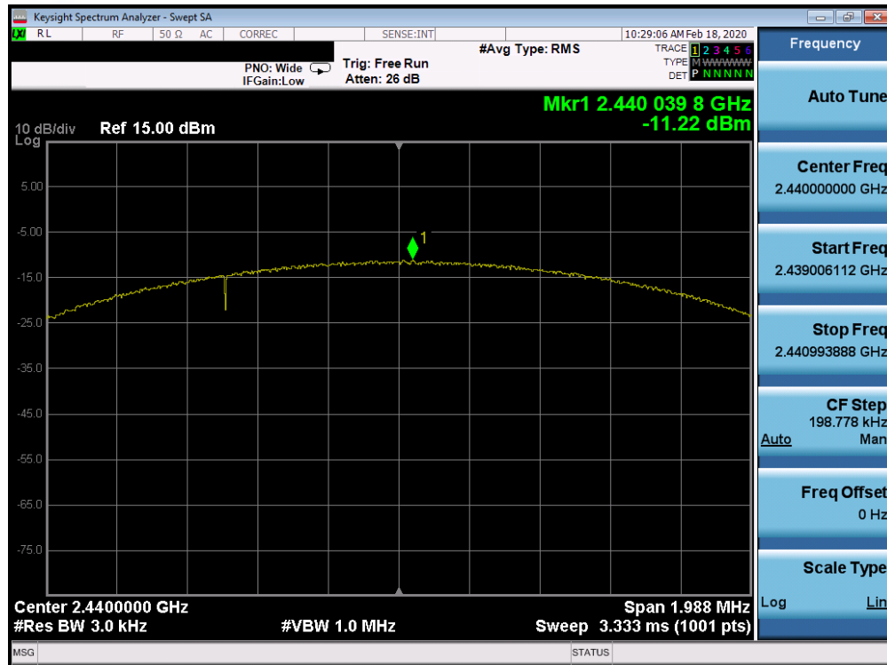
Plot 7-57. Power Spectral Density Plot TxBF Ant 4a (Bluetooth (LE), 2Mbps, iPA – Ch. 19)
