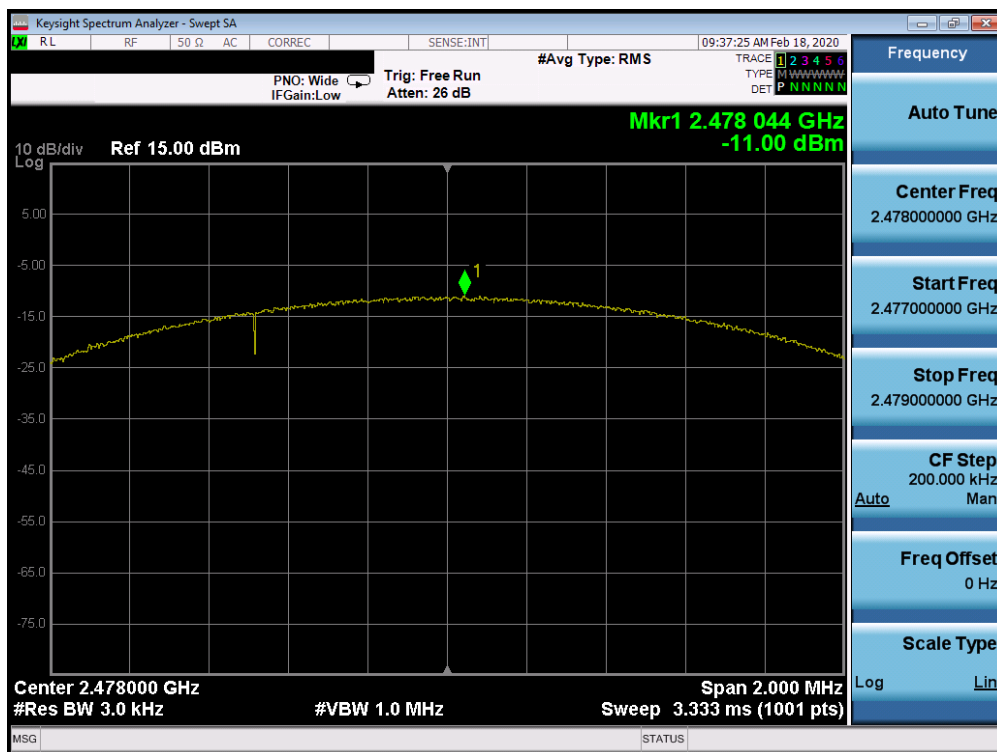
Plot 7-60. Power Spectral Density Plot TxBF Ant 2a (Bluetooth (LE), 2Mbps, iPA – Ch. 38)
