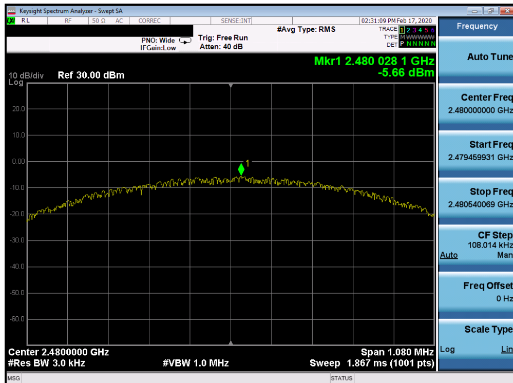
Plot 7-18. Power Spectral Density Plot Ant 4a (Bluetooth (LE), 1Mbps, iPA – Ch. 39)
