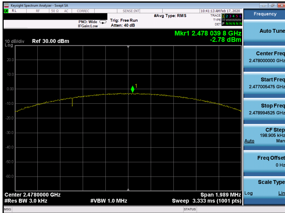
Plot 7-33. Power Spectral Density Plot Ant 2a (Bluetooth (LE), 2Mbps, ePA – Ch. 38)
