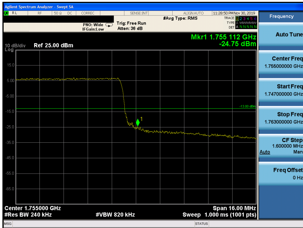
Plot 7-227. Upper Band Edge Plot (Band 4 – 20.0MHz QPSK – RB Size 100)
