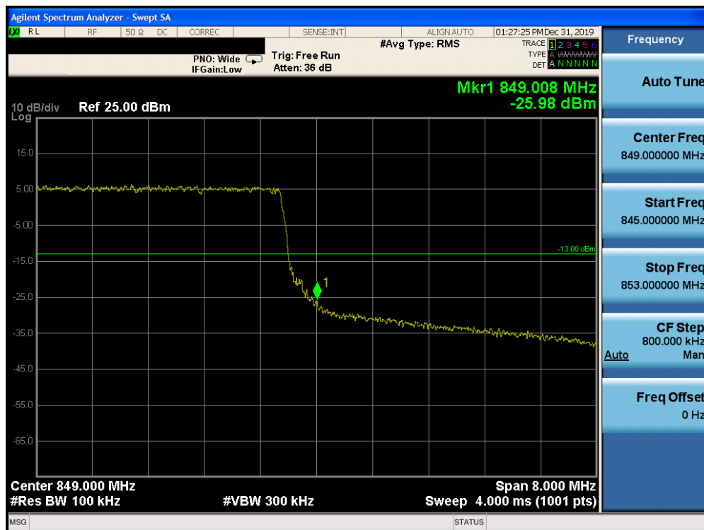
Plot 7-204. Upper Band Edge Plot (Band 26 – 10.0MHz QPSK – RB Size 50)
