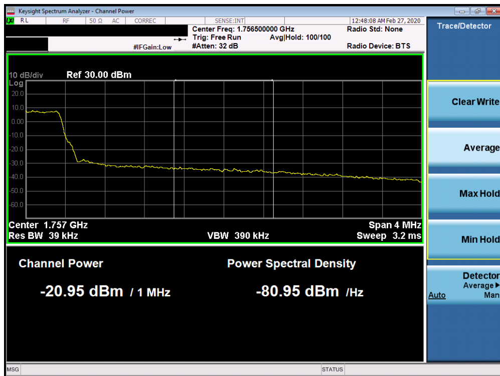
Plot 7-212. Upper Extended Band Edge Plot (Band 4 – 3.0MHz QPSK – RB Size 15)
