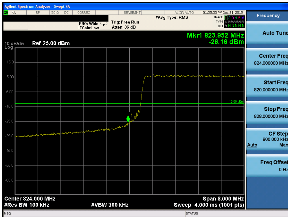
Plot 7-203. Lower Band Edge Plot (Band 26 – 10.0MHz QPSK – RB Size 50)
