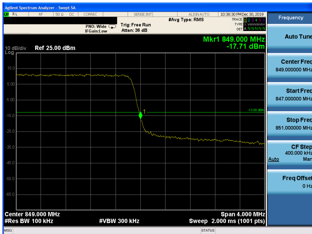
Plot 7-192. Upper Band Edge Plot (Band 5 – 3.0MHz QPSK – RB Size 15)
