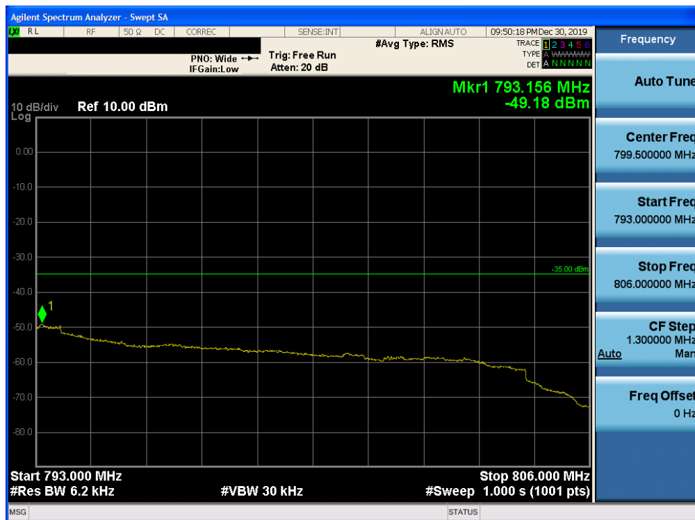
Plot 7-188. Upper Emission Mask Edge Plot (Band 13 – 10.0MHz QPSK – RB Size 50)
