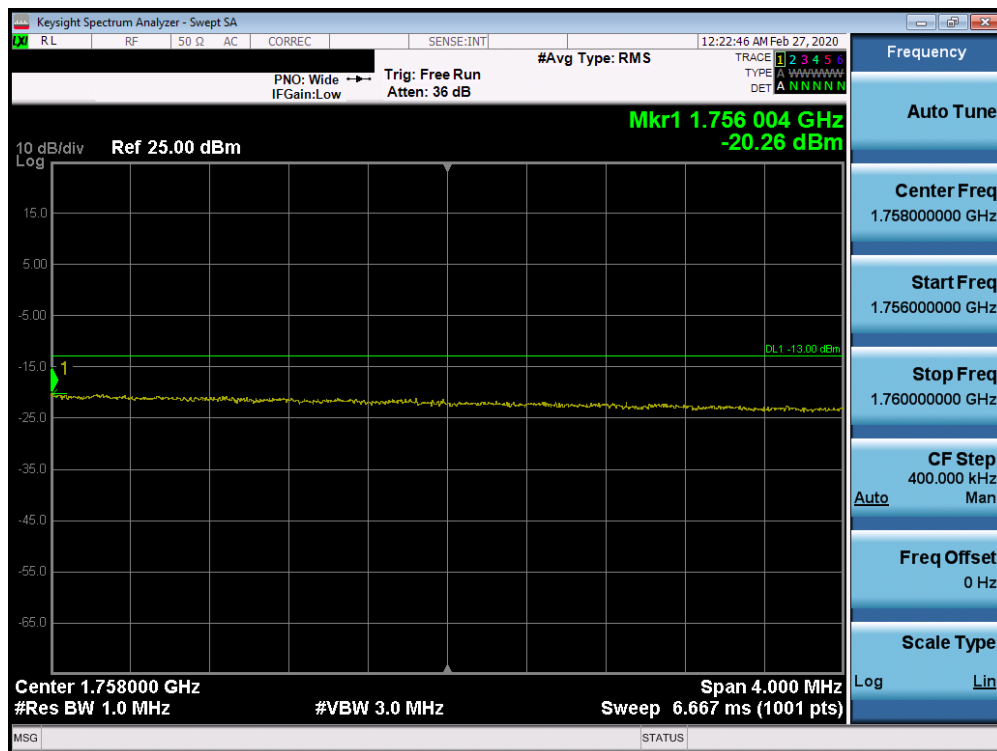
Plot 7-228. Upper Extended Band Edge Plot (Band 4 – 20.0MHz QPSK – RB Size 100)
