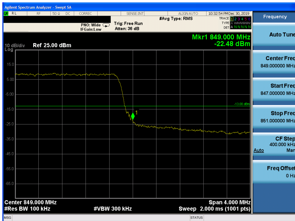
Plot 7-194. Upper Band Edge Plot (Band 5 – 5.0MHz QPSK – RB Size 25)
