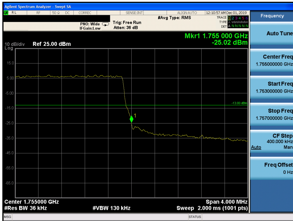
Plot 7-211. Upper Band Edge Plot (Band 4 – 3.0MHz QPSK – RB Size 15)
