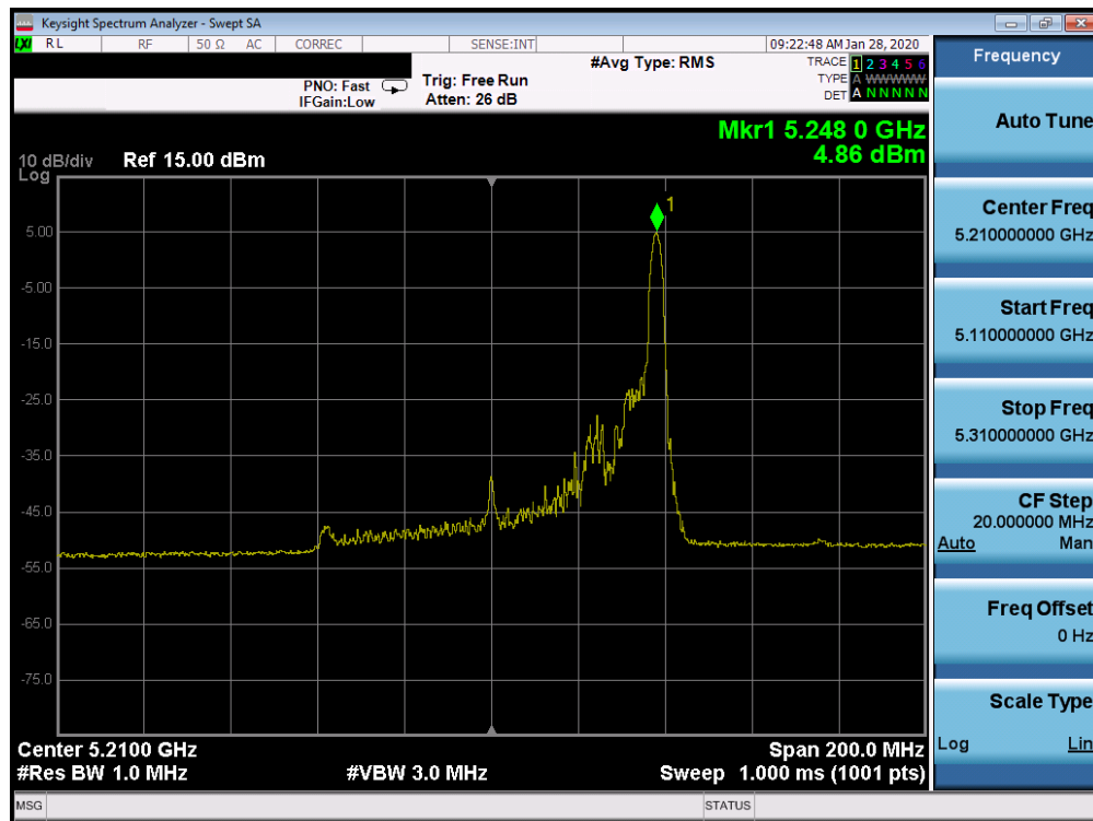
Plot 7-311. Power Spectral Density Plot ISSED SISO CORE 0 (80MHz BW 802.11ax Index 36 – RU26 (UNII Band 1) – Ch. 42)
