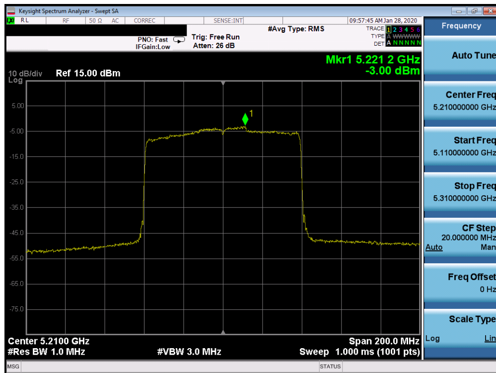
Plot 7-312. Power Spectral Density Plot ISSED SISO CORE 0 (80MHz BW 802.11ax – RU996 (UNII Band 1) – Ch. 42)
