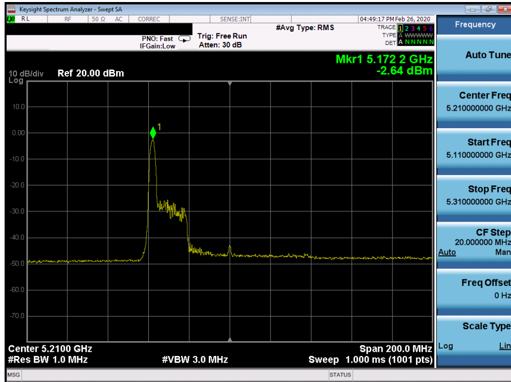
Plot 7-665. Power Spectral Density Plot ISD CDD CORE 0 (80MHz BW 802.11ax Index 0 – RU26 (UNII Band 1) – Ch. 42)
