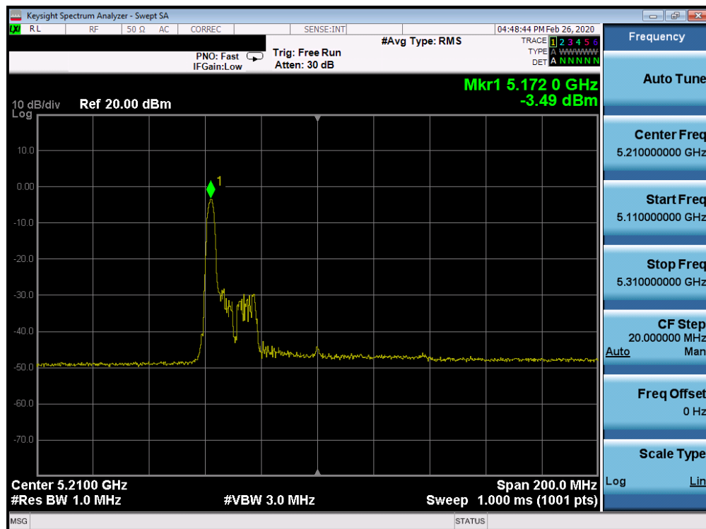
Plot 7-666. Power Spectral Density Plot ISD CDD CORE 1 (80MHz BW 802.11ax Index 0 – RU26 (UNII Band 1) – Ch. 42)
