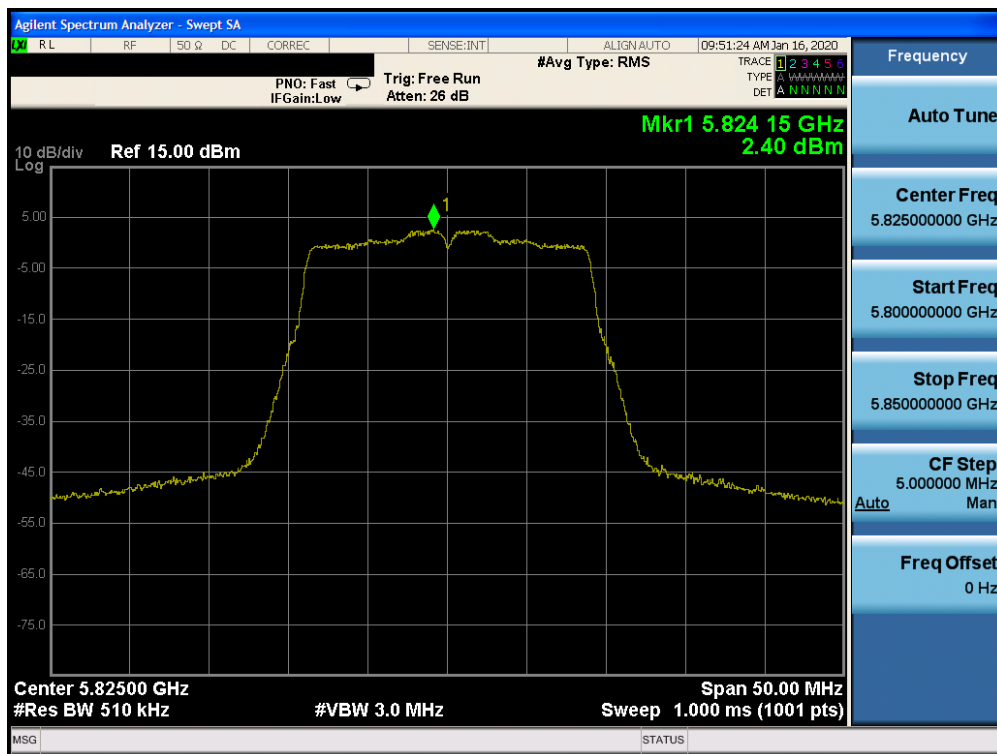
Plot 7-166. Power Spectral Density Plot CDD CORE 1 (20MHz BW 802.11n (UNII Band 3) – Ch. 165)
