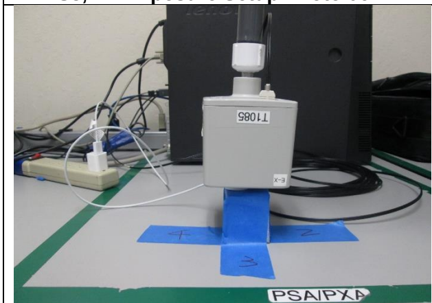
Center, RF Exposure Setup Photo 0cm
