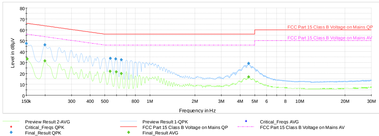
Plot 7-29. AC Line Conducted Plot with Bluetooth LE (L1, ePA - Ch.19, with AC/DC Adapter)
