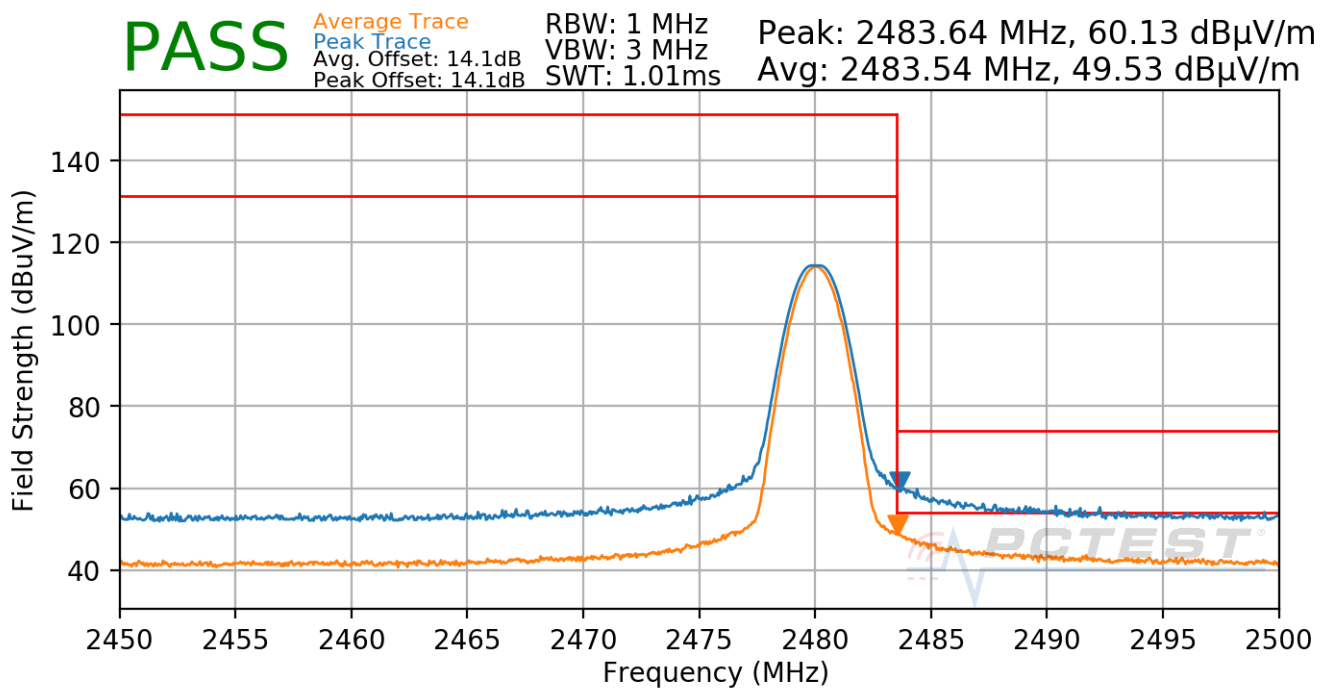
Plot 7-39. Radiated Restricted Upper Band Edge Measurement
