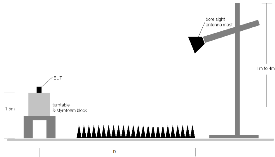
Figure 7-8. Radiated Measurement Setup >1GHz
