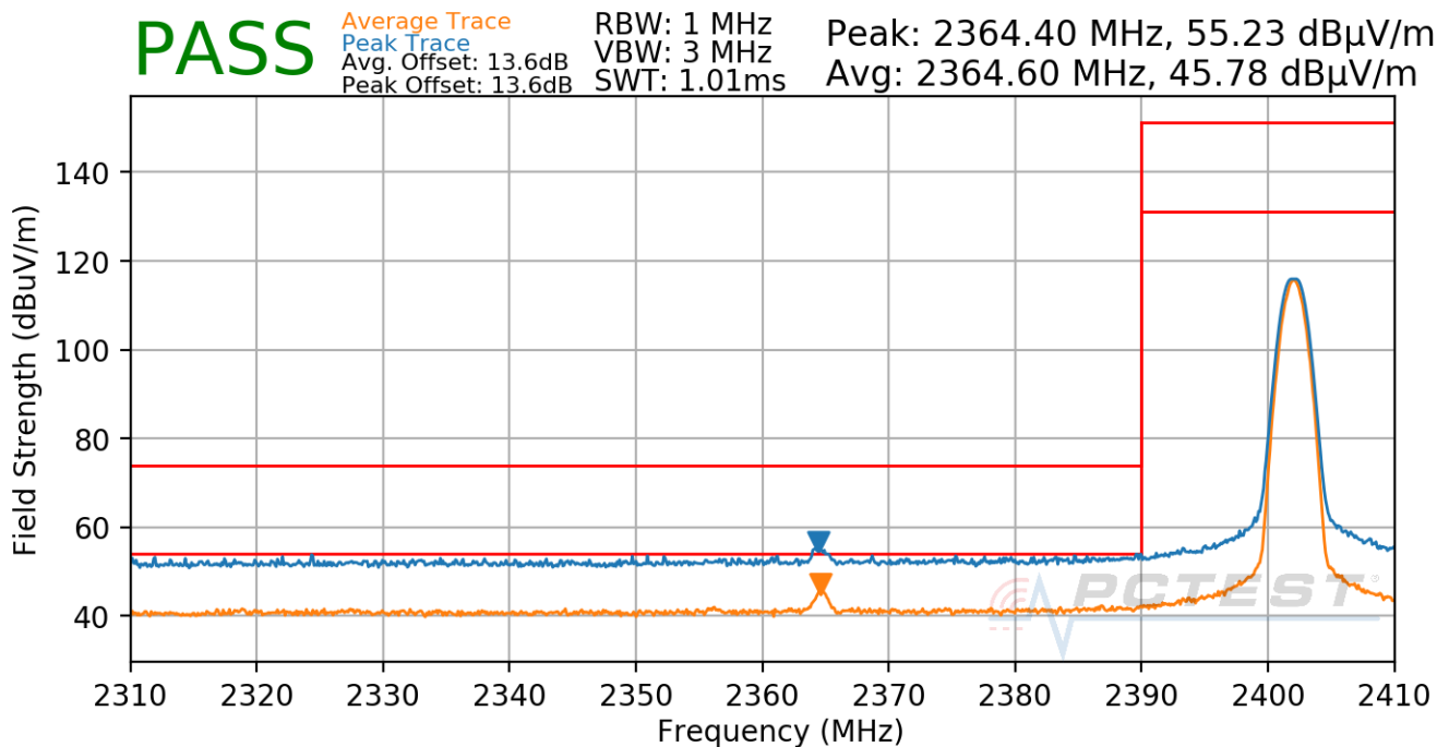
Plot 7-37. Radiated Restricted Lower Band Edge Measurement
