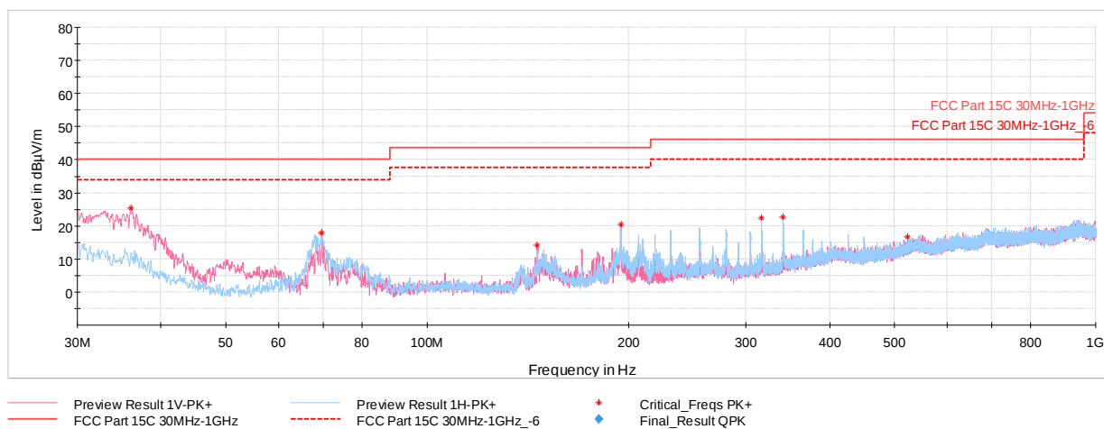
Plot 7-42. Radiated Spurious Plot Below 1GHz (Simultaneous Tx, with AC/DC Adapter)
