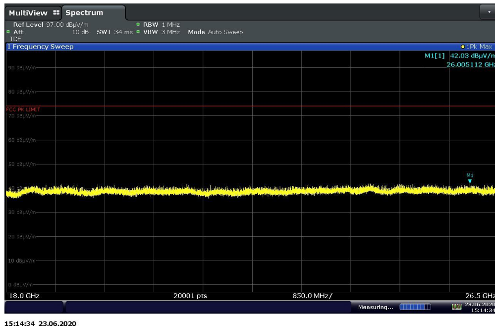
Plot 7-33. Radiated Spurious Emissions above 18GHz (GFSK ePA – Ch. 39, Pol. V)
