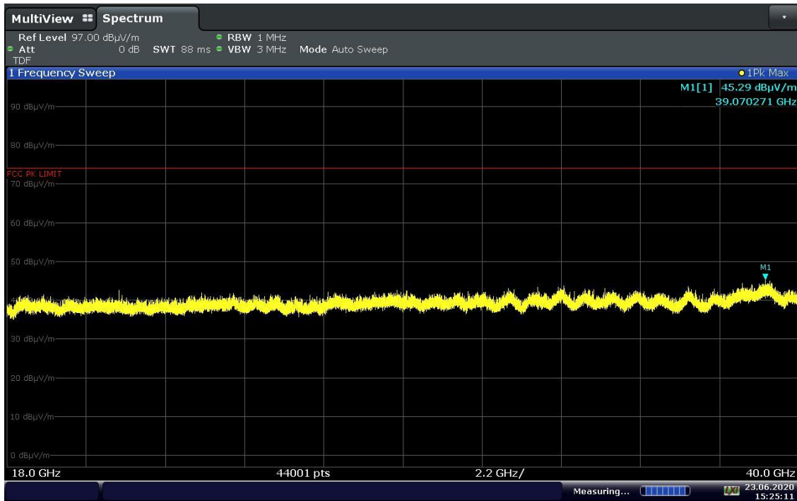
Plot 7-35. Radiated Spurious Plot 18GHz– 40GHz (Simultaneous Tx - Pol. H)
