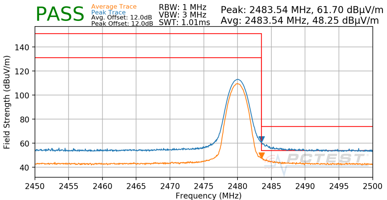
Plot 7-40. Radiated Restricted Upper Band Edge Measurement
