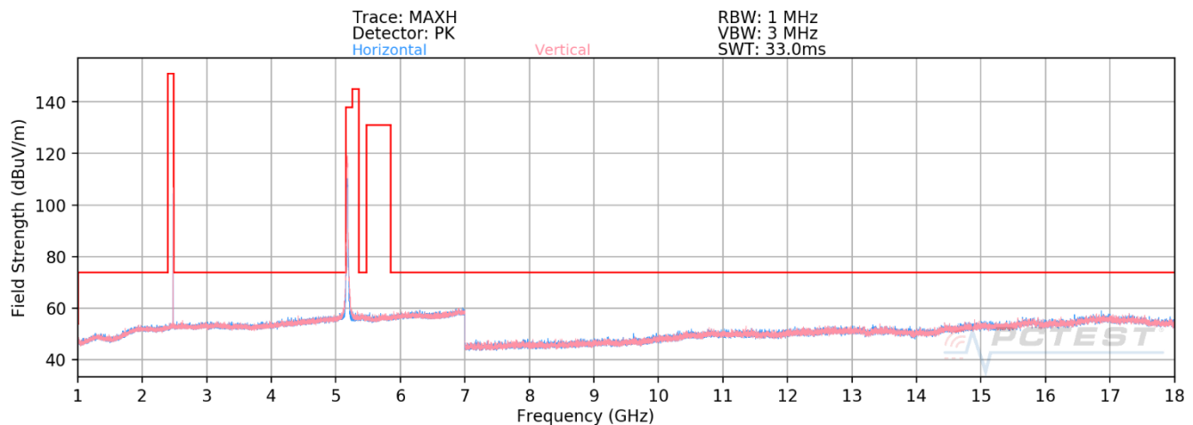
Plot 7-34. Radiated Spurious Plot above 1GHz (Simultaneous Tx)
