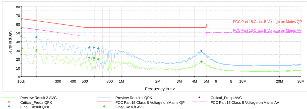
Plot 7-43. AC Line-Conducted Test Plot - Ch.39 (L1, with AC/DC Adapter)
