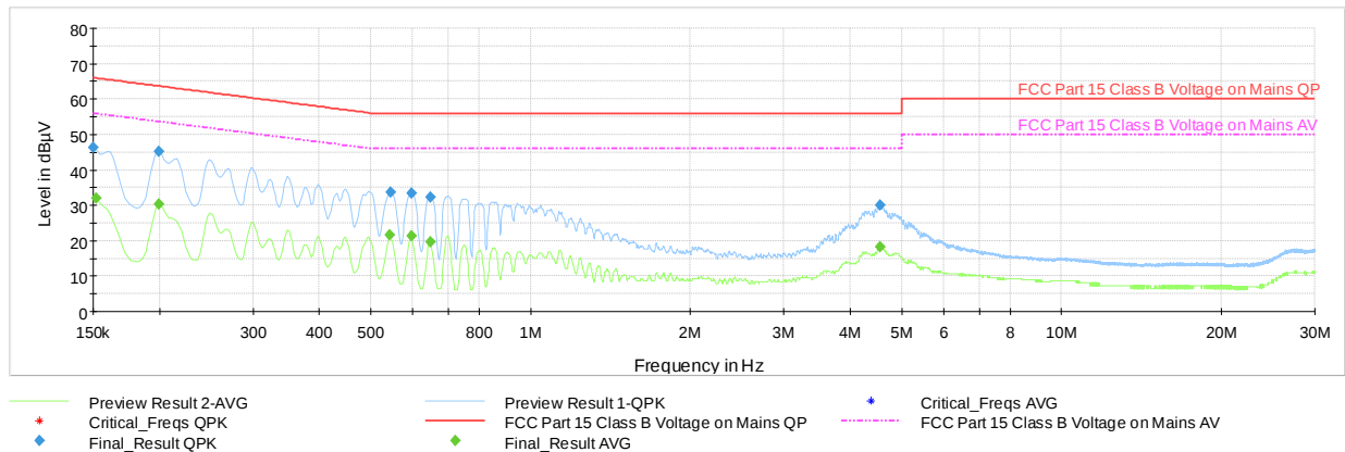
Plot 7-44. AC Line-Conducted Test Plot - Ch.39 (N, with AC/DC Adapter)
