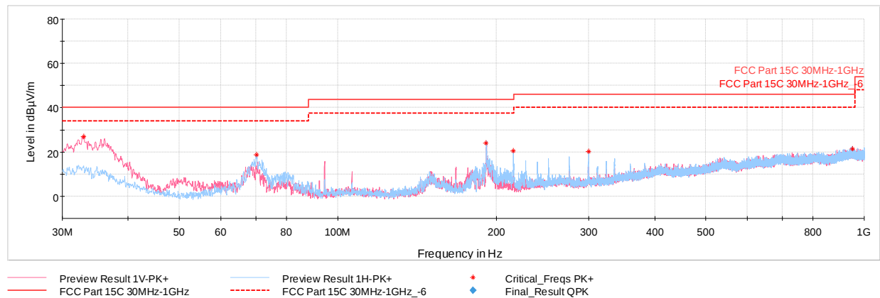
Plot 7-41. Radiated Spurious Plot Below 1GHz (GFSK ePA – Ch.39, with AC/DC Adapter)
