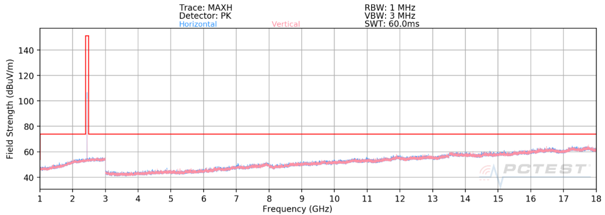
Plot 7-30. Radiated Spurious Emissions 1-18GHz (BT GFSK iPA – Ch. 39)
