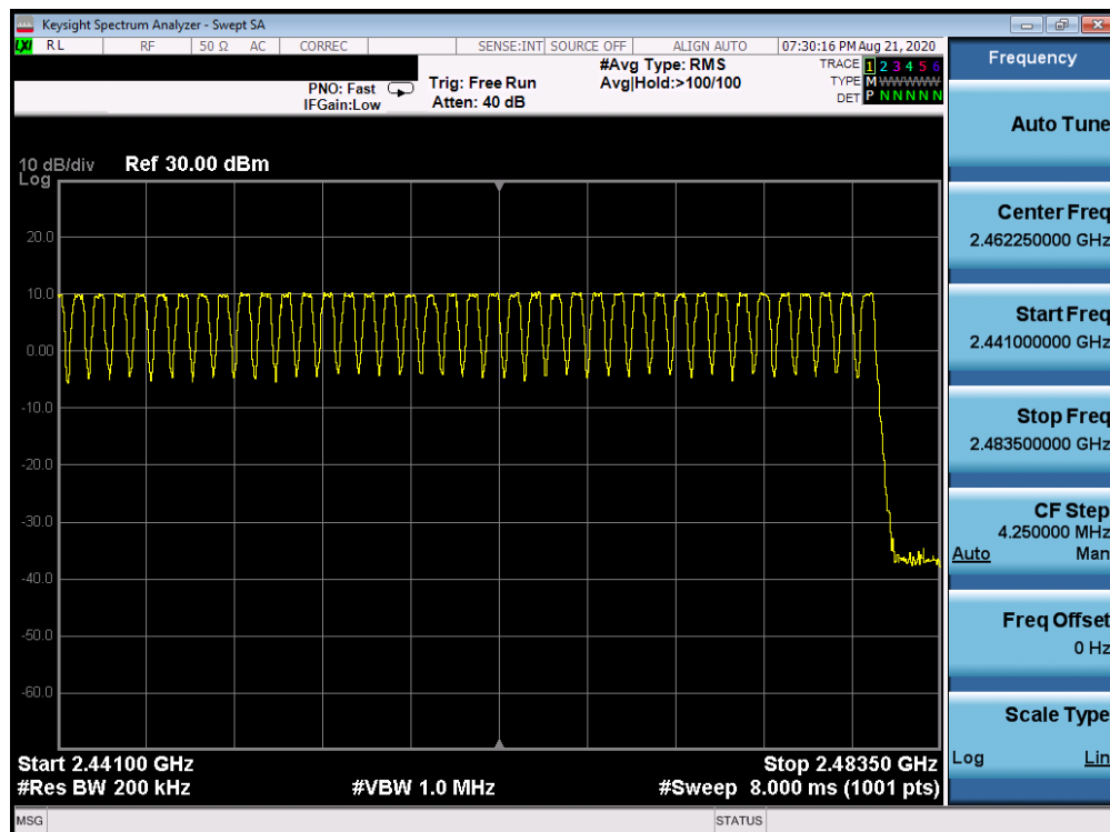
Plot 7-20. High End Spectrum Channel Hopping Plot (Bluetooth, GFSK, iPA)
