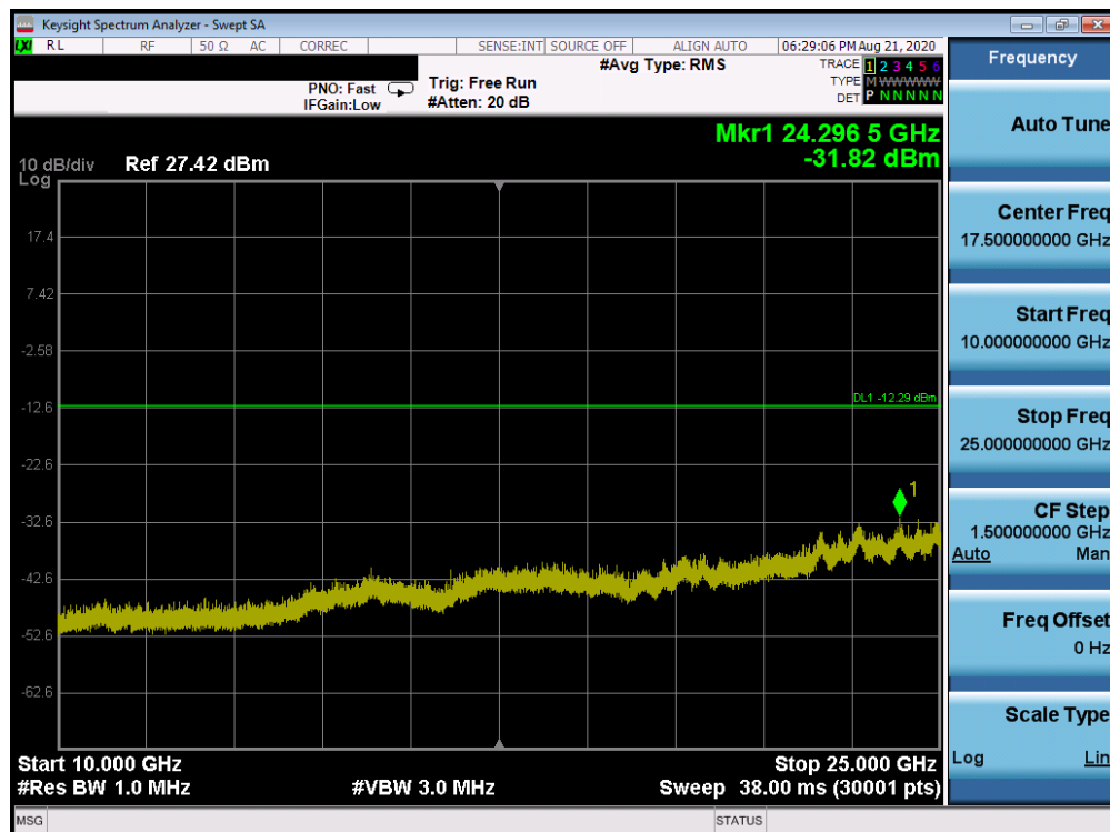
Plot 7-24. Conducted Spurious Plot (Bluetooth, GFSK, iPA – Ch. 0)
