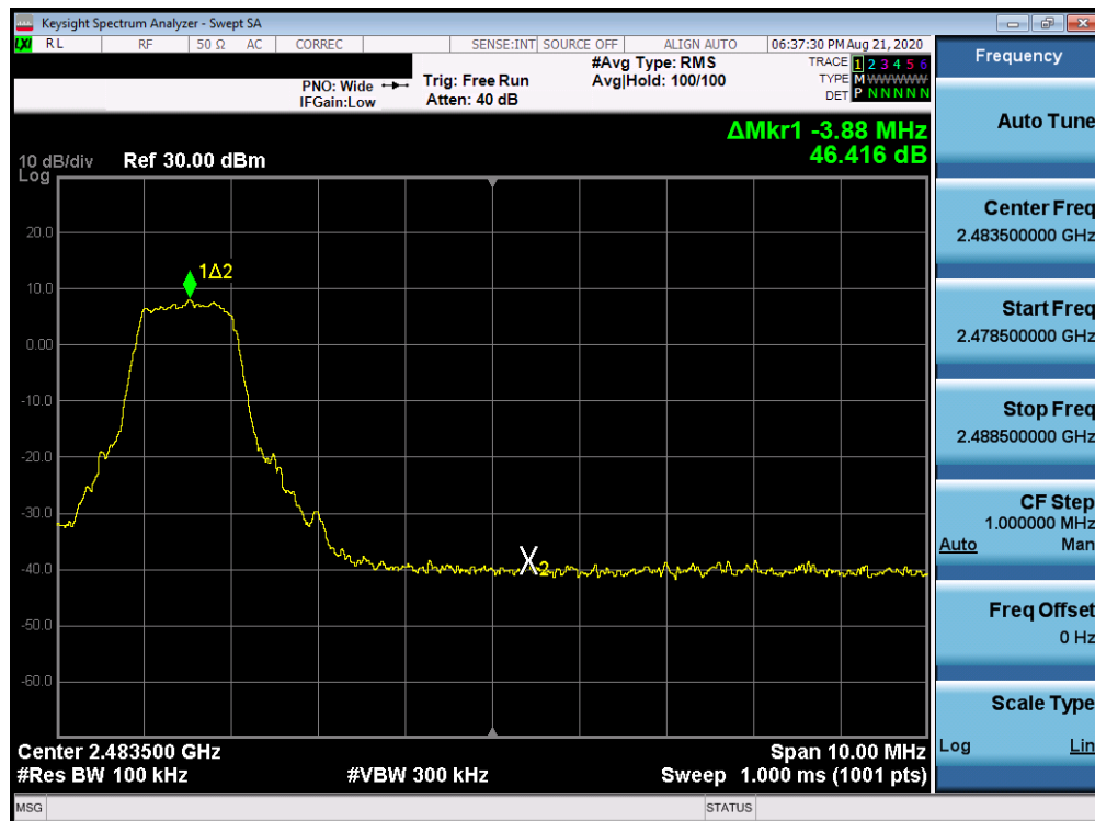
Plot 7-12. Band Edge Plot (Bluetooth with Hopping Disabled, \pi/4 -DQPSK, iPA – Ch. 78)
