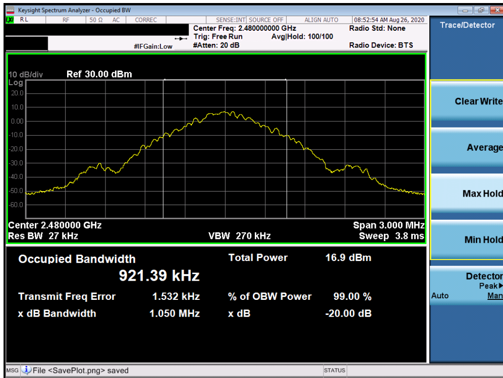
Plot 7-3. 20dB Bandwidth Plot (Bluetooth, GFSK, iPA – Ch. 78)
