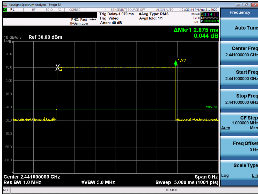
Plot 7-17. Time of Occupancy Plot (Bluetooth, GFSK, iPA)
