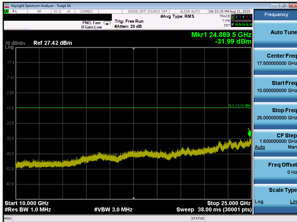
Plot 7-26. Conducted Spurious Plot (Bluetooth, GFSK, iPA Ch. 39)
