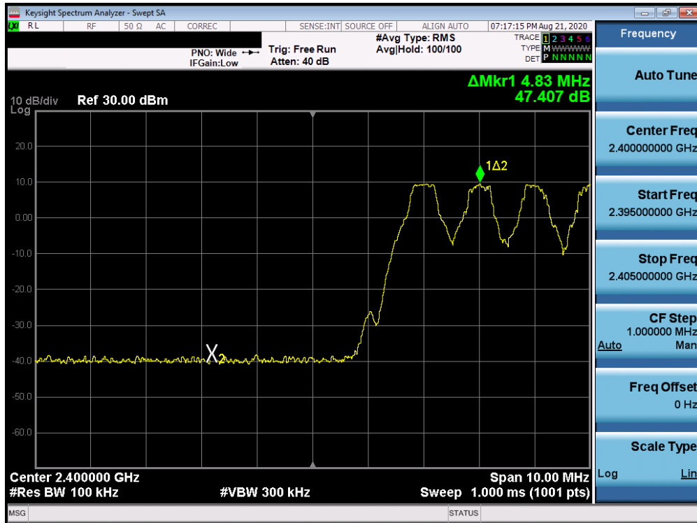
Plot 7-9. Band Edge Plot (Bluetooth with Hopping Enabled, GFSK, iPA)
