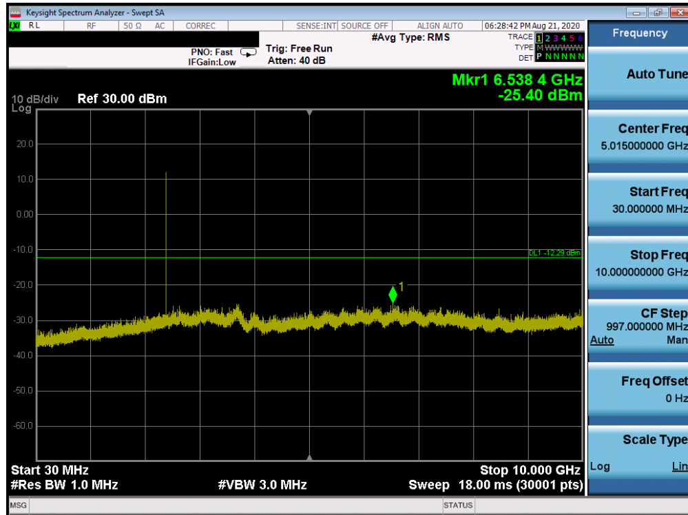
Plot 7-23. Conducted Spurious Plot (Bluetooth, GFSK, iPA – Ch. 0)
