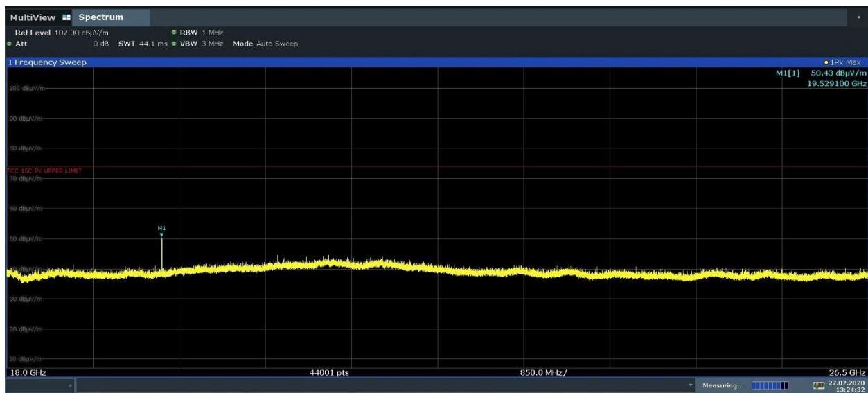
Plot 7-35. Radiated Spurious Emissions 18-26.5GHz (GFSK ePA – Ch. 39, Pol. V)
