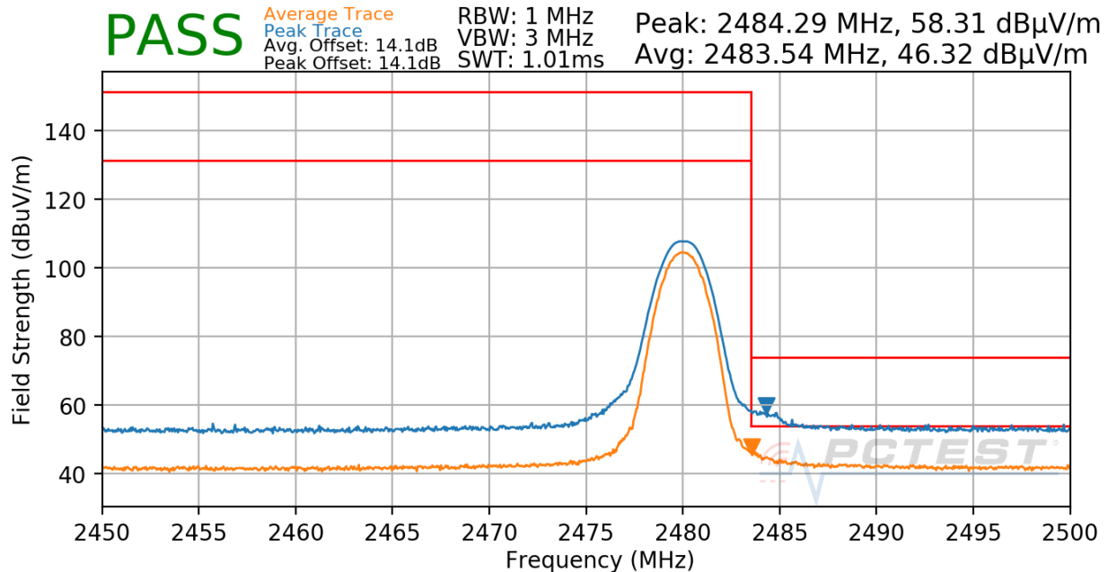
Plot 7-41. Radiated Restricted Upper Band Edge Measurement
