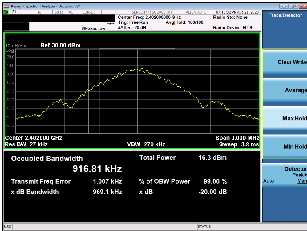
Plot 7-1. 20dB Bandwidth Plot (Bluetooth, GFSK, iPA – Ch. 0)
