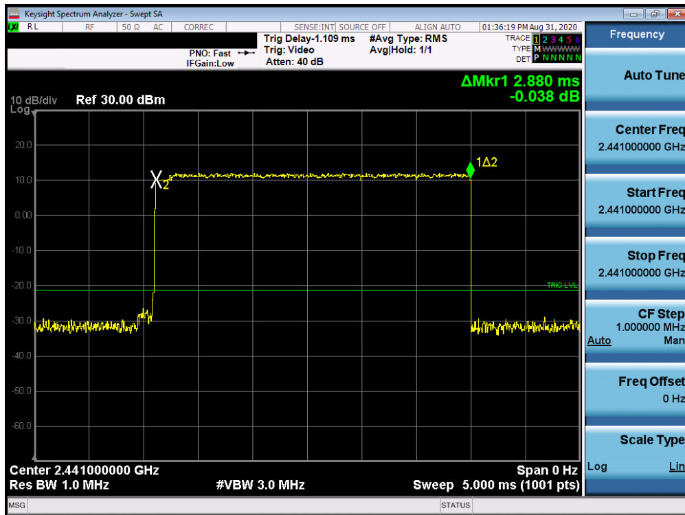
Plot 7-18. Time of Occupancy Plot (Bluetooth, \pi/4 -DQPSK, iPA)
