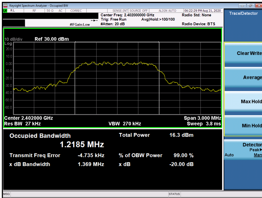
Plot 7-4. 20dB Bandwidth Plot (Bluetooth, \pi/4 -DQPSK, iPA – Ch. 0)
