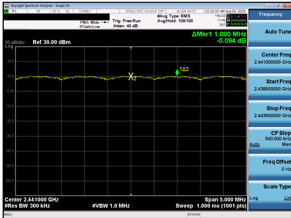
Plot 7-16. Channel Spacing Plot (Bluetooth, \pi/4 -DQPSK, iPA)
