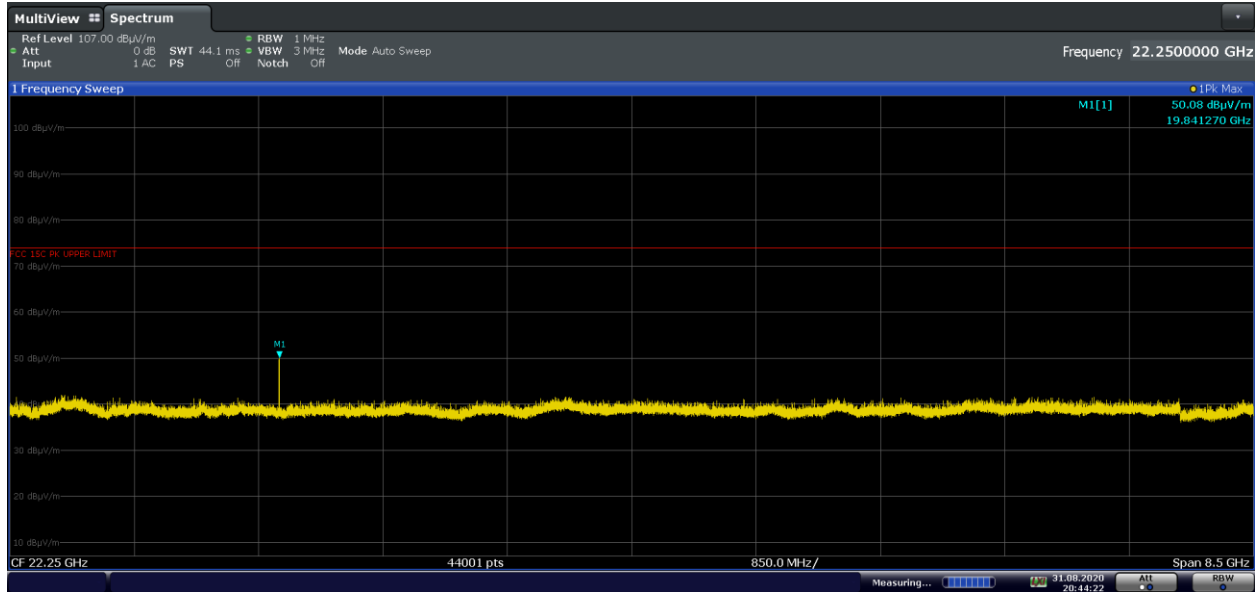
Plot 7-36. Radiated Spurious Emissions 18-26.5GHz (GFSK iPA – Ch.78, Pol. H)
