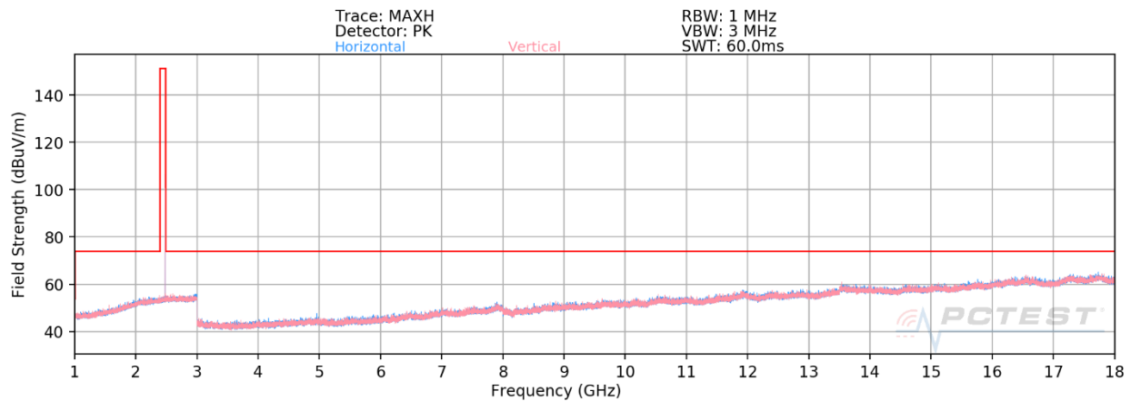
Plot 7-31. Radiated Spurious Emissions 1-18GHz (BT GFSK iPA – Ch. 78)
