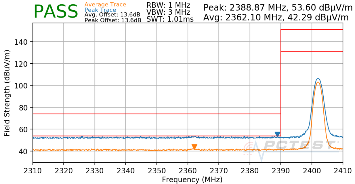
Plot 7-39. Radiated Restricted Lower Band Edge Measurement
