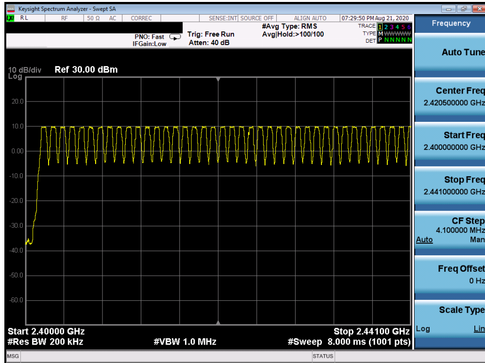
Plot 7-19. Low End Spectrum Channel Hopping Plot (Bluetooth, GFSK, iPA)
