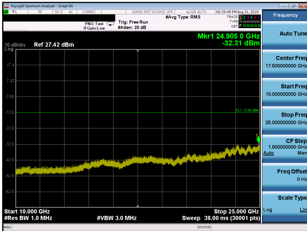
Plot 7-28. Conducted Spurious Plot (Bluetooth, GFSK, iPA – Ch. 78)
