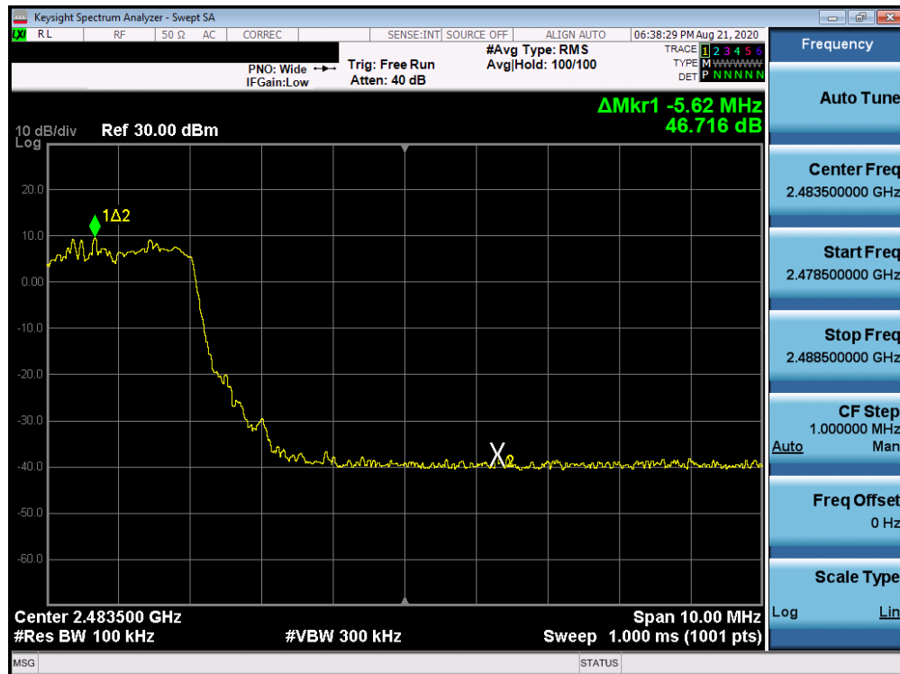
Plot 7-14. Band Edge Plot (Bluetooth with Hopping Enabled, \pi/4 -DQPSK, iPA)
