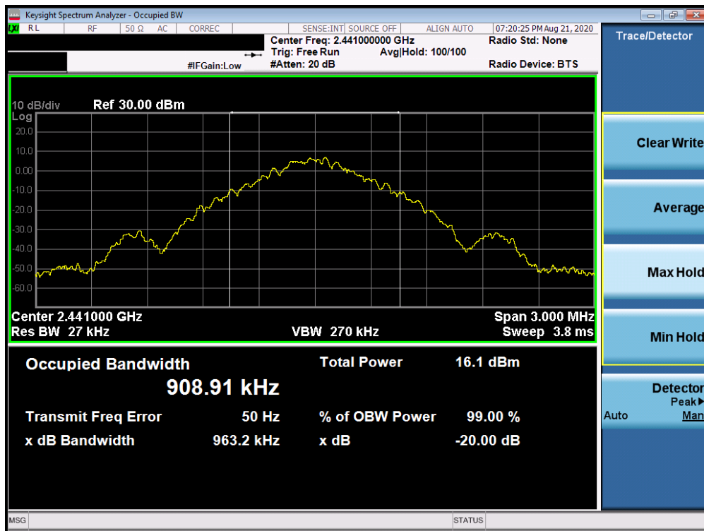
Plot 7-2. 20dB Bandwidth Plot (Bluetooth, GFSK, iPA – Ch. 39)
