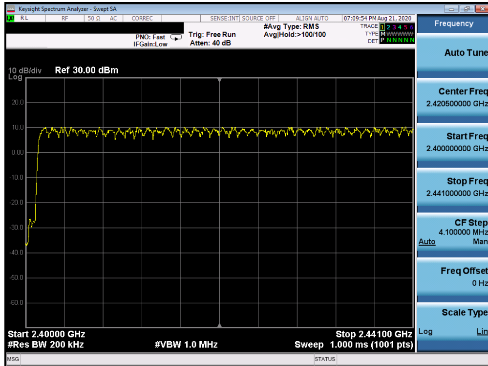
Plot 7-21. Low End Spectrum Channel Hopping Plot (Bluetooth, \pi/4 -DQPSK, iPA)
