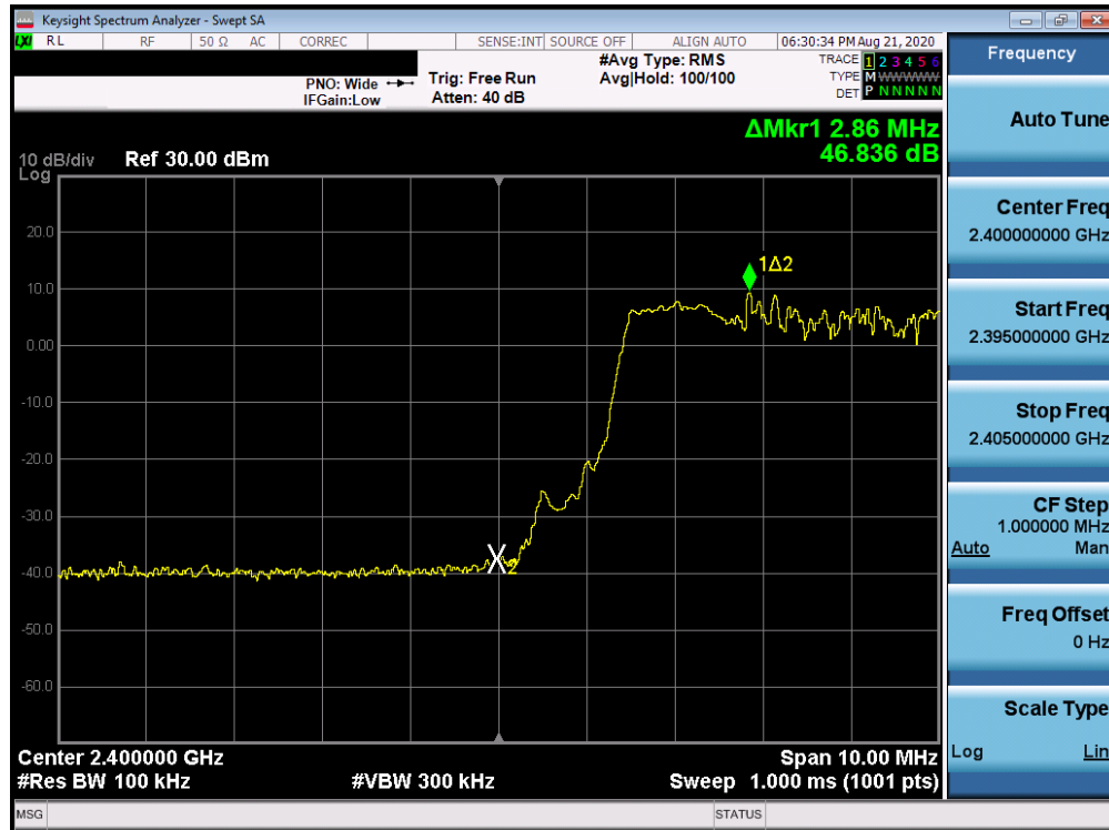
Plot 7-13. Band Edge Plot (Bluetooth with Hopping Enabled, \pi/4 -DQPSK, iPA)
