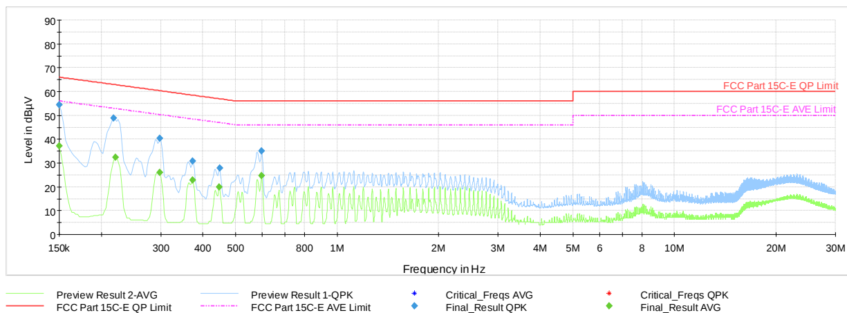
Plot 7-43. AC Line-Conducted Plot with GFSK iPA Ch.39 (L1, with Laptop)
