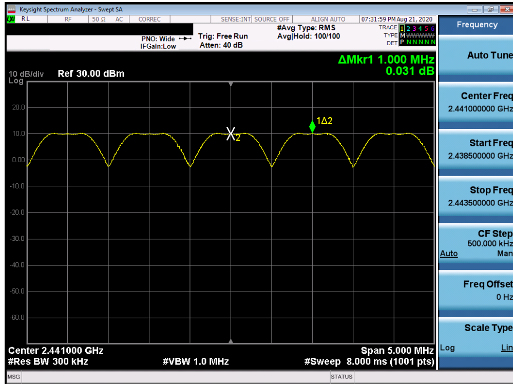
Plot 7-15. Channel Spacing Plot (Bluetooth, GFSK, iPA)
