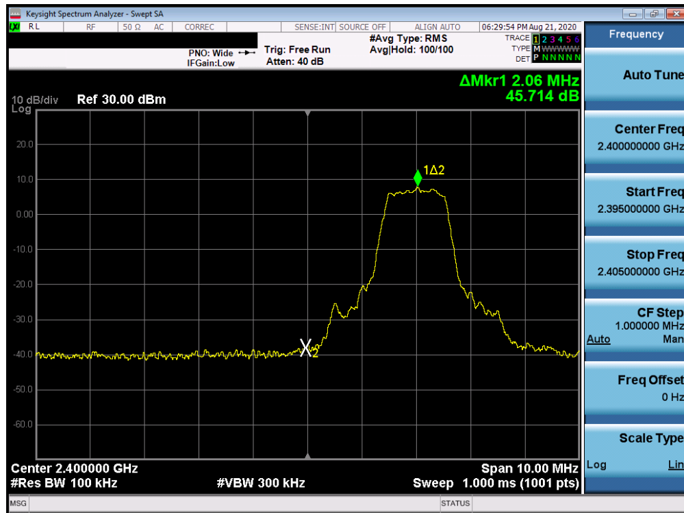
Plot 7-11. Band Edge Plot (Bluetooth with Hopping Disabled, \pi/4 -DQPSK, iPA – Ch. 0)
