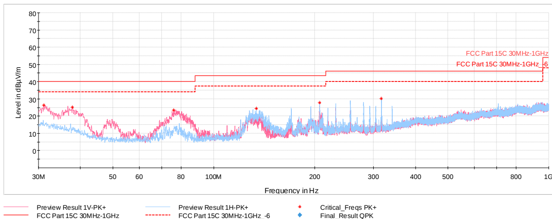
Plot 7-42. Radiated Spurious Emissions 30MHz-1GHz (GFSK iPA – Ch.39, with AC/DC Adapter)
