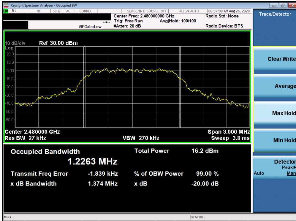
Plot 7-6. 20dB Bandwidth Plot (Bluetooth, \pi/4 -DQPSK, iPA – Ch. 78)
