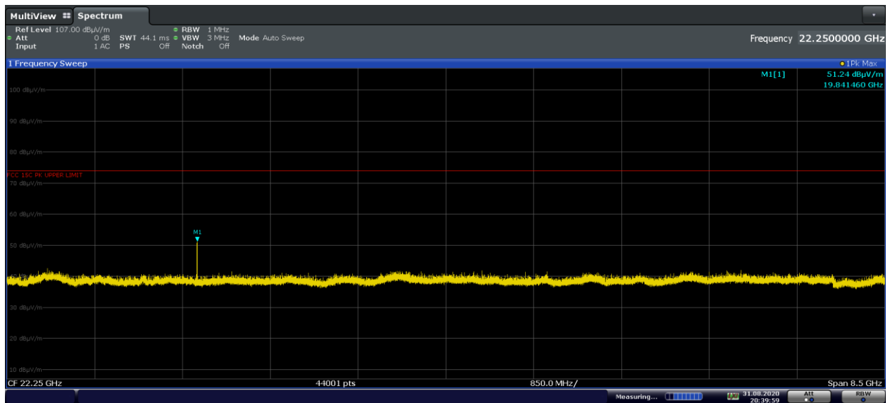
Plot 7-37. Radiated Spurious Emissions 18-26.5GHz (GFSK iPA – Ch.78, Pol. V)
