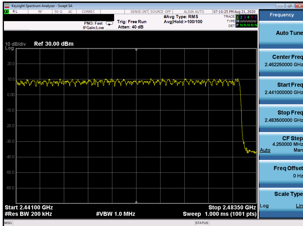
Plot 7-22. High End Spectrum Channel Hopping Plot (Bluetooth, \pi/4 -DQPSK, iPA)
