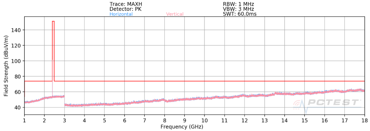
Plot 7-29. Radiated Spurious Emissions 1-18GHz (BT GFSK iPA – Ch. 0)
