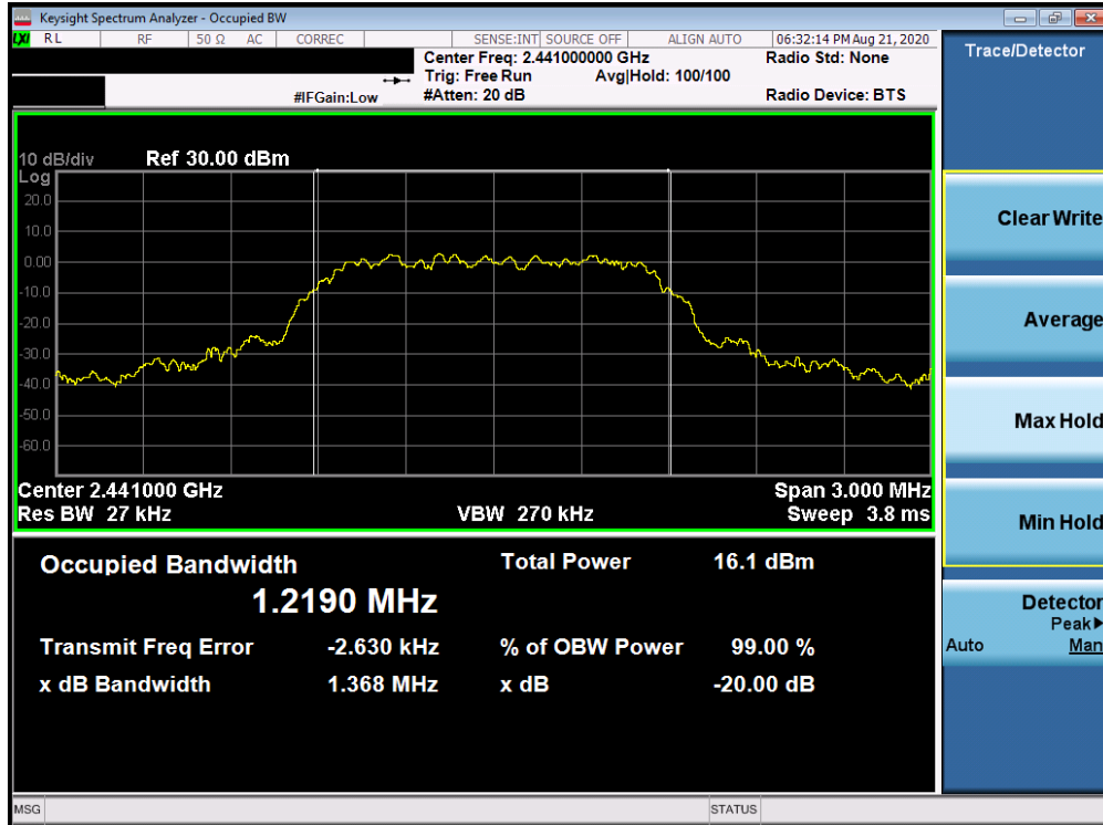
Plot 7-5. 20dB Bandwidth Plot (Bluetooth, \pi/4 -DQPSK, iPA – Ch. 39)
