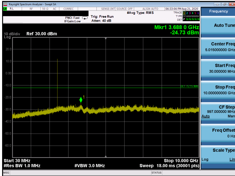
Plot 7-25. Conducted Spurious Plot (Bluetooth, GFSK, iPA – Ch. 39)
