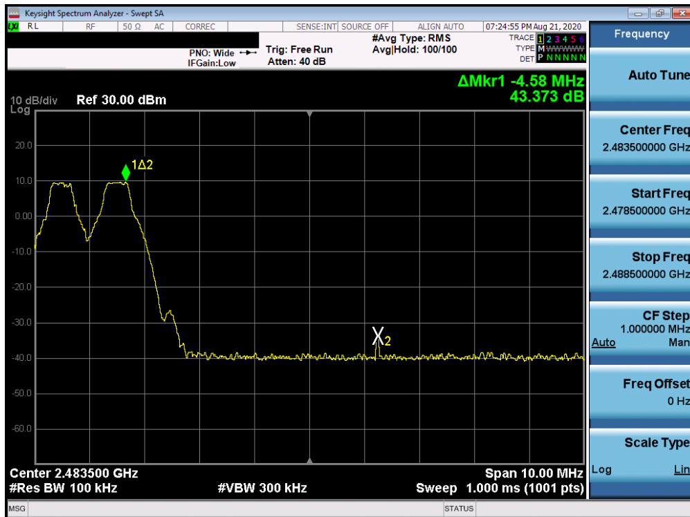
Plot 7-10. Band Edge Plot (Bluetooth with Hopping Enabled, GFSK, iPA)
