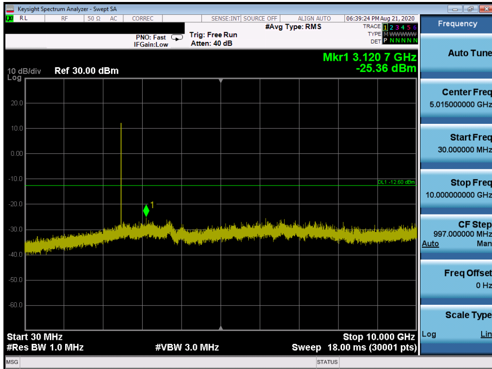
Plot 7-27. Conducted Spurious Plot (Bluetooth, GFSK, iPA – Ch. 78)
