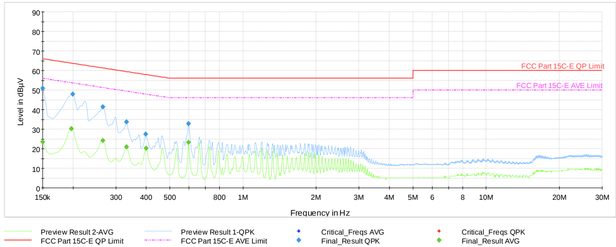
Plot 7-44. AC Line-Conducted Plot with GFSK iPA Ch.39 (N, with Laptop)
