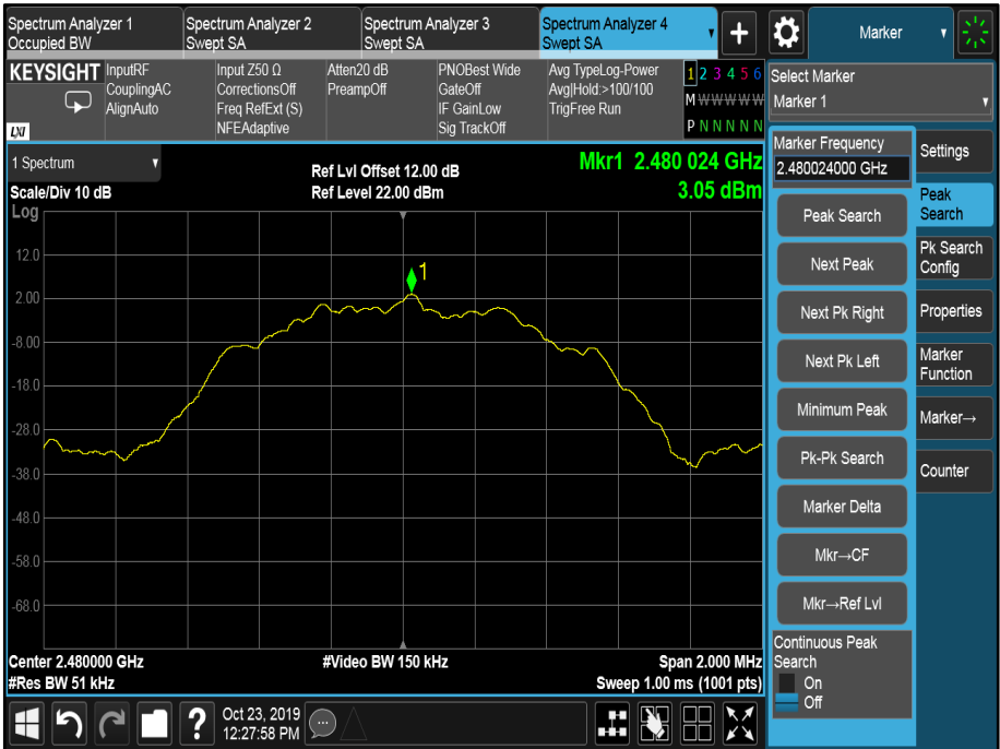
Figure 24 - 2480 MHz, Power Spectral Density
